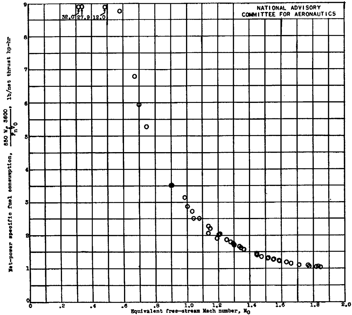
Figure 15.- Effect of equivalent free-stream Mach number M_0 on net-power specific fuel consumption \frac{550 W_p 3600}{P_n V_n} . 20-inch ram jet with 5-foot combustion chamber and 16.8-inch-diameter exhaust nozzle.
