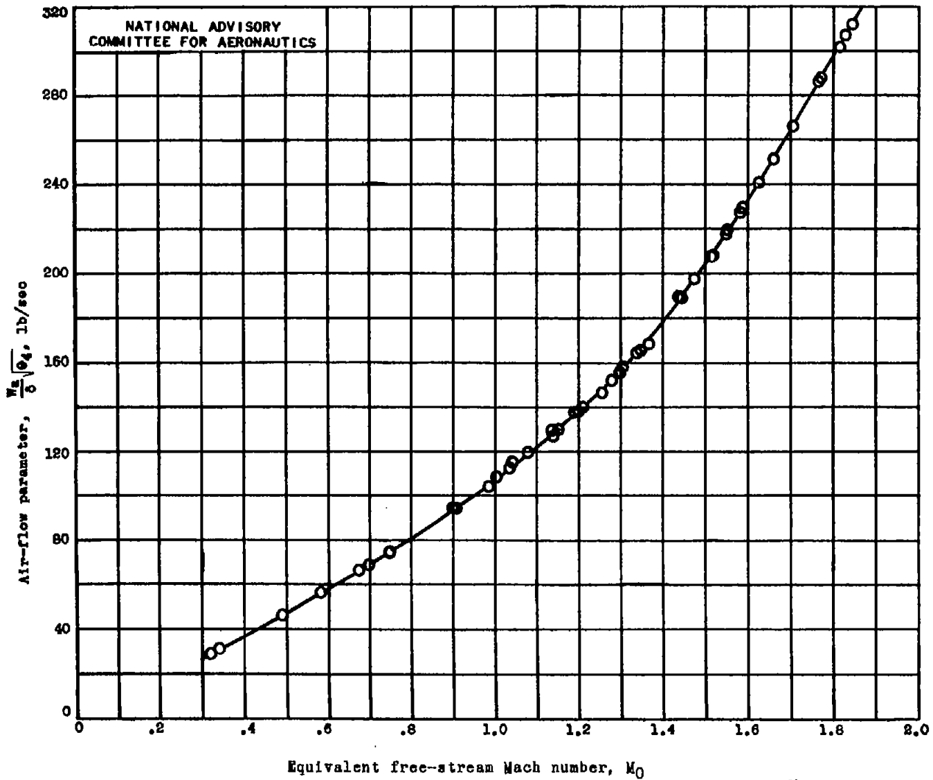
Figure 18.—Effect of equivalent free-stream Mach number M_0 on air-flow parameter \frac{W_0}{5} \sqrt{\theta_4} . 20-inch ram jet with 5-foot combustion chamber and 16.8-inch-diameter exhaust nozzle.
