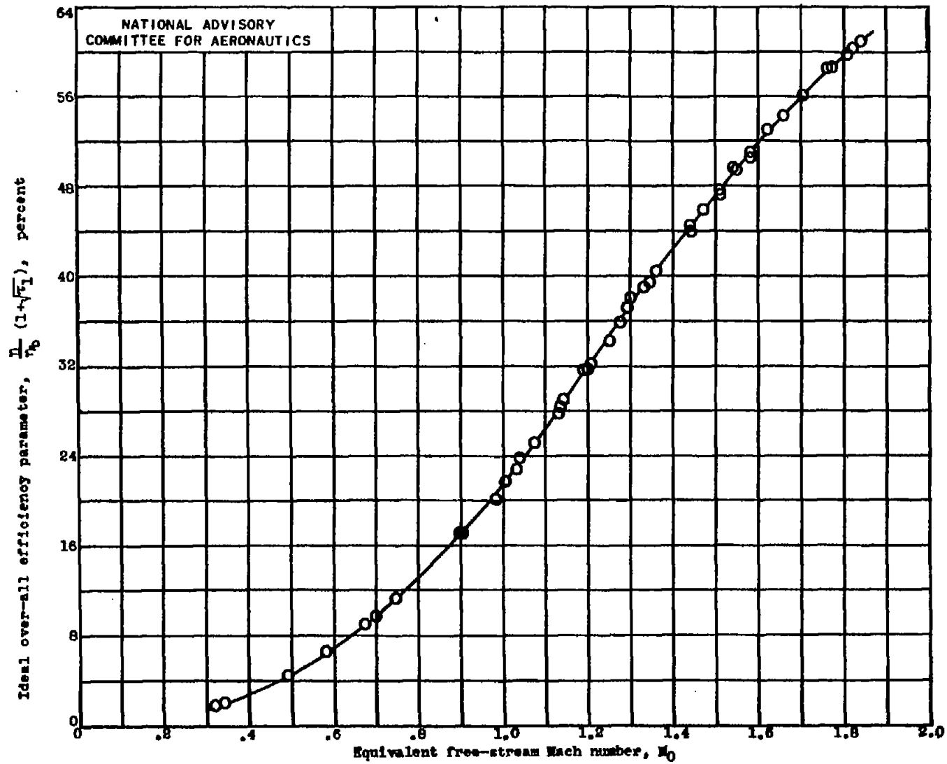
Figure 10.- Effect of equivalent free-stream Mach number M_0 on ideal over-all efficiency parameter \frac{\eta}{\eta_b} (1 + \sqrt{\tau_1}) . 20-inch ram jet with 5-foot combustion chamber and 16.8-inch-diameter exhaust nozzle.
