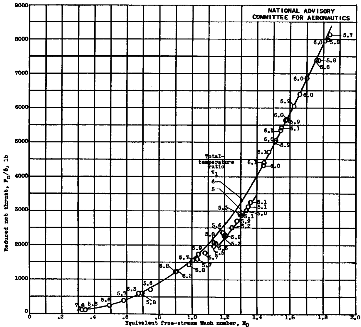
Figure 8.- Effect of equivalent free-stream Mach number M_0 and total-temperature ratio \tau_1 on reduced net thrust F_N/S . 20-inch ram jet with 5-foot combustion chamber and 16.8-inch-diameter exhaust nozzle; net thrust reduced to NACA standard atmospheric conditions at sea level.
