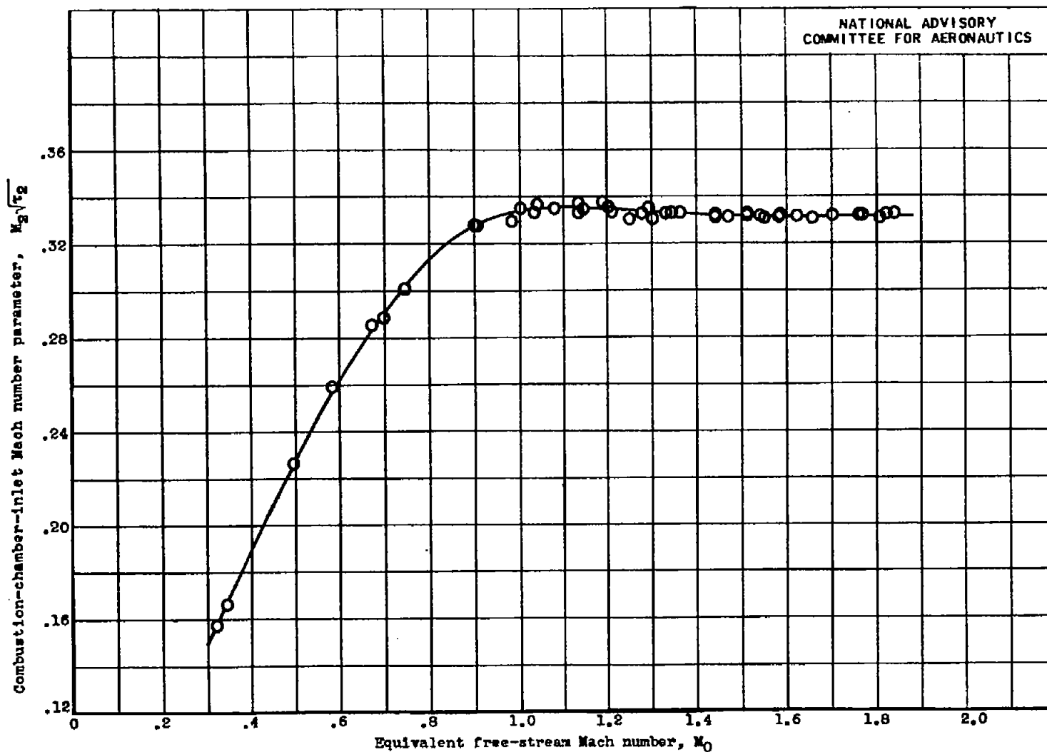
Figure 17.- Effect of equivalent free-stream Mach number M_0 on combustion-chamber-inlet Mach number parameter M_2\sqrt{\tau_2} . 20-inch ram jet with 5-foot combustion chamber and 16.8-inch-diameter exhaust nozzle.
