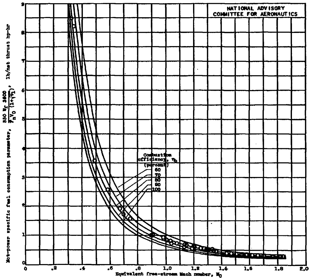
Figure 13.- Effect of equivalent free-stream Mach number M_0 and combustion efficiency \eta_c on net-power specific fuel consumption parameter \frac{550 W_f 3600}{F_n V_0 (1 + \gamma_1)} . 20-inch ram jet with 5-foot combustion chamber and 16.8-inch-diameter exhaust nozzle.
