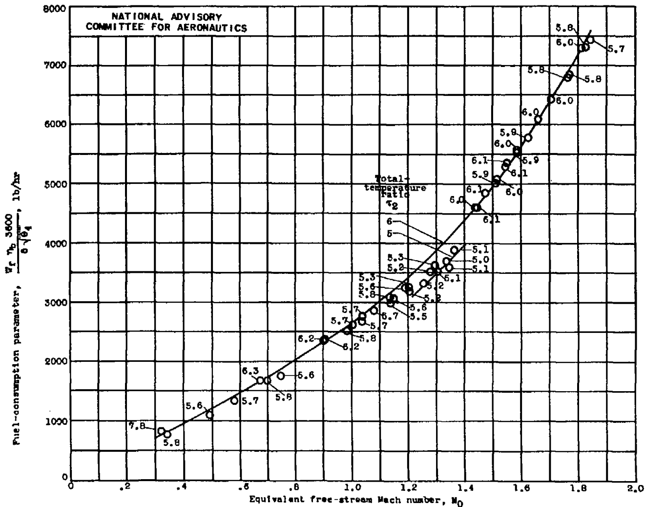
Figure 19.- Effect of equivalent free-stream Mach number M_0 and total-temperature ratio \tau_2 on fuel-consumption parameter \frac{W_f \eta_b 3600}{6 \sqrt{\theta_4}} . 20-inch ram jet with 5-foot combustion chamber and 16.8-inch-diameter exhaust nozzle.
