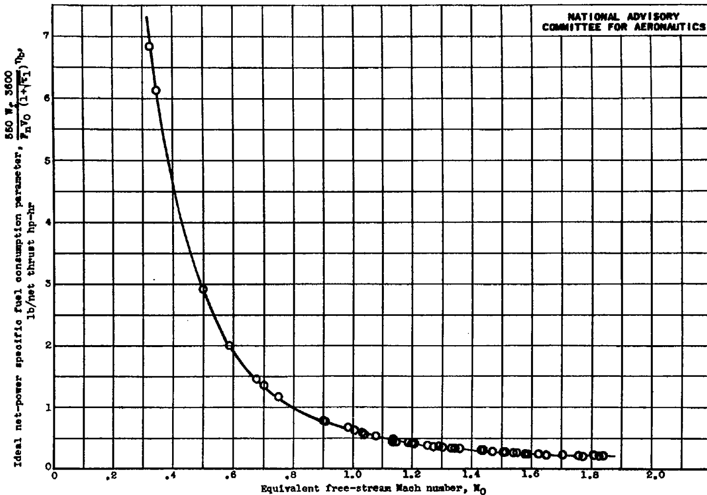
Figure 11.- Effect of equivalent free-stream Mach number M_0 on ideal net-power specific fuel consumption parameter \frac{560 W_f 3600}{F_n V_0 (1 + \sqrt{\epsilon})} \eta_b . 20-inch ram jet with 5-foot combustion chamber and 16.8-inch-diameter exhaust nozzle.
