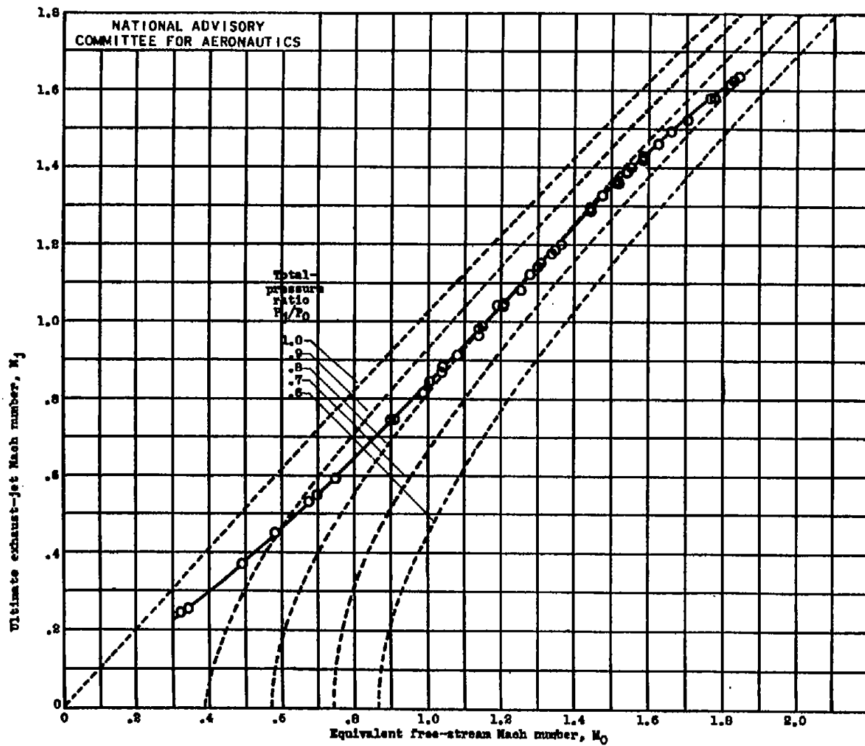
Figure 16.- Effect of equivalent free-stream Mach number M_0 and total-pressure ratio across ram jet P_j/P_0 on ultimate exhaust-jet Mach number M_j . Total-pressure ratio curves calculated for ratio of specific heats at exhaust-jet condition \gamma_j = 1.3 and at free-stream condition \gamma_0 = 1.4 . 20-inch ram jet with 5-foot combustion chamber and 10.8-inch-diameter exhaust nozzle.
