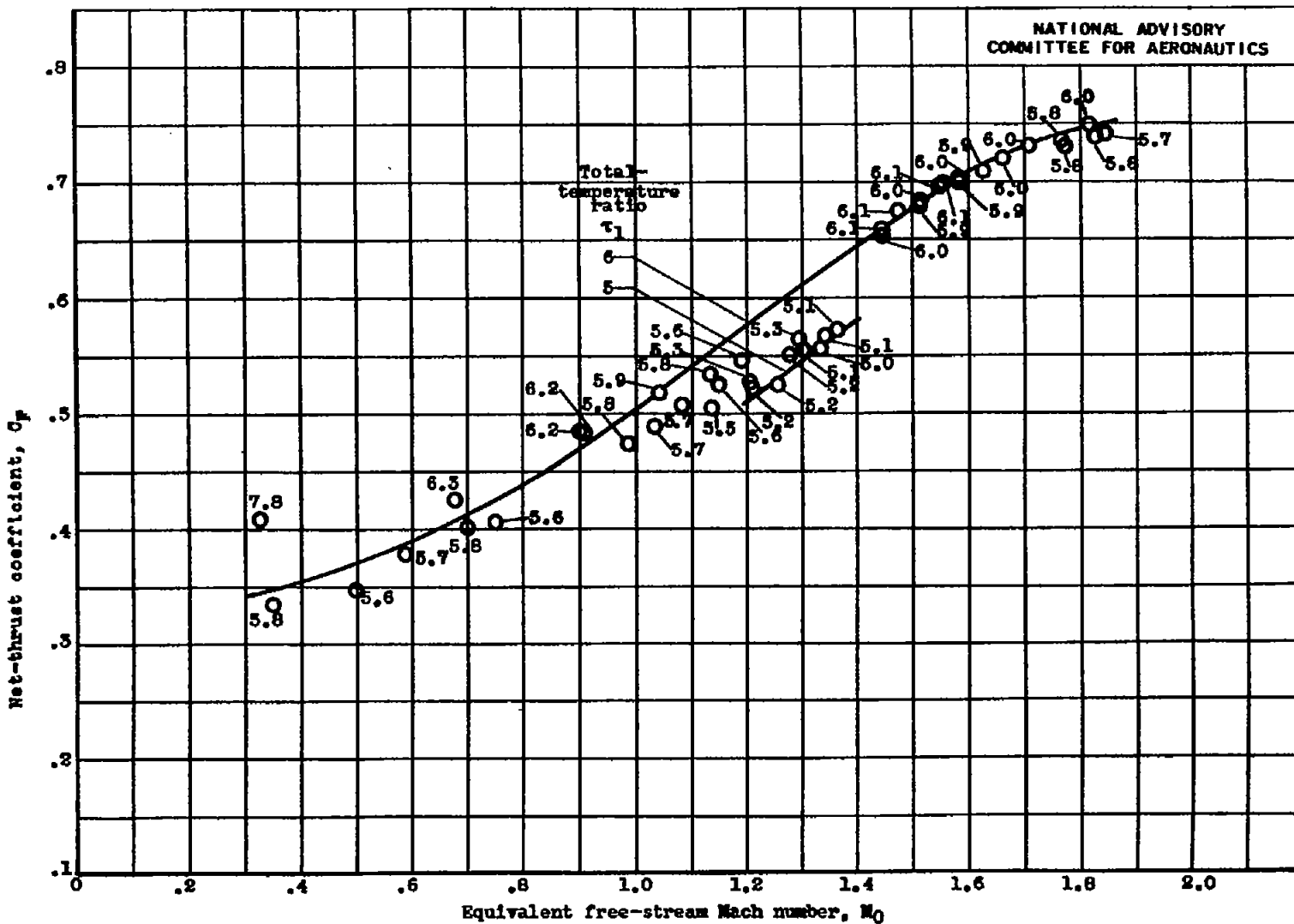
Figure 9.- Effect of equivalent free-stream Mach number M_0 and total-temperature ratio \tau_1 on net-thrust coefficient C_p . 20-inch ram jet with 5-foot combustion chamber and 16.8-inch-diameter exhaust nozzle.
