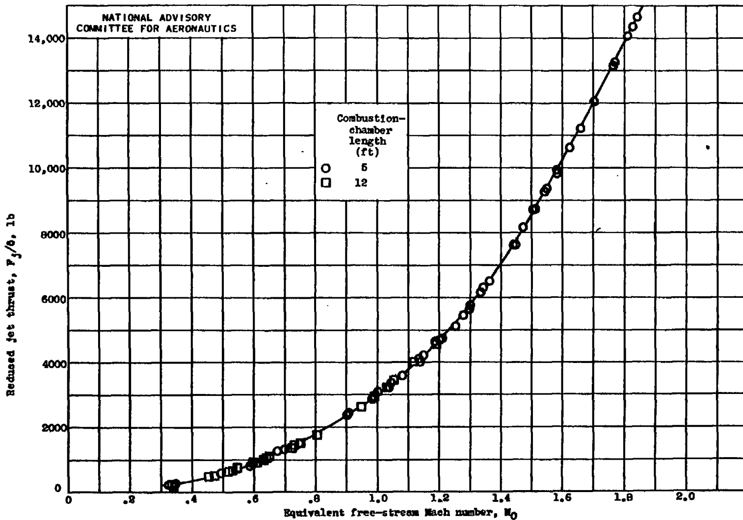
Figure 6.- Effect of equivalent free-stream Mach number M_0 and combustion-chamber length on reduced jet thrust F_j/\delta . 20-inch ram jet with 16.8-inch-diameter exhaust nozzle; jet thrust reduced to NACA standard atmospheric conditions at sea level.
