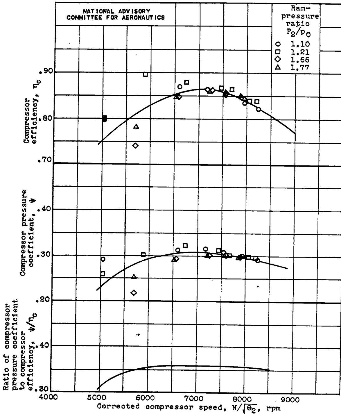
Figure 3.- Relation among compressor efficiency, compressor pressure coefficient, ratio of compressor coefficient to compressor efficiency, and corrected compressor speed. Compressor speed corrected to NACA standard atmospheric conditions at sea level.
