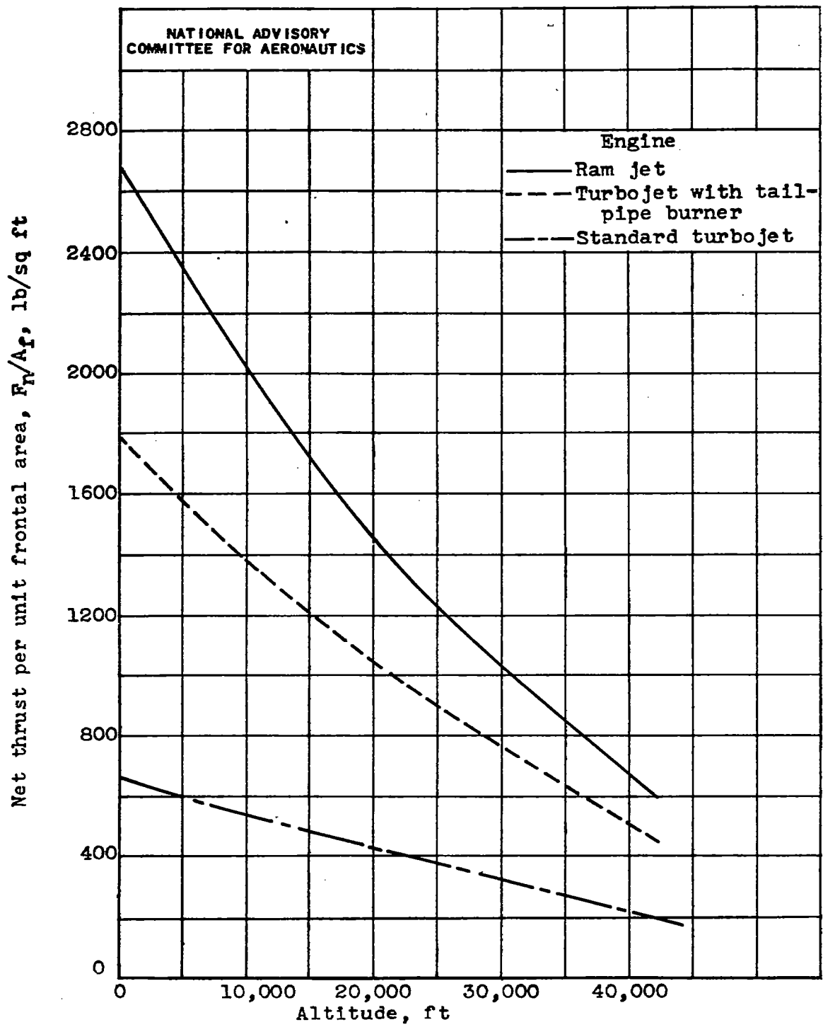
(b) Flight Mach number M_0 , 1.6. Figure 8.- Concluded. Relation between net thrust per unit frontal area and altitude for three jet-propulsion engines. Engines operating at respective limiting conditions; 100-percent ram recovery.
