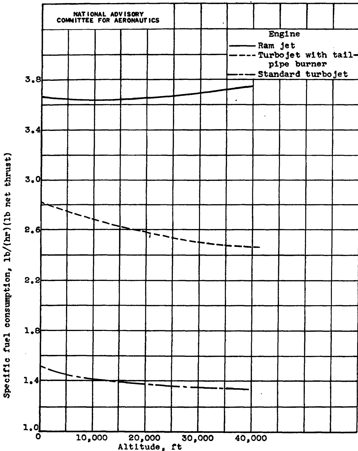
Figure 9.- Relation between specific fuel consumption based on net thrust and altitude for three jet-propulsion engines. Engines operating at respective limiting conditions; 100-percent ram recovery.
