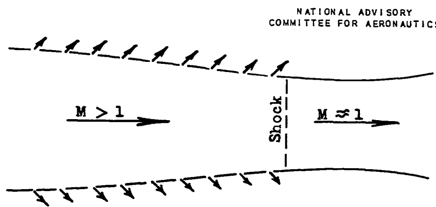
(c) Normal shock near throat.
