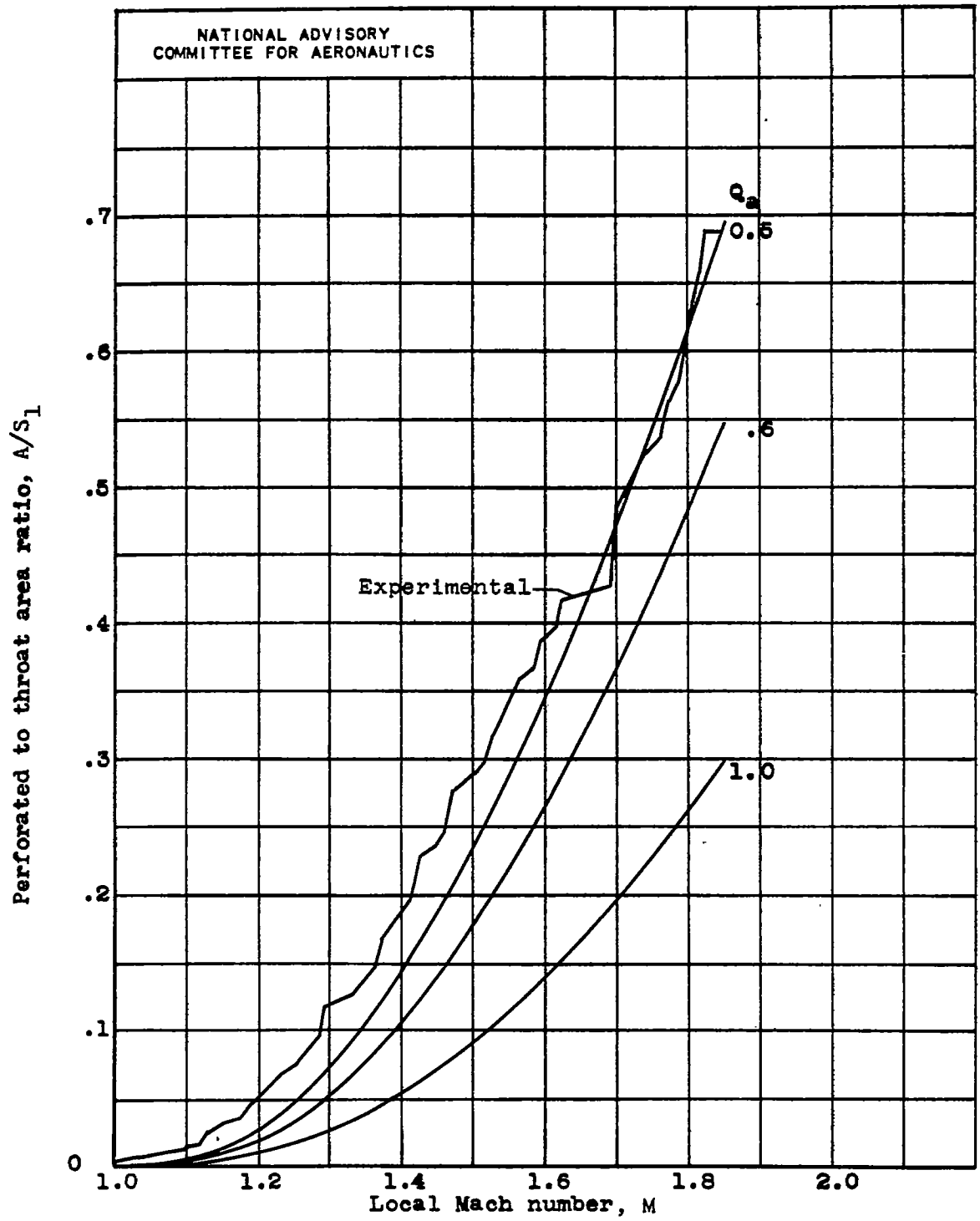
Figure 9.- Distribution of perforated area. Free-stream Mach number, 1.85. (Theoretical curves calculated with equation (17).)
