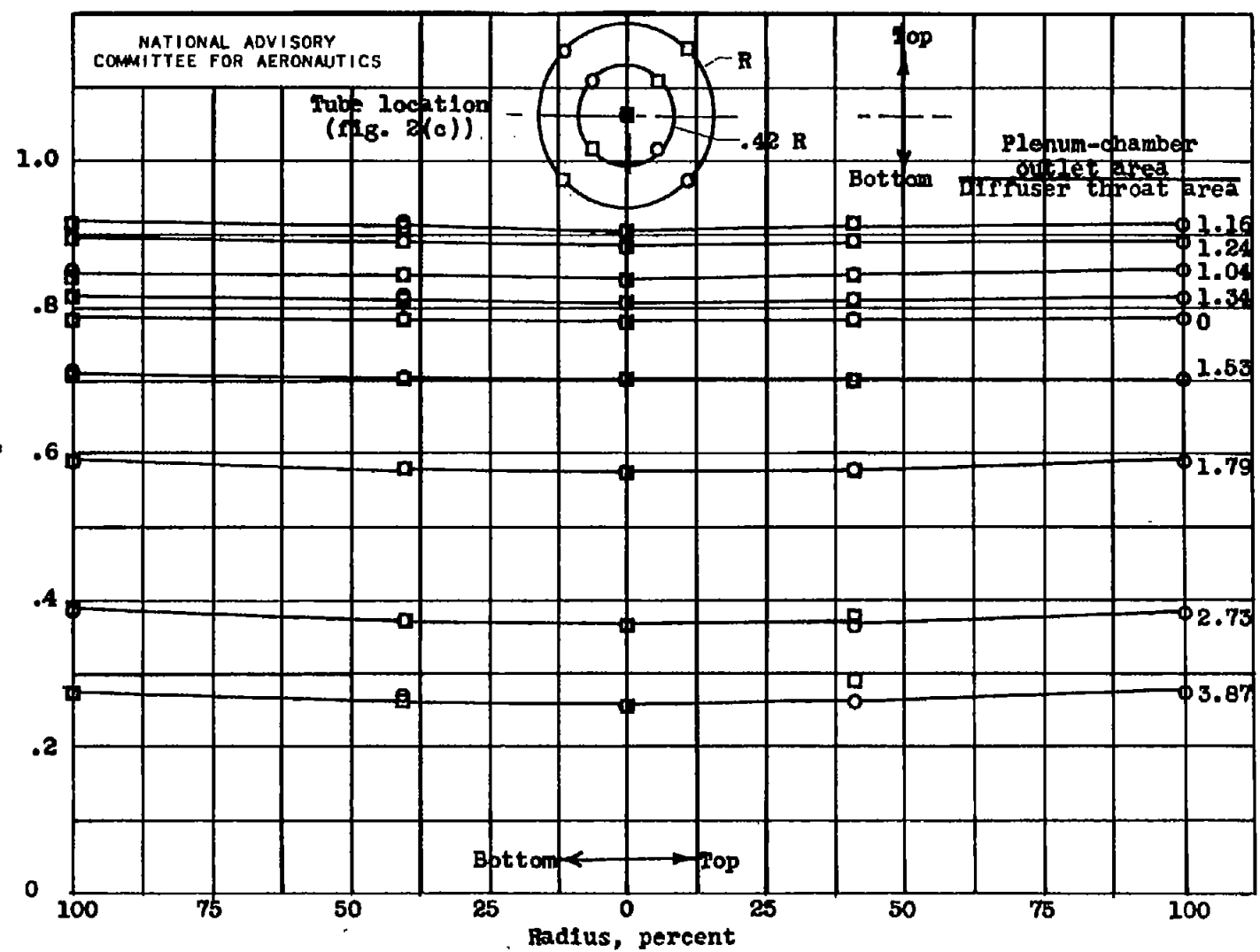
(a) Angle of attack, 0°. Figure 5.- Static-pressure distribution across diffuser outlet. Free-stream Mach number, 1.85.
