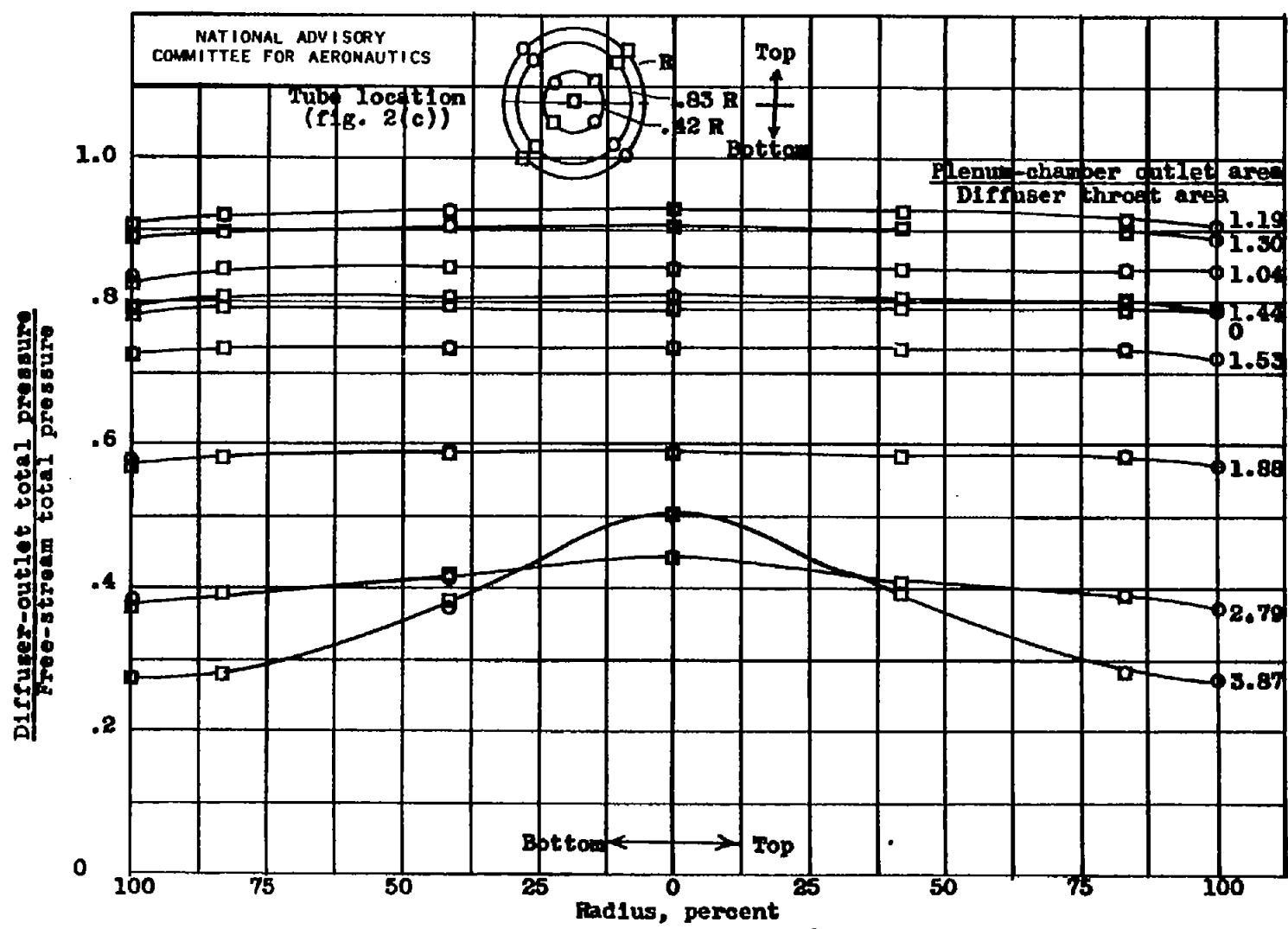
(b) Angle of attack, 3°. Figure 6.- Continued. Total-pressure distribution across diffuser outlet. Free-stream Mach number, 1.85.
