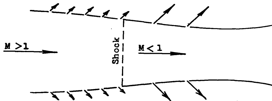
(b) Normal shock partly swallowed.
