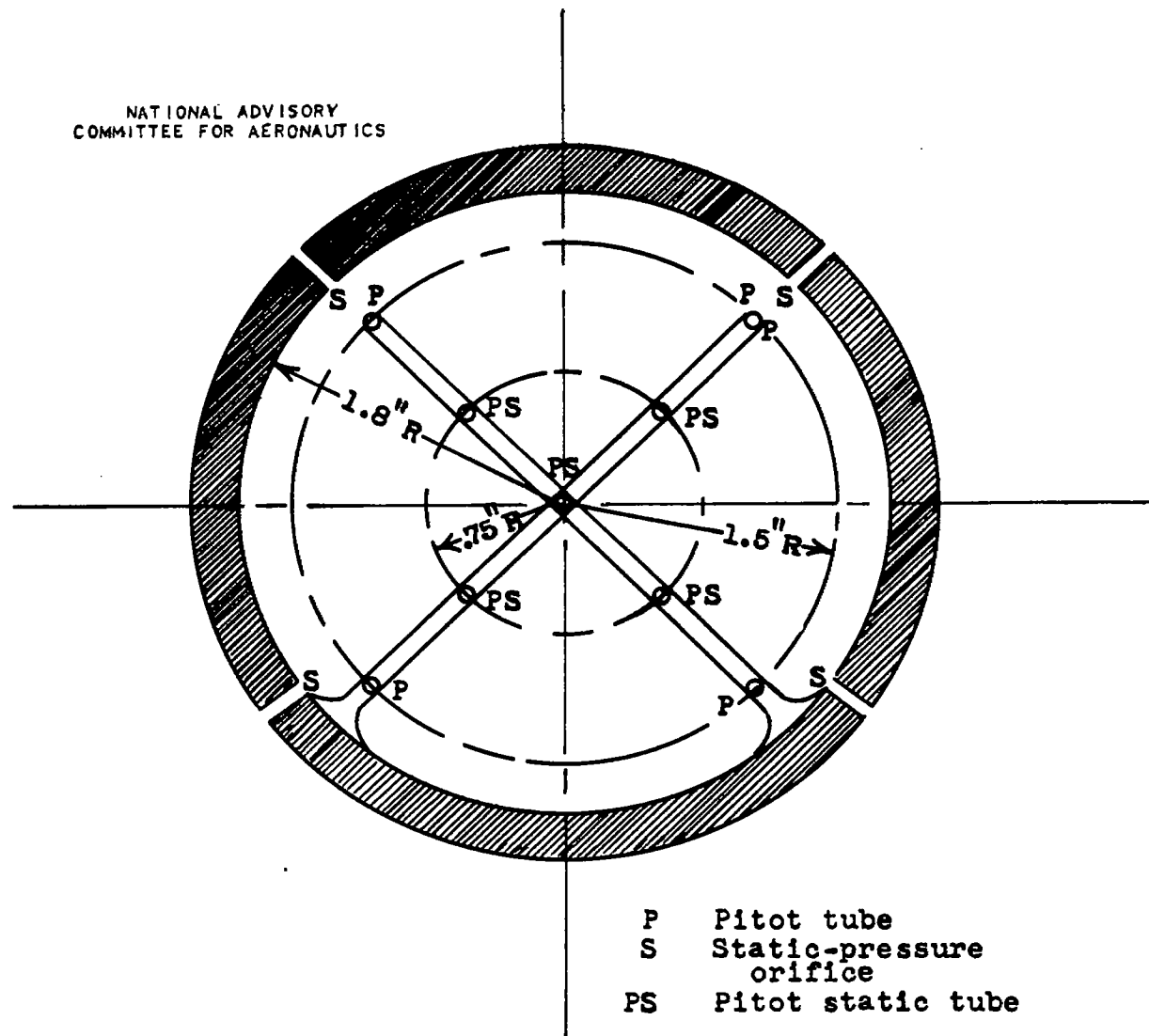
Cross section at AA (fig. 2(b))
