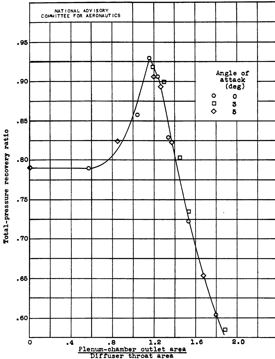
Figure 3.- Total-pressure recovery of perforated supersonic diffuser. Free-stream Mach number, 1.85.
