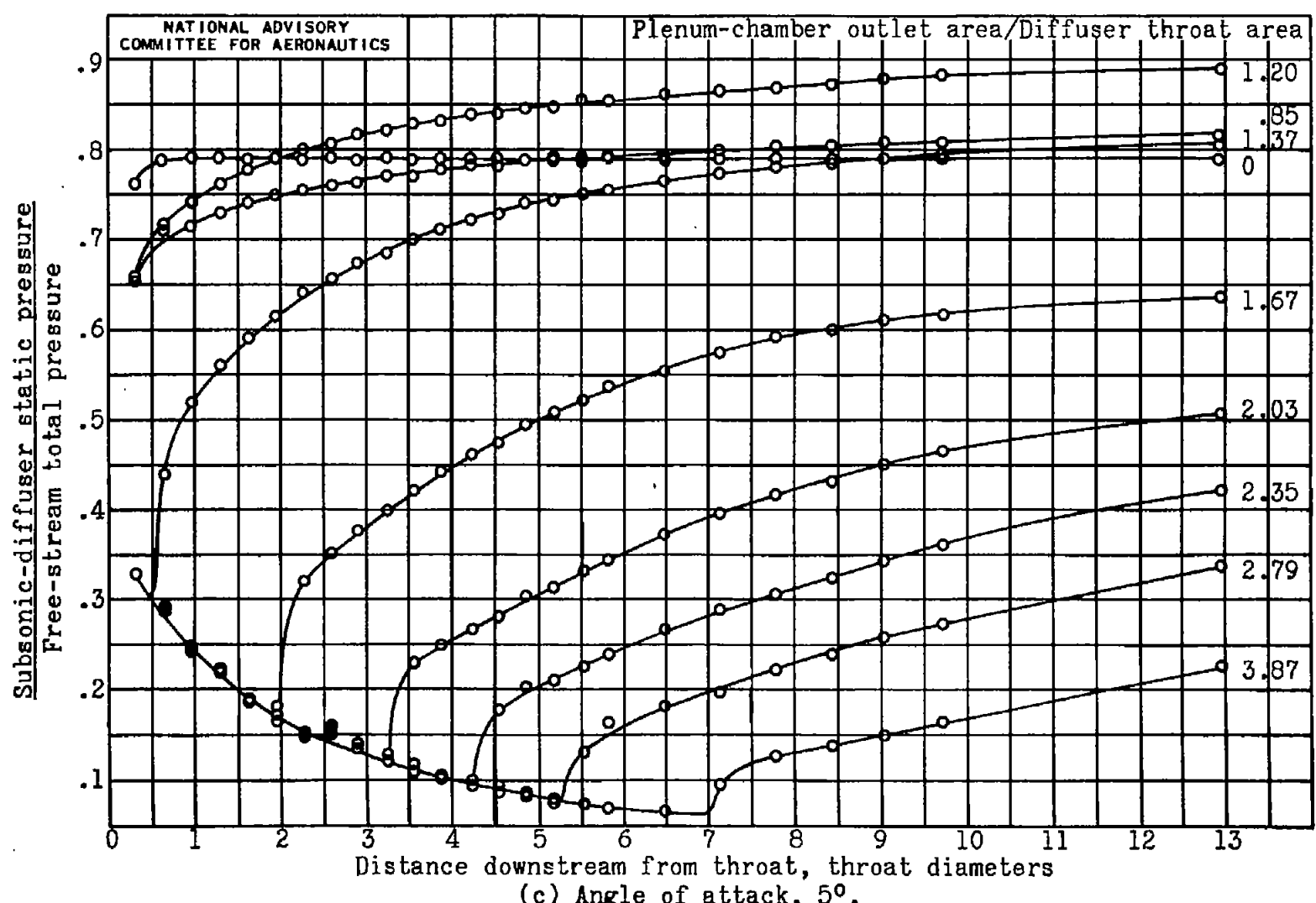
Figure 4.- Concluded. Static-pressure distribution along subsonic diffuser. Free stream Mach number, 1.85.
