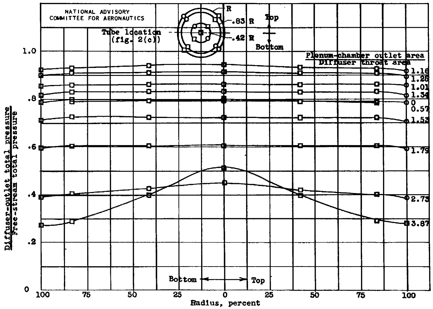
(a) Angle of attack, 0°. Figure 6.- Total-pressure distribution across diffuser outlet. Free-stream Mach number, 1.85.
