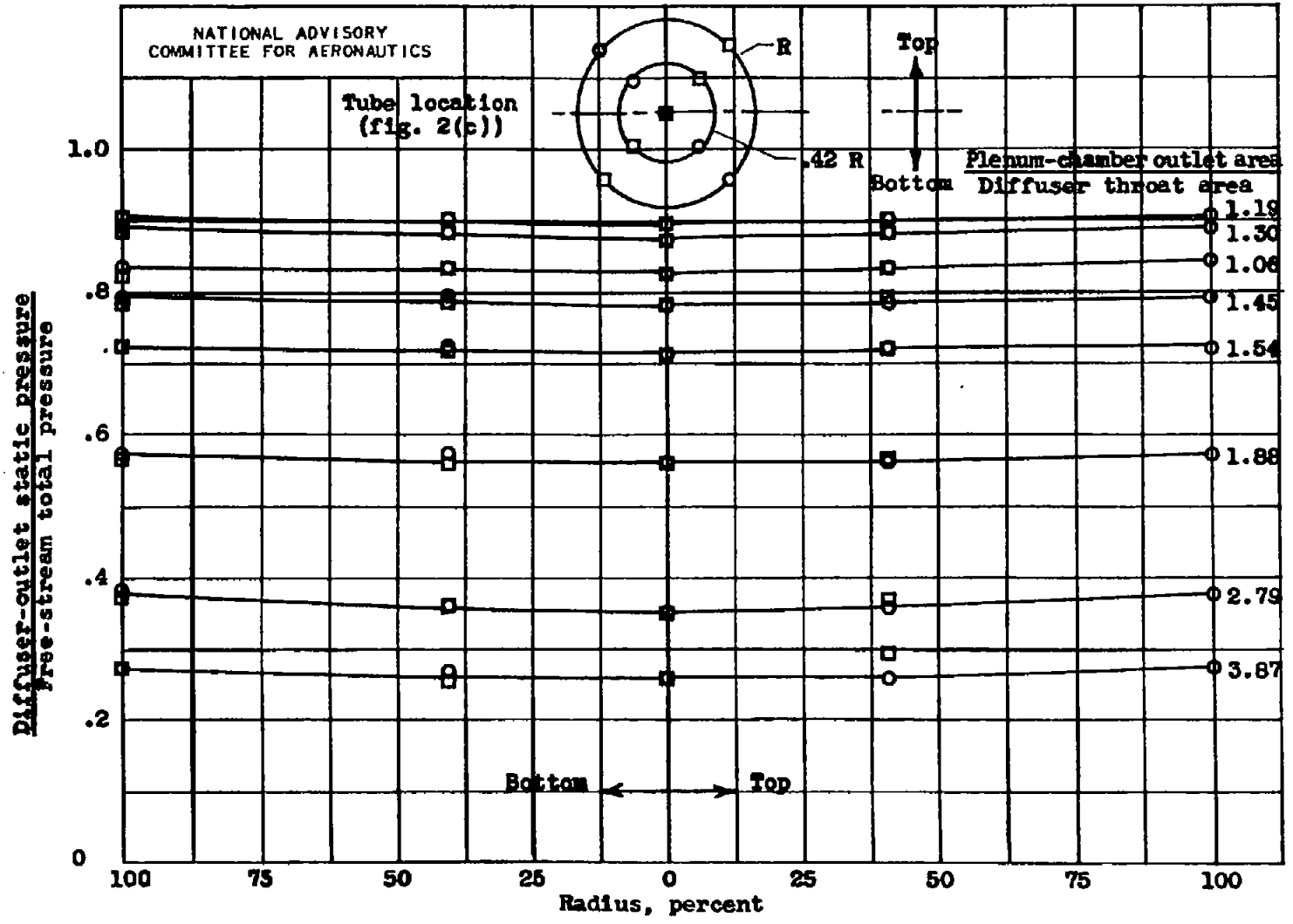
(b) Angle of attack, 3°.
