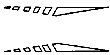
Busemann biplane
