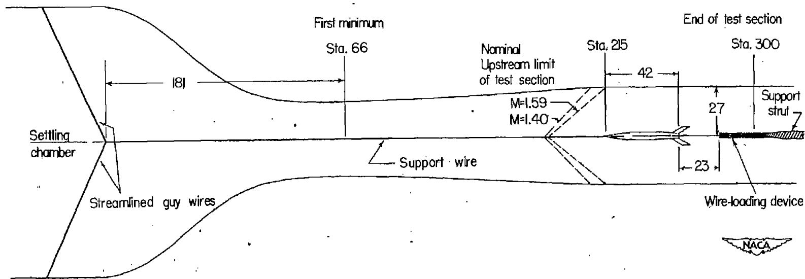
Figure 3.- Test setup for wire-supported model. All dimensions are in inches.
