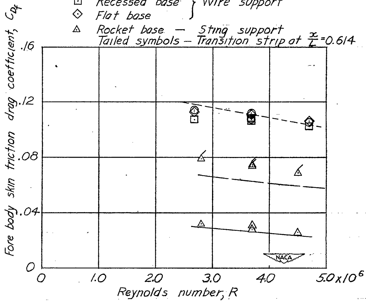
Figure 14.- Variation with Reynolds number of the forebody skin-friction coefficient of the wire- and sting-supported models (body alone). M = 1.59.
