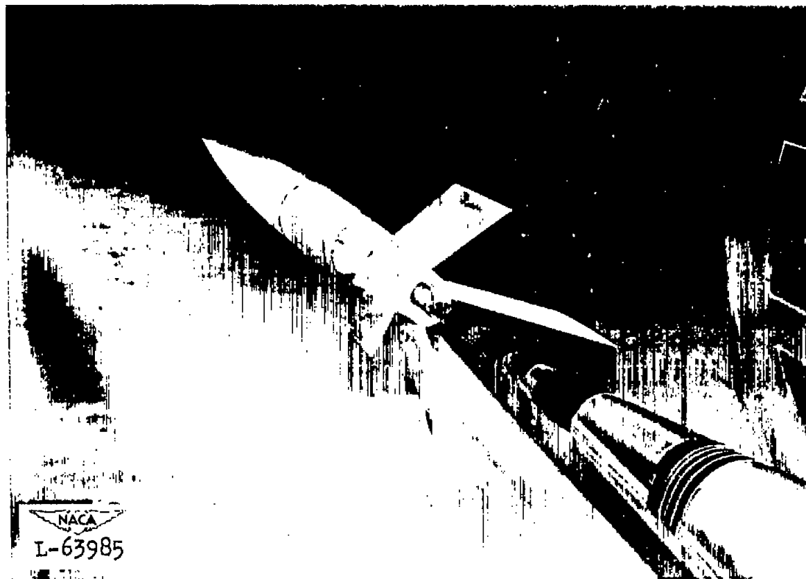
Figure 5.- Photograph of sting-supported model.
