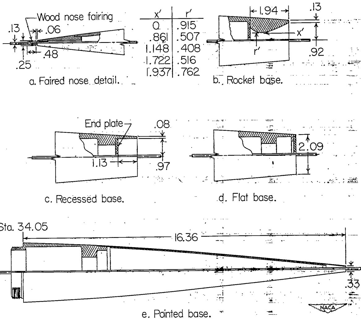
Figure 2.- Nose and base details of wire-supported model. All dimensions are in inches.
