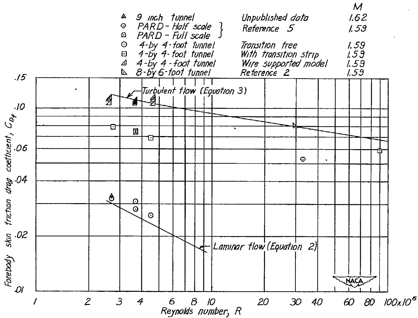
Figure 21.- Variation of forebody skin-friction drag coefficient over a large Reynolds number range near a Mach number of 1.6. \alpha = 0^\circ .
