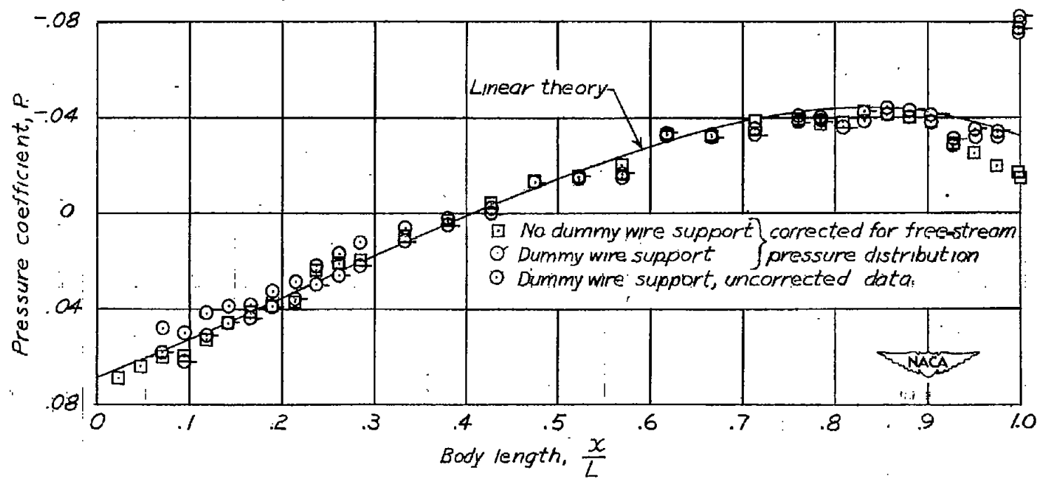
Figure 8.- Pressure distribution obtained on pressure model with and without the dummy wire support. M = 1.59 ; R = 3.7 \times 10^6 .
