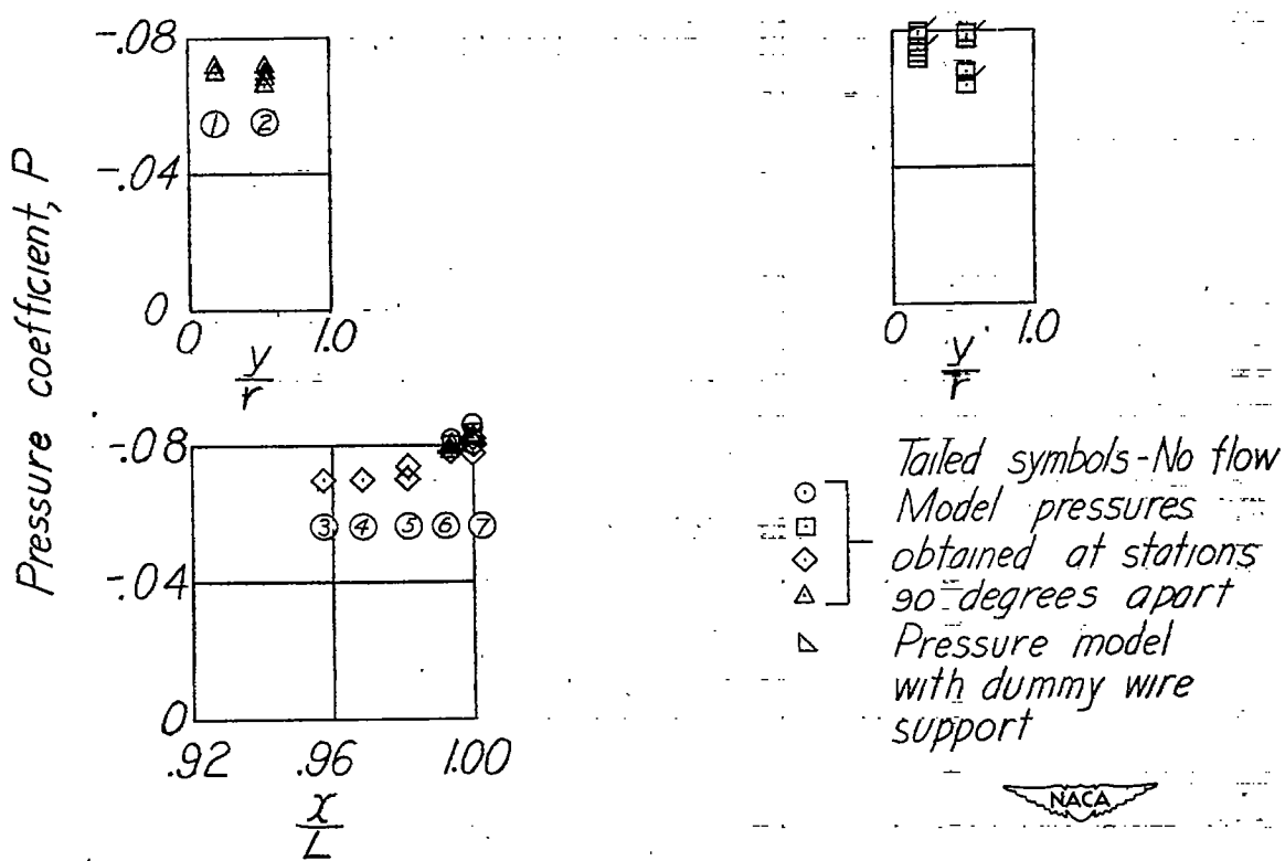
Figure 12.- Effect of wire support on base pressure distribution. M = 1.59 ; R = 3.7 \times 10^6 .
