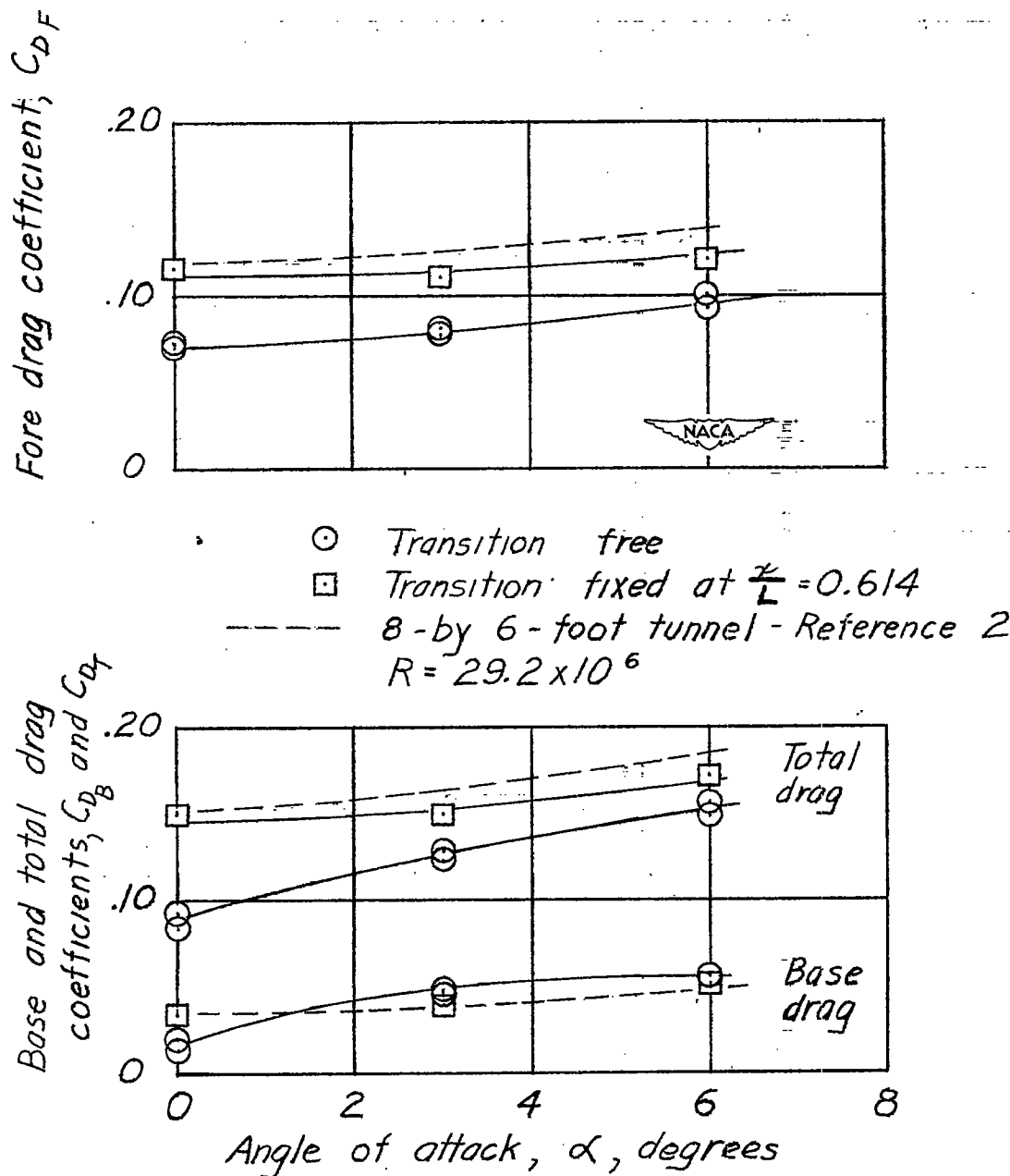
Figure 18.- Variation with angle of attack of the drag characteristics of the body alone. M = 1.59 ; R = 3.7 \times 10^6 .
