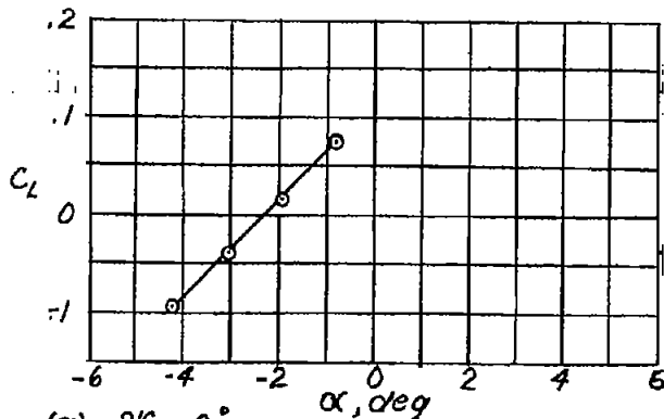
(a) \psi = 0^\circ Figure 20. - Variation of C_m , C_L and C_D with angle of attack for Model 2 with Ventral fin off; M = 1.65
