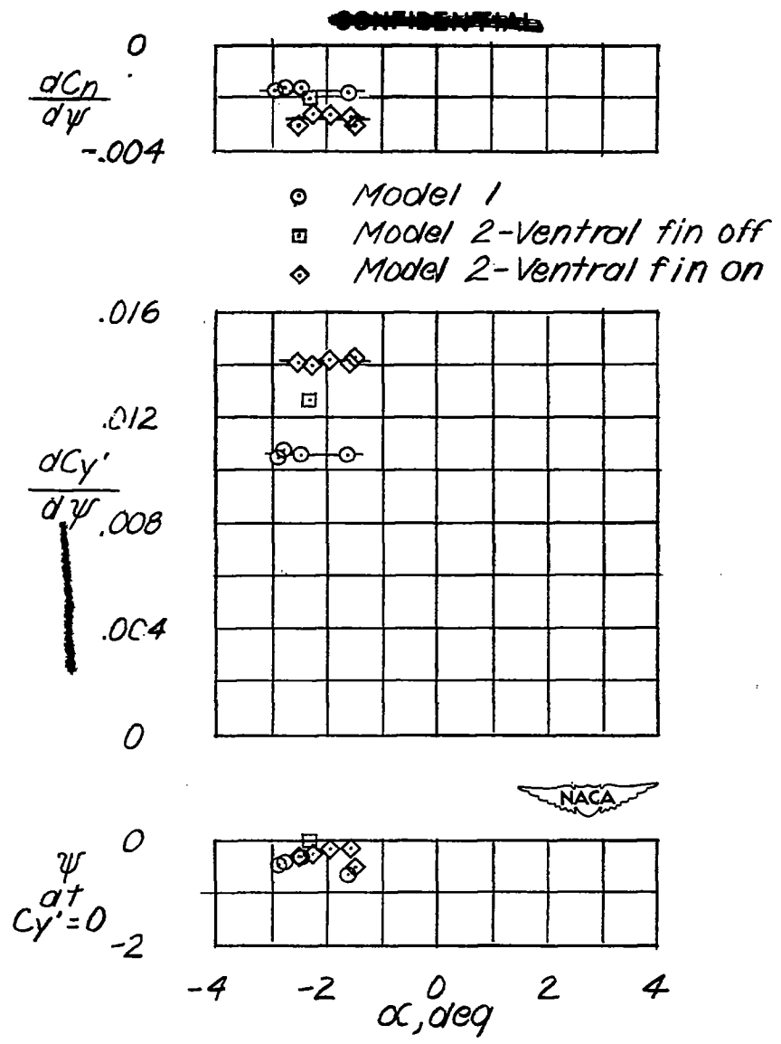
Figure 13. - Variation of dC_n/C_\psi , dC_{y'}/d\psi and \psi at C_{y'}=0 with angle of attack for Models 1 and 2; M = 1.90 .
