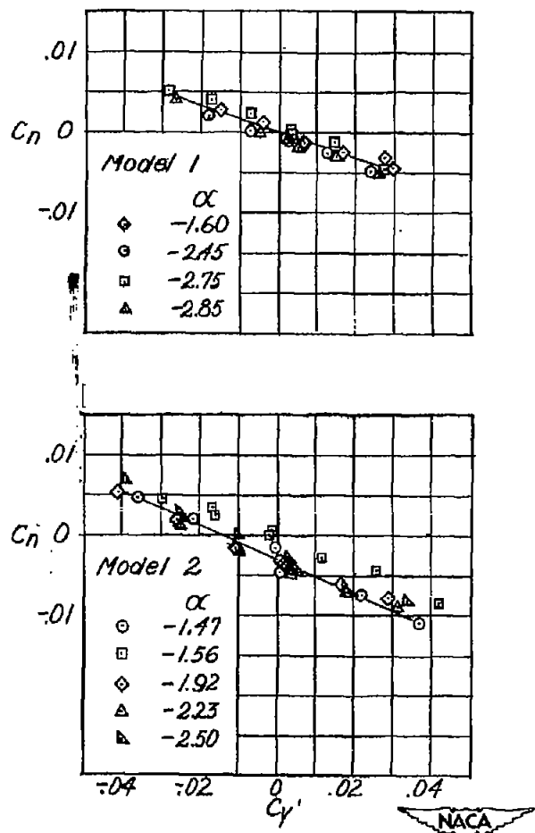
Figure 14. - Variation of C_n with C_{y'} for angles of attack for Models 1 and 2; M = 1.90 .
