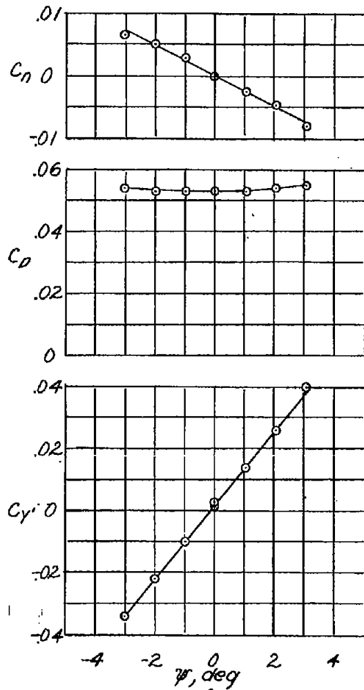
(a) \alpha = -1.78^\circ Figure 21. — Variation of C_n , C_{y'} and C_D with angle of yaw for Model 1; M = 1.55 .
