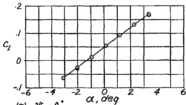
(a) \psi = 0^\circ Figure 17. - Variation of C_m , C_L and C_D with angle of attack for Model 2 with Ventral fin off; M = 2.32 .
