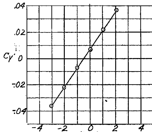
(a) \alpha = -1.47^\circ
