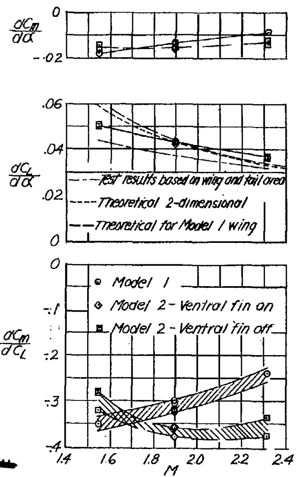
Figure 23. - Variation of dC_m/d\alpha , dC_l/d\alpha and dC_m/dC_l with M for Models 1 and 2.
