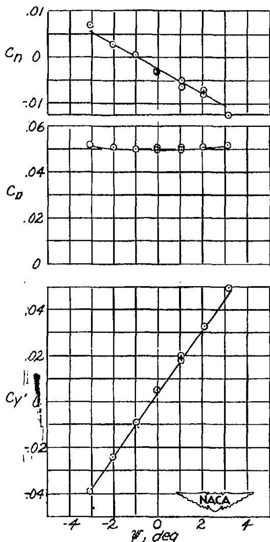
Figure 22 - Variation of C_n , C_y' and C_D with angle of yaw for Model 2 with ventral fin off; M=1.55 , \alpha = -2.02 .
