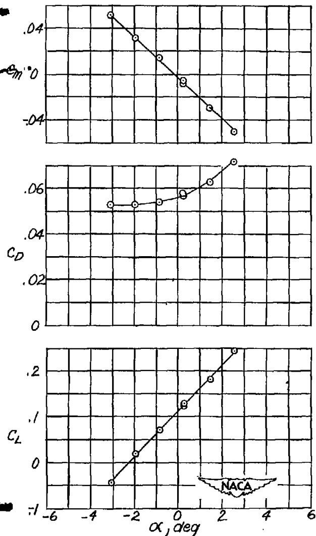
Figure 19. - Variation of C_m , C_L and C_p with angle of attack for Model 1; M = 1.55 ; \psi = 0^\circ .
