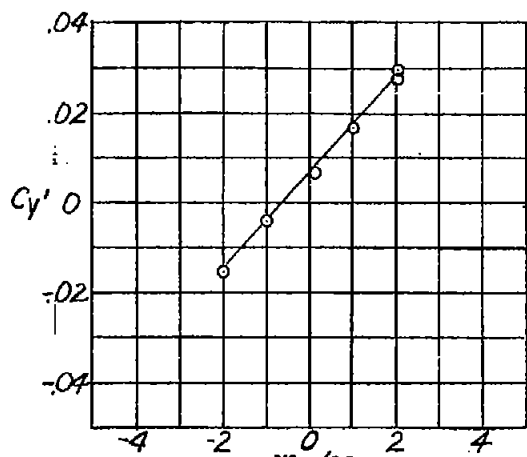
(a) \alpha = -1.60^\circ . Figure 7. - Variation of C_n , C_{y'} and C_D with angle of yaw for Model 1; M = 1.90 .
