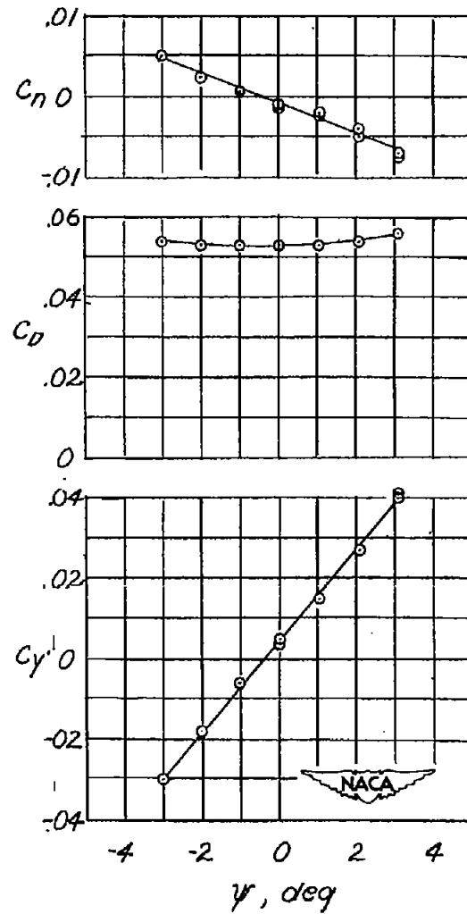
(b) \alpha = -1.78^\circ (Repeat test). Figure 21. — Continued.
