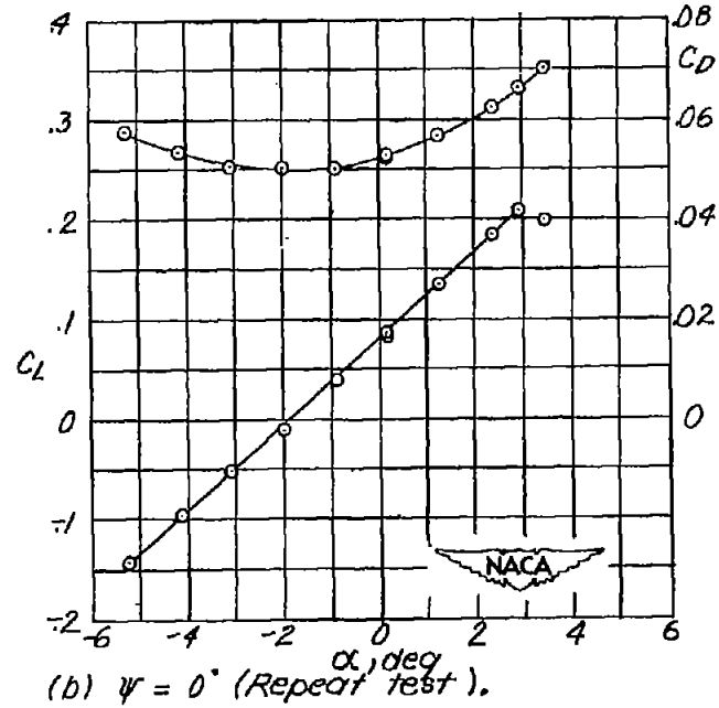
Figure 5.- Variation of C_m , C_L and C_D with angle of attack for model 1; M=1.90 .
