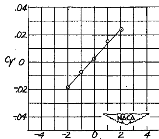
(b) \alpha = -2.45^\circ . Figure 7. - Continued.
