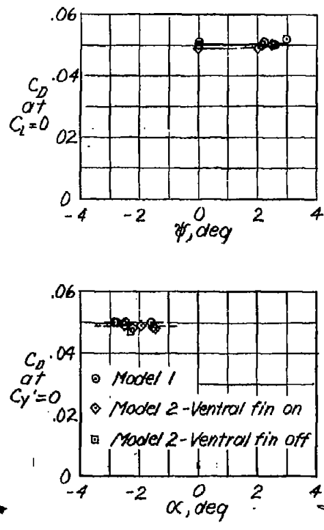
Figure 15. - Variation of C_D at C_L = 0 and C_{y'} = 0 with angles of attack and yaw for Models 1 and 2; M = 1.90 .
