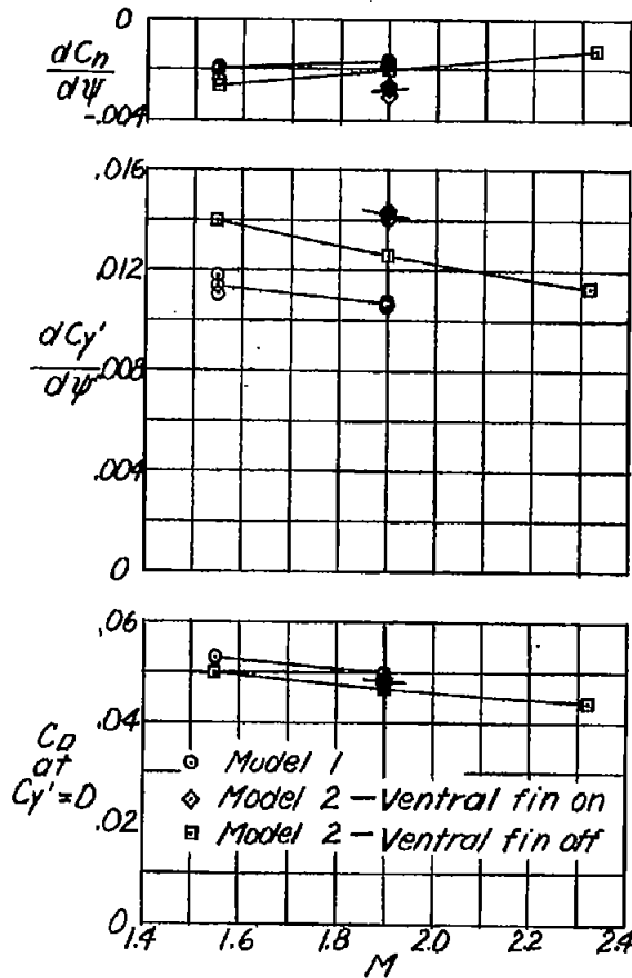
Figure 24. - Variation of \frac{dC_n}{d\psi} , \frac{dC_{y'}}{d\psi} and C_D at C_{y'}=0 with M for Models 1 and 2.
