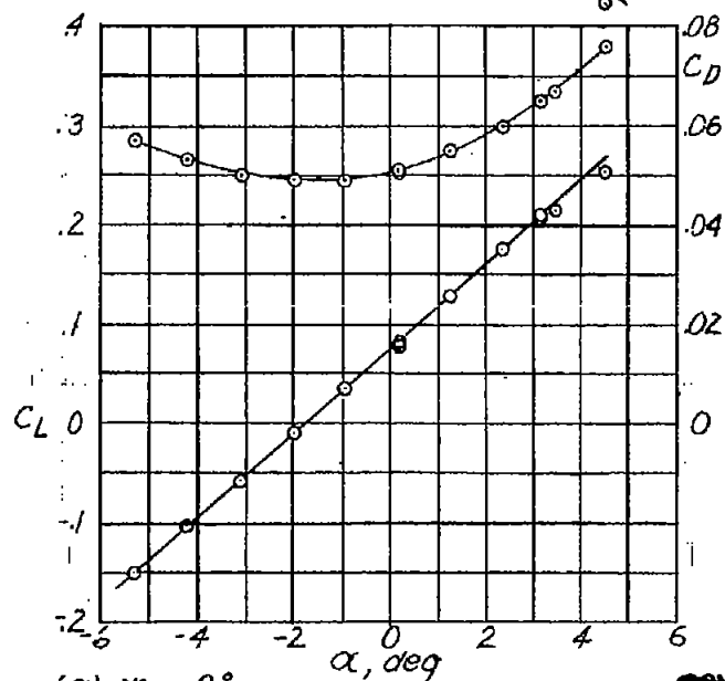
(a) \psi = 0^\circ .
