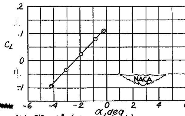
(b) \psi = 0^\circ (Repeat test). Figure 20. - Continued.
