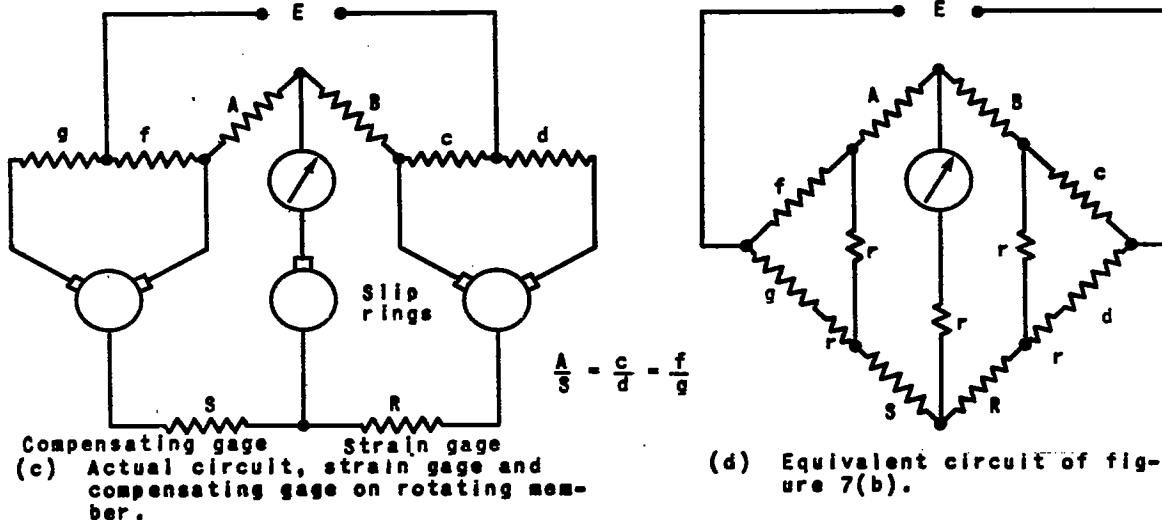
Figure 7. - Multiple-bridge circuits for elimination of contact-resistance errors in measurements through slip rings.
