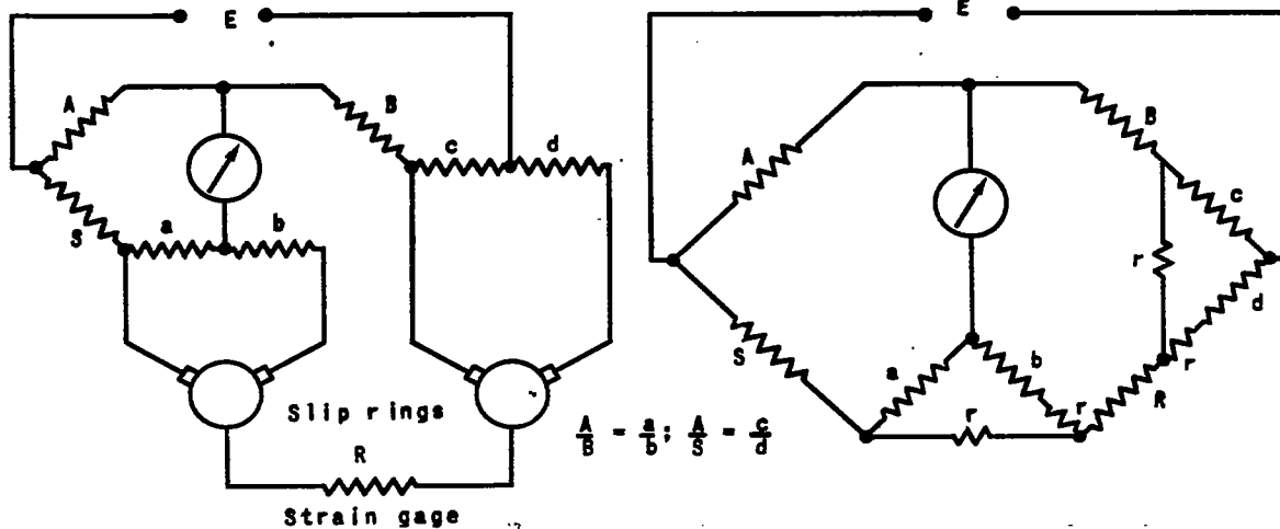
(b) Equivalent circuit of figure 7(a).
