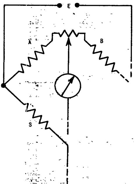
(c) Varying the ratio-arm setting.
