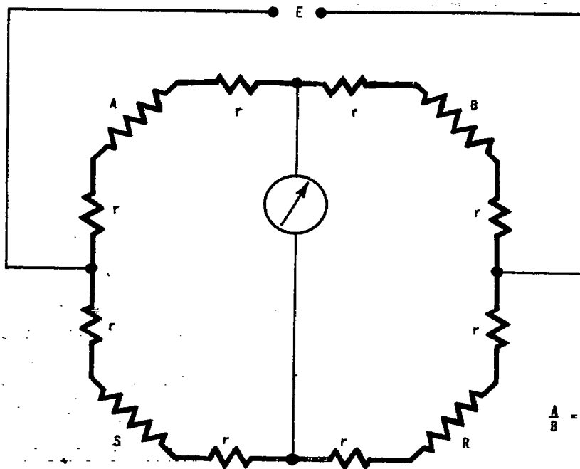
(a) Original Wheatstone bridge.
