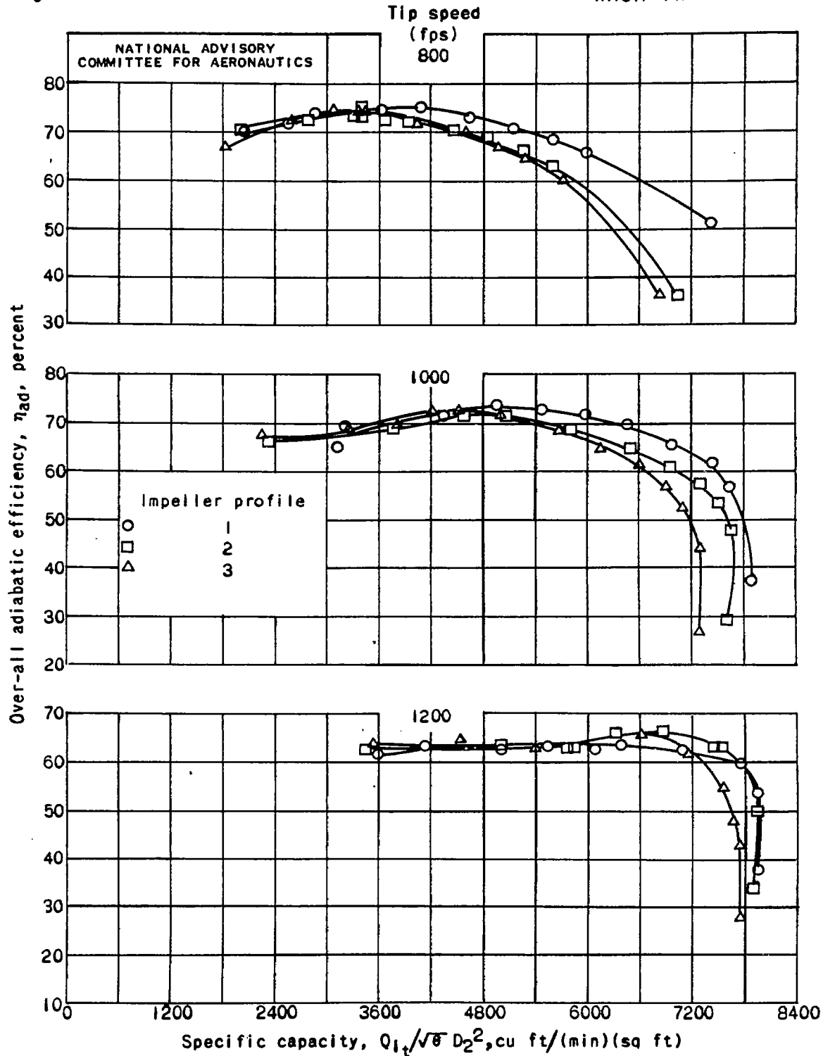
Figure 6. - Over-all adiabatic efficiencies of experimental radial-discharge impeller for three impeller passage-area variations.
