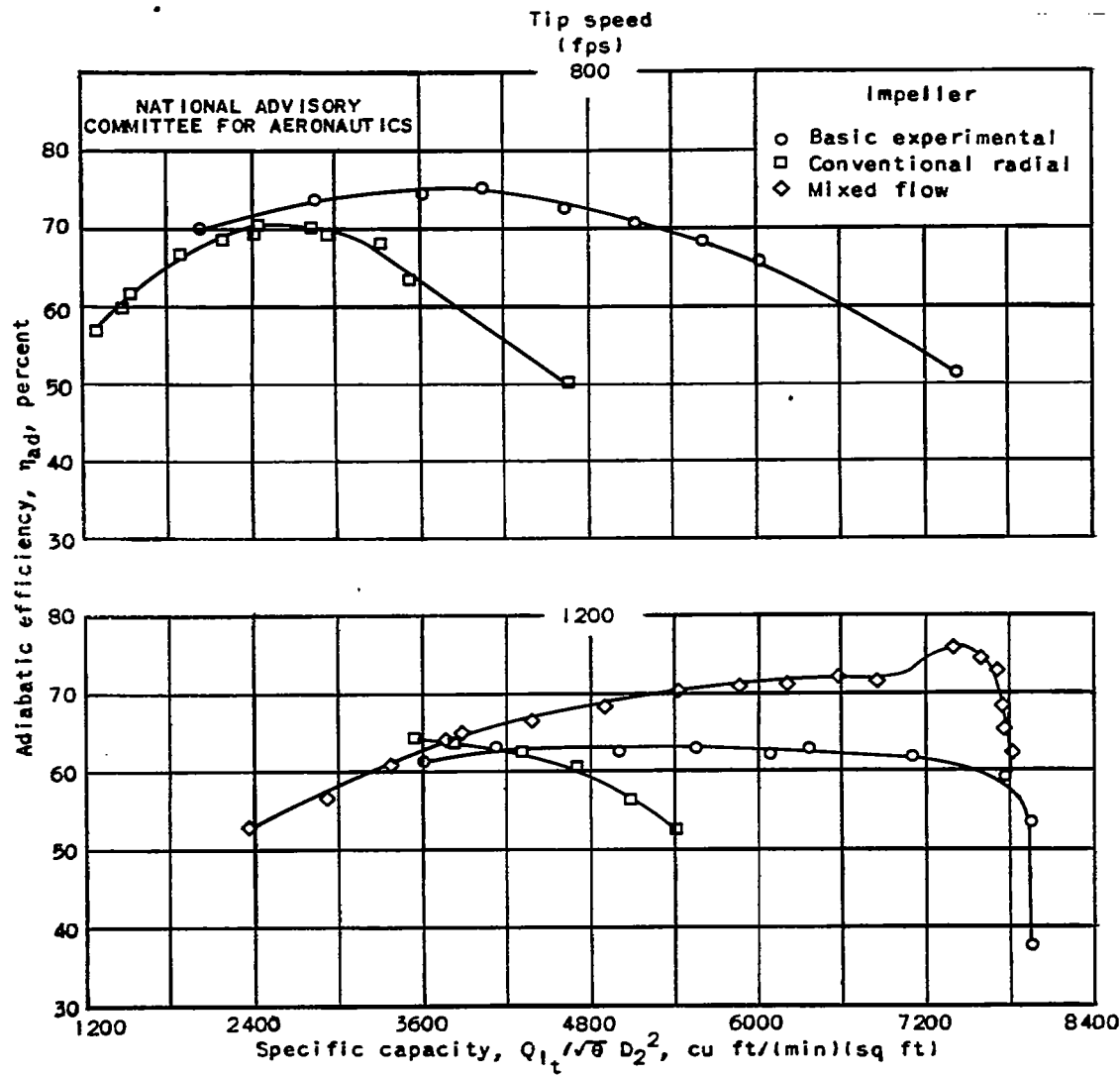
Figure 3. - Specific capacity of basic experimental radial-discharge, conventional radial, and mixed-flow impellers.
