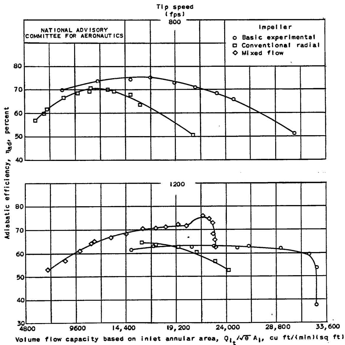
Figure 5. - Volume flow capacity based on inlet-annular area of basic experimental radial-discharge, conventional radial, and mixed-flow impellers.
