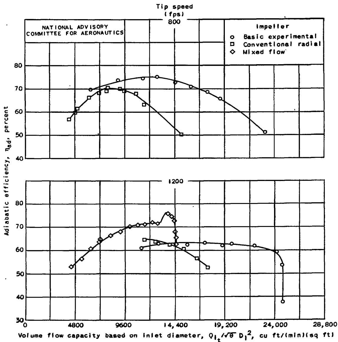
Figure 4. - Volume flow capacity based on inlet diameter of basic experimental radial-discharge, conventional radial, and mixed-flow impellers.
