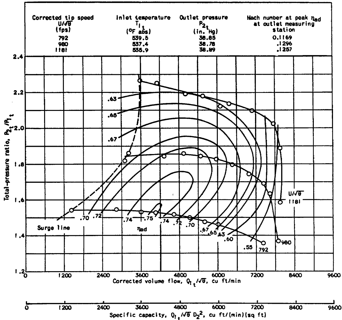
Figure 8. - Over-all performance characteristics of basic experimental radial-discharge impeller.
