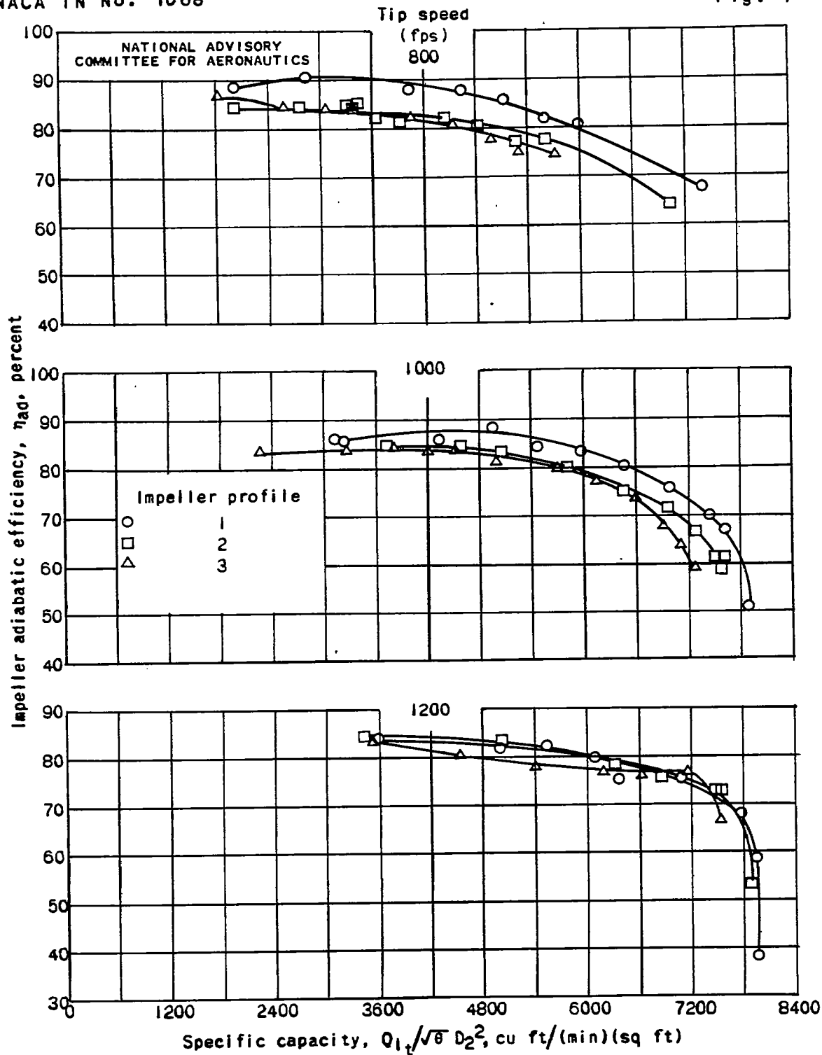
Figure 7. - Impeller adiabatic efficiencies of experimental radial-discharge impeller for three impeller passage-area variations.
