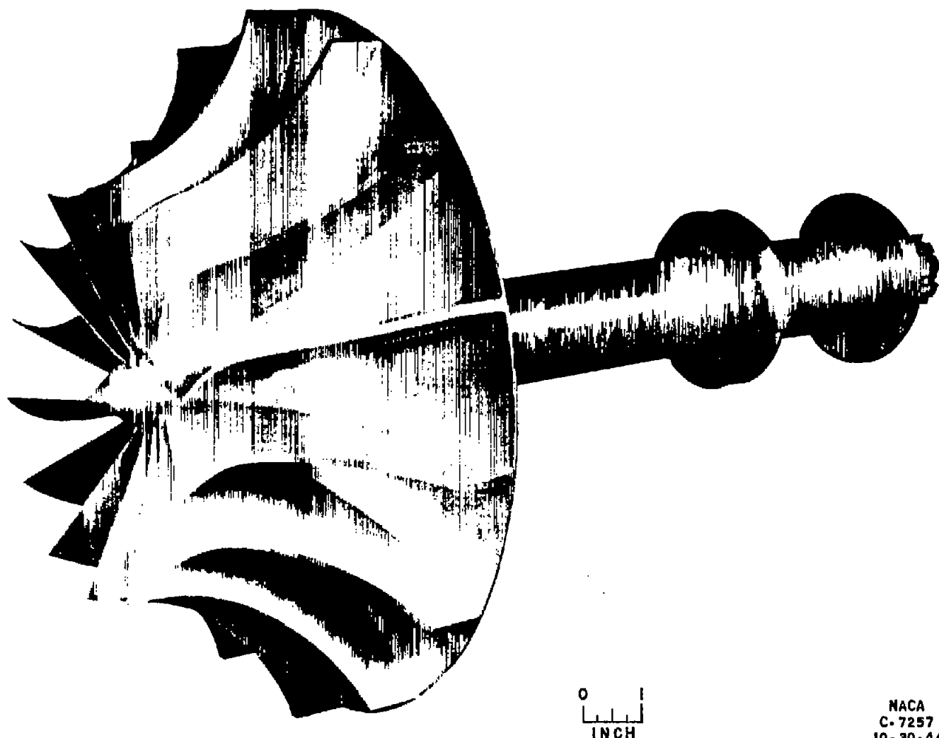
Figure 1. - Basic experimental radial-discharge impeller having a large axial-plane curvature and constant passage area along a mean flow path taken in an axial plane.
