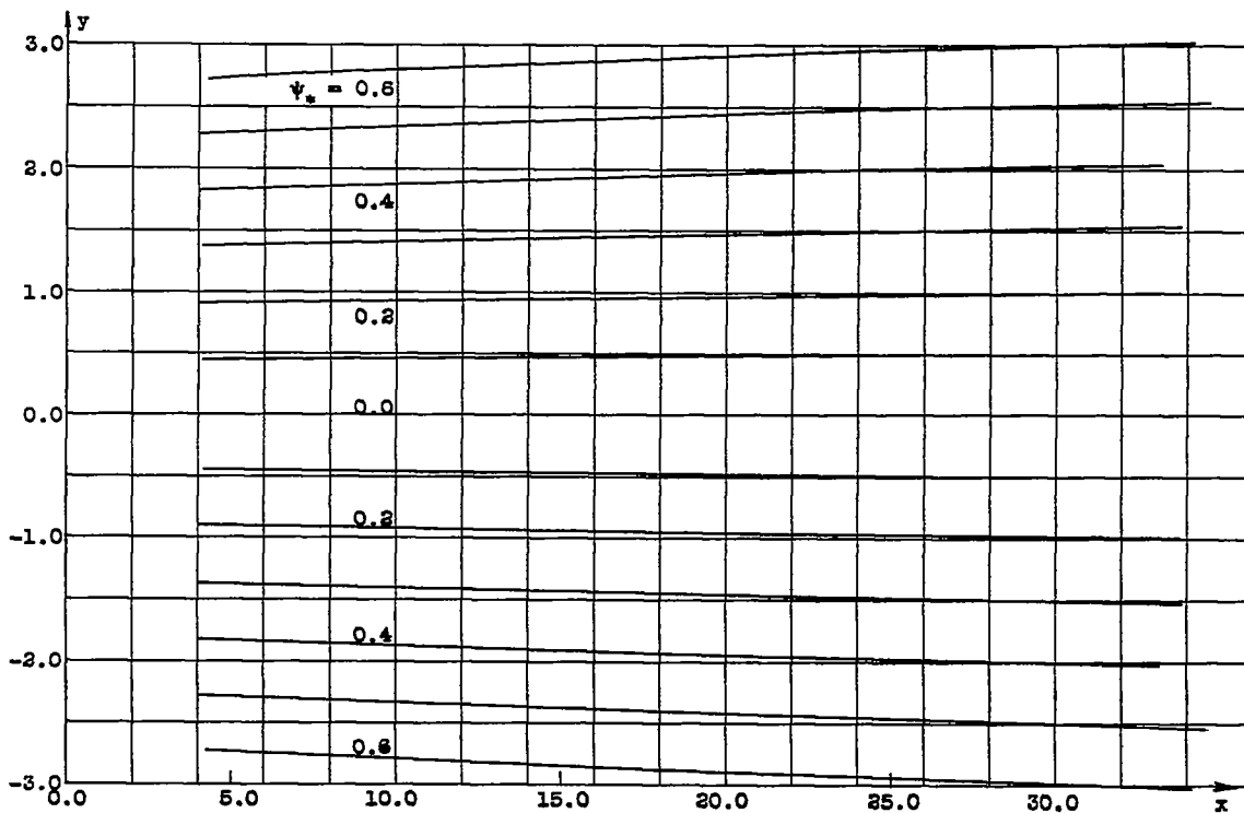
Diagram II.- Streamlines of the supersonic flow (53) in the physical plane.
