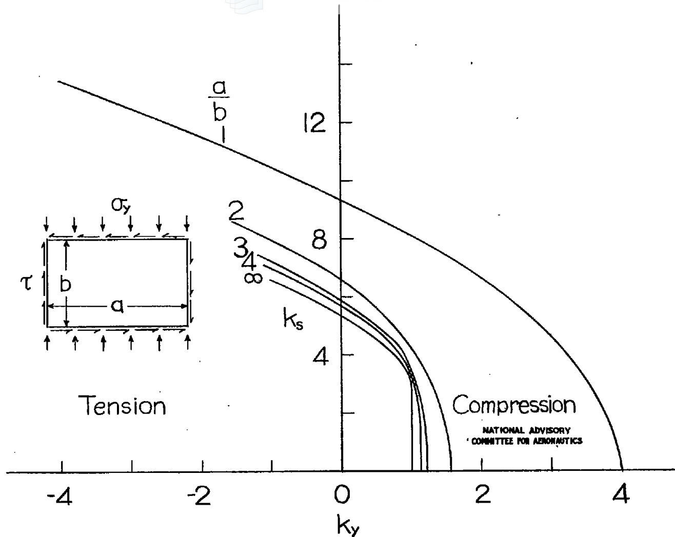
Figure 6.- Transition in the form of interaction curve for shear and transverse direct stress for a simply supported rectangular flat plate as the length-width ratio changes from 1 to \infty in terms of stress coefficients k_s and k_y . k_s = \frac{\tau t b^2}{\pi^2 D} ; k_y = \frac{\sigma_y t b^2}{\pi^2 D} .
