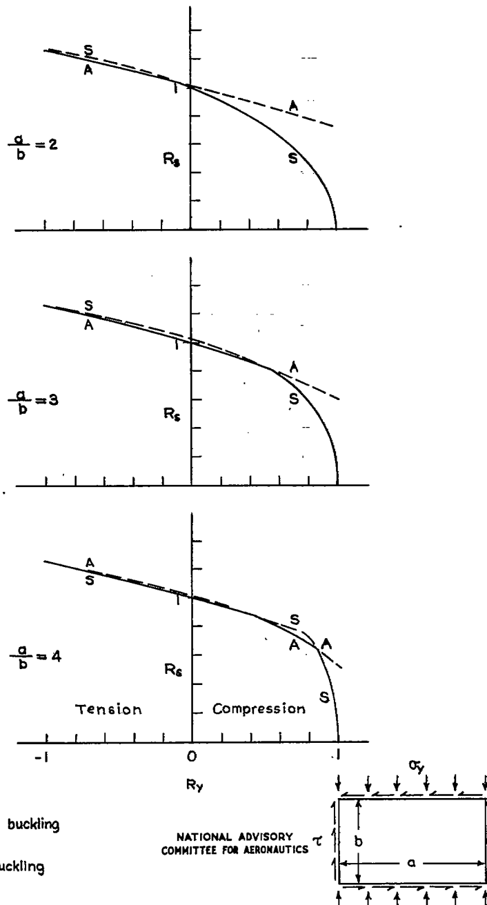
Figure 4.- Interaction curves in terms of stress ratios R_s and R_y
