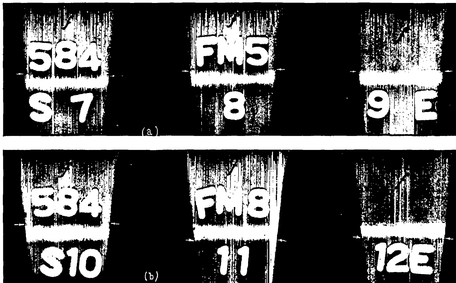
All fatigue failures at toe of face bead; no internal defects.
