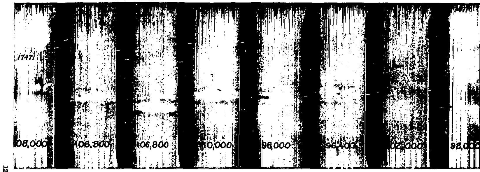
Figure 13.—Radiograph of metal-arc-welded static tension specimens in \frac{1}{8} -inch SAE 4130 sheet.
