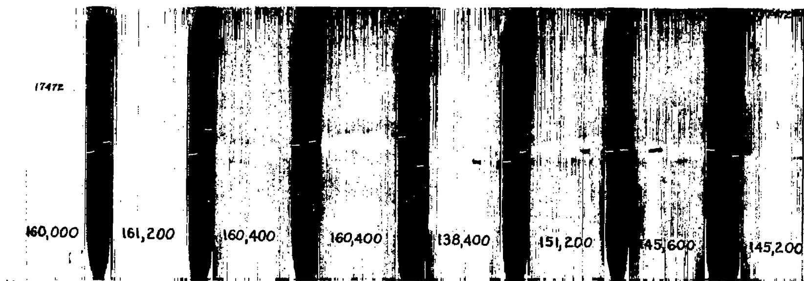
Figure 17.—Radiograph of metal-arc-welded static tension specimens in \frac{1}{8} -inch SAE 4130 sheet.
