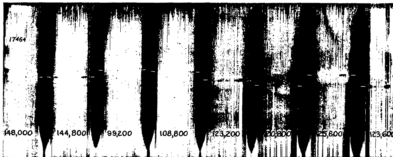
Figure 7.—Radiograph of metal-arc-welded static tension specimens in \frac{1}{8} -inch SAE 4130 sheet.
