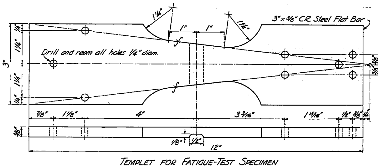
FIGURE 19—SPECIMEN AND TEMPLET FOR PLATE BENDING-FATIGUE TEST
