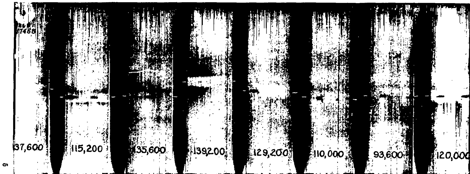
Figure 6.—Radiograph of metal-arc-welded static tension specimens in \frac{1}{8} -inch SAE 4130 sheet.
