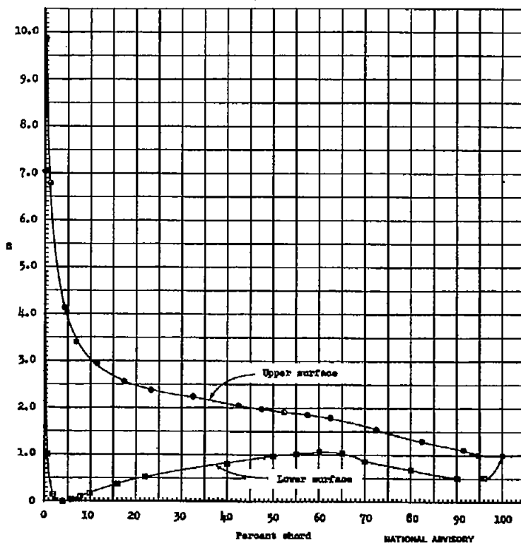
(t) \alpha_0 = 12.2^\circ . Figure 4.- Continued.
