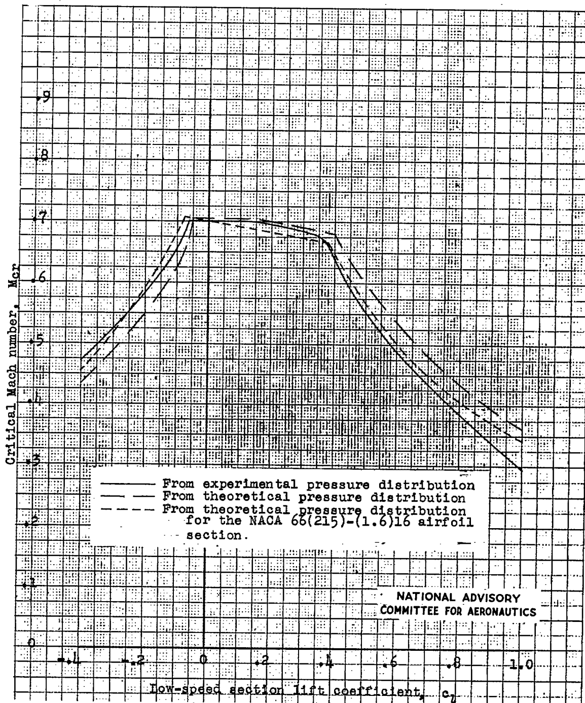
(d) NACA 66(215)-216 \left\{ \begin{matrix} a = -0.6, & c_{l1} = -0.5 \\ a = 1.0, & c_{l1} = 0.7 \end{matrix} \right\} airfoil section.
