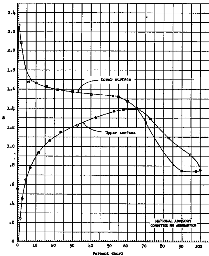
Figure 7.- Experimental pressure distribution of the NACA 66(215)-216 \left\{ \begin{array}{l} \kappa = 0.6, \quad \sigma_{t1} = -0.5 \\ \alpha = 1.0, \quad \sigma_{t2} = 0.5 \end{array} \right. airfoil section. R = 6 \times 10^6 ; 2D tests 539 and 572.
