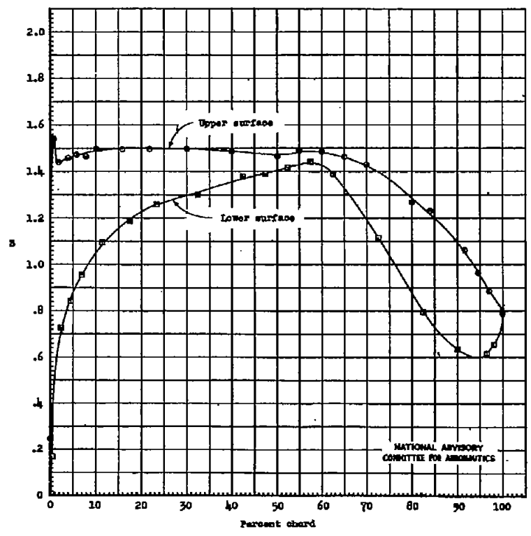
(2) \alpha_0 = 0.8^\circ Figure 3.- Continued.
