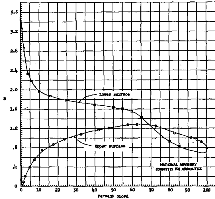
(a) \alpha_0 = -6.1^\circ
