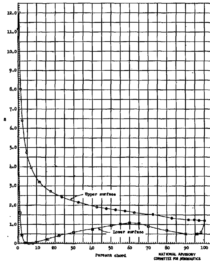
(t) \alpha_0 = 16.2^\circ . Figure 5.- Continued.
