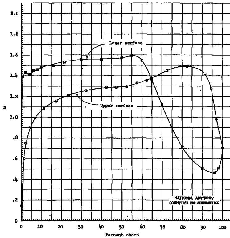
(h) \alpha_0 = -3.1^\circ Figure 5.- Continued.
