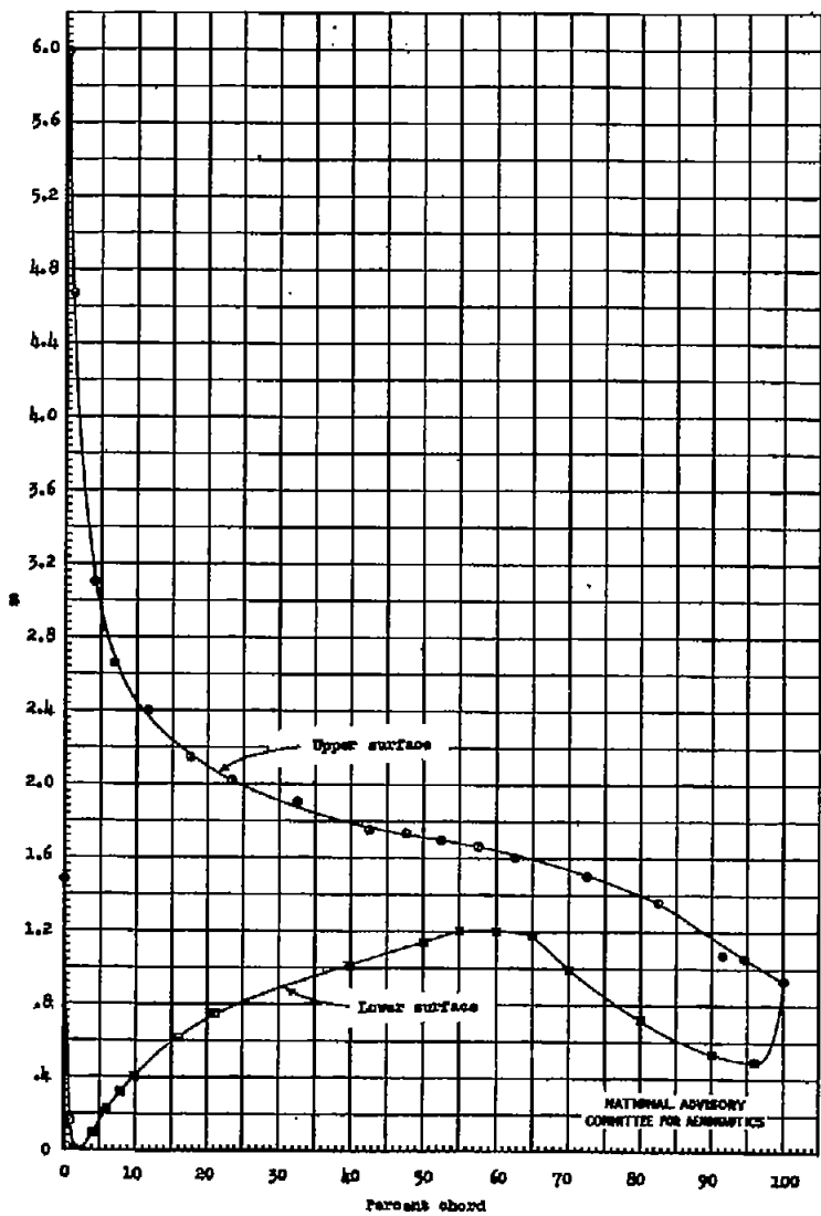
(a) \alpha_0 = 8.1^\circ . Figure 4.- Continued.
