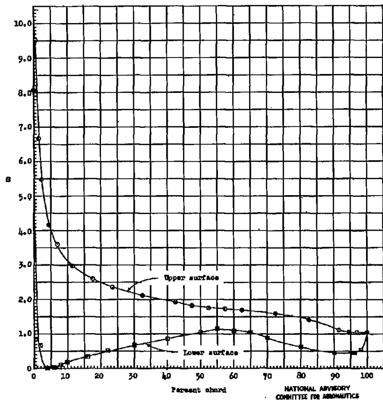
(s) \alpha_0 = 12.2^\circ . Figure 5.- Continued.
