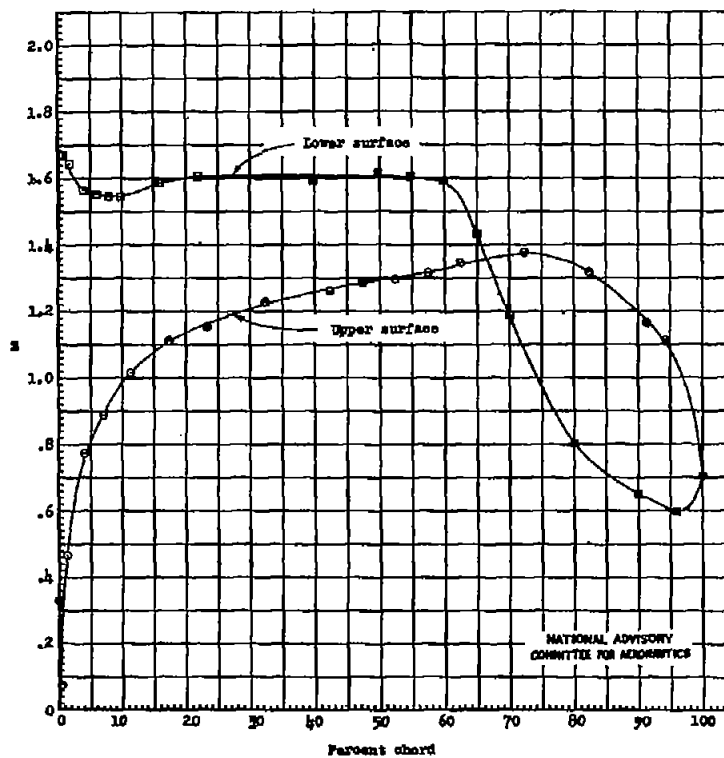
(h) \alpha_0 = -3.4^\circ . Figure 4.- Continued.
