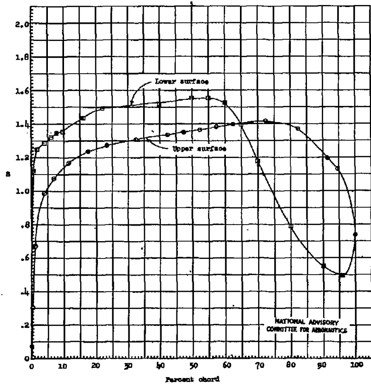
(k) \alpha_0 = -2.0^\circ . Figure 4.- Continued.
