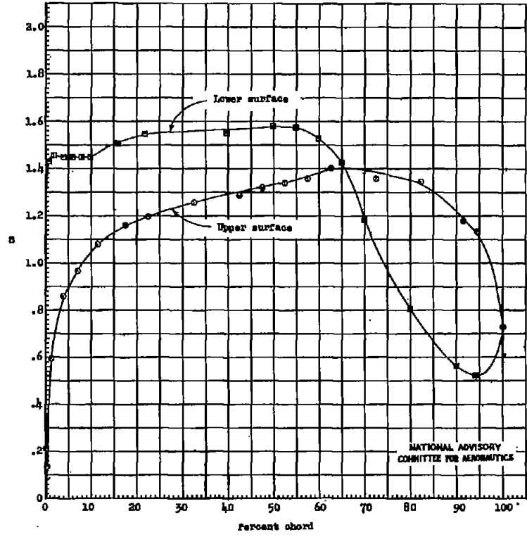
(j) \alpha_0 = -2.8^\circ .
