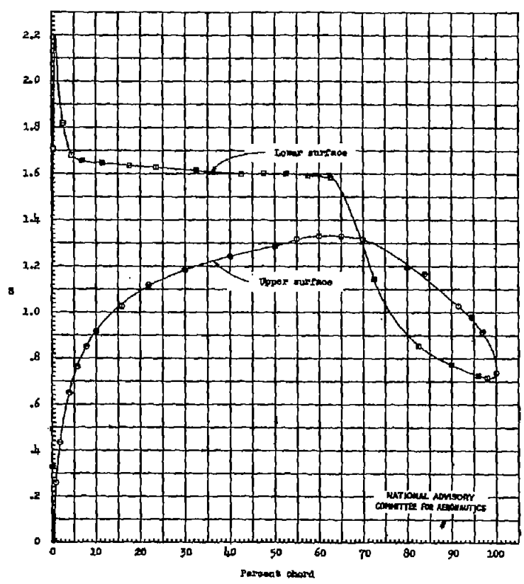
(a) \alpha_0 = -4.1^\circ
