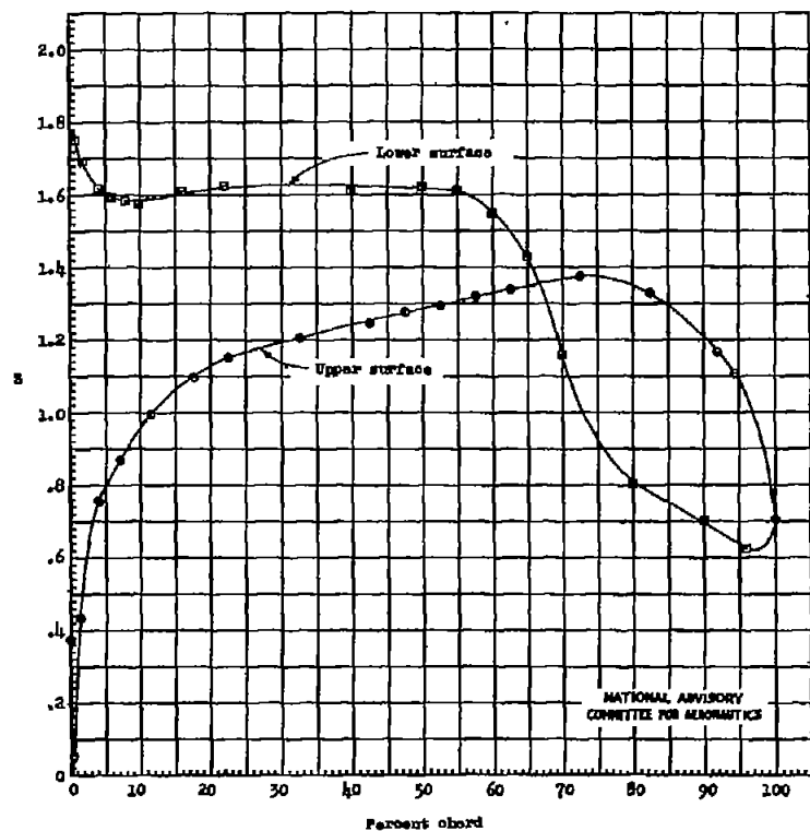
(g) \alpha_0 = -3.6^\circ . Figure 4.- Continued.
