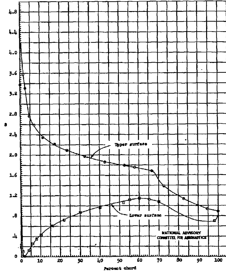
(h) \alpha_0 = 8.1^\circ Figure 7.- Continued.
