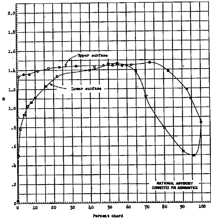
(a) \alpha_0 = 0^\circ . Figure 4.- Continued.
