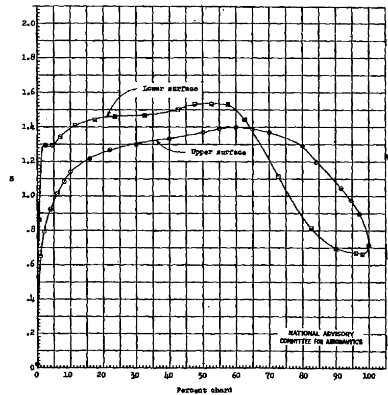
(b) \alpha_0 = -2.0^\circ
