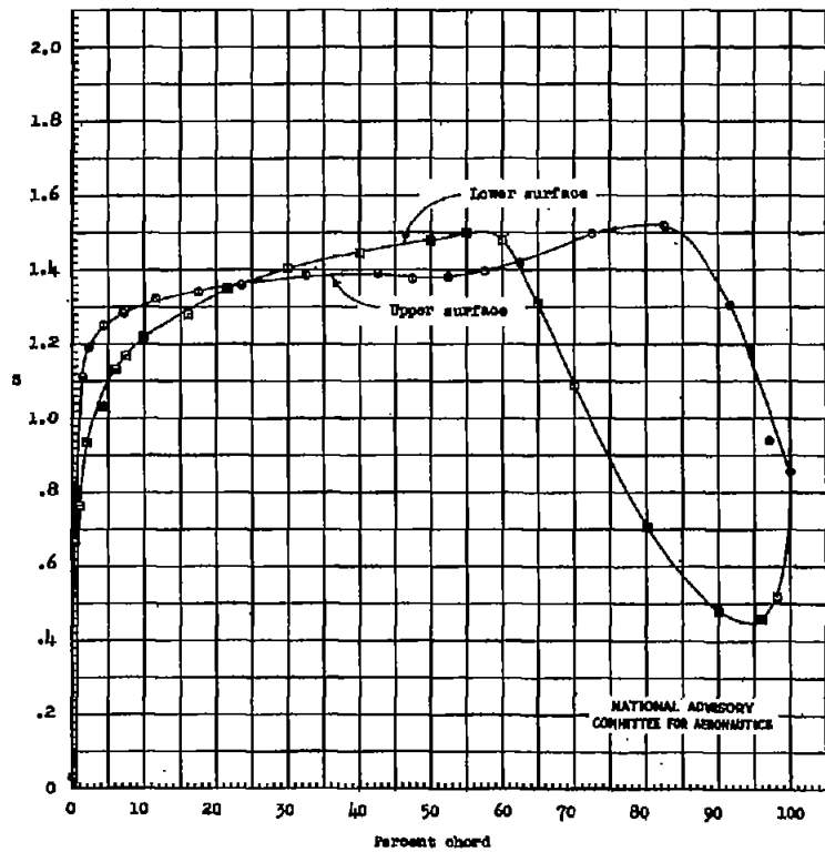
(k) \alpha_0 = -1.0^\circ .
