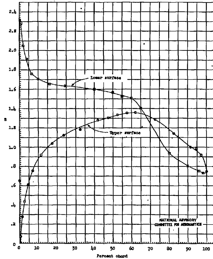
(b) \alpha_0 = -4.1^\circ
