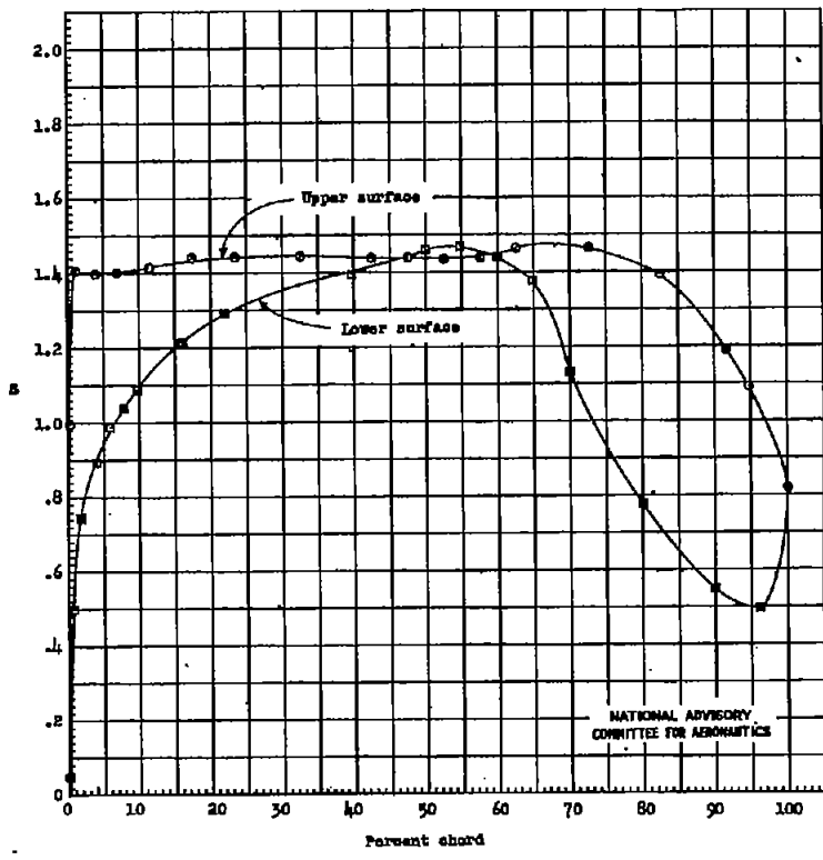
(a) \alpha_0 = 0.3^\circ . Figure 4.- Continued.
