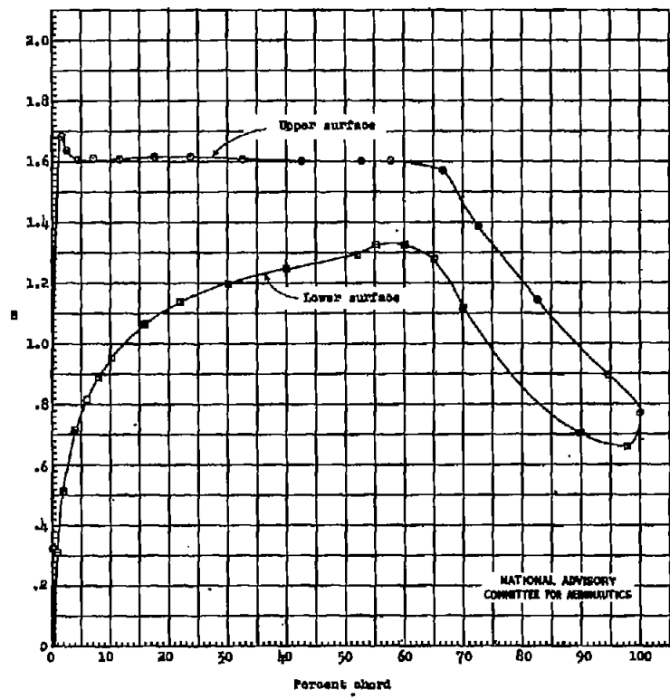
(f) \alpha_0 = 2.0^\circ Figure 7.- Continued.
