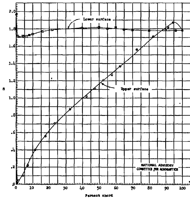
(a) \alpha_0 = -20.3^\circ .
