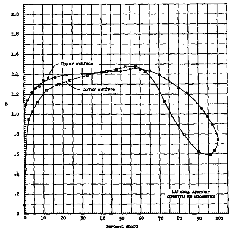
(f) \alpha_0 = -0.5^\circ Figure 3.- Continued.
