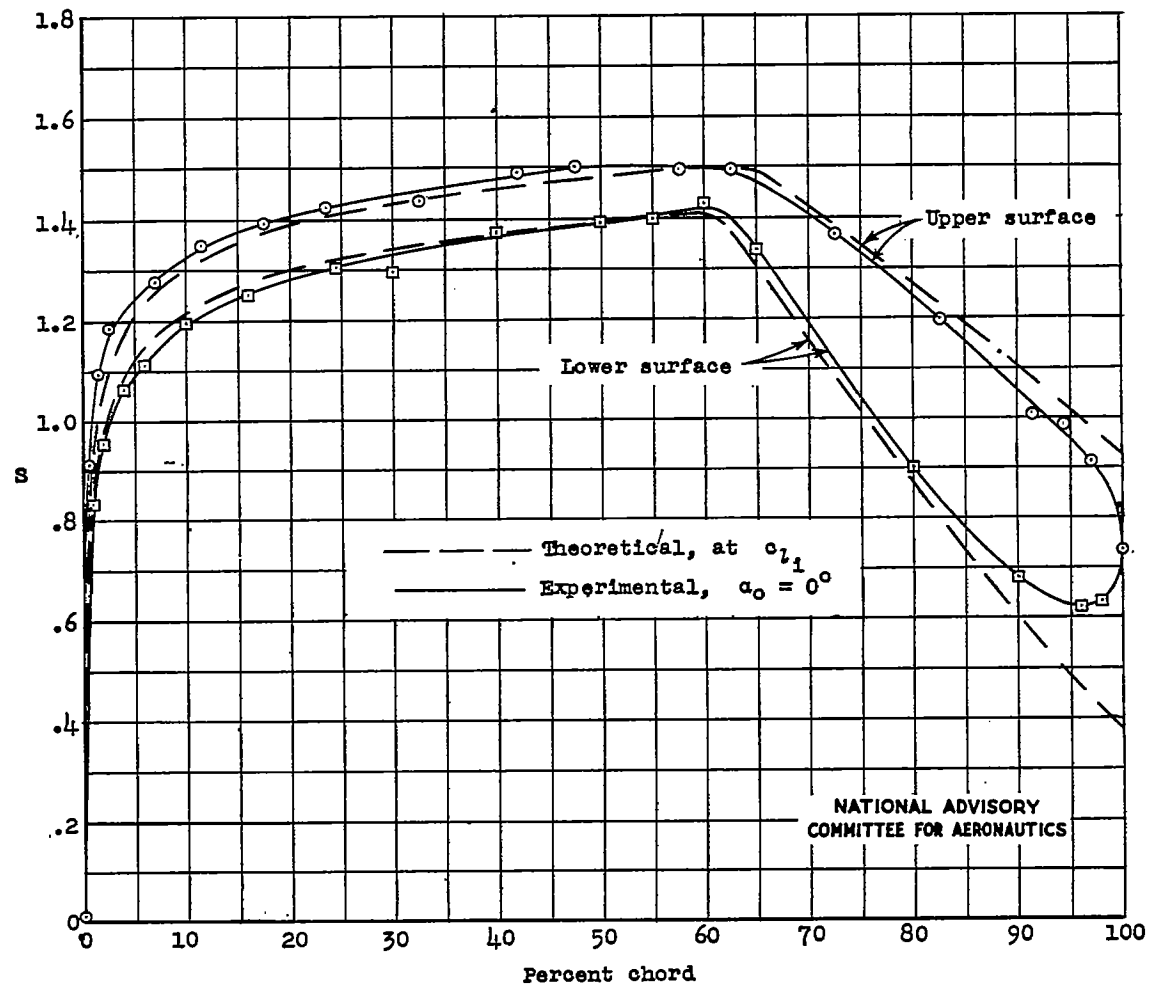
(d) NACA 66(215)-216 \left\{ \begin{array}{l} a = 0.6, \alpha_{i1} = -0.5 \\ a = 1.0, \alpha_{i1} = 0.7 \end{array} \right\} airfoil section.
