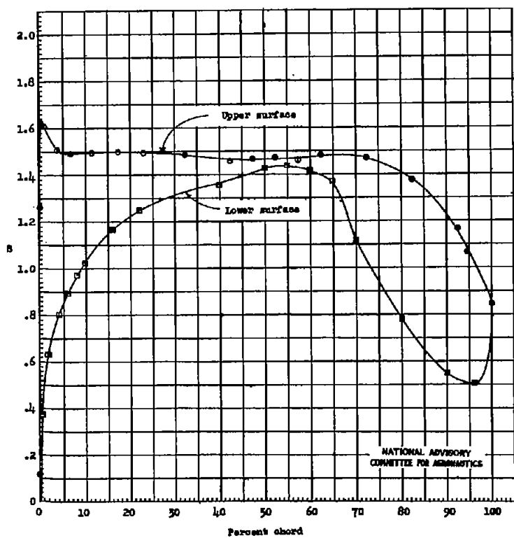
(a) \alpha_0 = 1.0^\circ . Figure 4.- Continued.
