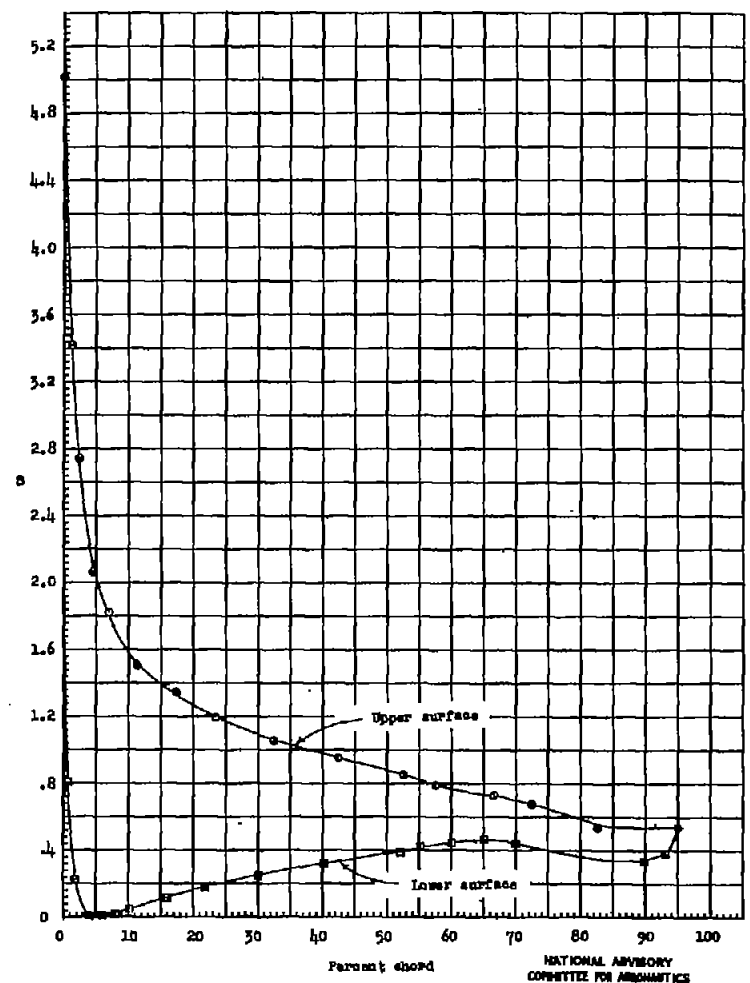
(1) \alpha_0 = 16.2^\circ . Figure 7.- Concluded.
