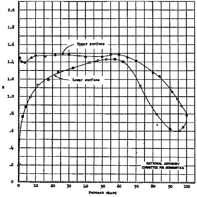
(1) \alpha_0 = 0.5^\circ Figure 3.- Continued.
