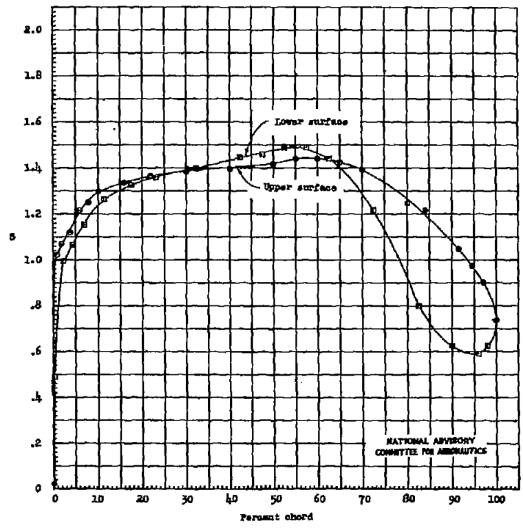
(e) \alpha_0 = -0.8^\circ Figure 3.- Continued.
