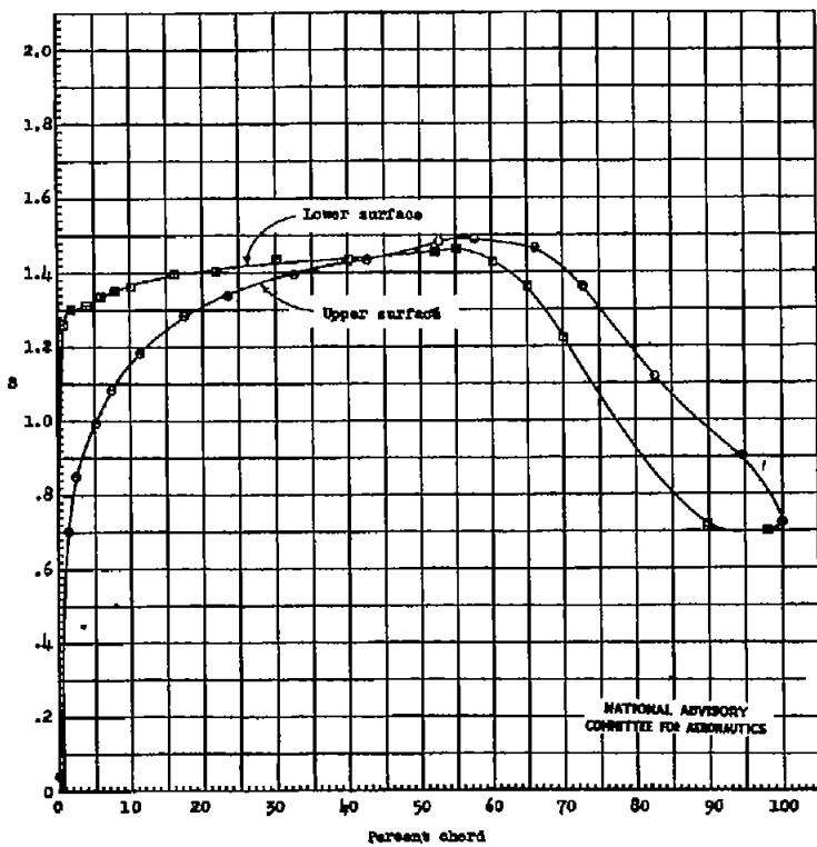
(c) \alpha_0 = -1.5^\circ Figure 7.- Continued.
