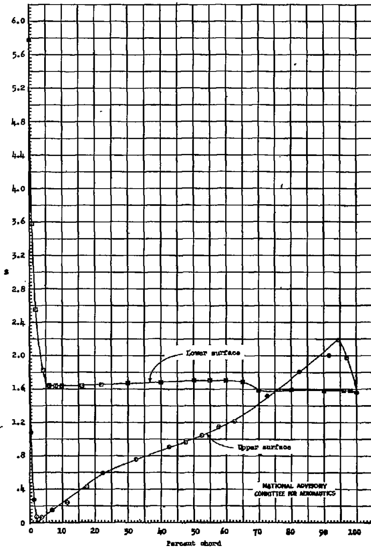
Figure 5.- Experimental pressure distribution of the NACA 66(215)-416 airfoil section, B = 6 \times 10^6 ; XOF test 632.
