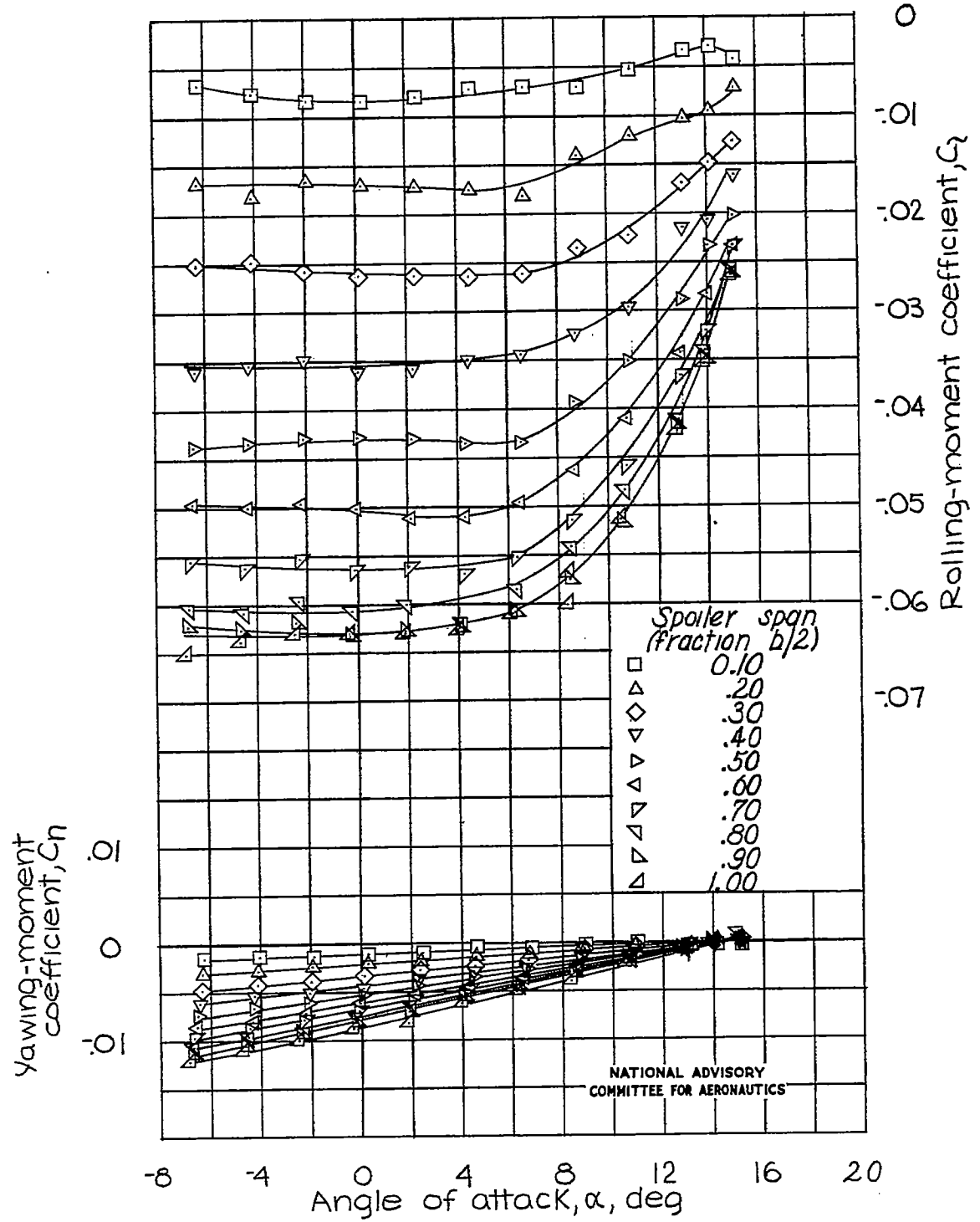
Figure 4.- Variation of aerodynamic characteristics with spoiler span. Outboard spoilers; M = 0.27 ; R = 2.69 \times 10^6 .
