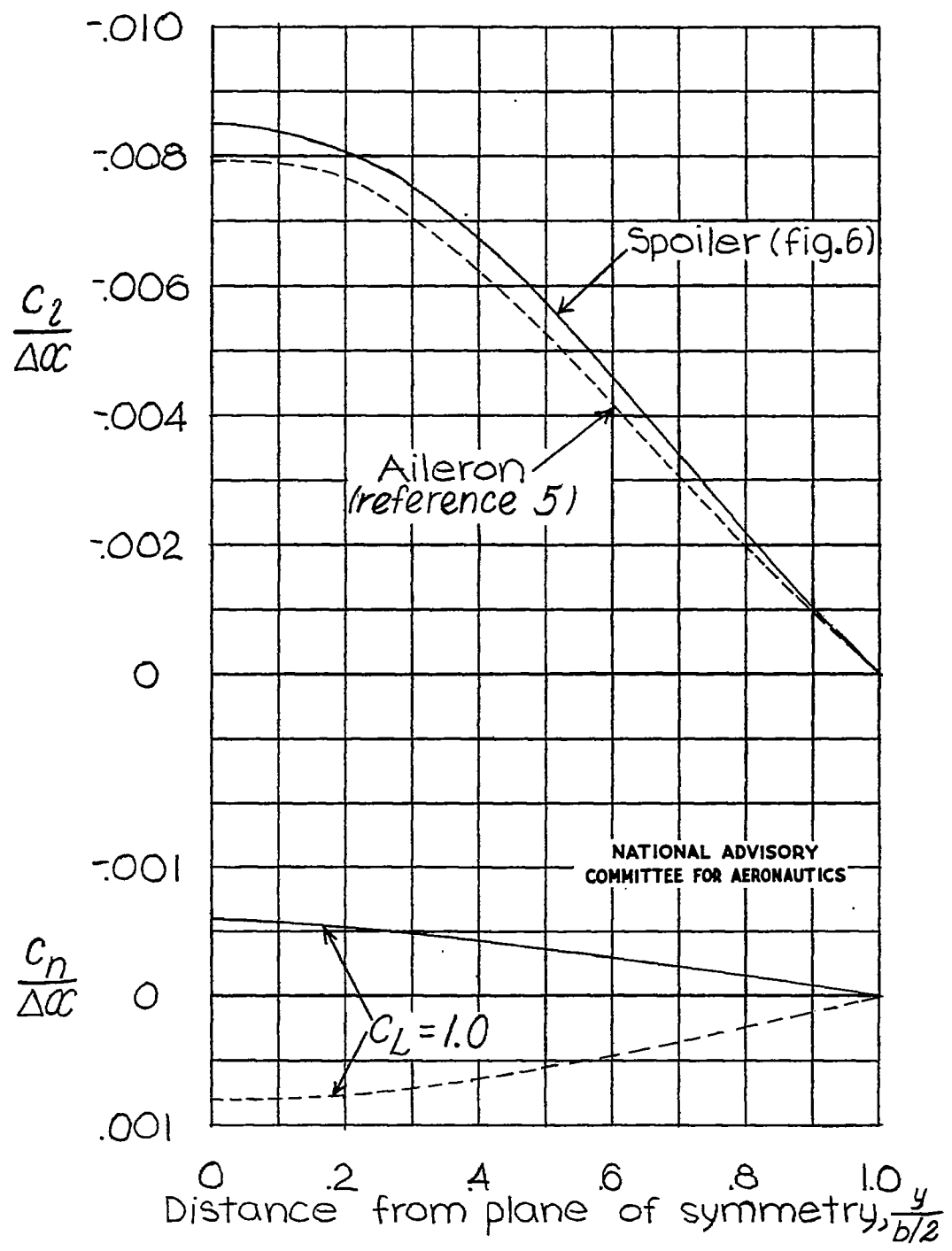
Figure 7.- Comparison of variation of rolling-moment and yawing-moment effectiveness parameters with spanwise location for ailerons (theoretical) and spoilers (experimental). Aileron values extrapolated for a wing of A = 10 , \lambda = 0.50 .
