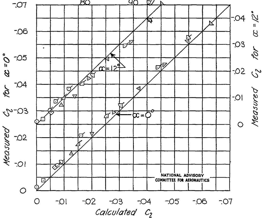
Figure 5.- Comparison of calculated rolling-moment coefficients obtained from outboard spoilers with measured rolling-moment coefficients obtained from inboard or isolated spoilers for different spoiler spanwise locations.
