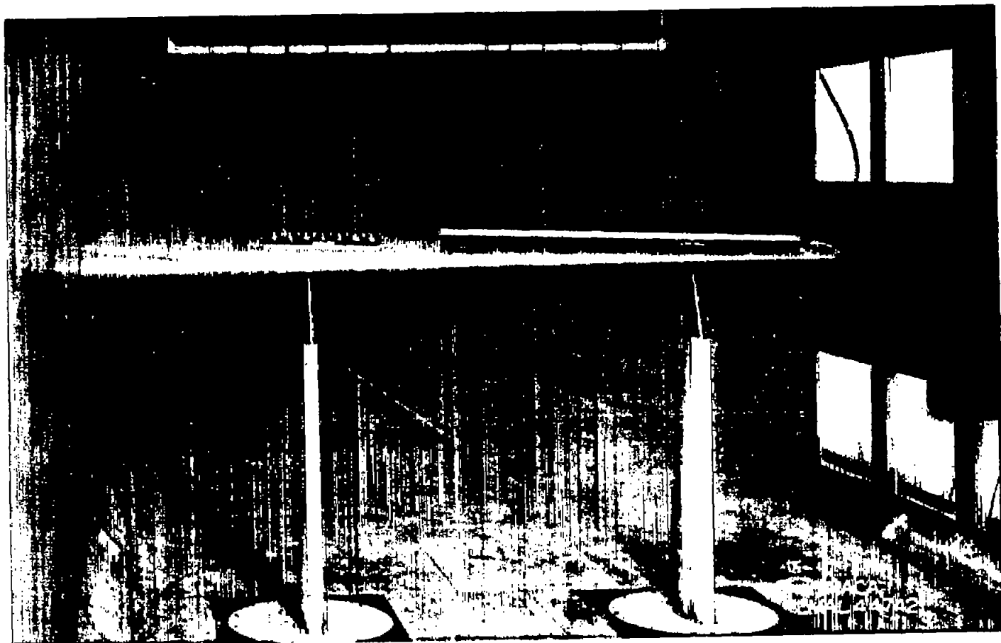
Figure 1.- General setup of spoiler mounted on semispan-wing model.
