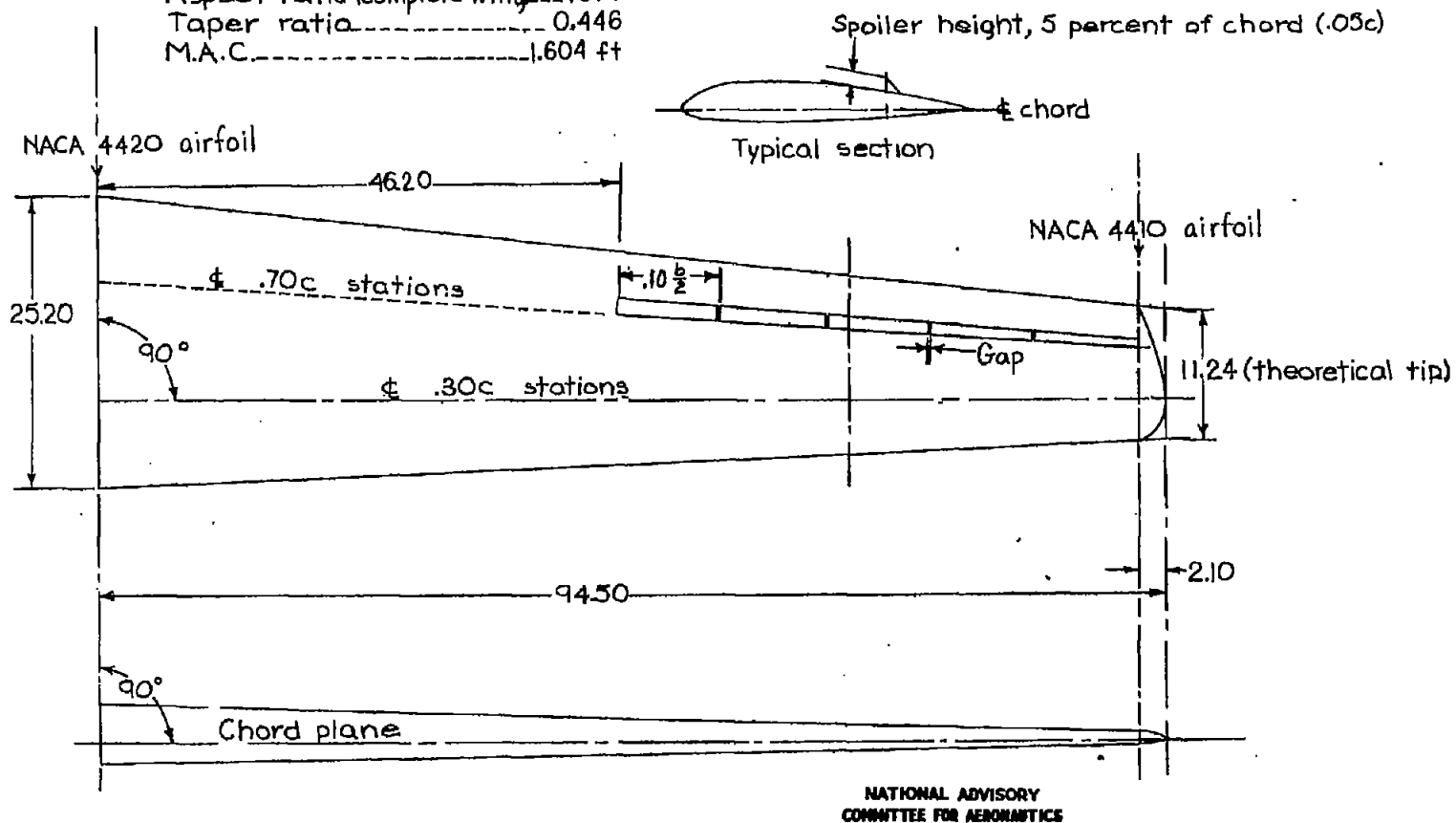
Figure 2.- Diagram of model used in spoiler investigation. Typical spoiler installation (50-percent semispan spoiler). All dimensions are in inches.
