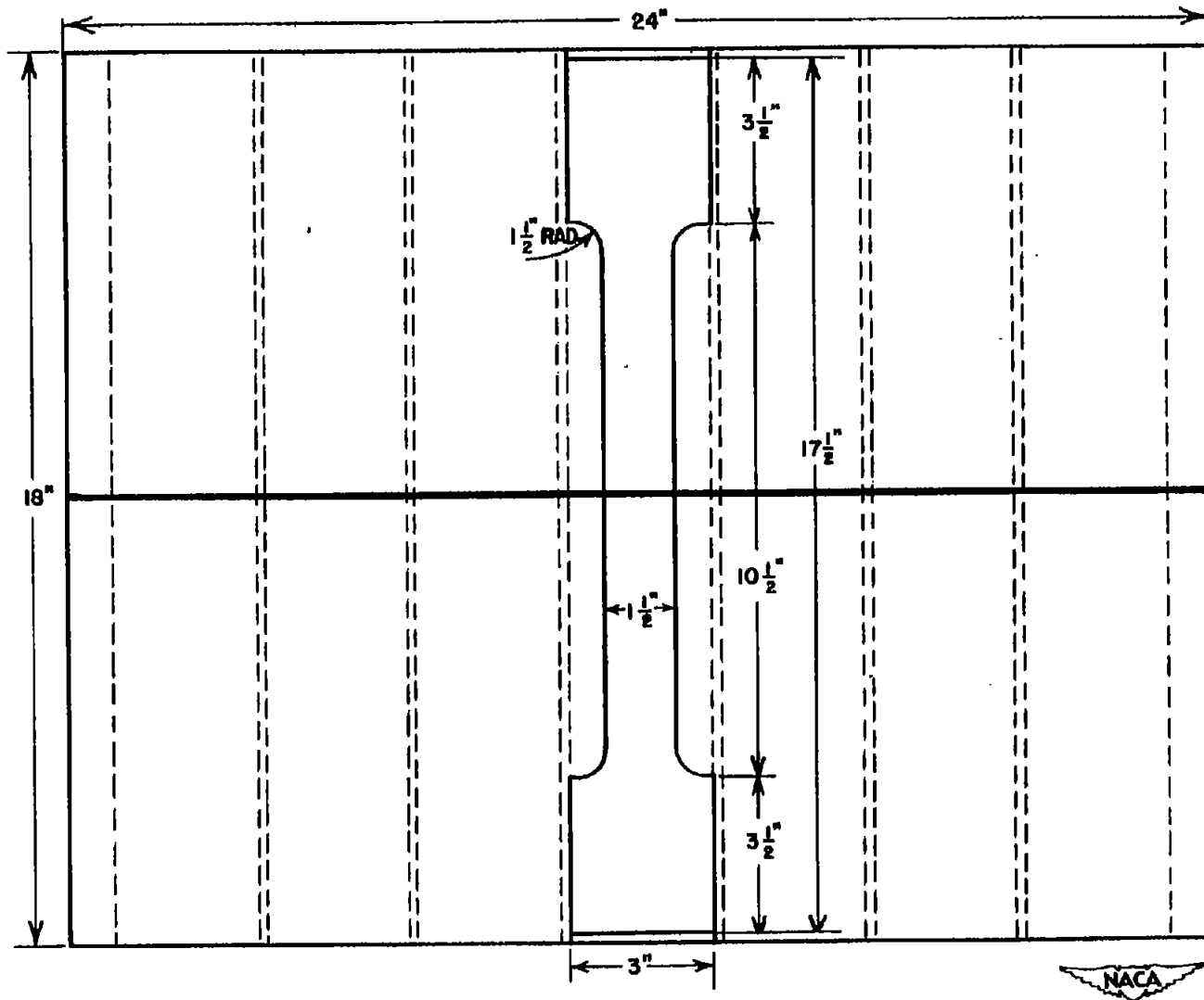
Figure 42.- Multi-arc-welded joint and fatigue test specimen.
