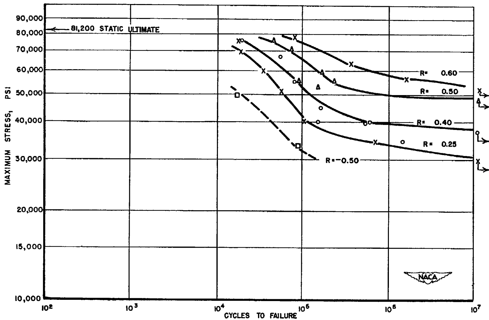
Figure 4.- Direct-stress fatigue strength of 0.040-inch 75S-T Alclad sheet. Test section 1.0 inch wide. Specimens cut in the direction of rolling. (R = min. load/max. load. Positive values indicate tension; negative values, compression.)
