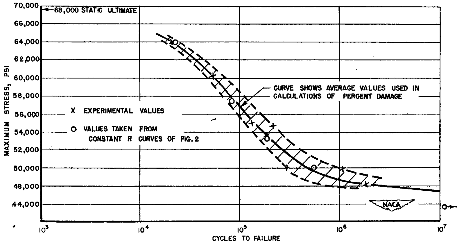
Figure 49.- Scatter band of fatigue strengths of unnotched sheet specimens of 24S-T Alclad tested at a constant mean of 40,000 psi.
