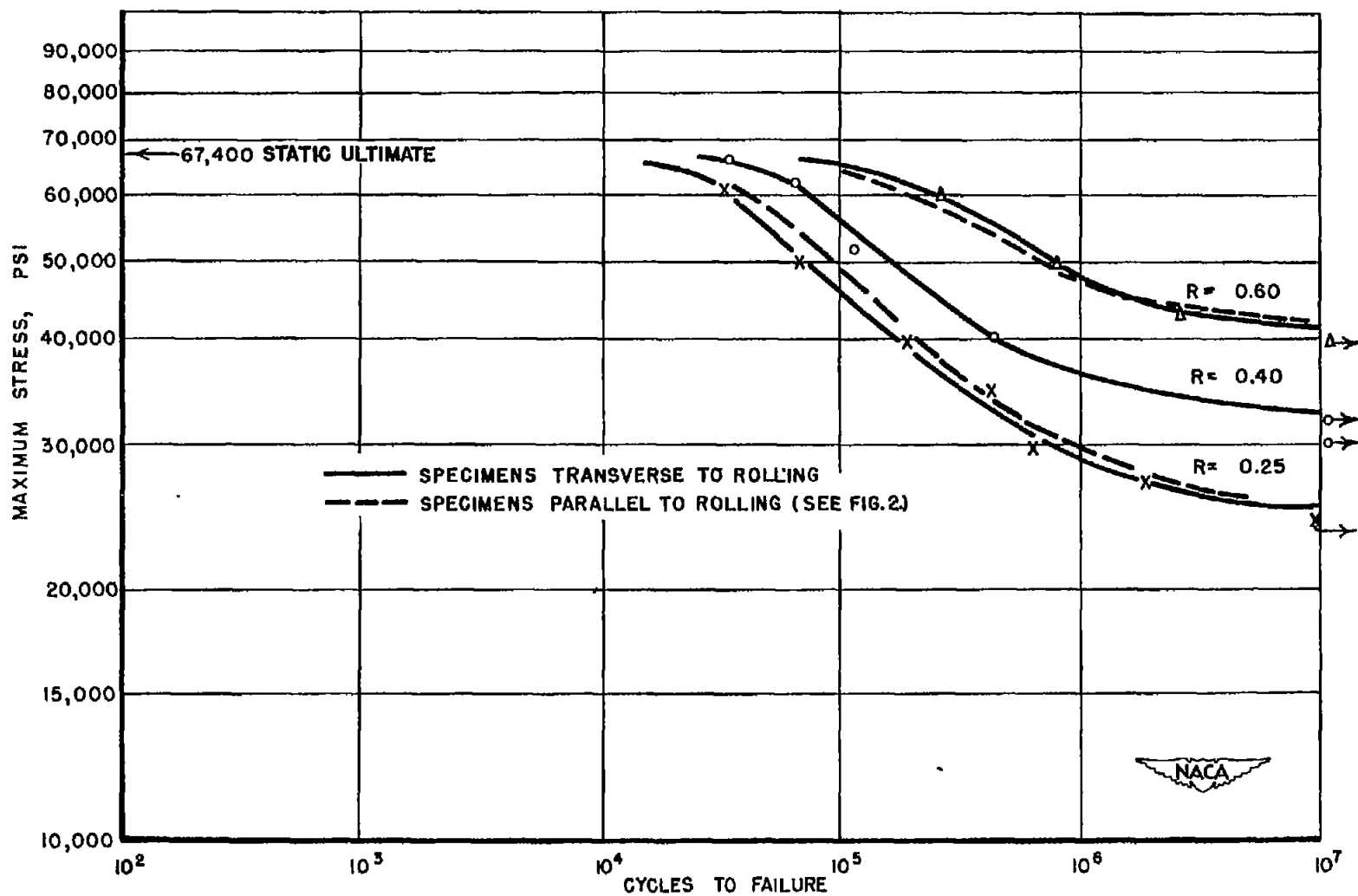
Figure 7.- Direct-stress fatigue strength of 0.040-inch 24S-T Alclad sheet. Test section 1.0 inch wide. Specimens cut transverse to direction of rolling. (R = min. load/max. load. Positive values indicate tension.)
