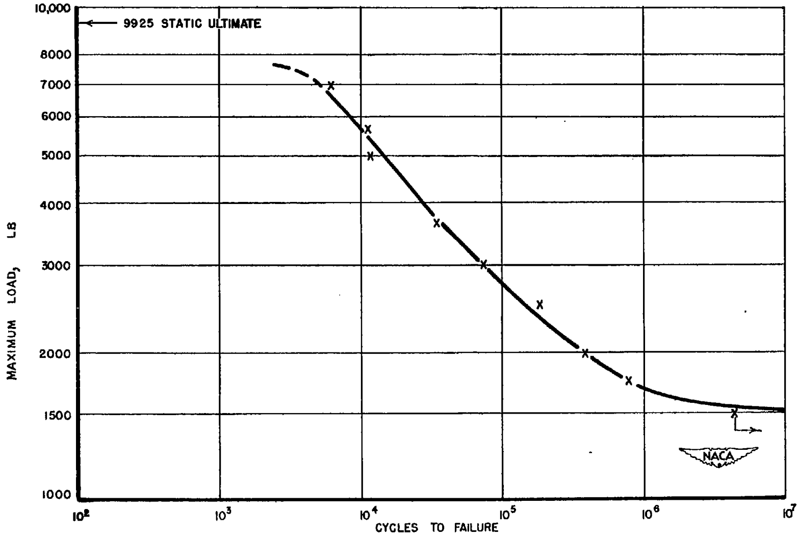
Figure 38.- Direct-stress fatigue test results for lap joints of 75S-T Alclad with two rows of flush rivets. Joints 4\frac{1}{2} inches wide; each row contains eight rivets \frac{1}{2} inch apart; rows \frac{1}{2} inch apart. (R = min. load/max. load = 0.40, in tension.)
