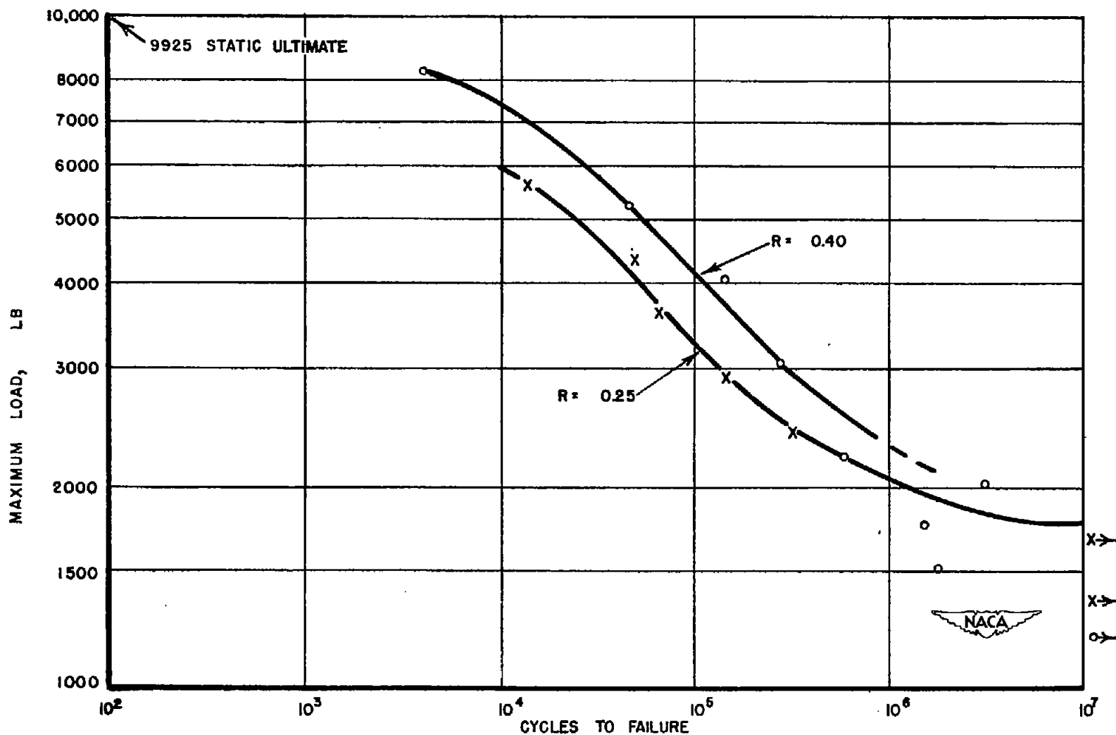
Figure 37.- Direct-stress fatigue test results for lap joints of 24S-T Alclad with three rows of flush rivets. Joints 4\frac{1}{2} inches wide; each row contains eight rivets \frac{1}{2} inch apart; rows \frac{1}{2} inch apart. (R = min. load/max. load. Positive values indicate tension.)
