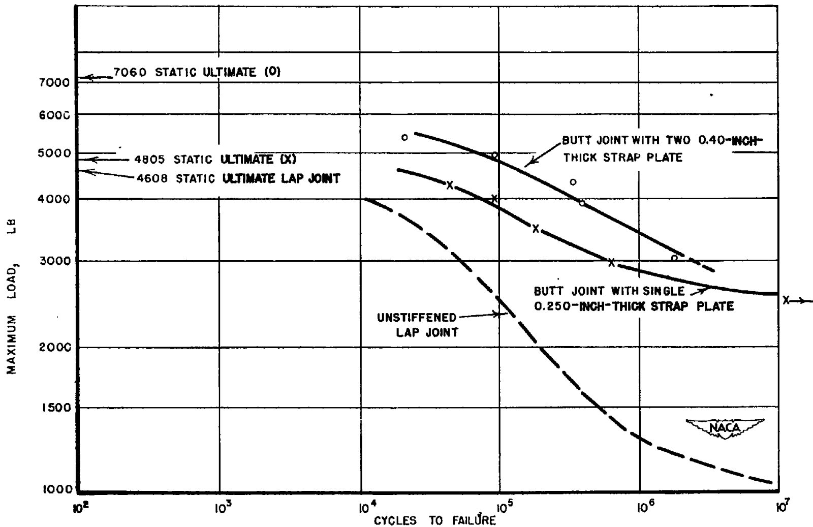
Figure 41.- Direct-stress fatigue test results for riveted butt joints of 0.040-inch 24S-T Alclad with various stiffeners. (R = min. load/max. load = 0.40, in tension.)
