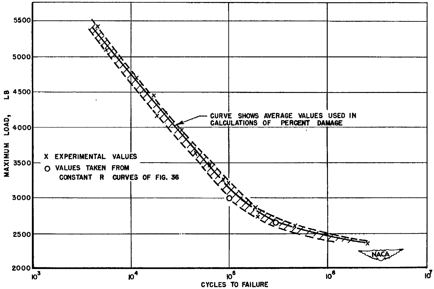
Figure 53.- Scatter band of fatigue strength of lap joints of 24S-T Alclad with two rows of flush rivets. Mean load, 1840 pounds.
