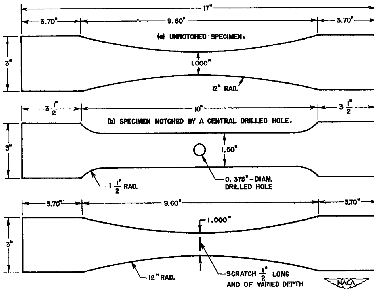
(c) SPECIMEN WITH SCRATCH IN CENTER SECTION. Figure 1.- Sheet specimens used in fatigue tests.
