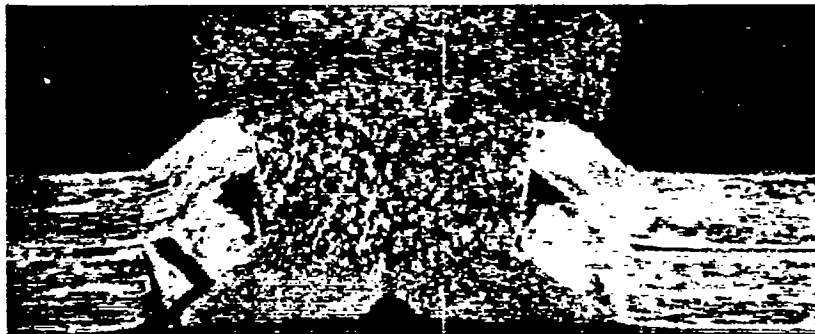
(a) Rivet from joint made by coin dimpling. (Loaded at 150 lb/rivet; lifetime, 2,579,300 cycles)
