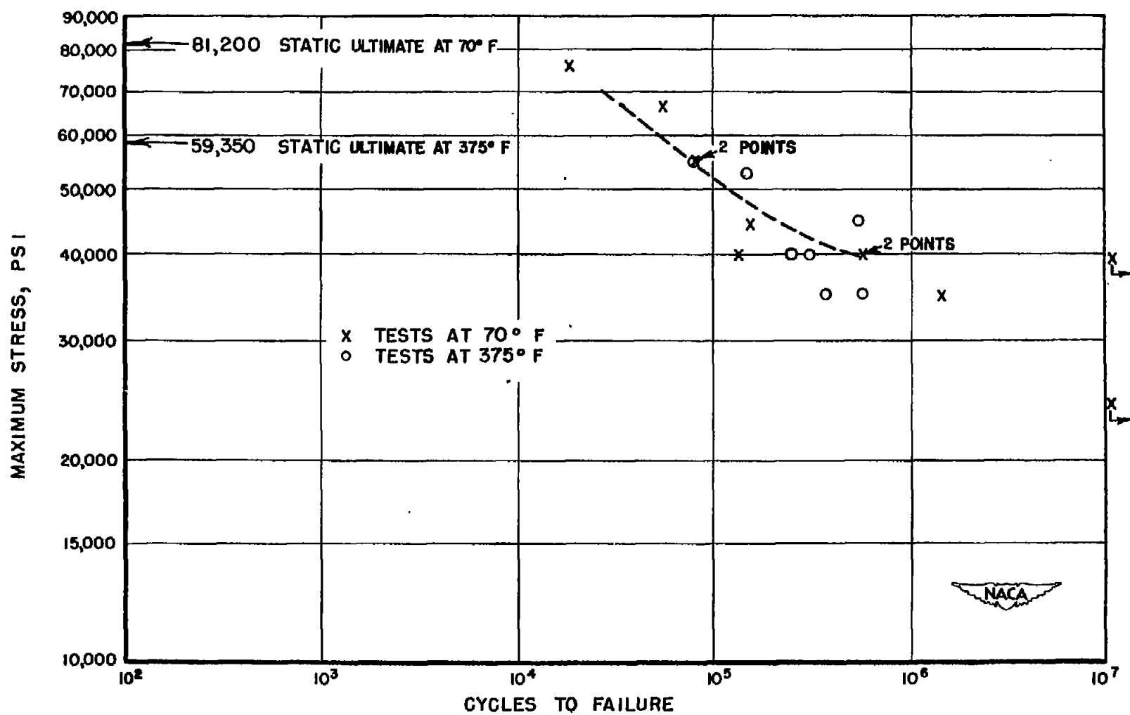
Figure 47.- Results of fatigue tests of 75S-T Alclad sheet at 375° F. Test section, 1,000 by 0.040 inch. Each specimen held at temperature for 1 hour preceding test and tested at temperature. (R = min. load/max. load = 0.40, in tension.)
