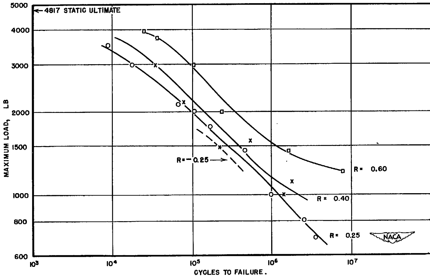
Figure 29.- Direct-stress fatigue strength of riveted lap joints of 0.040-inch R303-T275 clad sheet with a single row of eight rivets. ( R = min. load/max. load. Positive values indicate tension; negative values, compression.)
