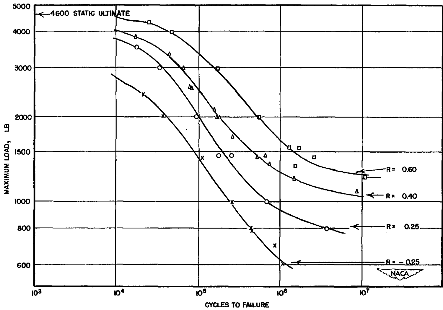
Figure 27.- Direct-stress fatigue strength of riveted lap joints of 0.040-inch 24S-T Alclad sheet with a single row of eight rivets. (R = min. load/max. load. Positive values indicate tension; negative values, compression.)
