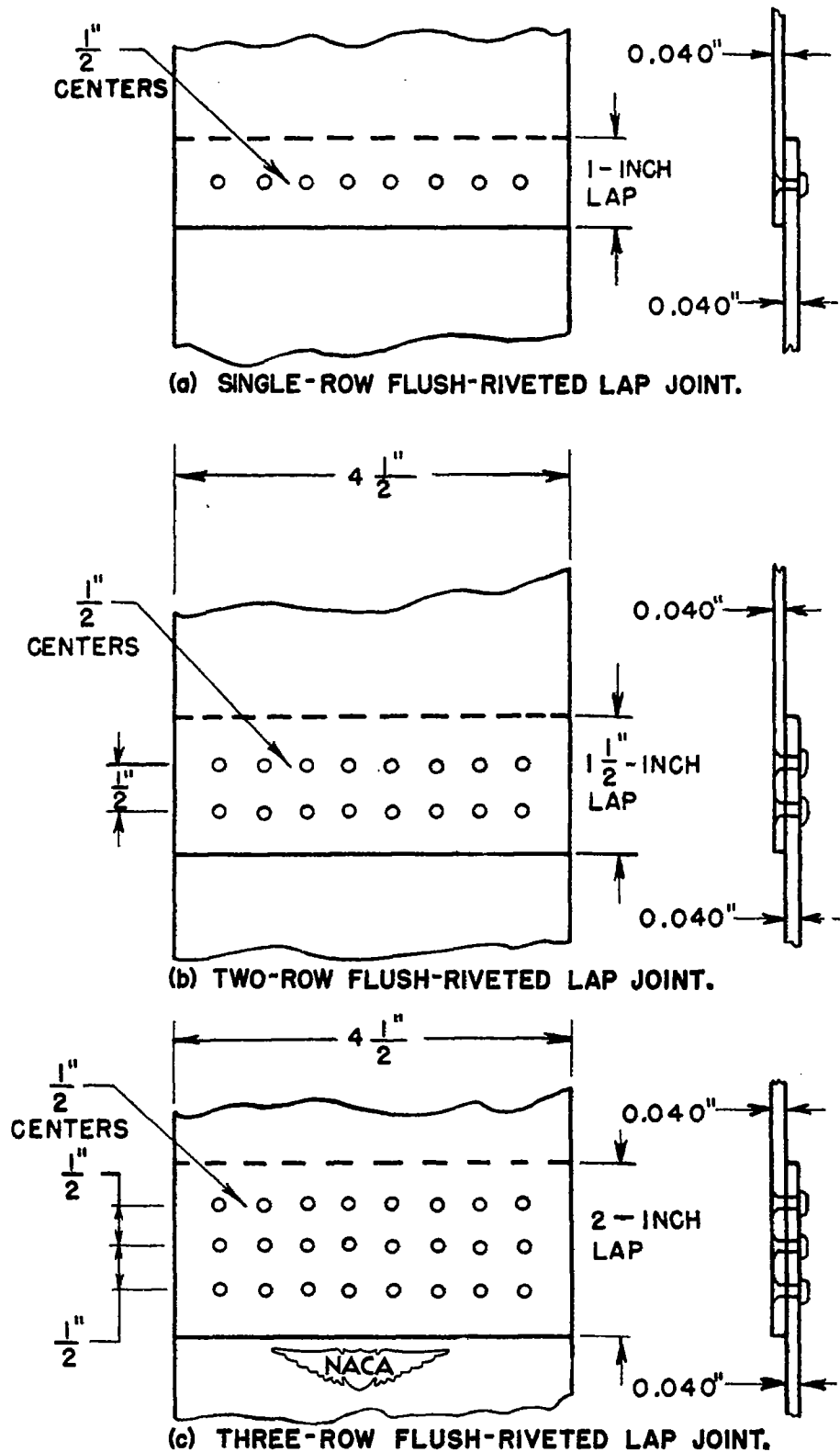
Figure 24.- Riveted lap-joint fatigue test specimens. (Length between grips about 12 in.)
