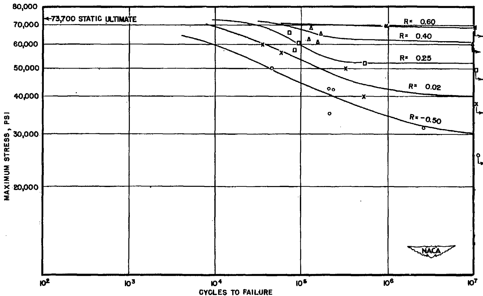
Figure 3.- Direct-stress fatigue strength of 0.040-inch 245-T bare sheet. Test section 1.0 inch wide. Specimens cut in the direction of rolling. (R = min. load/max. load. Positive values indicate tension; negative values, compression.)
