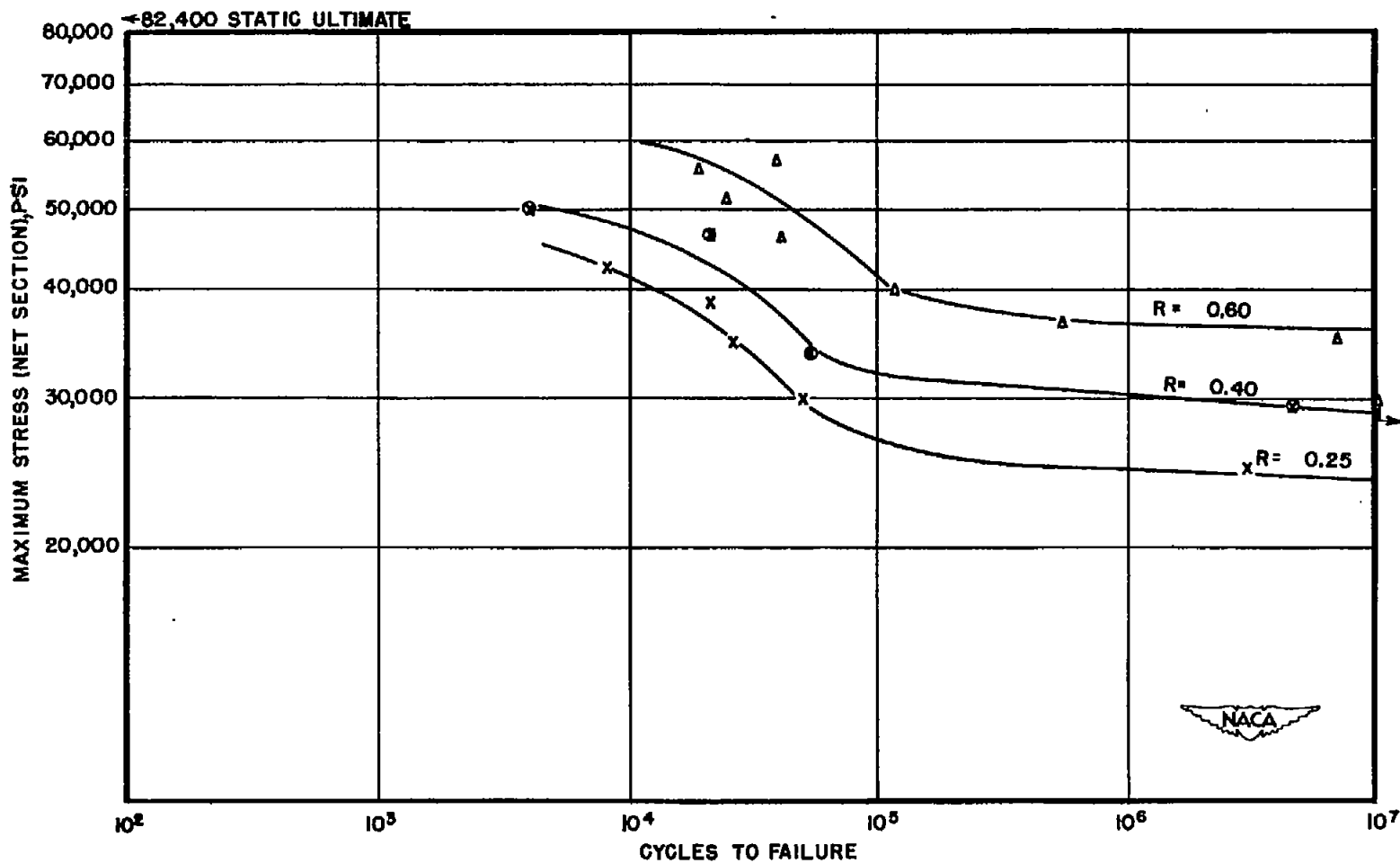
Figure 14.- Direct-stress fatigue strength of 0.040-inch R303-T275 bare sheet. Test section 1.5 inches wide with 0.375-inch-diameter hole. Specimens cut in the direction of rolling. (R = min. load/max. load. Positive values indicate tension.)
