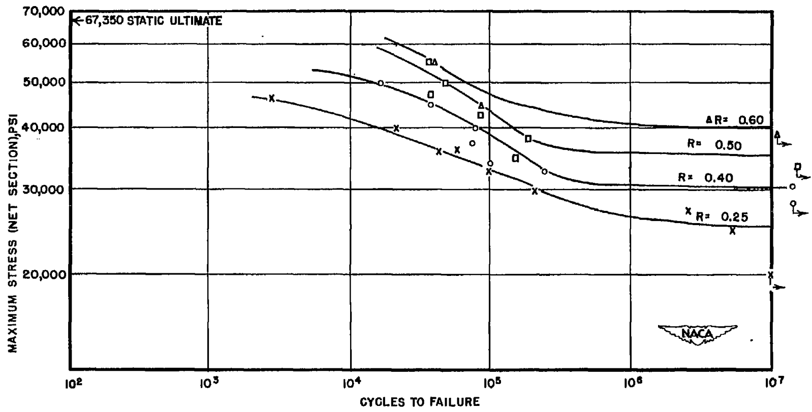
Figure 11.- Direct-stress fatigue strength of 0.040-inch 243-T bare sheet. Test section 1.5 inches wide with 0.375-inch-diameter hole. Specimens cut in the direction of rolling. (R = min. load/max. load. Positive values indicate tension.)
