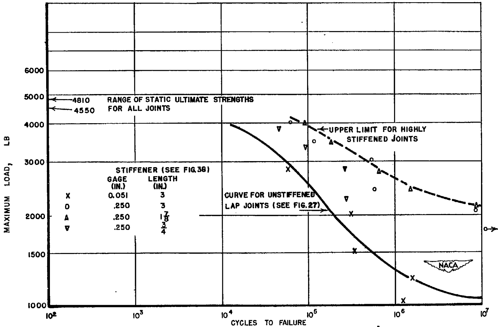
Figure 40.- Direct-stress fatigue test results for riveted lap joints of 0.040-inch 24S-T Alclad with various stiffeners. (R = min. load/max. load = 0.40, in tension.)
