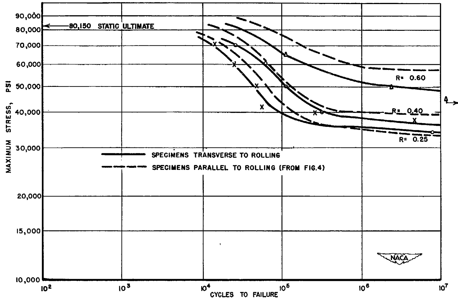
Figure 8.- Direct-stress fatigue strength of 0.040-inch 75S-T Alclad sheet. Test section 1.0 inch wide. Specimens cut transverse to rolling. (R = min. load/max. load. Positive values indicate tension.)
