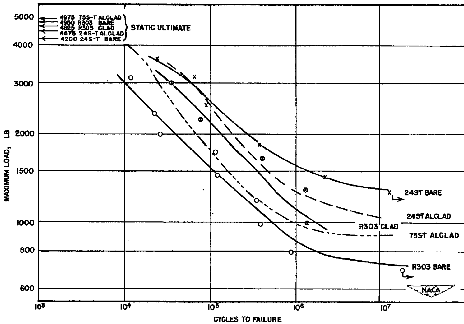
Figure 30.- Comparison of fatigue strengths of simple riveted lap joints of 0.040-inch sheets of various alloys with a single row of eight rivets. (R = min. load/max. load = 0.40, in tension.)
