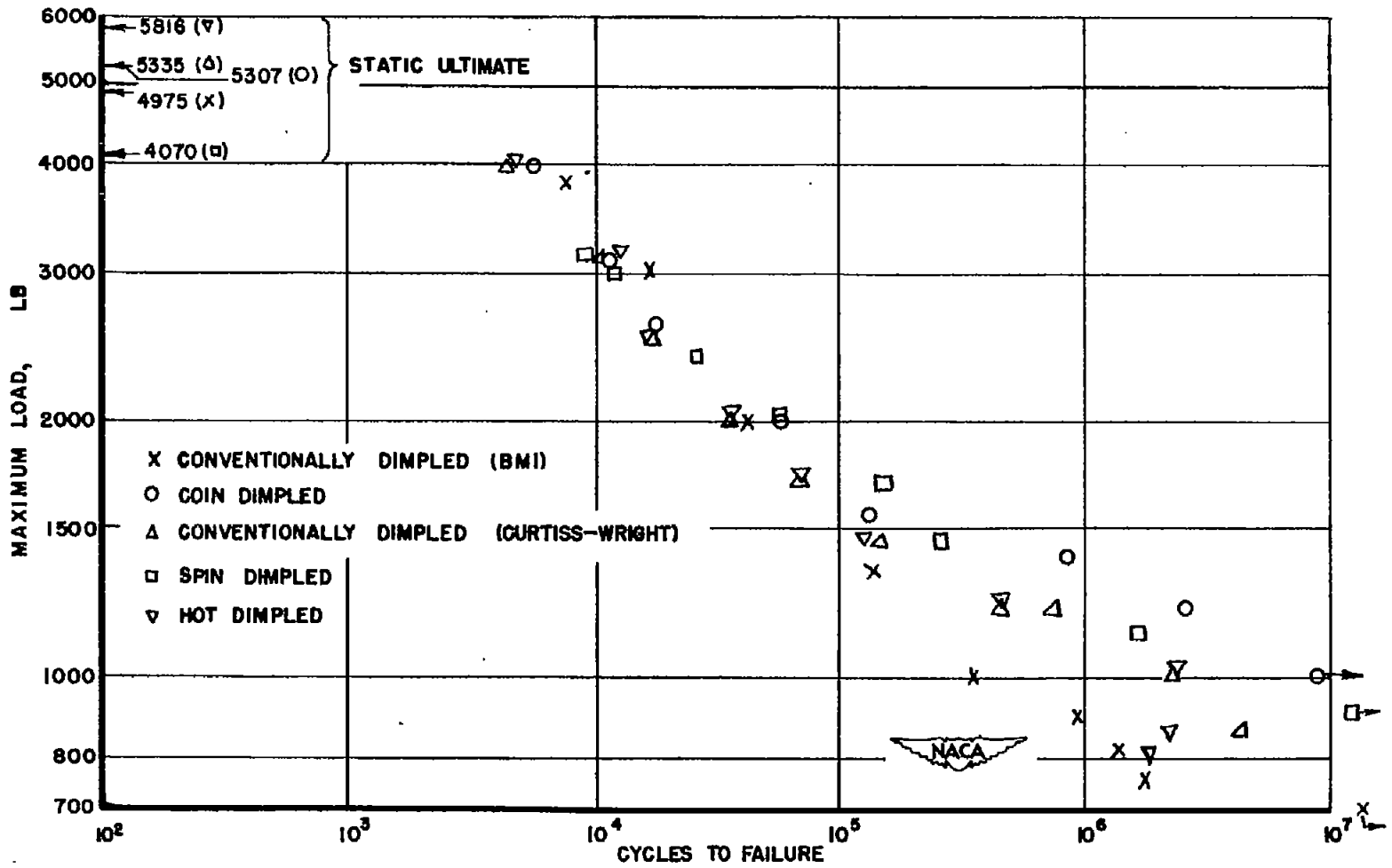
Figure 35.- Results of direct-stress fatigue tests for several sets of single-row flush-riveted lap joints of 75S-T Alclad sheets. (R = min. load/max. load = 0.40, in tension.)
