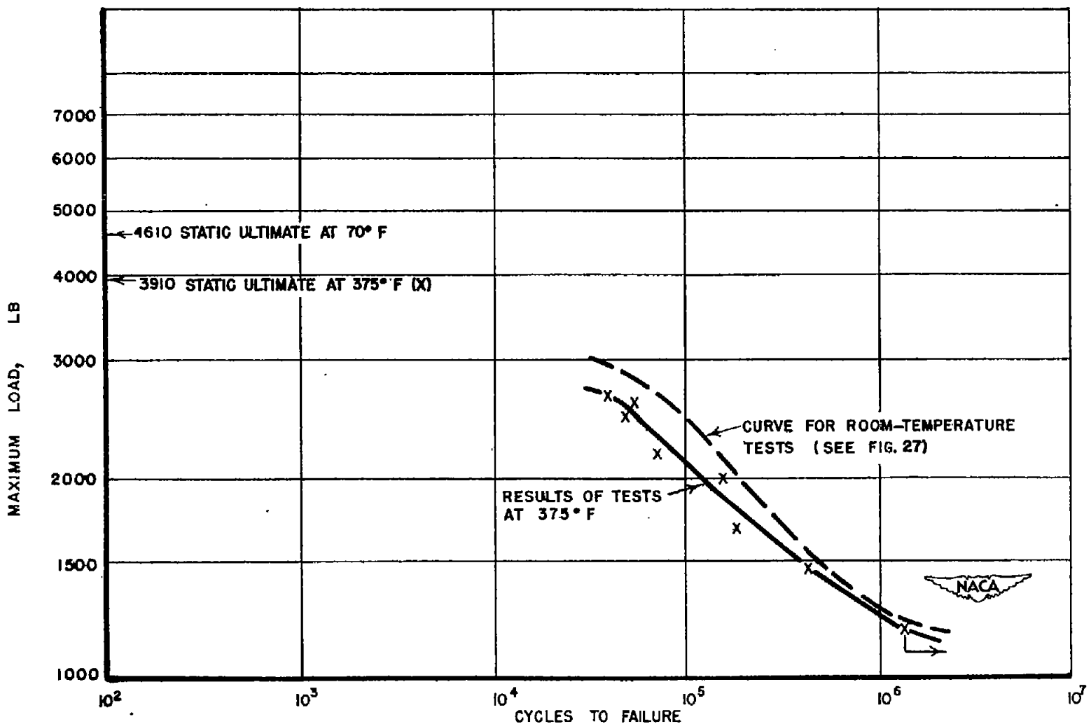
Figure 48.- Results of fatigue tests at 375° F for single-row riveted lap joints of 24S-T Alclad sheet. (R = min. load/max. load = 0.40, in tension.)
