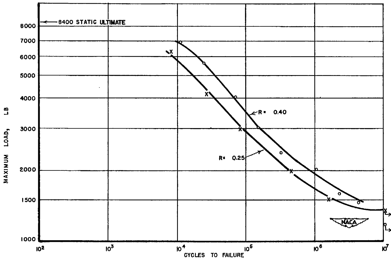
Figure 36.- Direct-stress fatigue strength of lap joints of 24S-T Alclad with two rows of flush rivets. Joints 4\frac{1}{2} inches wide; each row contains eight rivets \frac{1}{2} inch apart; rows \frac{1}{2} inch apart. (R = min. load/max. load. Positive values indicate tension.)
