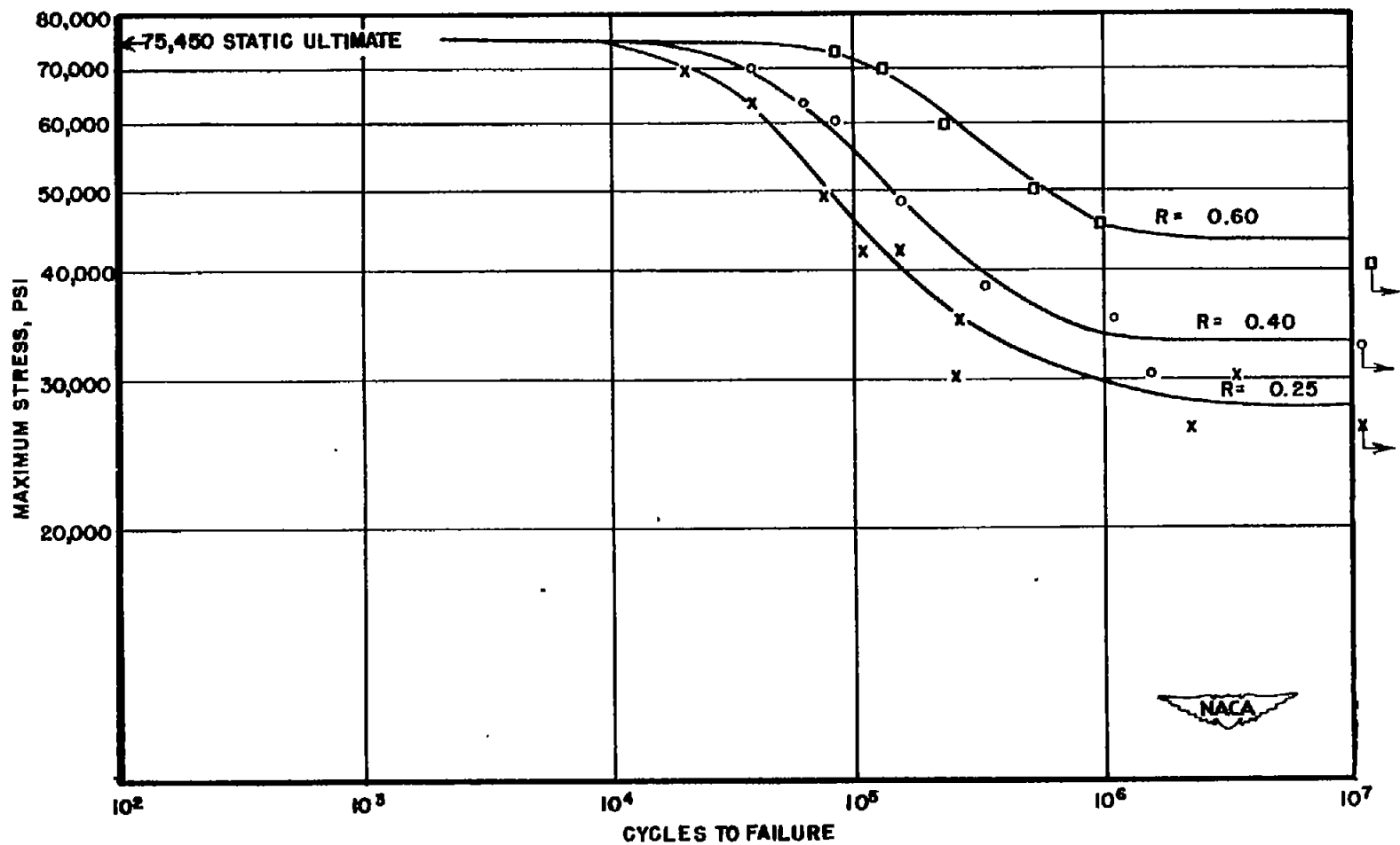
Figure 5.- Direct-stress fatigue strength of 0.040-inch R303-T275 clad sheet. Test section 1.0 inch wide. Specimens cut in the direction of rolling. (R = min. load/max. load. Positive values indicate tension.)
