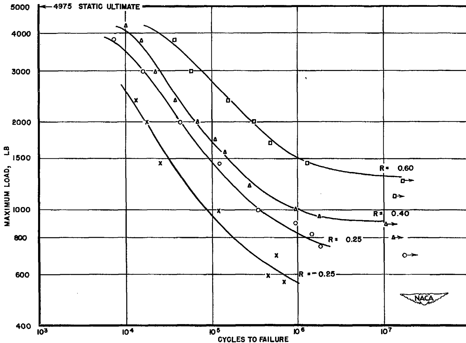
Figure 28.- Direct-stress fatigue strength of riveted lap joints of 0.040-inch 75S-T Alclad sheet with a single row of eight rivets. (R = min. load/max. load. Positive values indicate tension; negative values, compression.)
