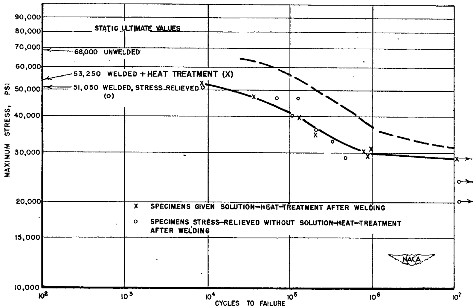
Figure 43.- Direct-stress fatigue test results for multi-arc-welded specimens of 0.040-inch 24S-T Alclad. (R = min. load/max. load = 0.40, in tension.)
