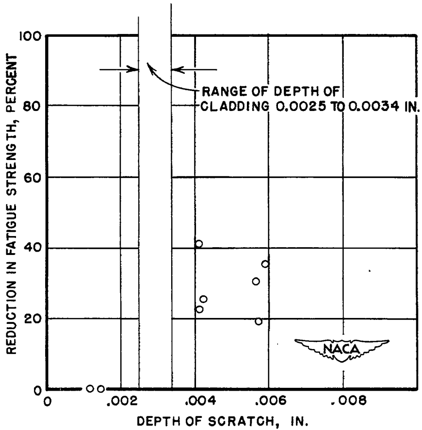
Figure 17.- Effect of scratches of various depths on the fatigue strength of 0.102-inch-thick 24S-T Alclad sheet.
