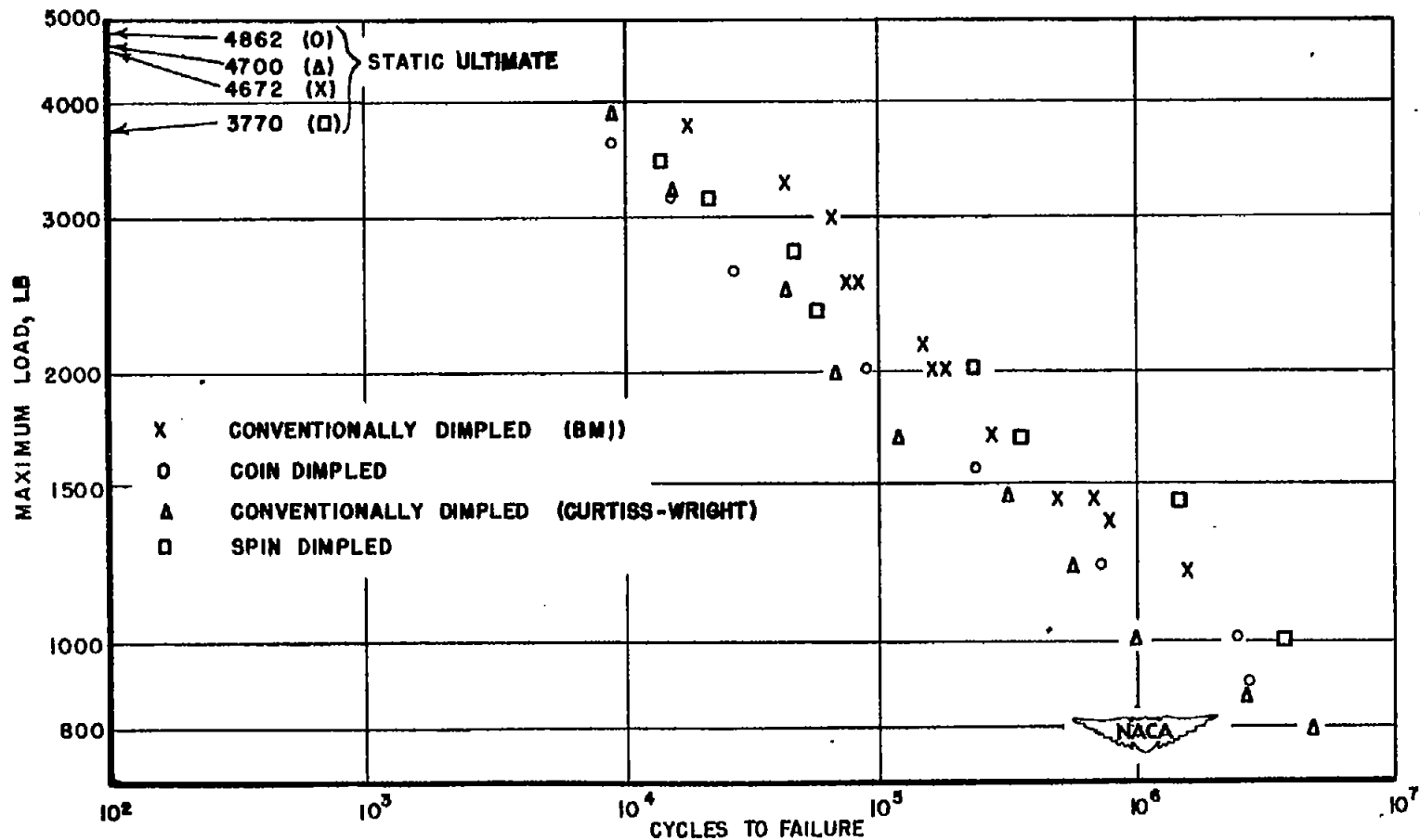
Figure 34.- Results of direct-stress fatigue tests for several sets of single-row flush-riveted lap joints of 24S-T Alclad sheet. (R = min. load/max. load = 0.40, in tension.)
