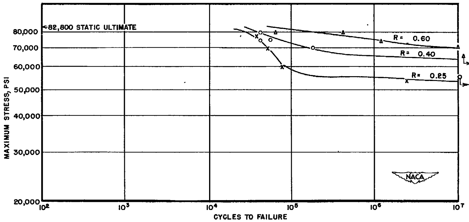
Figure 6.- Direct-stress fatigue strength of 0.040-inch R303-T275 bare sheet. Test section 1.0 inch wide. Specimens cut in the direction of rolling. (R = min. load/max. load. Positive values indicate tension.)
