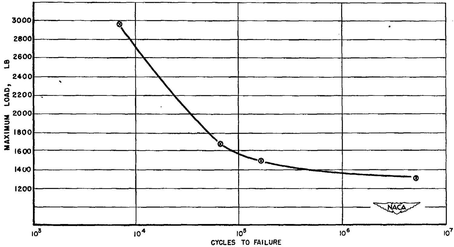
Figure 52.- Constant-mean-load fatigue curve for lap joints of 75S-T Alclad with a single row of flush rivets. Mean load, 1055 pounds. Points taken from constant R curves of figure 28.
