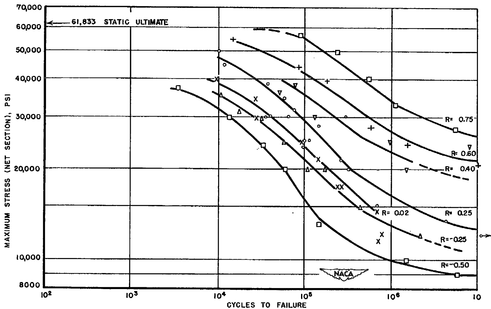
Figure 10.- Direct-stress fatigue strength of 0.040-inch 24S-T Alclad sheet. Test section 1.5 inches wide with 0.375-inch-diameter hole. Specimen cut in the direction of rolling. (R = min. load/max. load. Positive values indicate tension; negative values, compression.)
