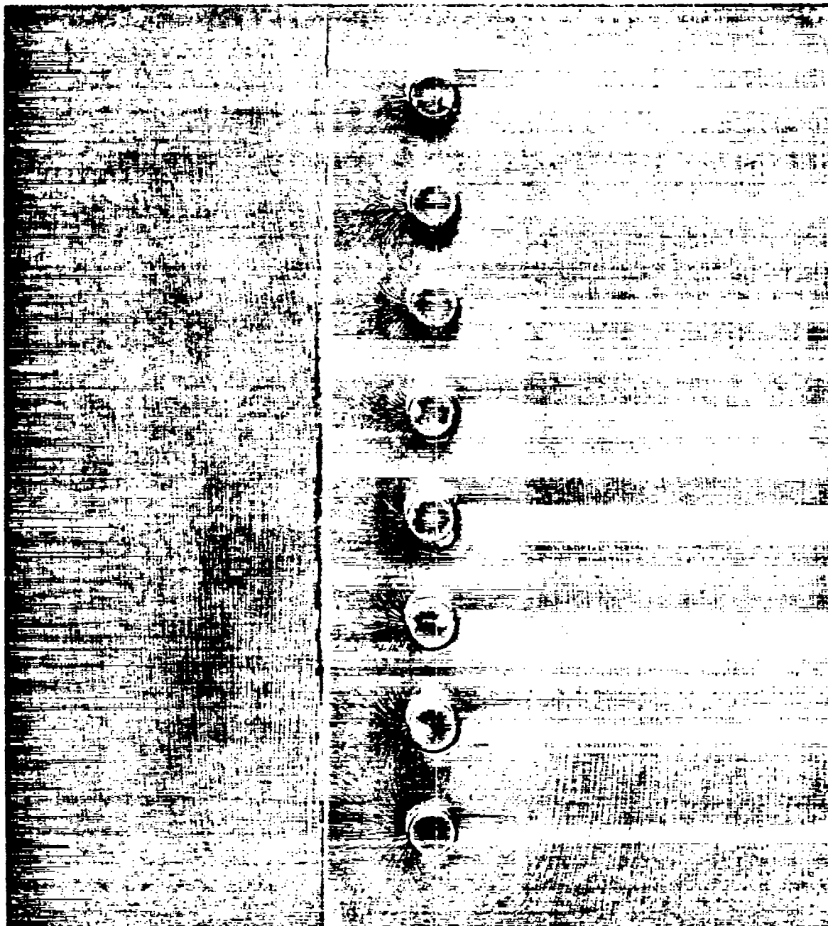
Figure 19.- Stress-coat pattern in a lap joint with a single row of rivets.
