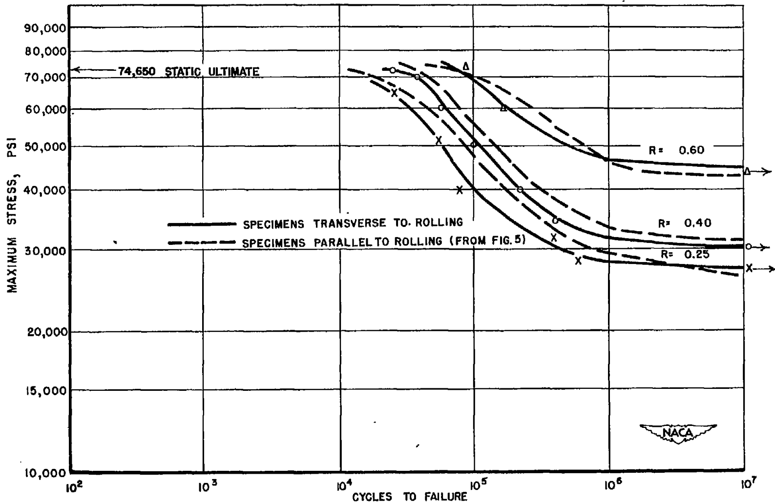
Figure 9.- Direct-stress fatigue strength of 0.040-inch R303-T275 clad sheet. Test section 1.0 inch wide. Specimens cut transverse to direction of rolling. (R = min. load/max. load. Positive values indicate tension.)
