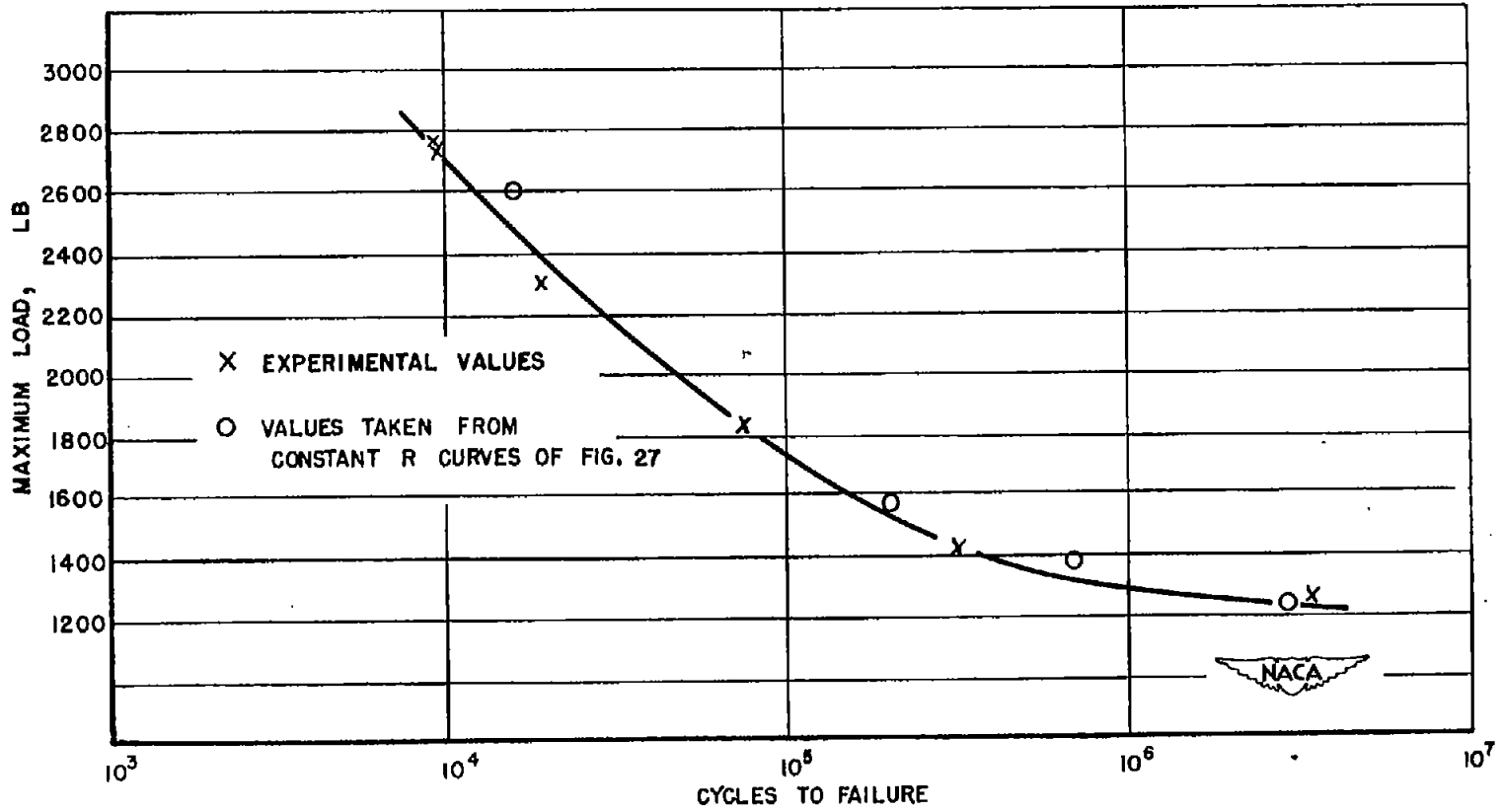
Figure 51.- Constant-mean-load fatigue curve for lap joints of 24S-T Alclad with a single row of flush rivets. Mean load, 975 pounds.
