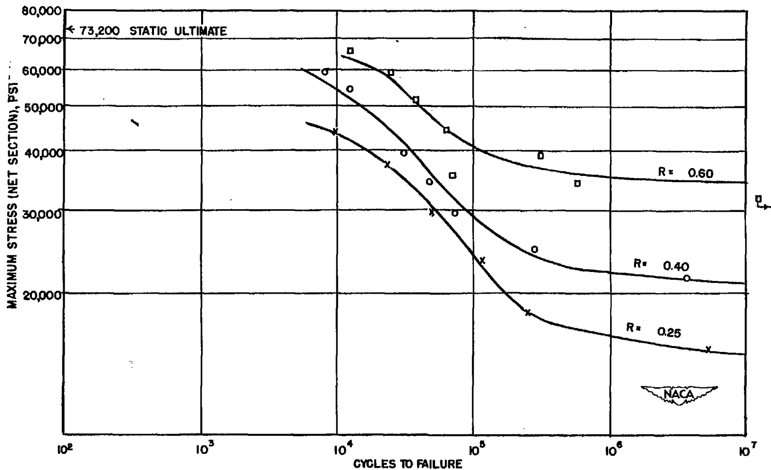
Figure 13.- Direct-stress fatigue strength of 0.040-inch R303-T275 clad sheet. Test section 1.5 inches wide with 0.375-inch-diameter hole. Specimens cut in the direction of rolling. (R = min. load/max. load. Positive values indicate tension.)
