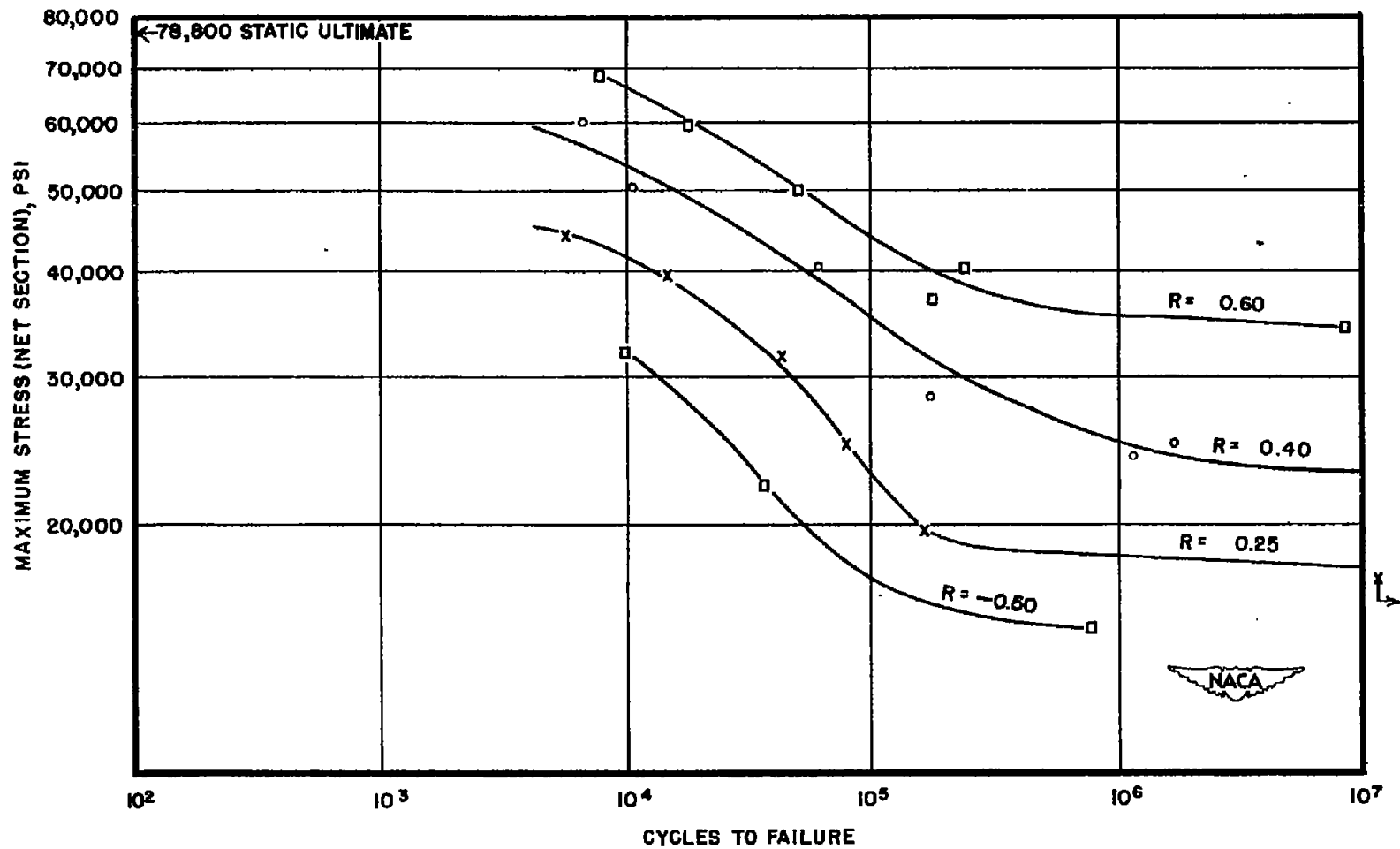
Figure 12.- Direct-stress fatigue strength of 0.040-inch 75S-T Alclad sheet. Test section 1.5 inches wide with 0.375-inch-diameter hole. Specimens cut in the direction of rolling. (R = min. load/max. load. Positive values indicate tension; negative values, compression.)
