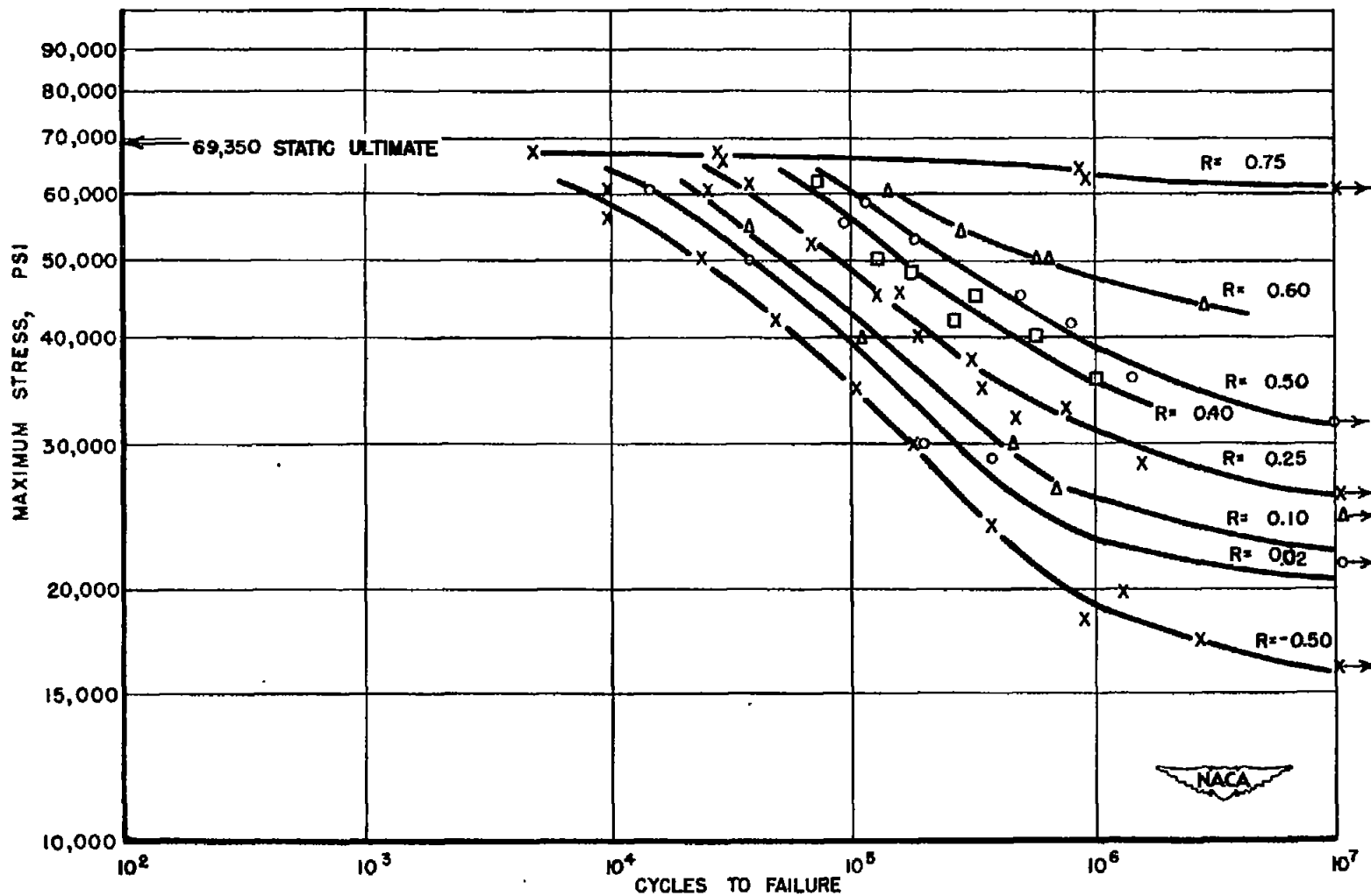
Figure 2.- Direct-stress fatigue strength of 0.040-inch 24S-T Alclad sheet. Test section 1.0 inch wide. Specimens cut in the direction of rolling. (R = min. load/max. load. Positive values indicate tension; negative values, compression.)
