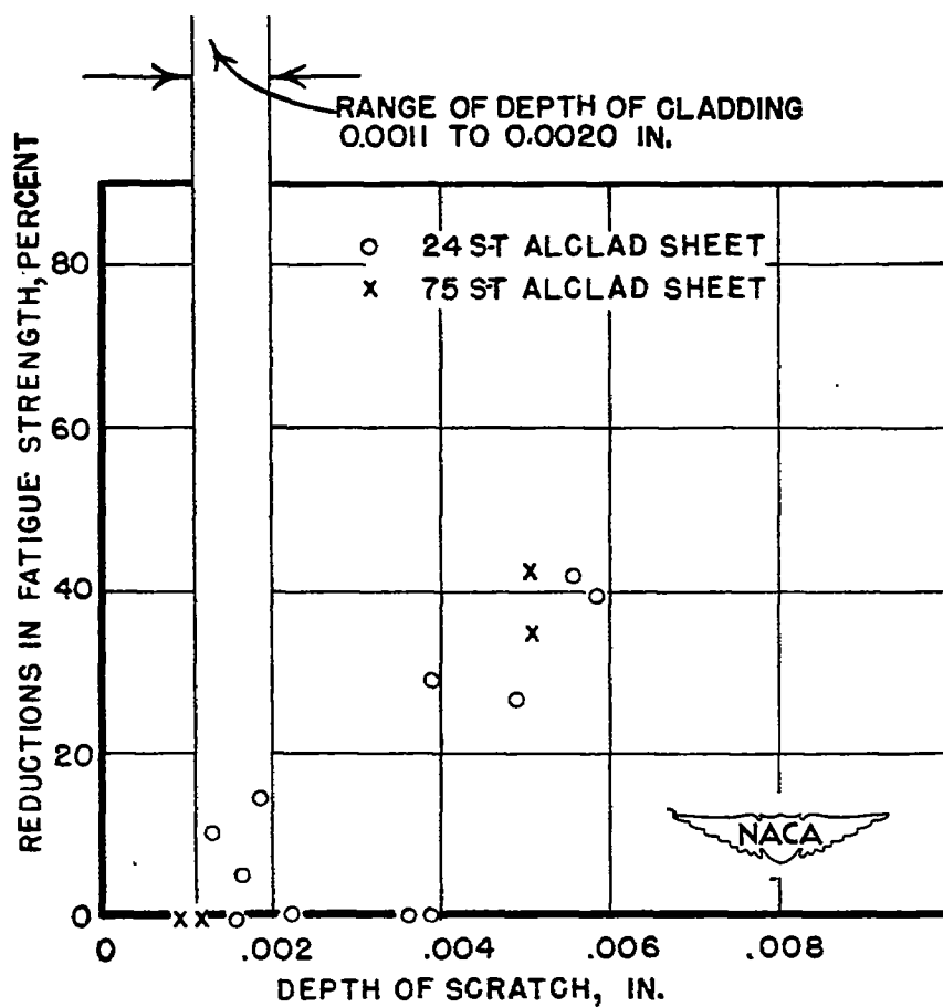
Figure 16.- Effect of scratches of various depths on the fatigue strength of 0.040-inch-thick 24S-T Alclad sheet and 75S-T Alclad sheet.
