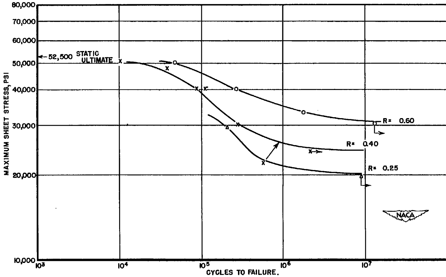
Figure 45.- Direct-stress fatigue test results for sheet efficiency of riveted 0.040-inch sheets of Alclad 24S-T. See figure 23 for details of specimen. (R = min. load/max. load. Positive values indicate tension.)
