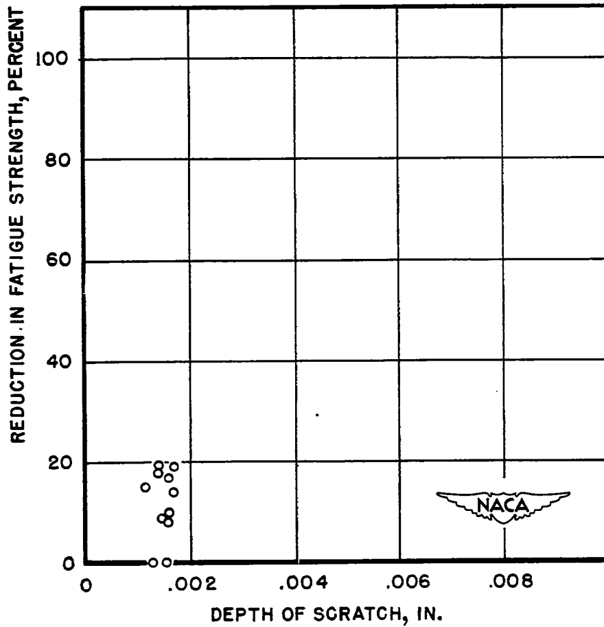
Figure 18.- Effect of scratches of various depths on the fatigue strength of 0.040-inch-thick 24S-T bare sheet.
