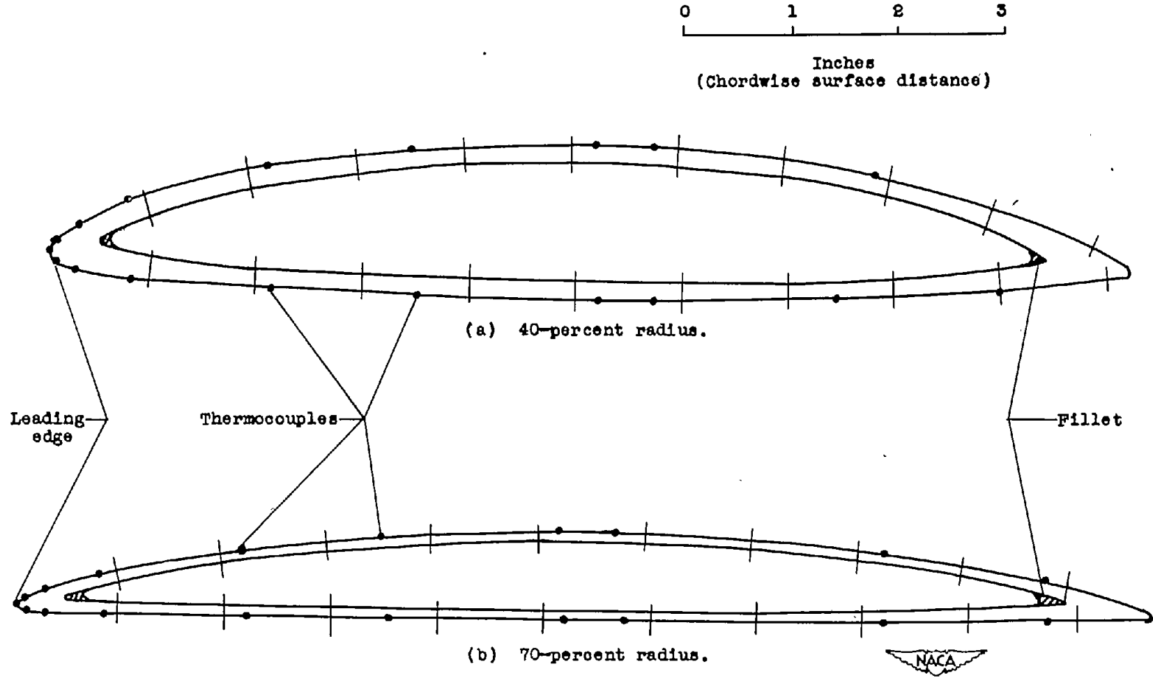
Figure 8.- Chordwise thermocouple locations.
