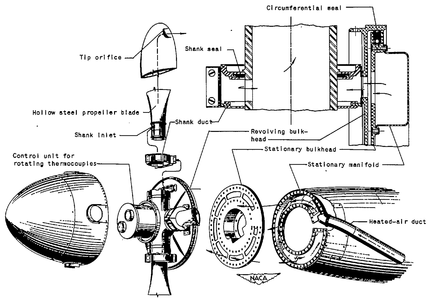
Figure 3. - Details of air-heated propeller installation.
