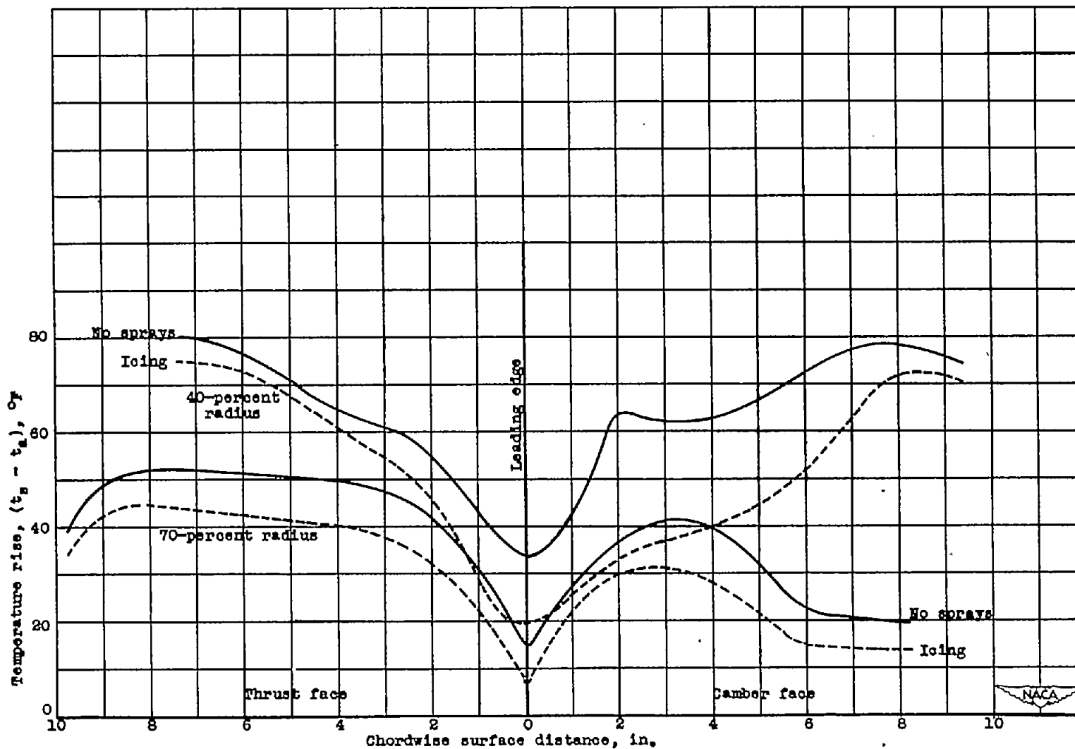
Figure 13.- Comparison of blade-surface temperature rise above tunnel-air temperature for no-spray and icing conditions at 40- and 70-percent blade radius. Blade angle, 28^\circ ; propeller speed, 1050 rpm; heating rate, 35,000 Btu per hour per blade.
