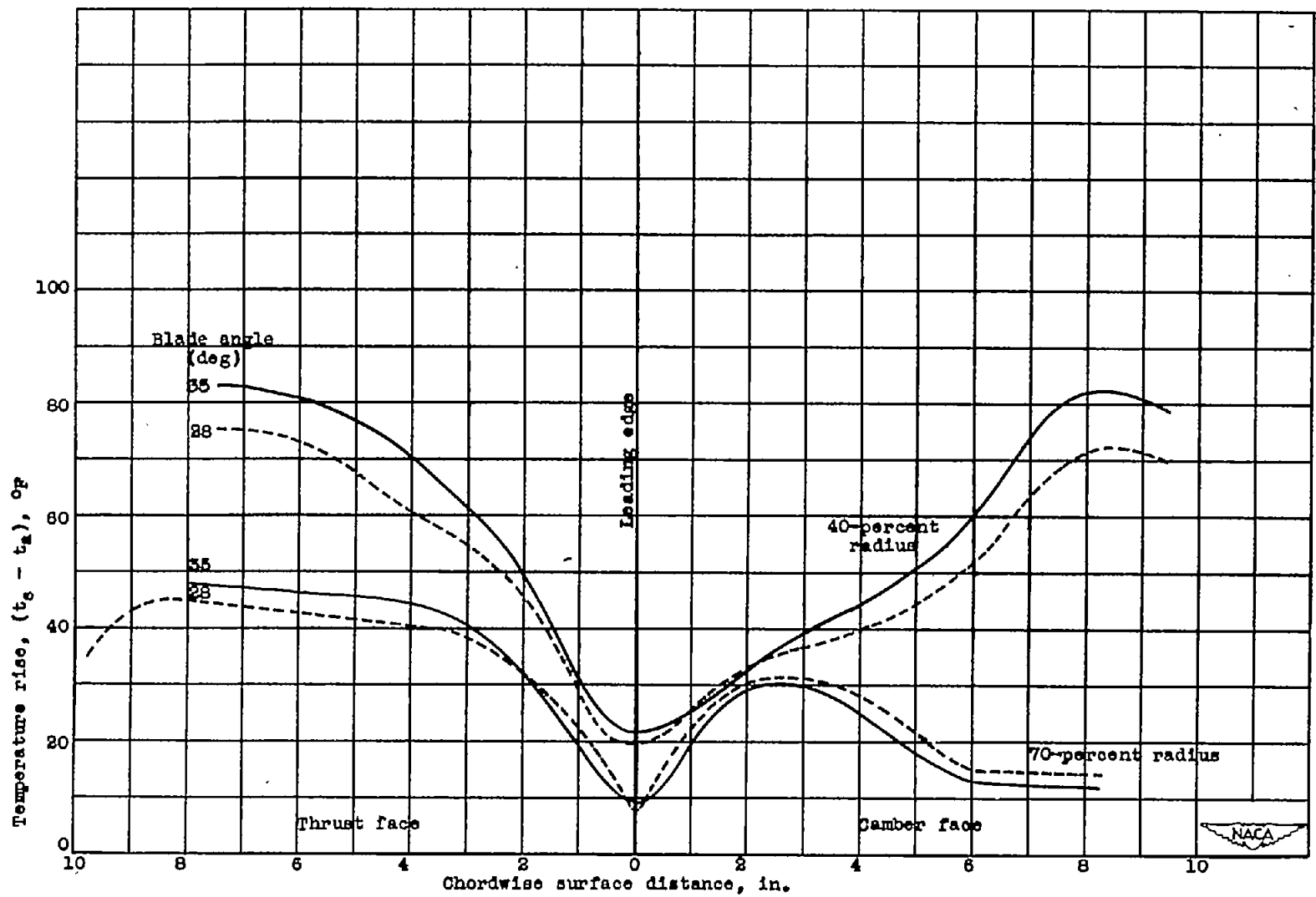
Figure 14.- Comparison of blade-surface temperature rise above tunnel-air temperature for icing conditions at 40- and 70-percent blade radius, using blade angles of 28° to 35° with propeller speeds of 1050 and 850 rpm, respectively. Heating rate, 35,000 Btu per hour per blade.
