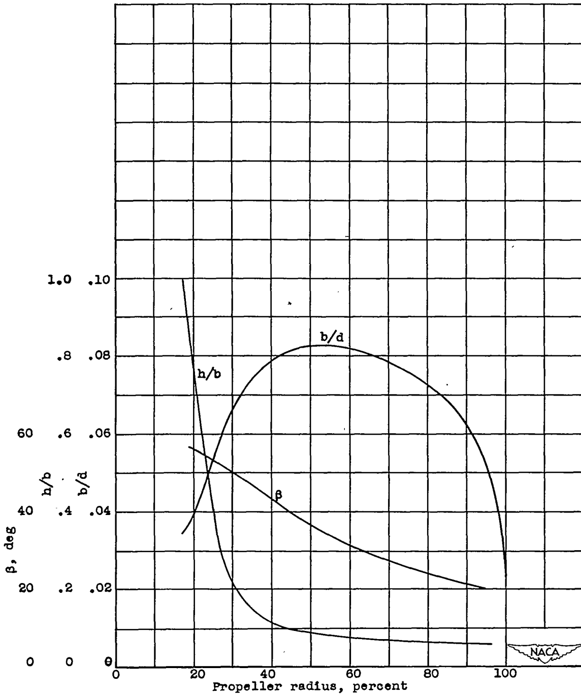
Figure 2.- Blade characteristics of hollow steel air-heated propeller. Propeller diameter, 10 feet, 2 inches; \beta , blade angle, degrees; h , blade thickness, feet; b , blade chord, feet; d , propeller diameter, feet.
