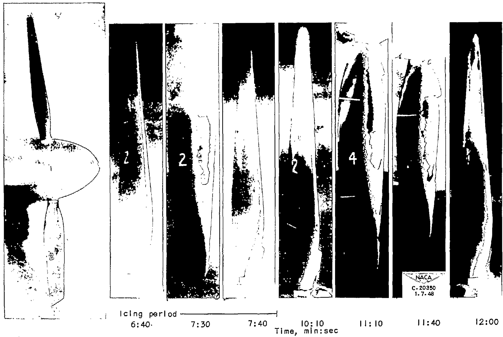
Figure 16. - Stroboscopic photographs of unheated propeller blades during and following 10-minute icing period. Tunnel-air temperature, 11° F; blade angle, 35°; propeller speed, 850 rpm.
