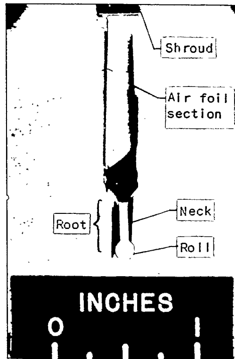
(b) Long-necked turbine blade, side view.
