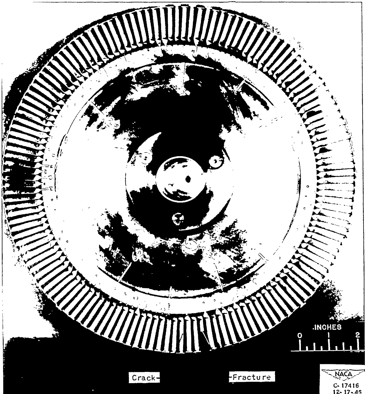
(a) Turbine wheel showing cracked and fractured blades.
