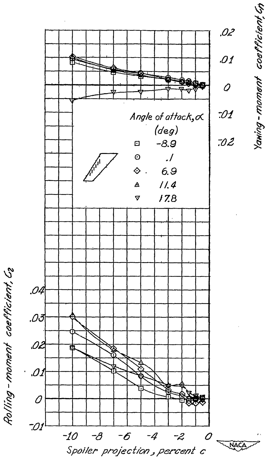
Figure 11.- Variation of rolling-moment and yawing-moment coefficients with spoiler projection. Spoiler 18.
