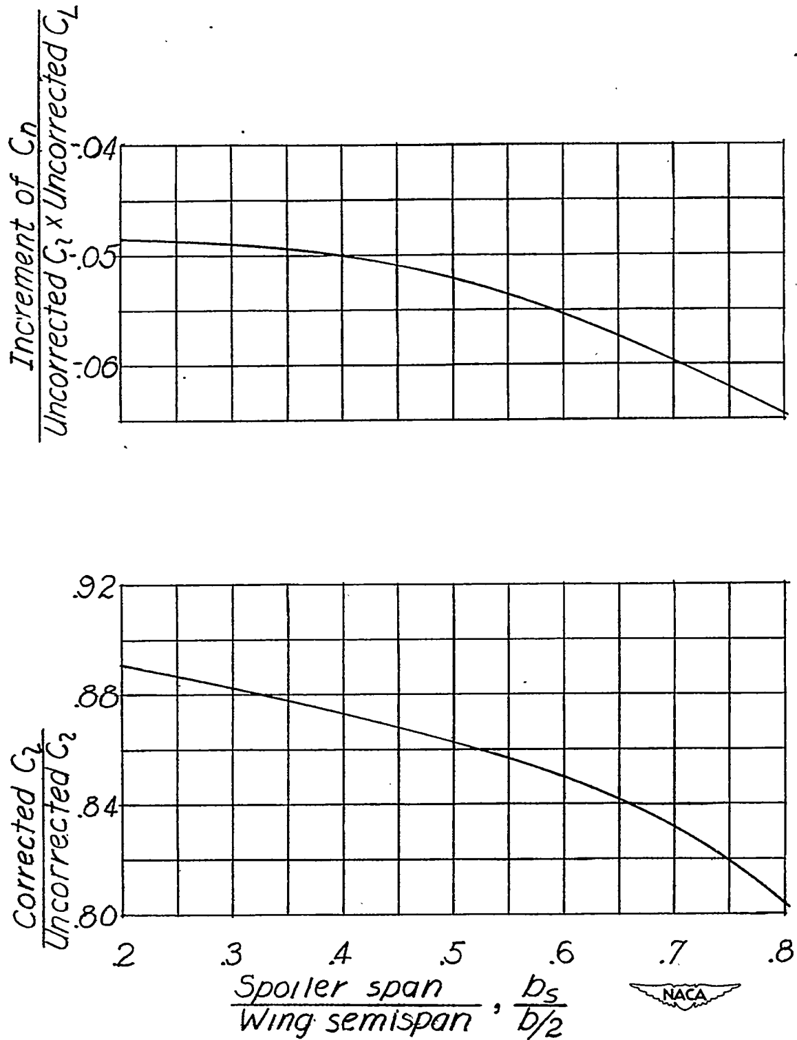
Figure 2.- Variation of corrections to rolling-moment and yawing-moment coefficients with ratio of spoiler span to wing semispan.
