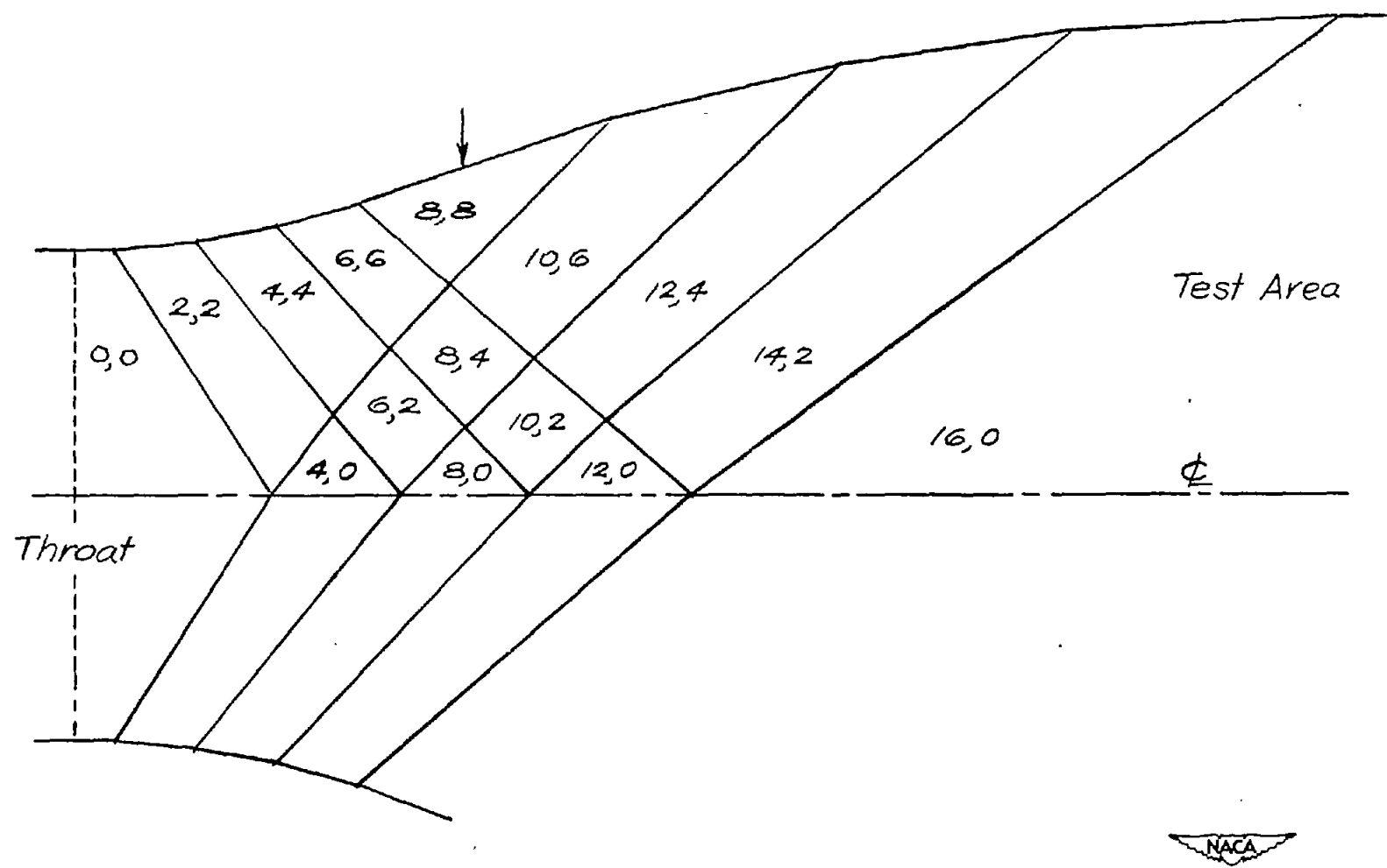
Figure 8.- Flow field in a nozzle with no waves reflected.
