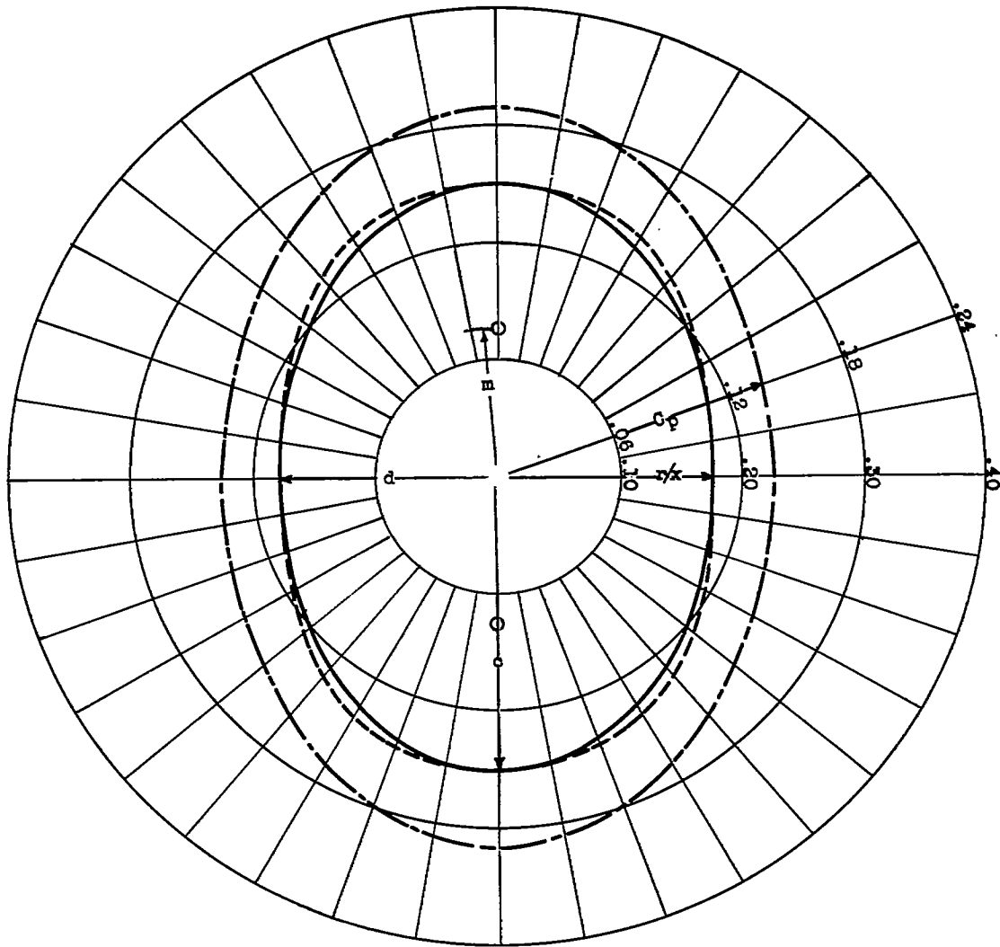
Figure 5. - Comparison of desired elliptical body with calculated body and resulting pressure distribution. \beta = 1.5 ; m = 0.125 ; K/U = 0.0220 .
