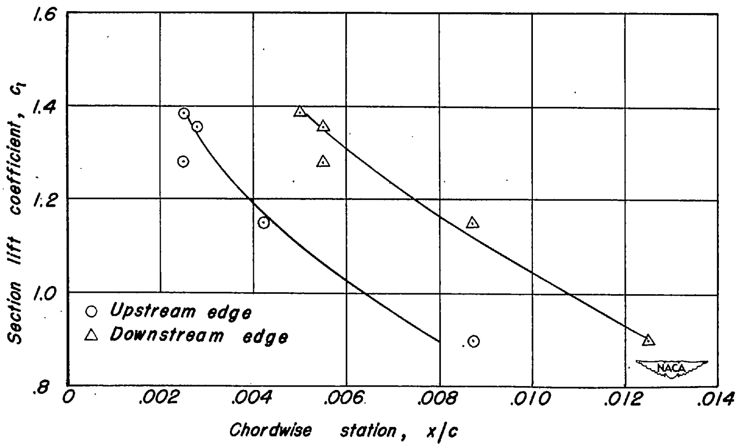
Figure 11.- Extent of the band of froth on the basic airfoil as indicated by liquid film.
