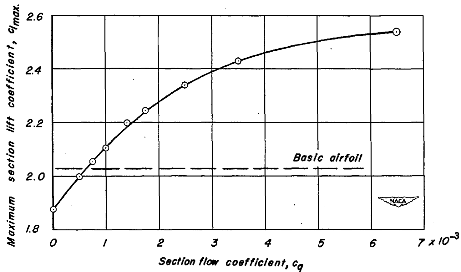
Figure 7.- Variation of maximum lift with flow coefficient for the model with the flap deflected 40°. Slot 15.
