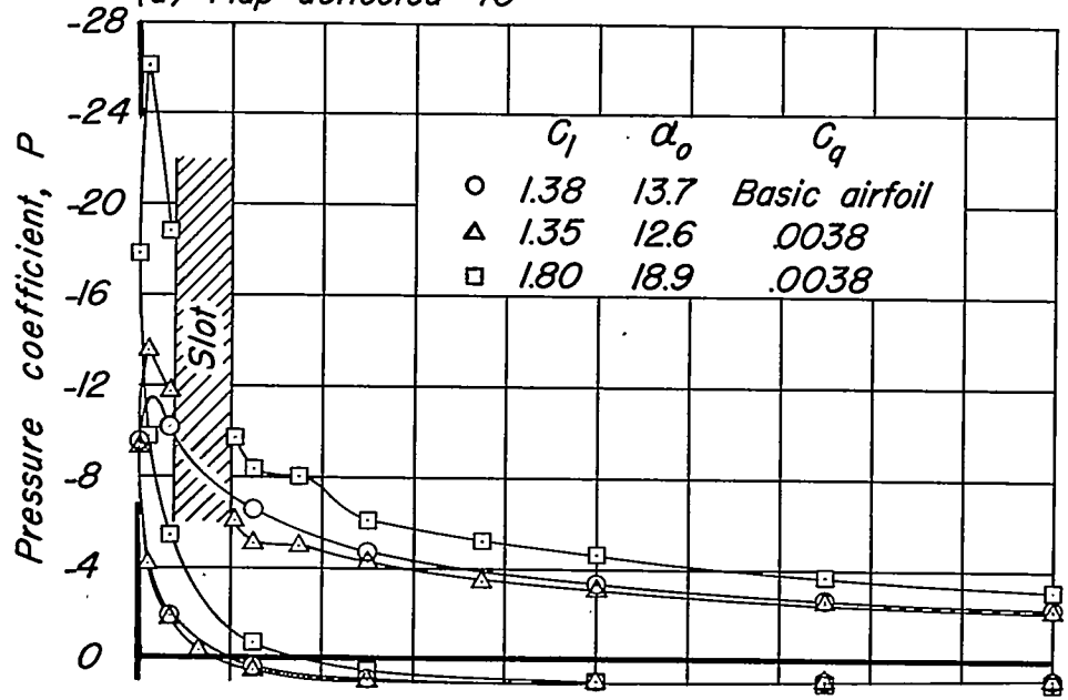
(a) Flap deflected 40°
