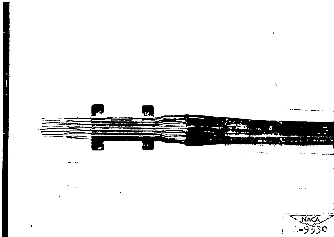
Figure 3.- Detail of small boundary-layer rake or "mouse."
