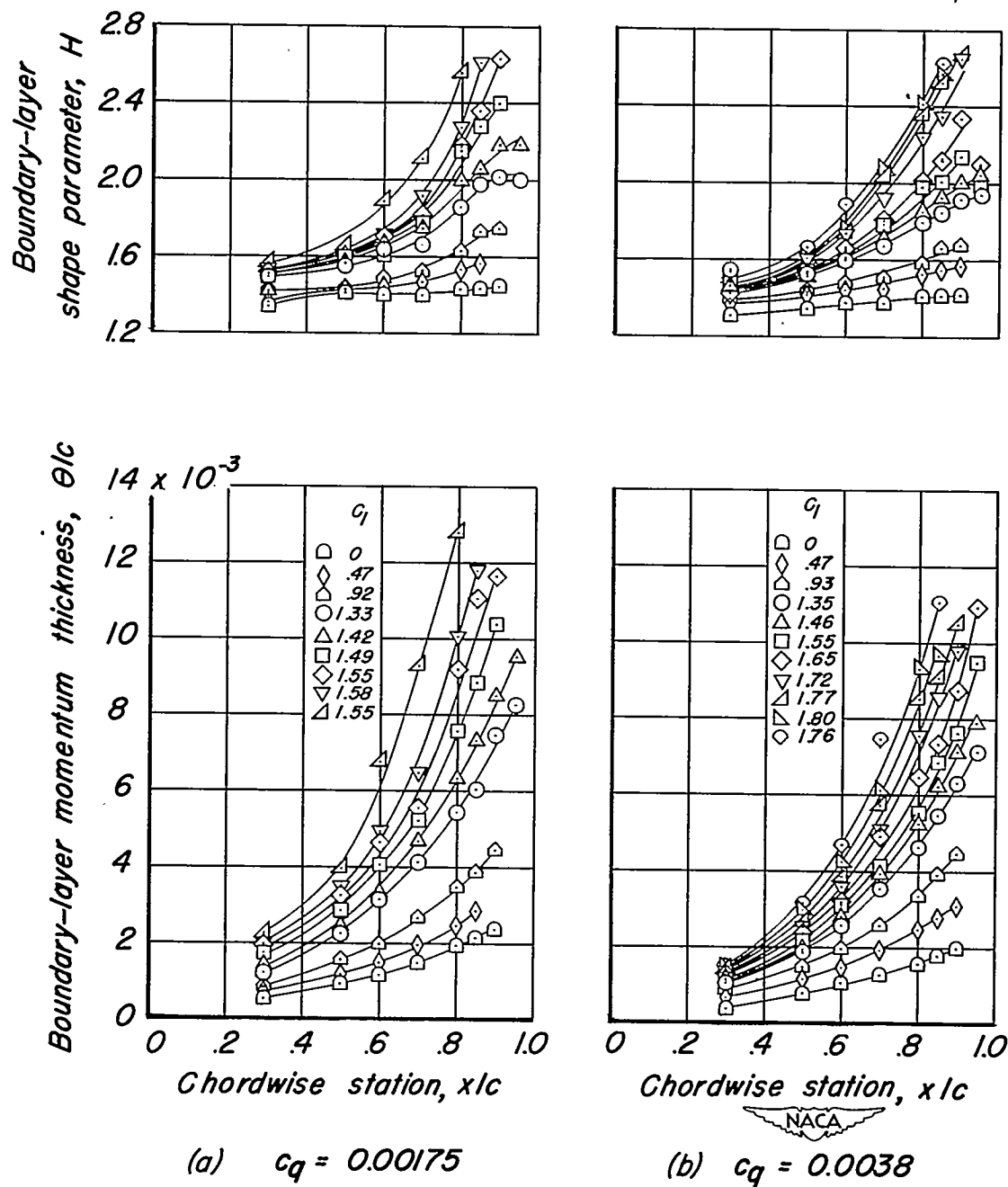
Figure 12.- Chordwise variation of the boundary-layer shape parameter and momentum thickness. Slot 15.
