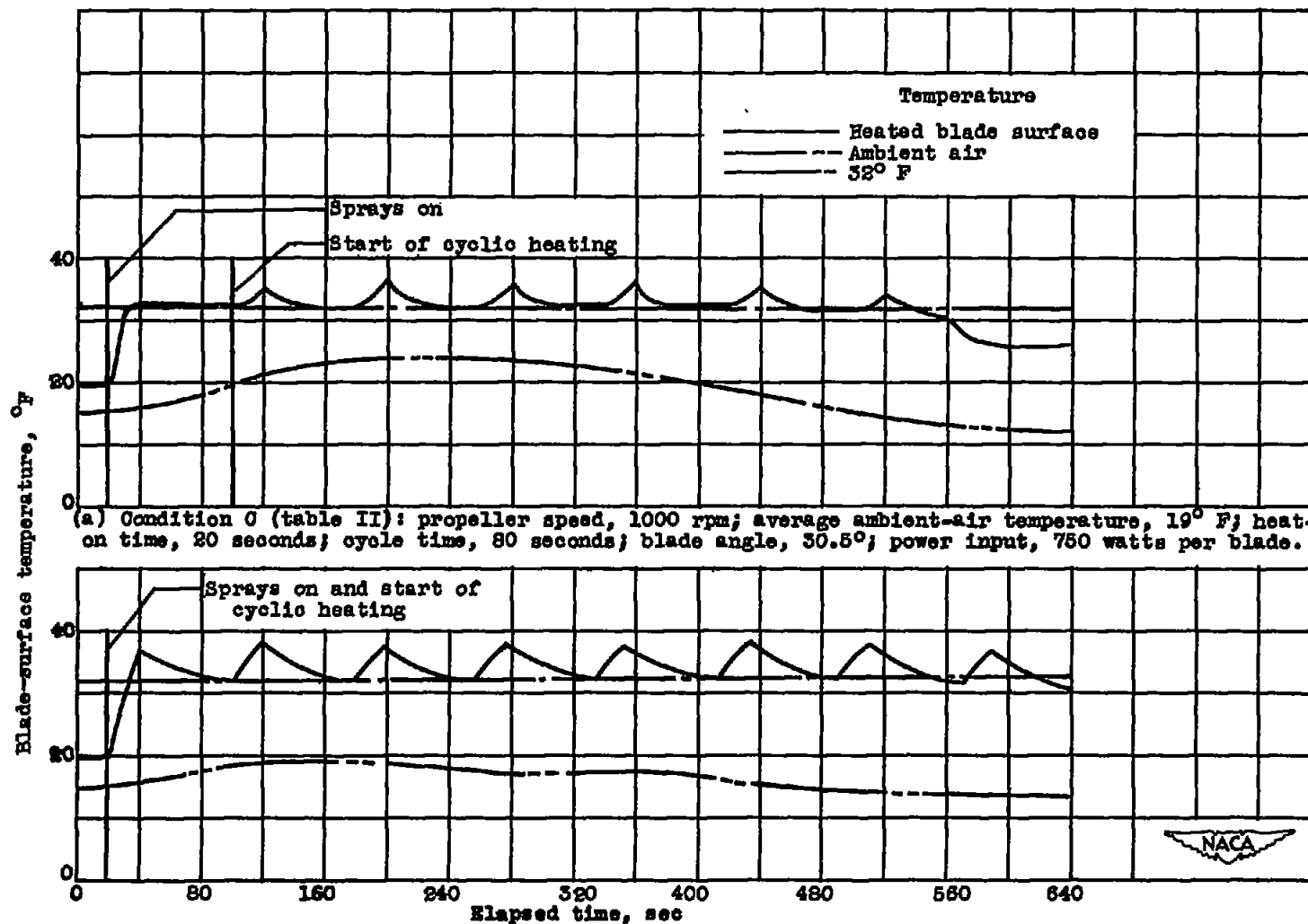
Figure 10. - Typical variation of leading-edge blade-surface temperature with time during cyclic de-icing at 33-percent radius.
