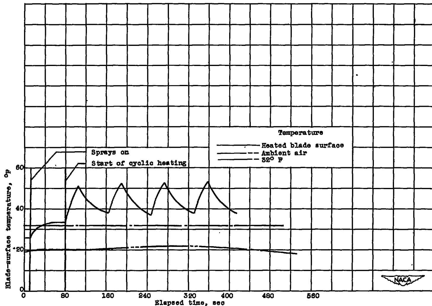
(1) Condition N (table II): propeller speed, 800 rpm; average ambient-air temperature, 20° F; heat-on time, 24 seconds; cycle time, 84 seconds; blade angle, 34.5°; power input, 1250 watts per blade. Figure 10. - Concluded. Typical variation of leading-edge blade-surface temperature with time during cyclic de-icing at 35-percent radius.
