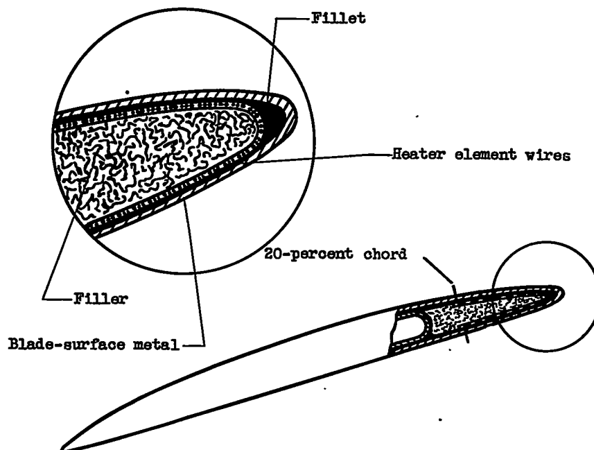
(b) Cross section of heater at propeller-radius ratio of 0.75.
