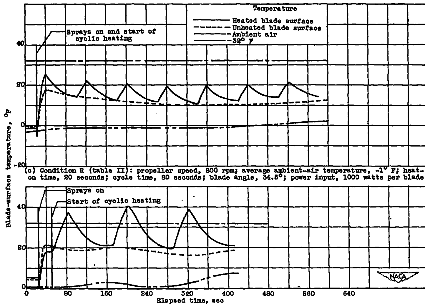
Figure 10. - Continued. Typical variation of leading-edge blade-surface temperature with time during cyclic de-icing at 33-percent radius.
