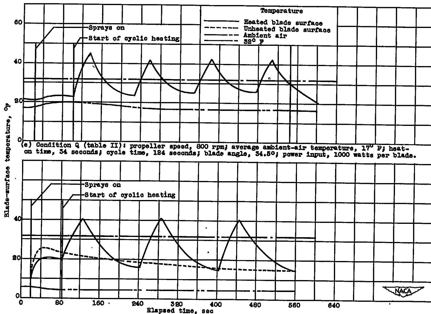
Figure 10. - Continued. Typical variation of leading edge blade-surface temperature with time during cyclic de-icing at 33-percent radius.
