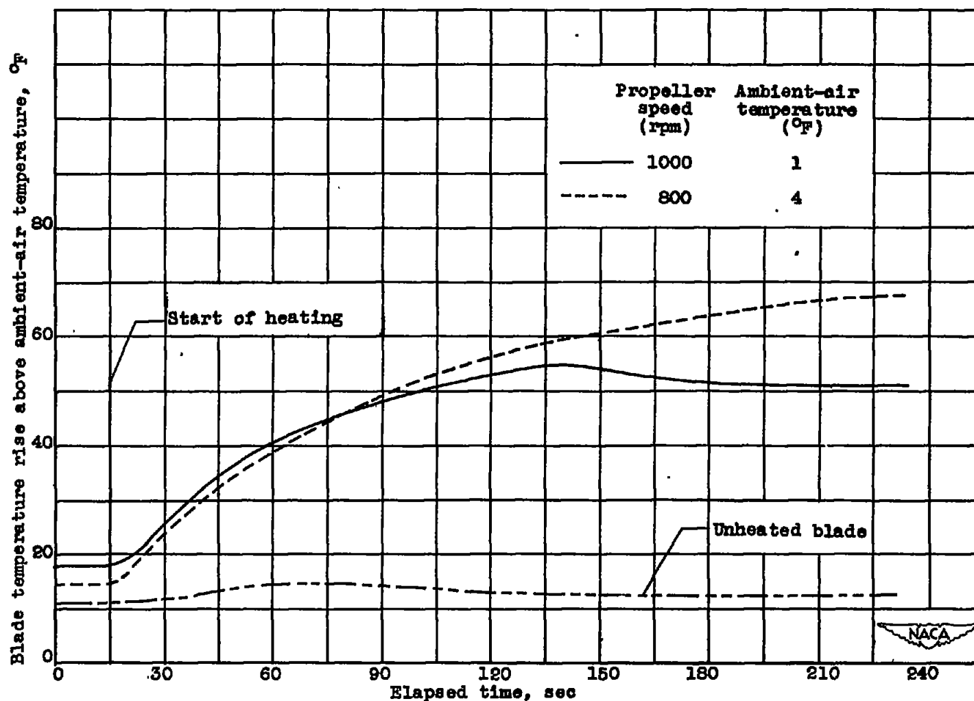
(a) Temperature rise of leading edge at 33-percent radius.
