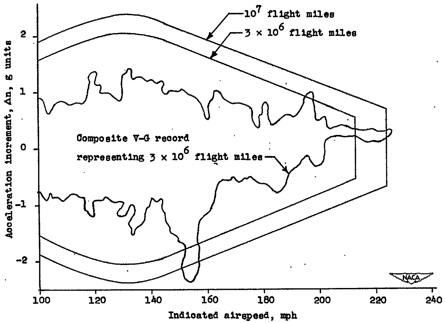
Figure 3.- Comparison of calculated flight envelopes with the composite V-G record for the prewar period.
