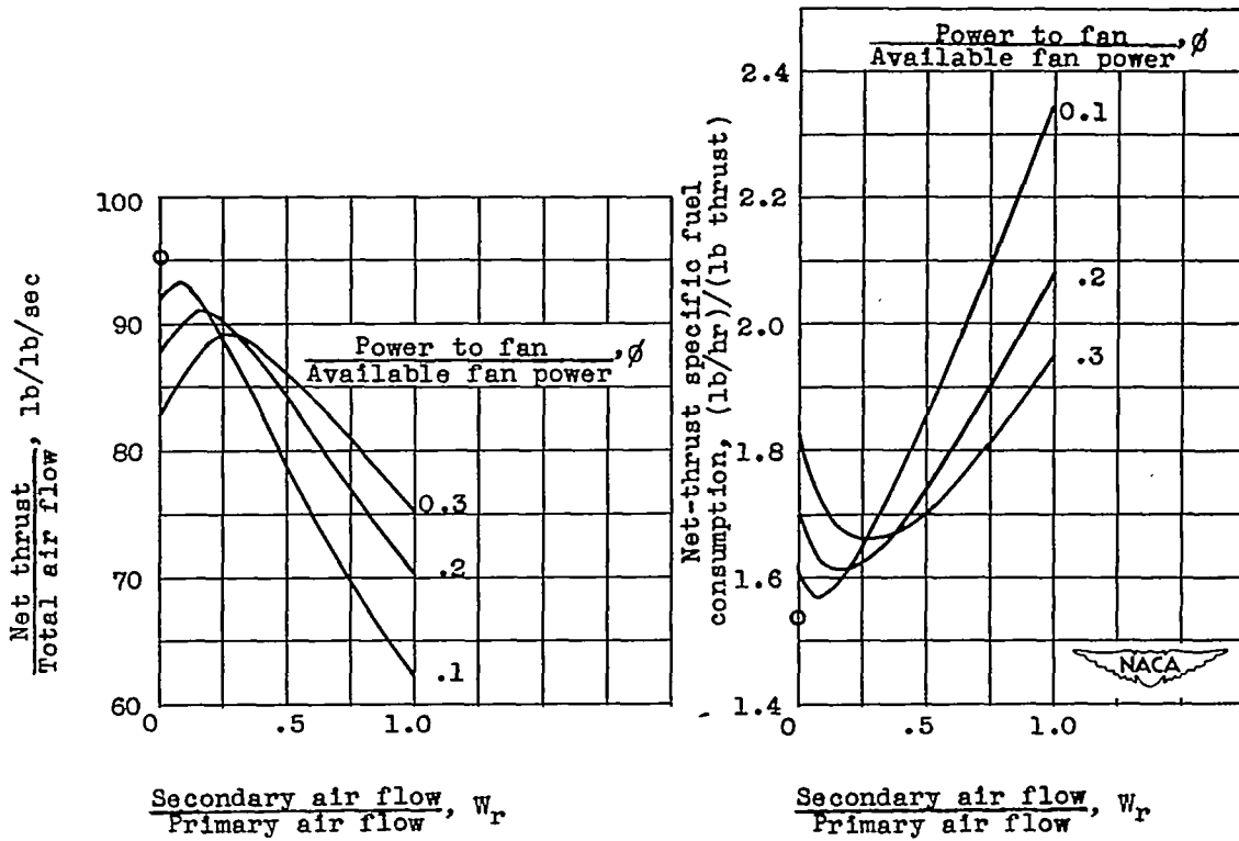
Figure 2. - Effect of varying ratio of secondary air flow to primary air flow and ratio of power to fan to available fan power with net thrust per pound of air and net-thrust specific fuel consumption for ducted-fan engines with auxiliary burning. Mach number, 0.3; altitude, 30,000 feet.
