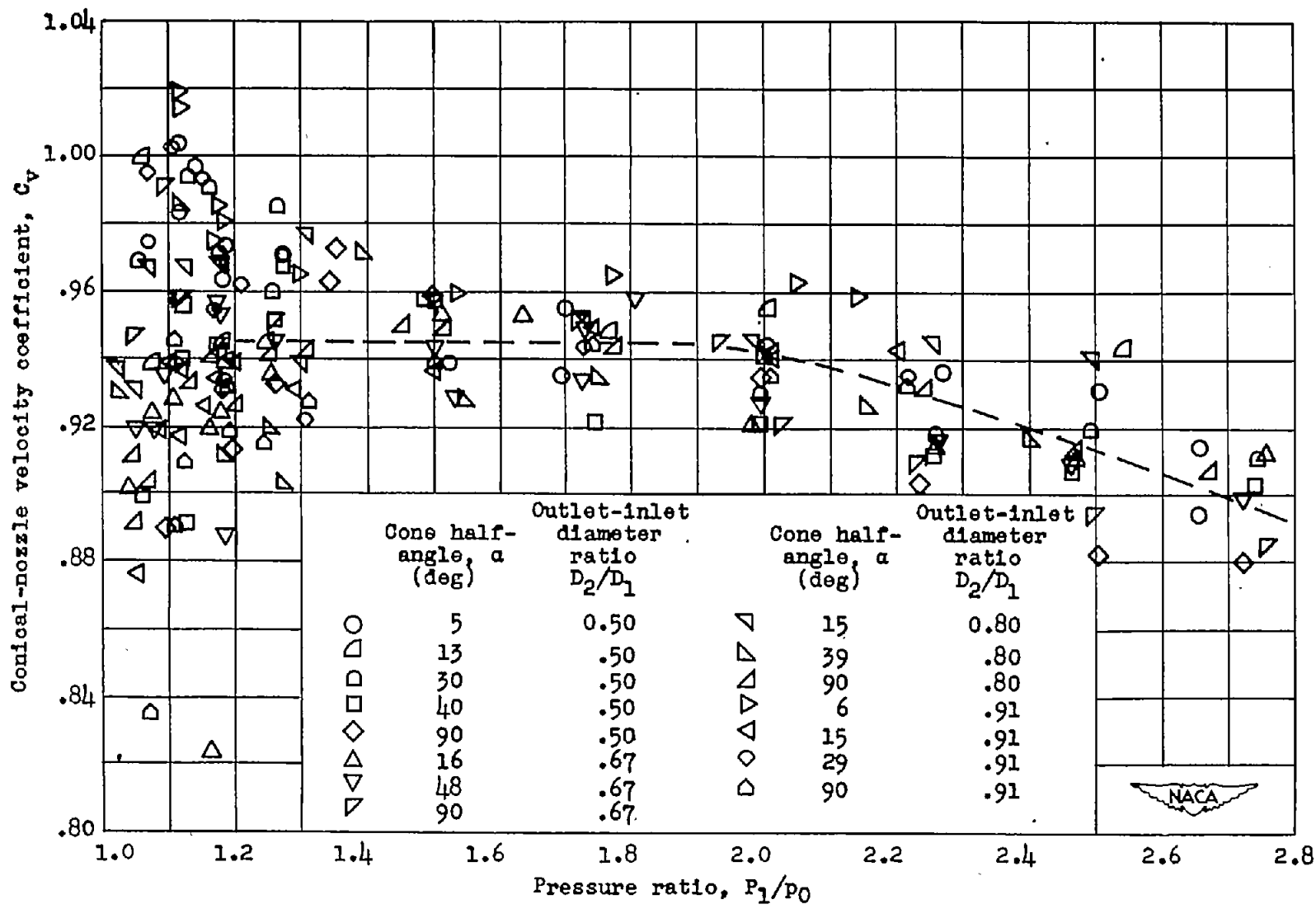
Figure 8.- Variation of conical-nozzle velocity coefficient with pressure ratio for various cone half-angles and outlet-inlet diameter ratios.
