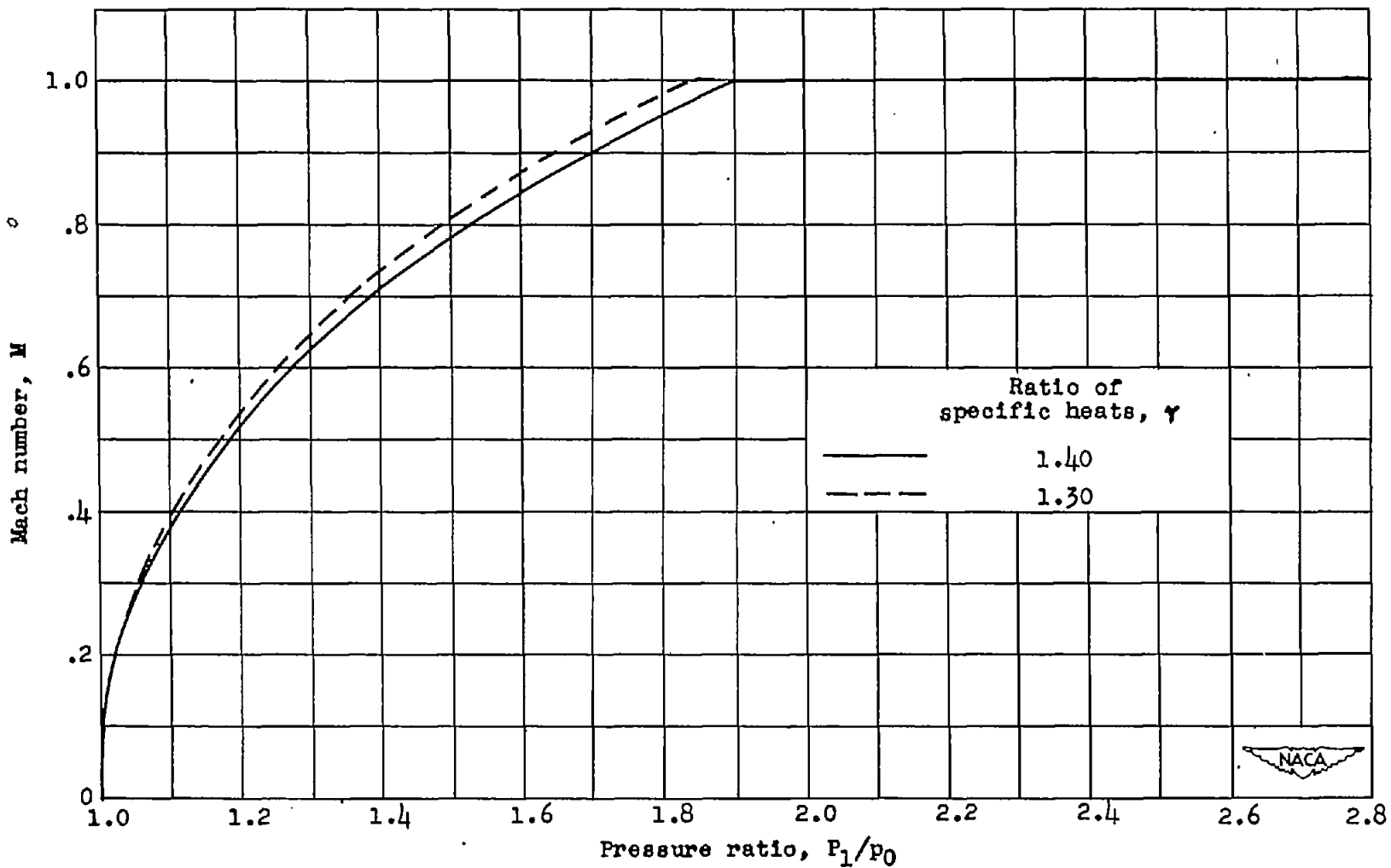
Figure 3. - Comparison of Mach number for two values of ratio of specific heats over range of pressure ratios. ( \gamma for model nozzles, approximately 1.40; \gamma for full-scale nozzles, 1.30 to 1.40.)
