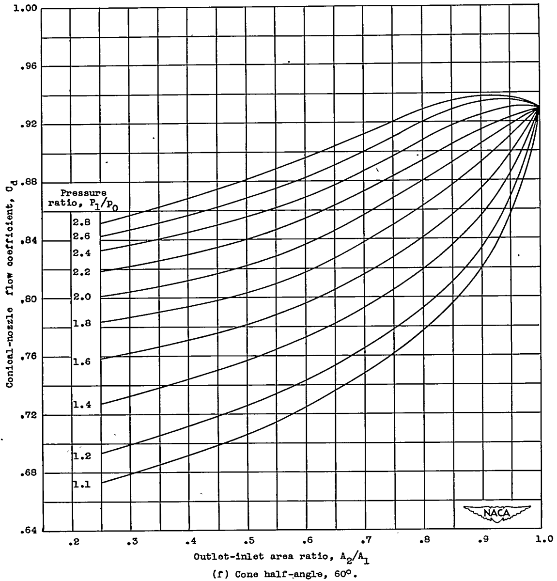
Figure 7.- Continued. Variation of conical-nozzle flow coefficient with outlet-inlet area ratio for various pressure ratios.
