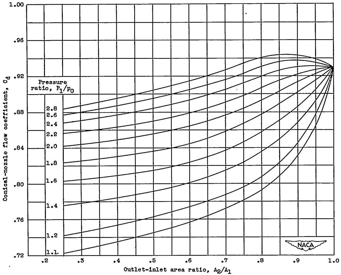
Figure 7.- Continued. Variation of conical-nozzle flow coefficient with outlet-inlet area ratio for various pressure ratios.
