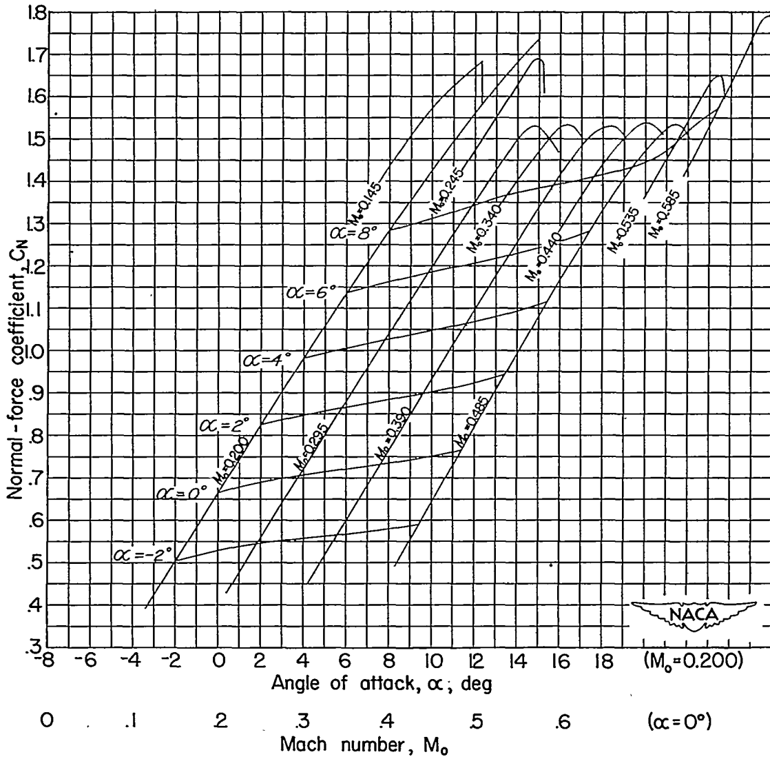
(b) Wing with partial-span flaps.
