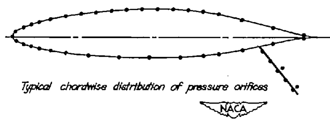
Figure 3.—Principal wing dimensions and locations of pressure orifices.
