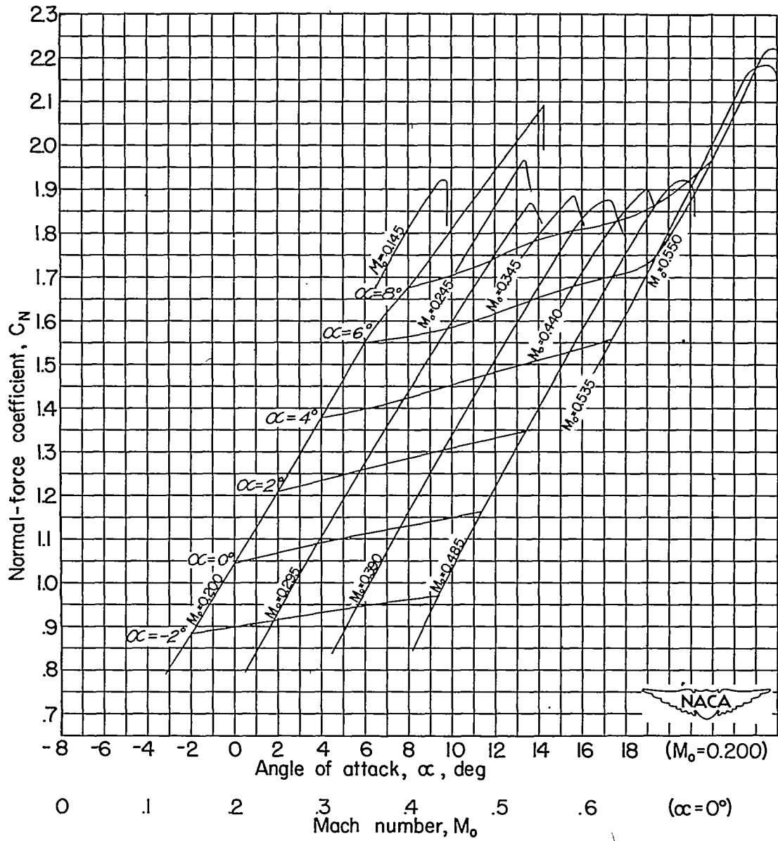
(c) Wing with full-span flaps.
