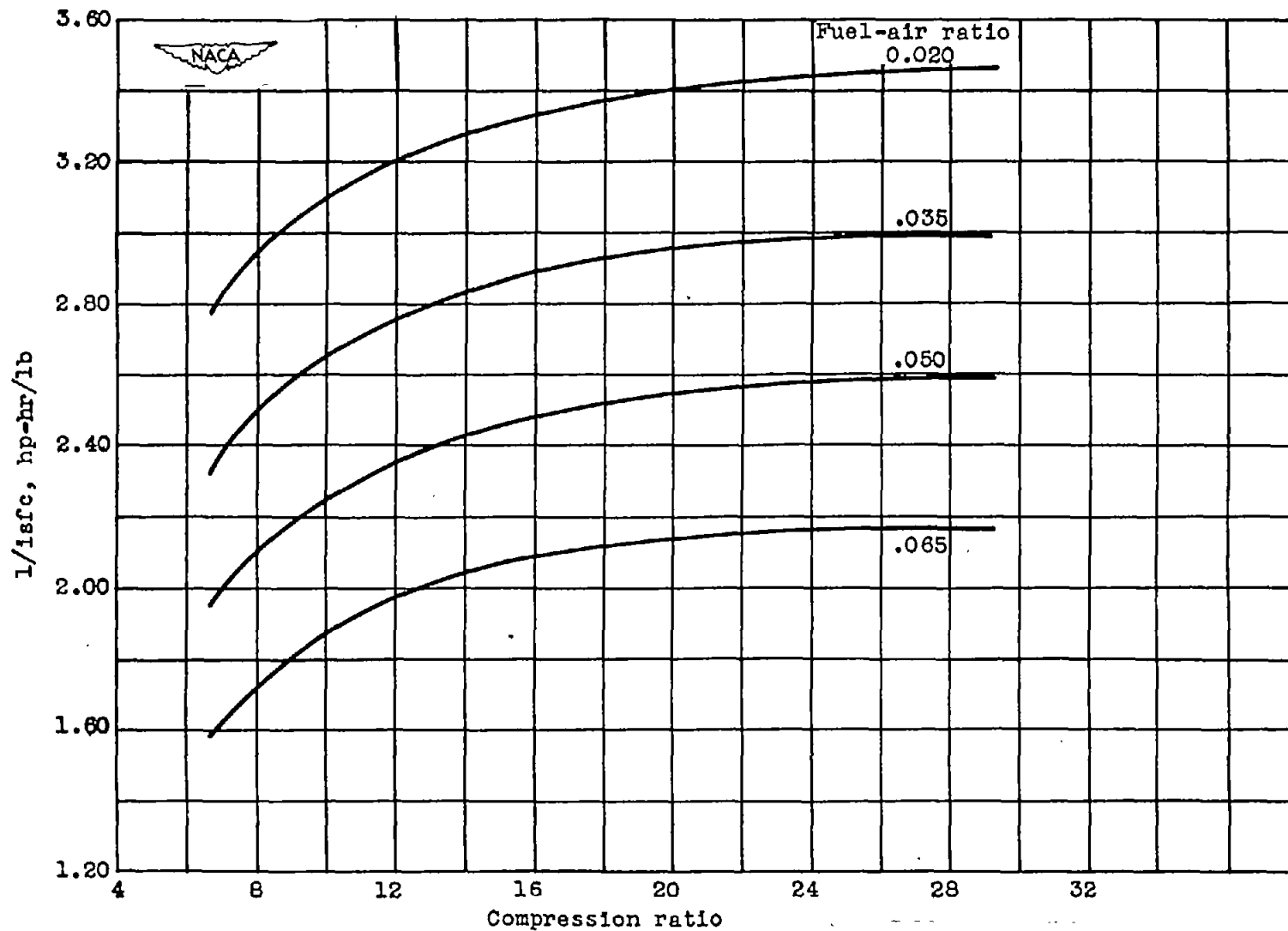
Figure 11. - Variation of indicated specific fuel consumption with compression ratio for various fuel-air ratios.
