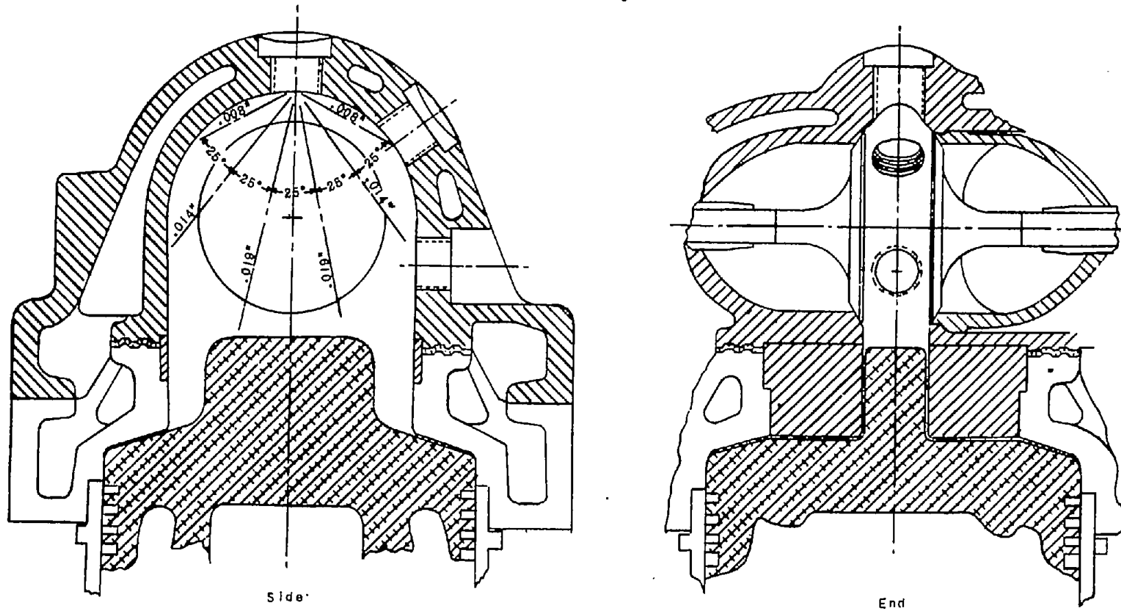
Figure 1. - Combustion chamber used in investigation of reference 3.
