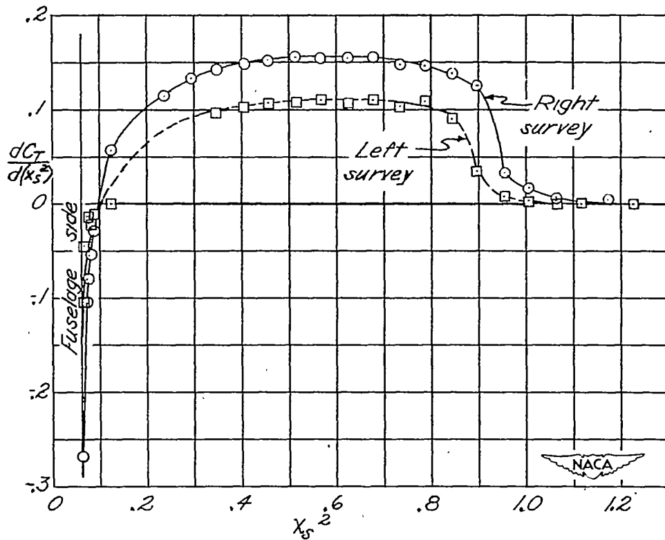
(a) Test conditions: \eta = 90.8 percent; J = 1.45 ; C_p = 0.147 ; C_T = 0.092 ; M = 0.301 ; M_t = 0.718 .
