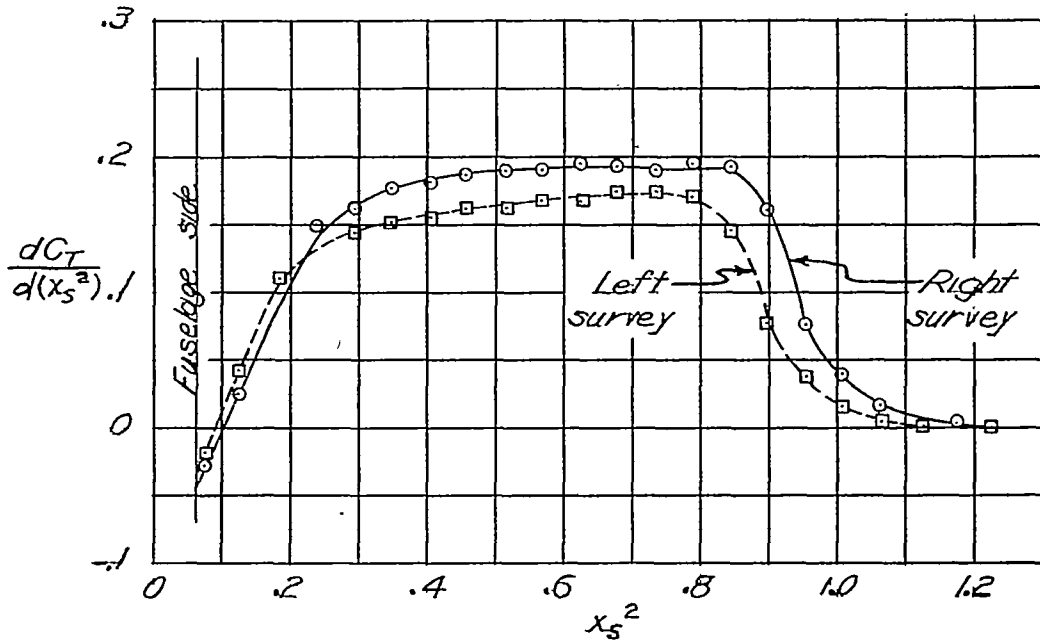
(a) Test conditions: \eta = 77.1 percent; J = 1.10 ; C_P = 0.188 ; C_T = 0.133 ; M = 0.249 ; M_t = 0.756 .
