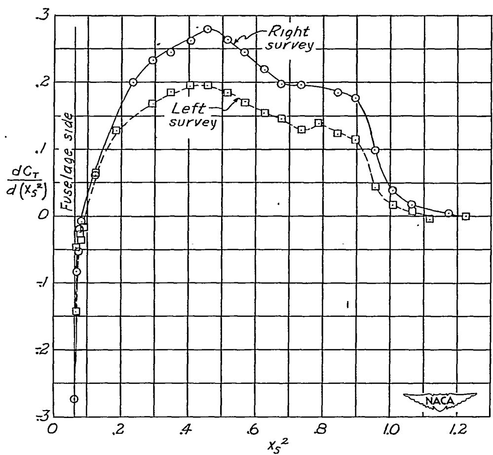
(a) Test conditions: \eta = 70.0 percent; J = 1.46 ; C_p = 0.315 ; C_T = 0.151 ; M = 0.304 ; M_t = 0.722 .
