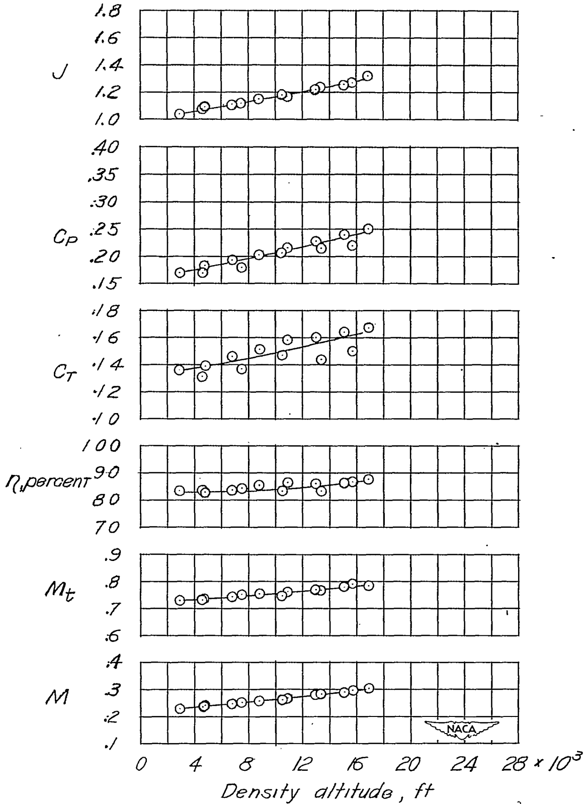
Figure 6.- Military-power climb at an indicated airspeed of 165 miles per hour with three-blade propeller on a fighter-type airplane.
