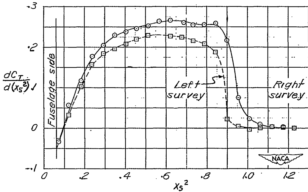
(d) Test conditions: \eta = 87.6 percent; J = 1.32 ; C_p = 0.251 ; C_T = 0.167 ; M = 0.303 ; M_t = 0.784 .
