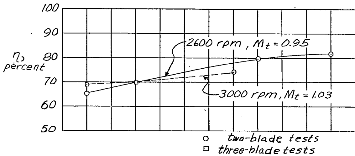
(a) Propeller as tested, with shank loss.
