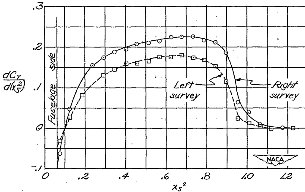
(d) Test conditions: \eta = 84.2 percent; J = 1.41 ; C_P = 0.233 ; C_T = 0.139 ; M = 0.334 ; M_t = 0.815 .
