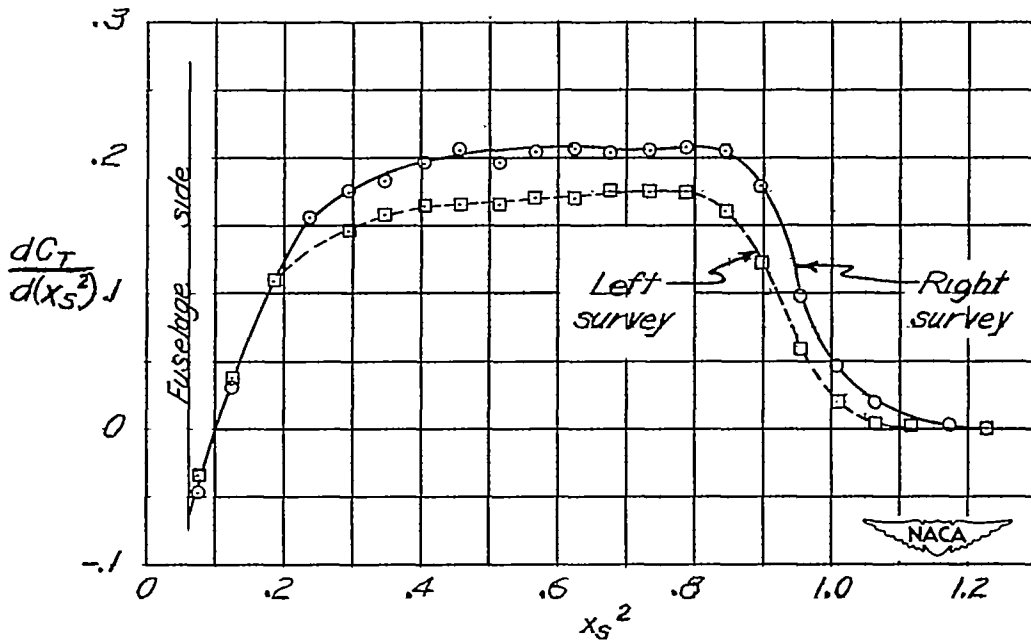
(b) Test conditions: \eta = 77.5 percent; J = 1.22 ; C_P = 0.220 ; C_T = 0.140 ; M = 0.280 ; M_t = 0.774 .
