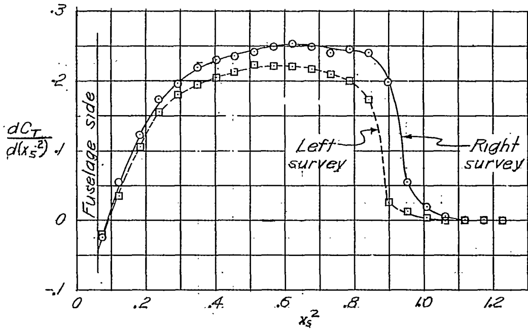
(c) Test conditions: \eta = 86.0 percent; J = 1.22 ; C_p = 0.228 ; C_T = 0.160 ; M = 0.280 ; M_t = 0.770 .
