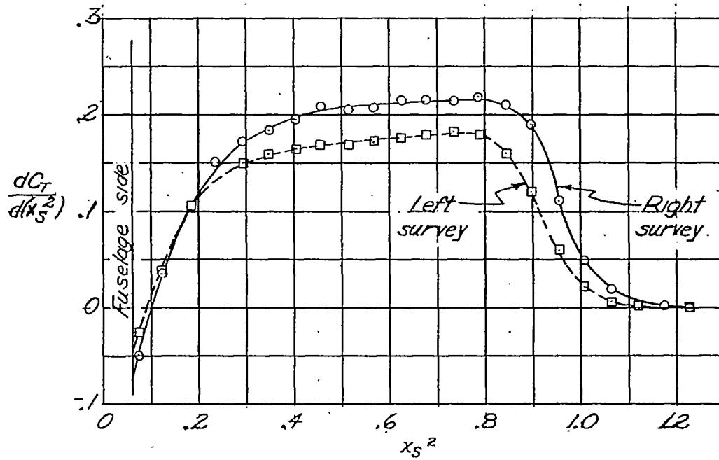
(c) Test conditions: \eta = 80.2 percent; J = 1.30 ; C_P = 0.231 ; C_T = 0.143 ; M = 0.300 ; M_t = 0.785 .
