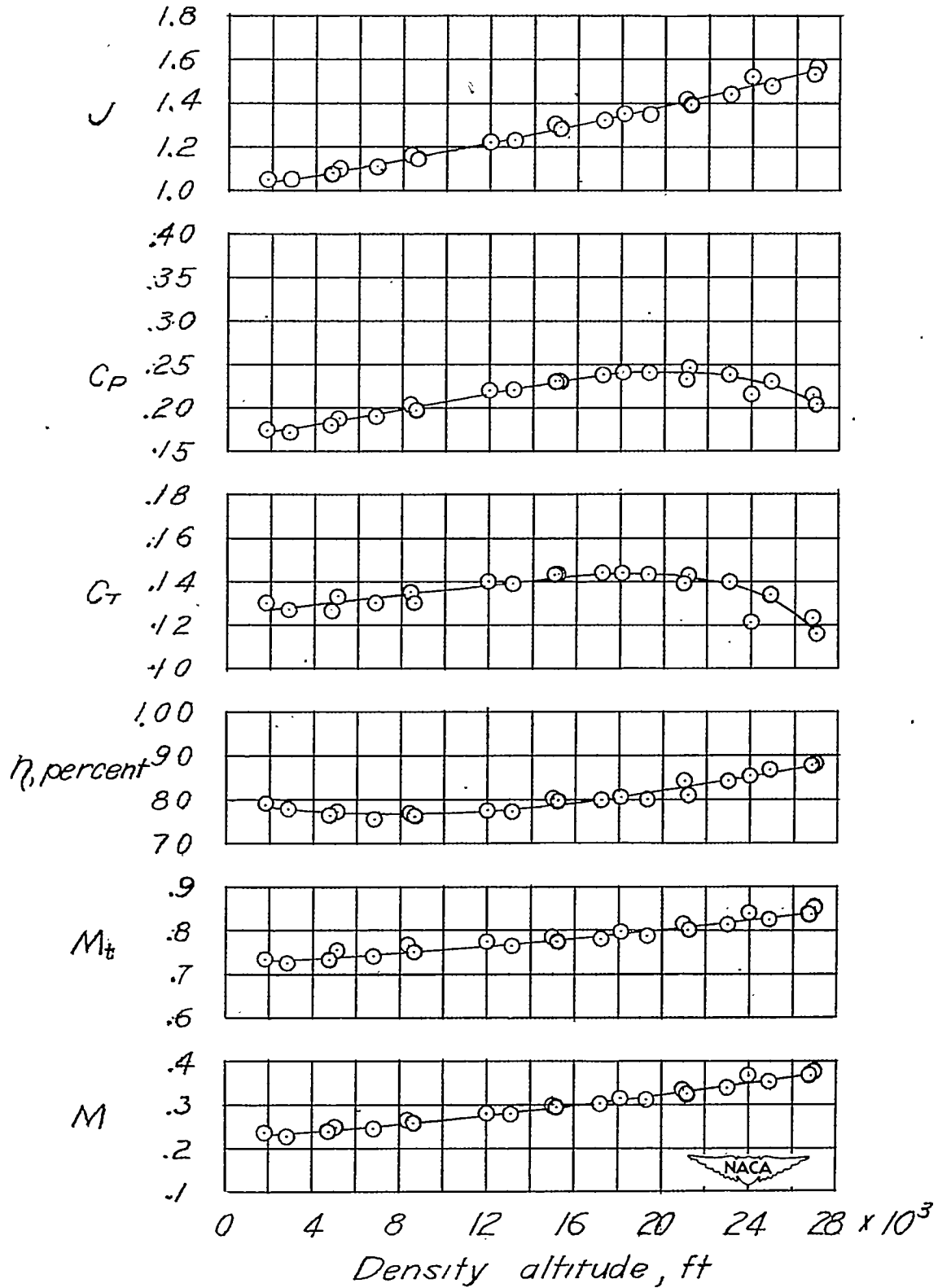
Figure 7.- Military-power climb at an indicated airspeed of 165 miles per hour with two-blade propeller on a fighter-type airplane.
