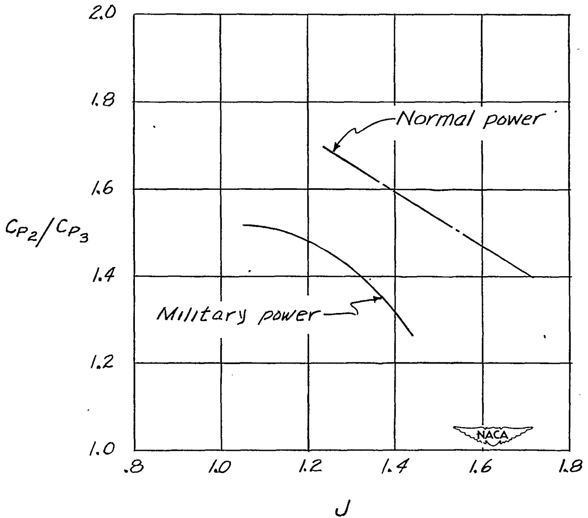
Figure 8.- Ratio of power coefficient per blade for two-blade operation to three-blade operation for various advance ratios in climbs.
