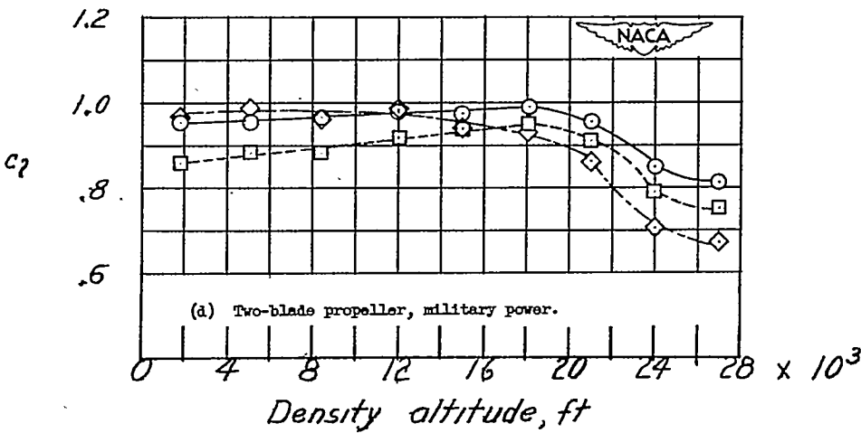
Figure 9.- Variation of c_2 of tested propeller with altitude in climbs.
