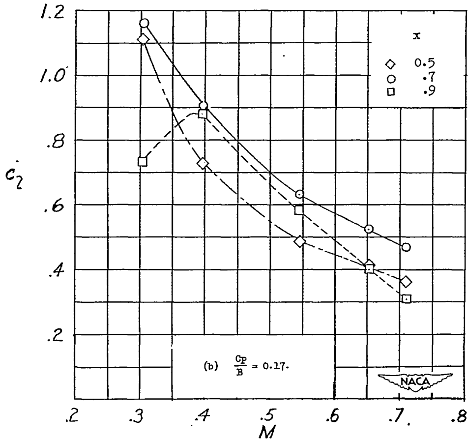
Figure 16.- Variation of c_2 of propeller tested with Mach number at high speeds. Engine speed, 2600 rpm.
