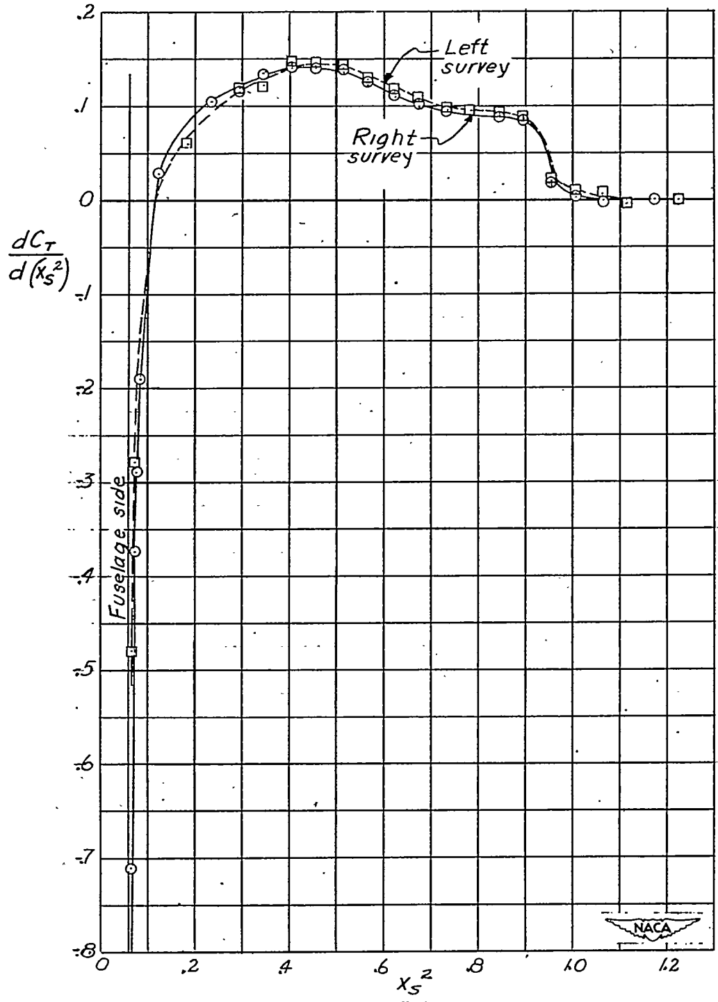
(e) Test Conditions: \eta = 81.5 percent; J = 3.42 ; C_p = 0.331 ; C_T = 0.079 ; M = 0.708 ; M_t = 0.961 .
