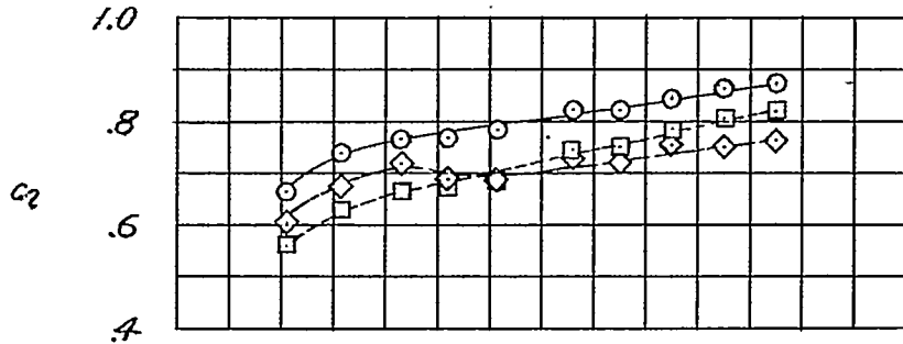
(a) Three-blade propeller, normal rated power.
