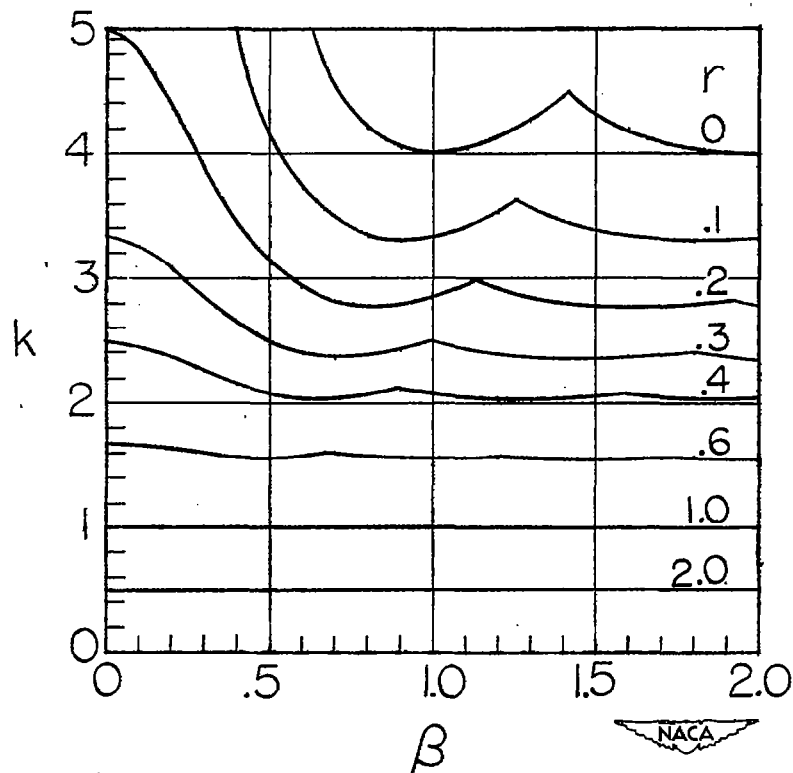
Figure 2.— Compressive-buckling coefficients for Metalite type sandwich plates stressed in the elastic range.
