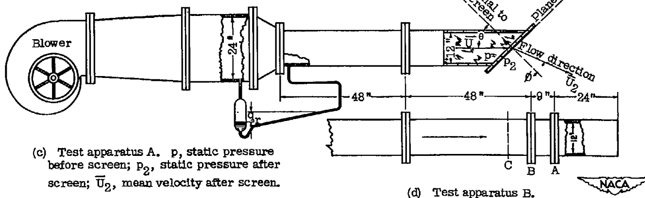
Figure 2.- Apparatus used in determining coefficients of screens and damping of spatial variations in speed.
