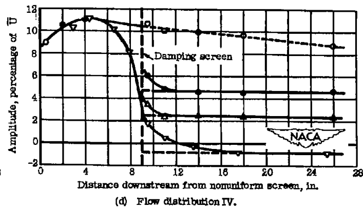
Figure 15.- Amplitude of spatial variations in speed as a function of distance along duct center line.
