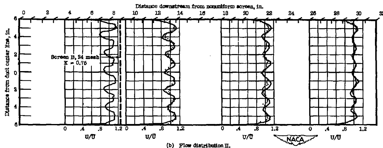
Figure 14.- Sample flow distributions used in determining effect of screens on variations in mean speed. Solid curves for screen absent; plotted points for screen present. All measurements made at \bar{U} = 25 feet per second.
