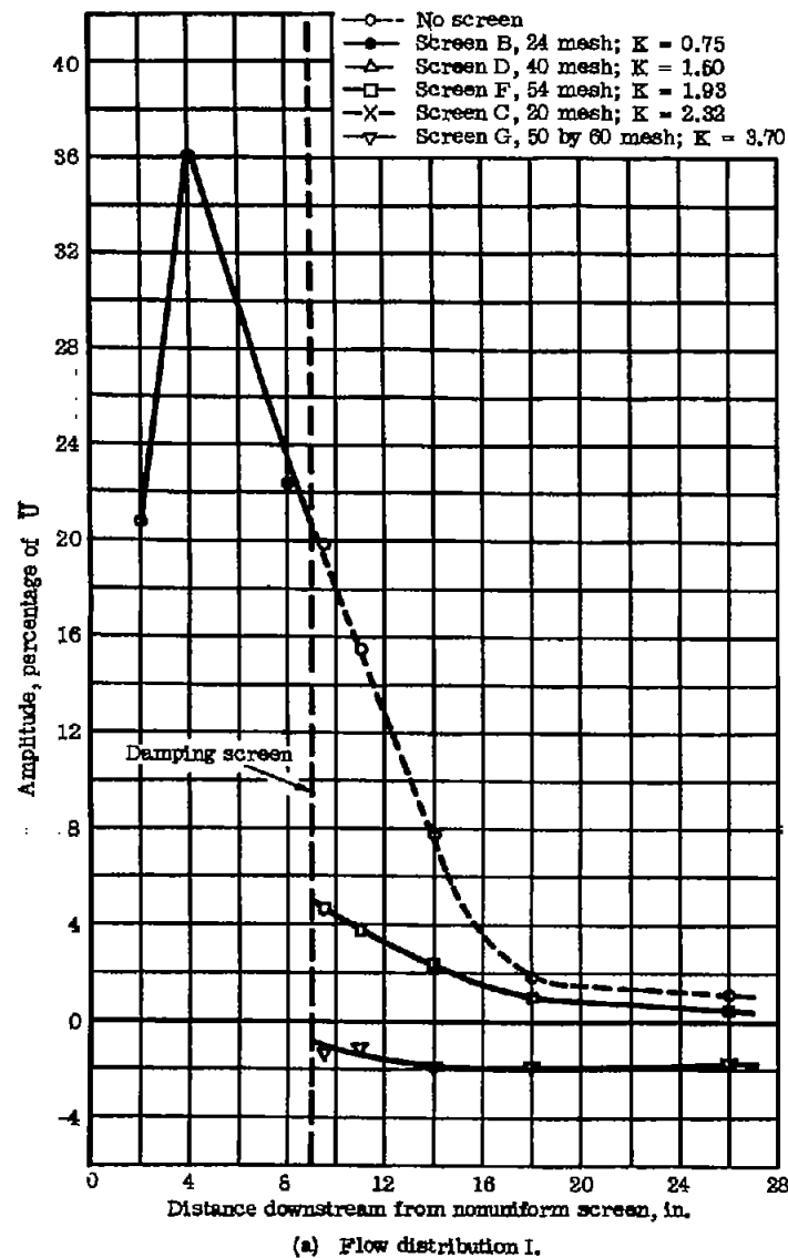
Figure 15.- Amplitude of spatial variations in speed as a function of distance along duct center line.
