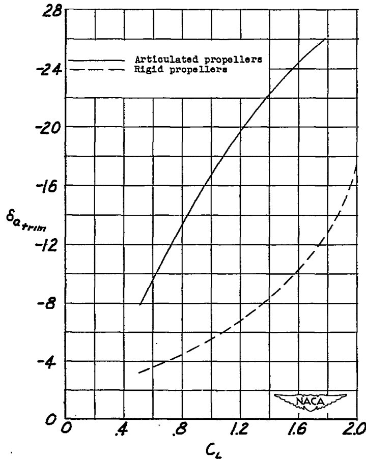
Figure 8.— Effect of propeller articulation on the variation of ailerator deflection required for trim with lift coefficient for simulated full-power operation. \delta_f = 0^\circ .
