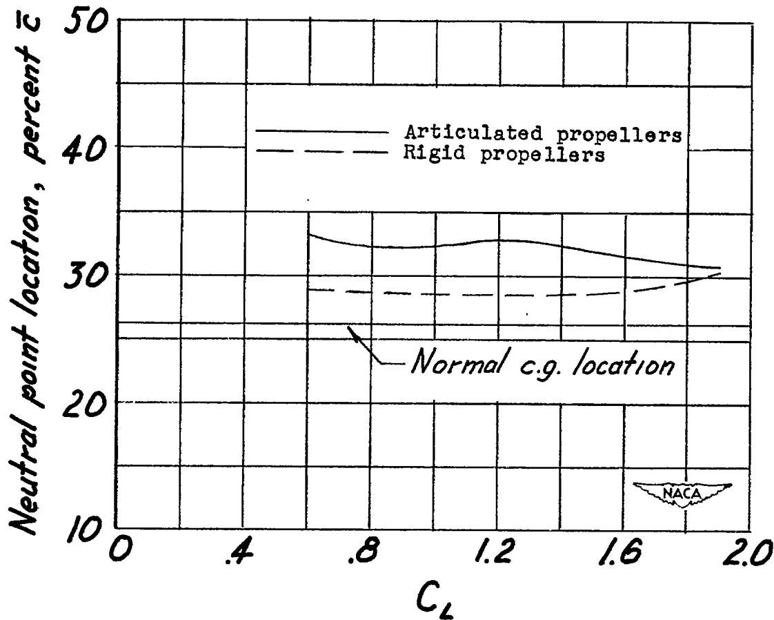
Figure 6.- Effect of propeller articulation on the stick-fixed longitudinal stability of the model for simulated full-power operation. \delta_P = 0^\circ .
