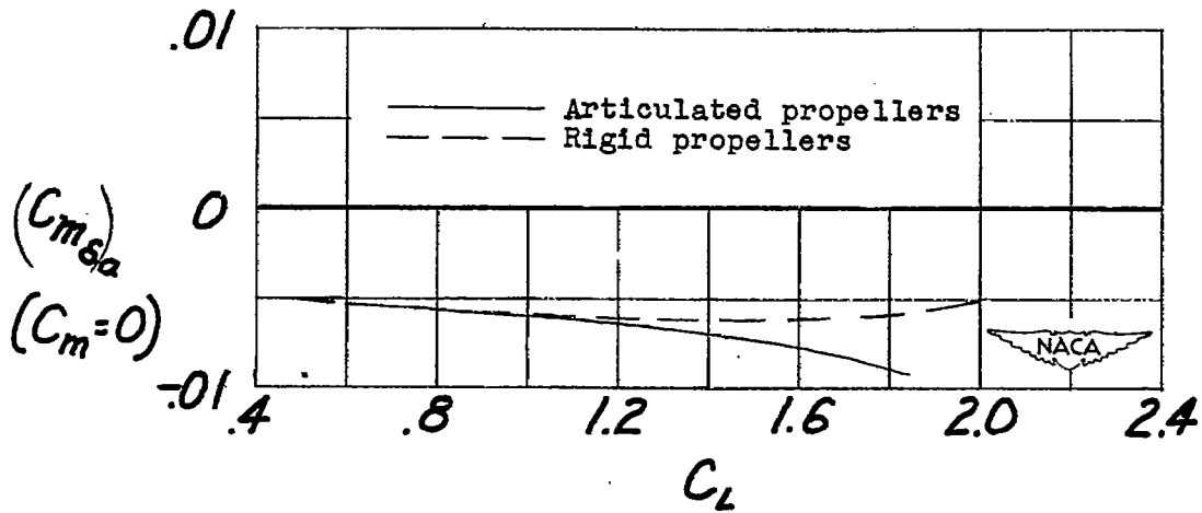
Figure 14.- Effect of propeller articulation on the variation of (C_{m\delta})_a with C_L for simulated full-power operation. \delta_P = 0^\circ .
