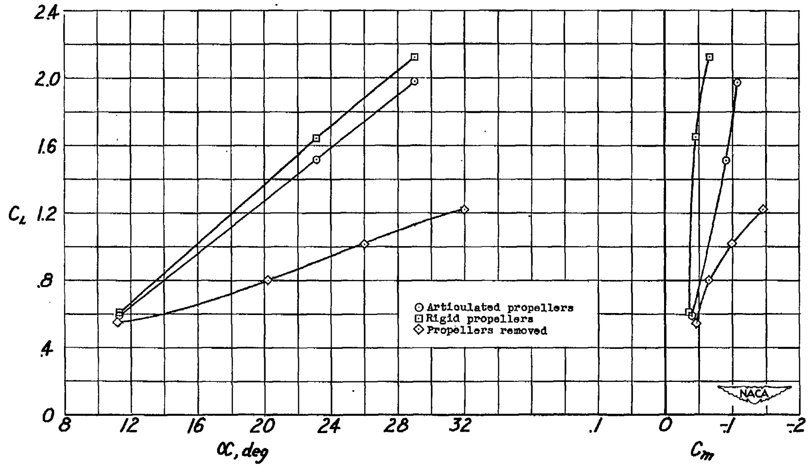
Figure 17.- Effect of full-power operation on the variation of \alpha and C_m with C_L for the model with the all-movable horizontal tail installed. \delta_P = 0^\circ .
