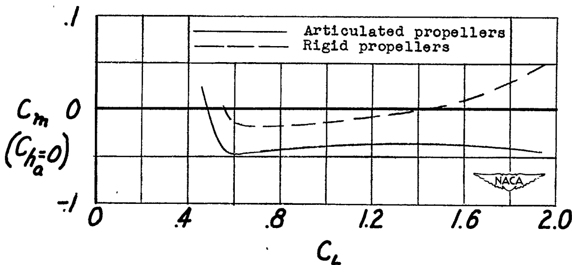
Figure 7.- Effect of propeller articulation on the variation of C_m with C_L for simulated full-power operation. \delta_P = 0^\circ .
