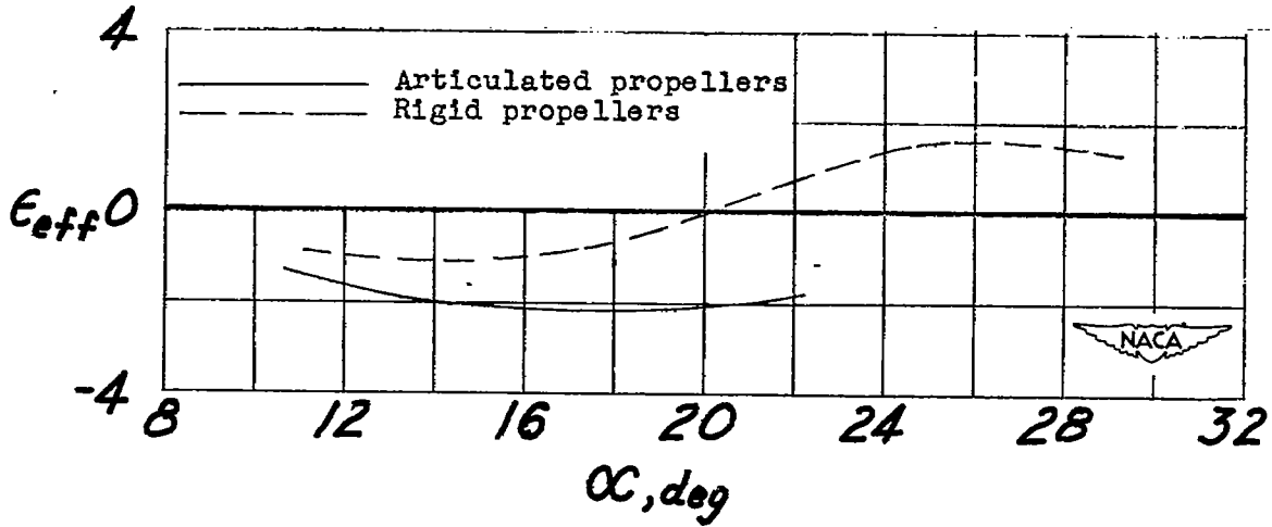
Figure 13.- Effect of propeller articulation on the variation of \epsilon_{eff} with \alpha for simulated full-power operation. \delta_P = 0^\circ .
