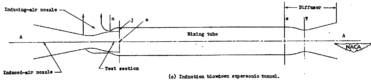
Figure 1.- Schematic drawings of the induction blowdown supersonic tunnel and a direct-discharge blowdown supersonic tunnel.
