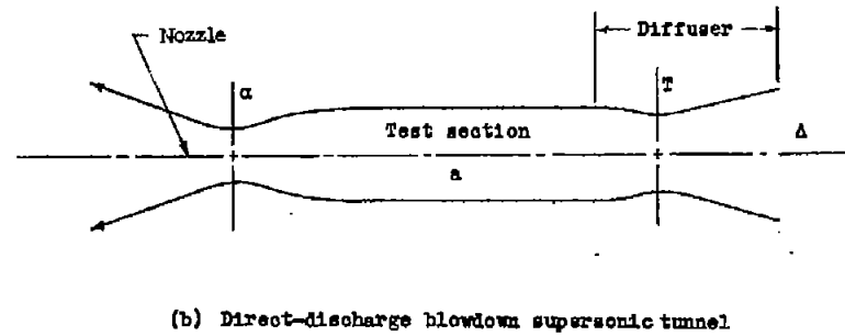
(b) Direct-discharge blowdown supersonic tunnel.
