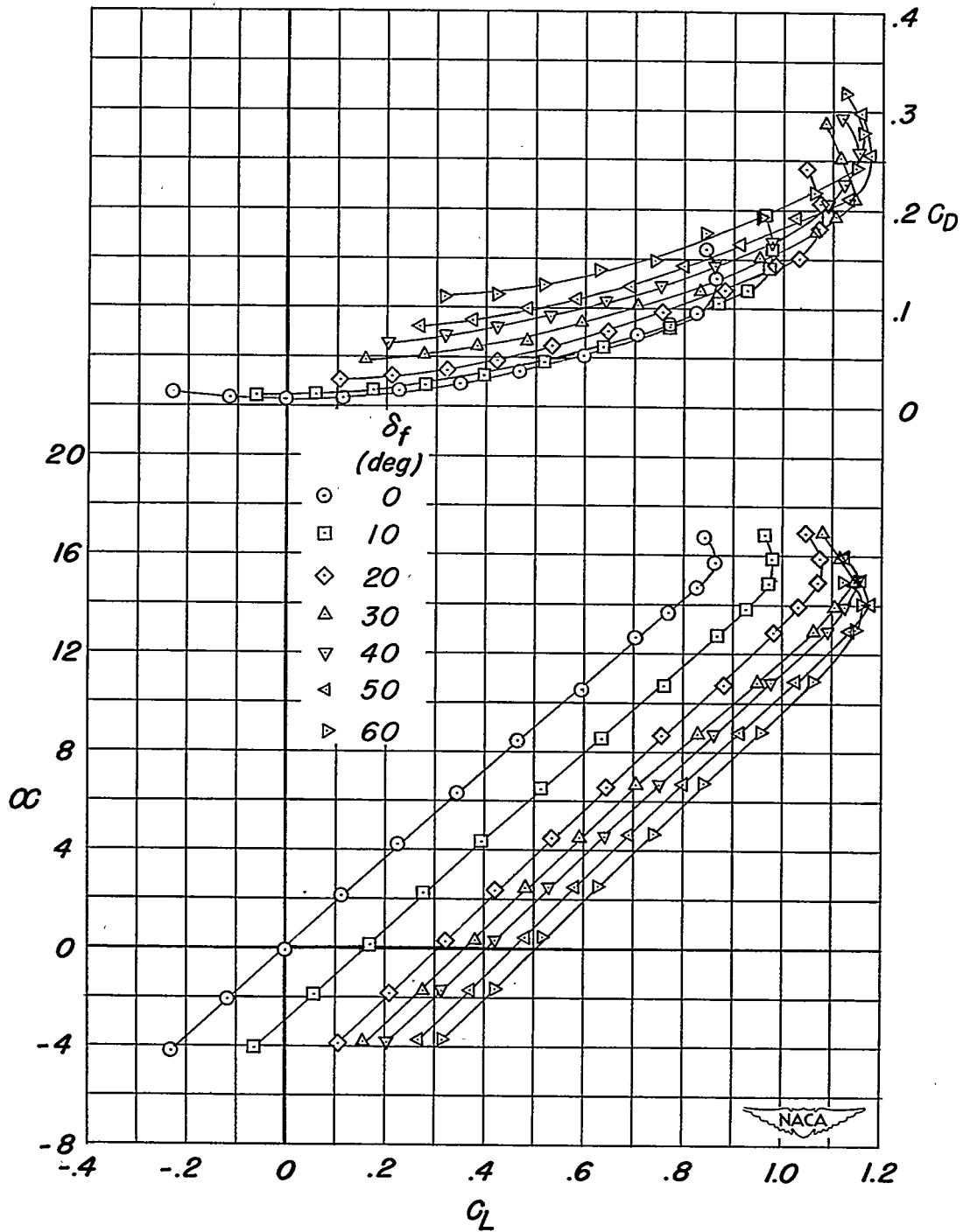
Figure 3.- Effect of flap deflection on the aerodynamic characteristics in pitch of the unswept wing of aspect ratio 3.13 equipped with inboard half-span flaps ( b_f = 0.484 \frac{b}{2} ). y_{f_i} = 0 ; y_{f_o} = 0.484 \frac{b}{2} .
