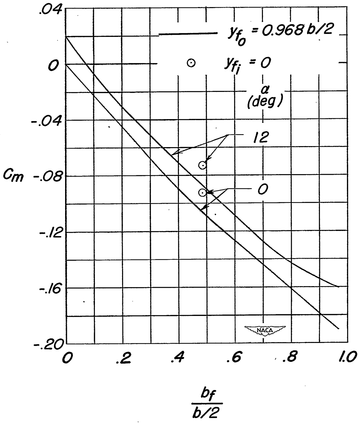
Figure 10.- Effects of flap span and spanwise location on the pitching-moment coefficient of the unswept wing of aspect ratio 3.13. \delta_f = 30^\circ .
