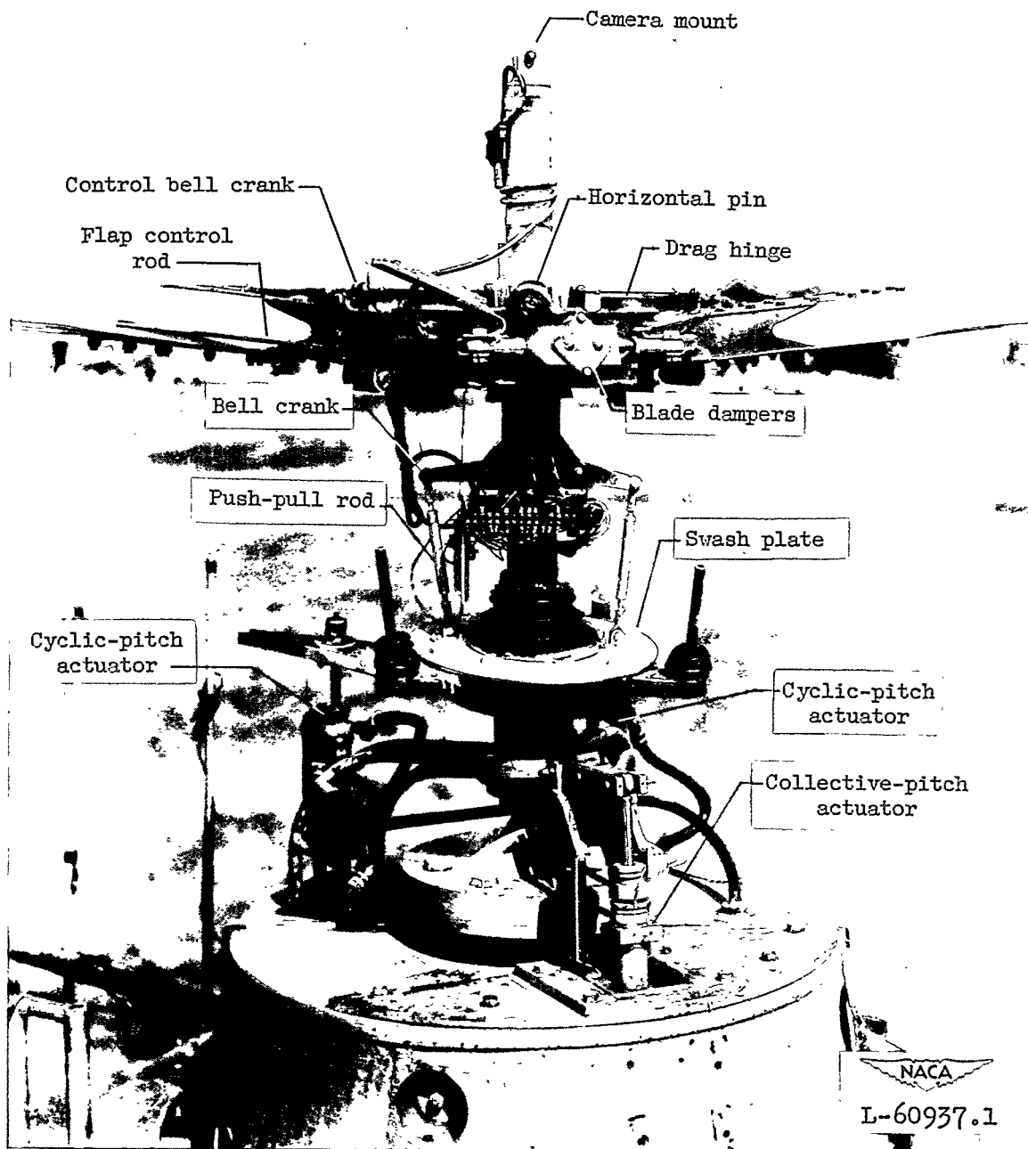
Figure 2.- Details of rotor-hub installation on the Langley helicopter tower.
