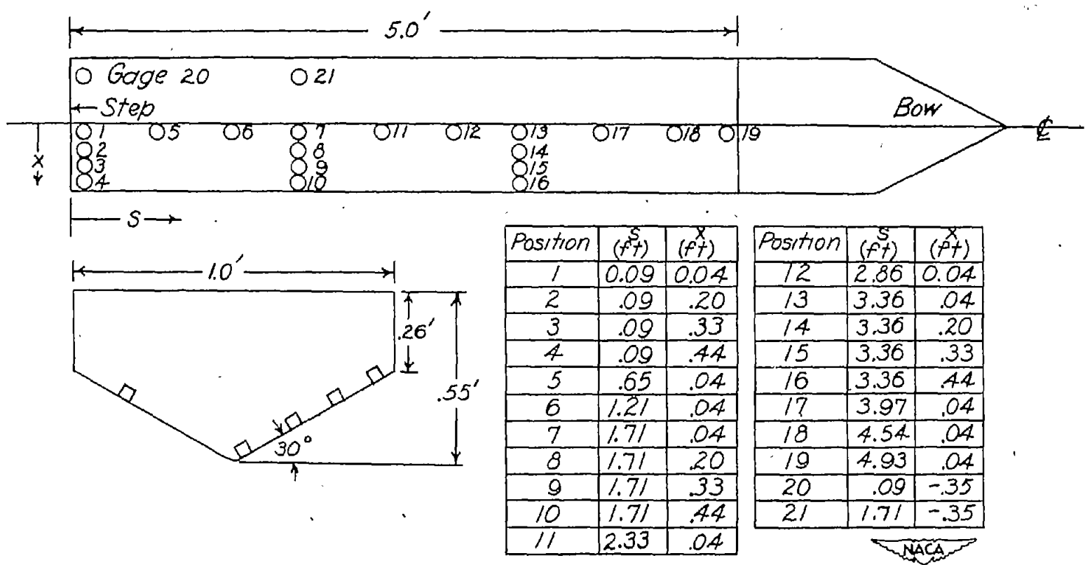
Figure 1.- Hull lines and pressure-gage positions on the model.
