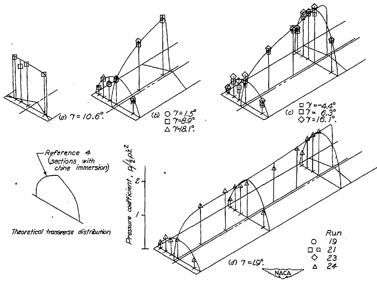
Figure 9.- Variation of instantaneous pressure coefficient \frac{p}{\frac{1}{2} \rho V^2} at successive stages of immersion for 45^\circ trim.
