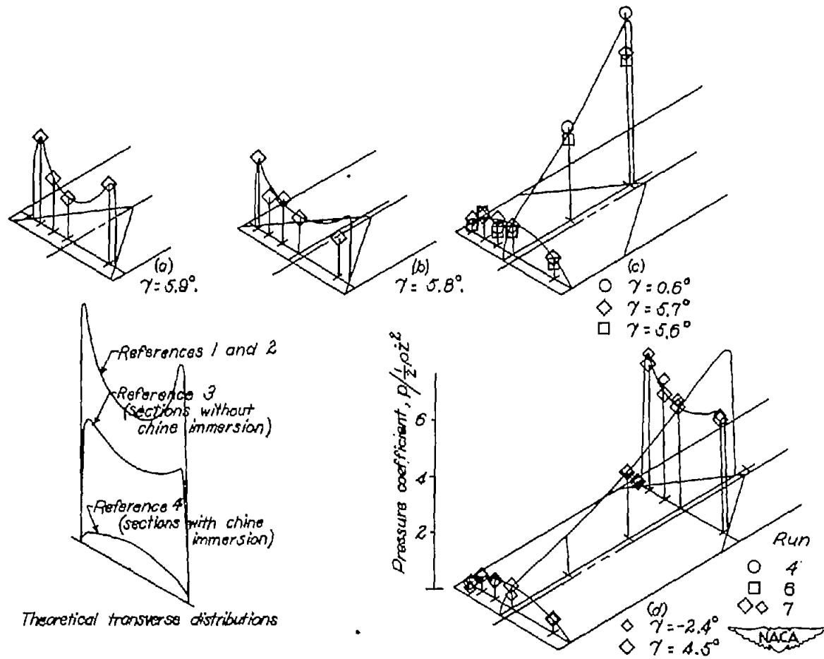
Figure 7.- Variation of instantaneous pressure coefficient \frac{p}{\frac{1}{2}\rho V^2} at successive stages of immersion for 15° trim.
