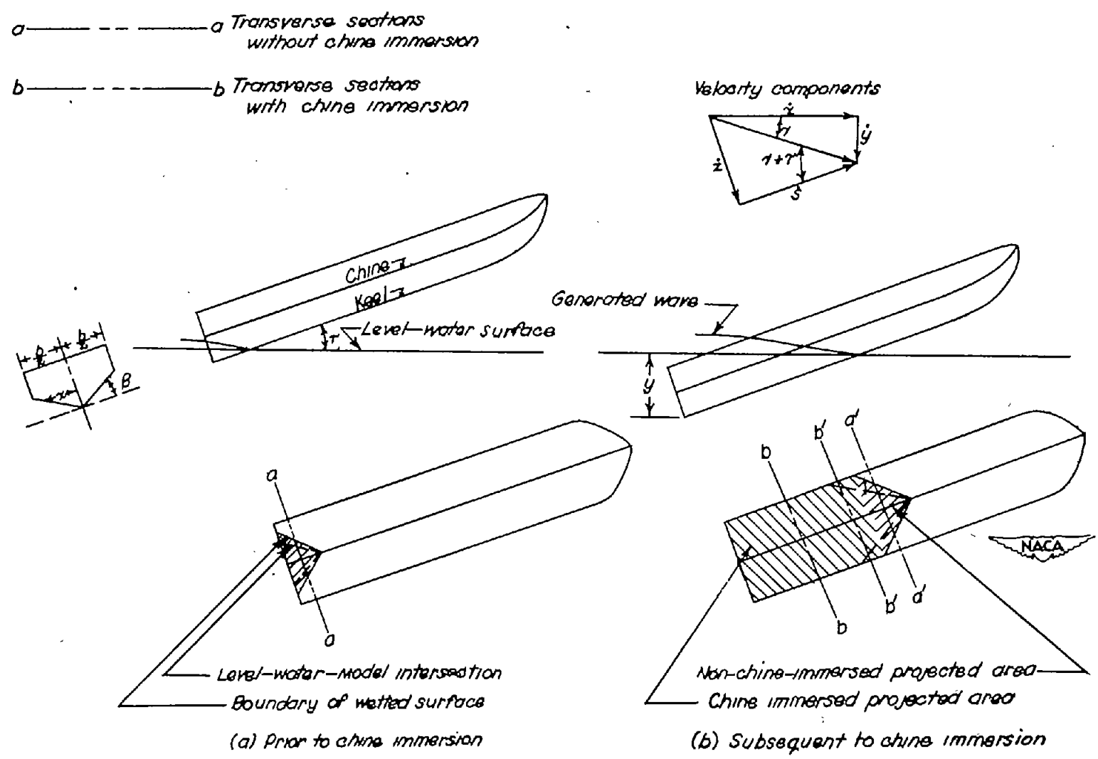
Figure 10.- Schematic diagram of landing.
