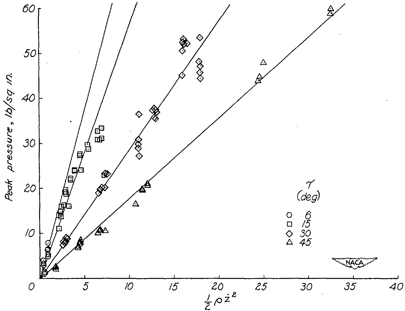
Figure 11.- Variation of peak pressure with \frac{1}{2} \rho z^2 for various trims.
