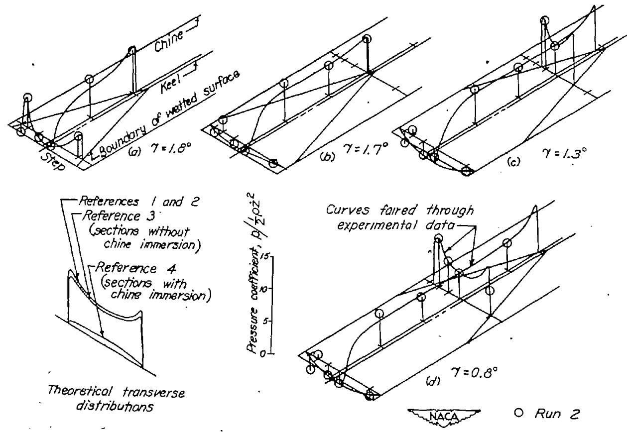
Figure 6.- Variation of instantaneous pressure coefficient \frac{p}{\frac{1}{2} \rho V^2} at successive stages of immersion for 6^\circ trim.
