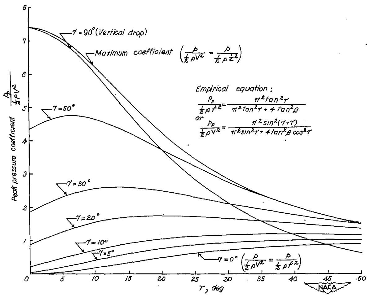
Figure 13.- Variation of peak pressure coefficient \frac{C_p}{\frac{1}{2} \rho V^2} with trim for various flight-path angles.
