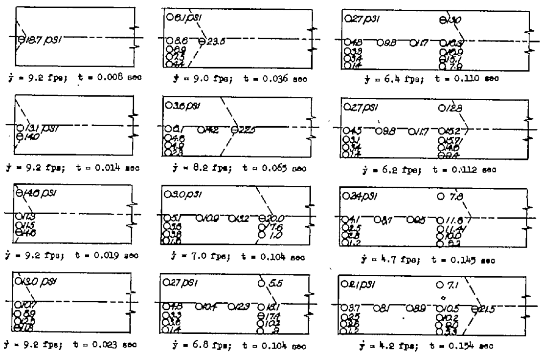
(c) Run 15: \tau = 30^\circ ; \dot{x}_0 = 51.6 feet per second; \dot{y}_0 = 9.3 feet per second. Figure 4.- Continued.
