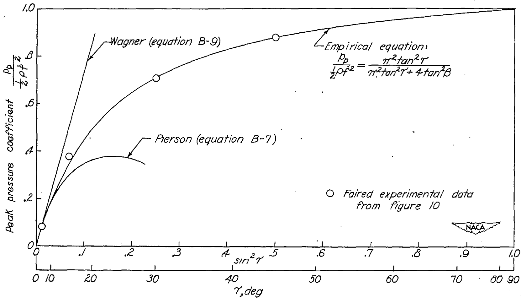
Figure 12.- Variation of peak pressure coefficient \frac{P_p}{\frac{1}{2}\rho V^2} with trim.
