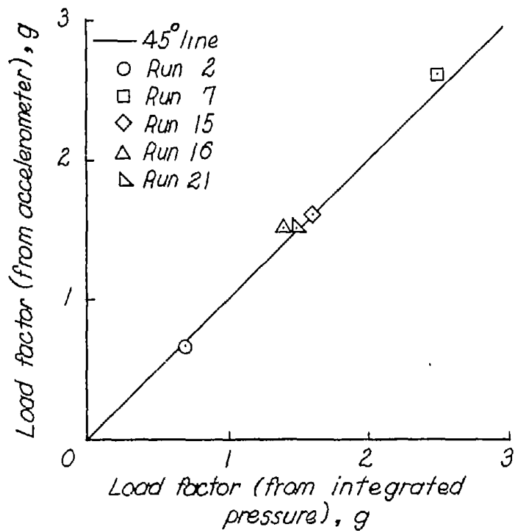
(a) Maximum vertical load factor.
