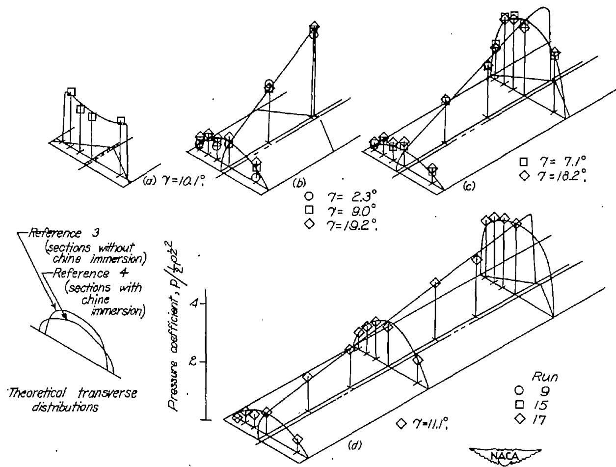
Figure 8.- Variation of instantaneous pressure coefficient \frac{P}{\frac{1}{2}\rho V^2} at successive stages of immersion for 30^\circ trim.
