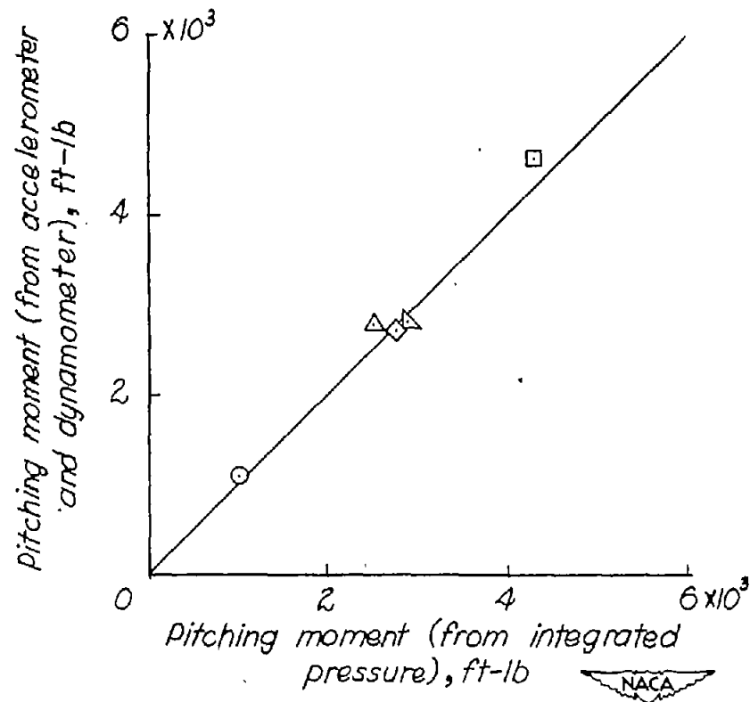
(b) Pitching moment about step at time of maximum load.
