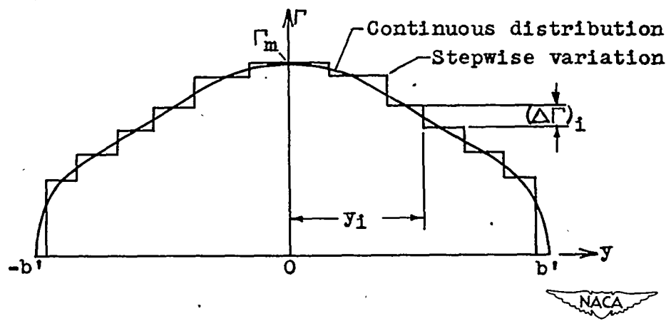
(b) Spanwise distribution of circulation.
