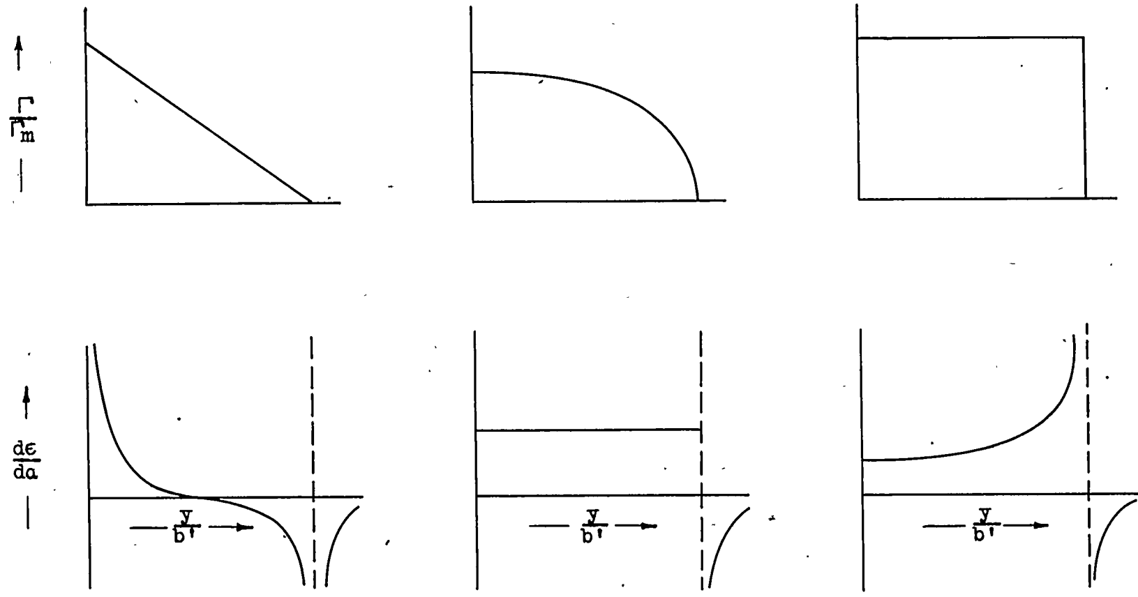
(a) Triangular loading. (b) Elliptical loading. (c) Uniform loading.
