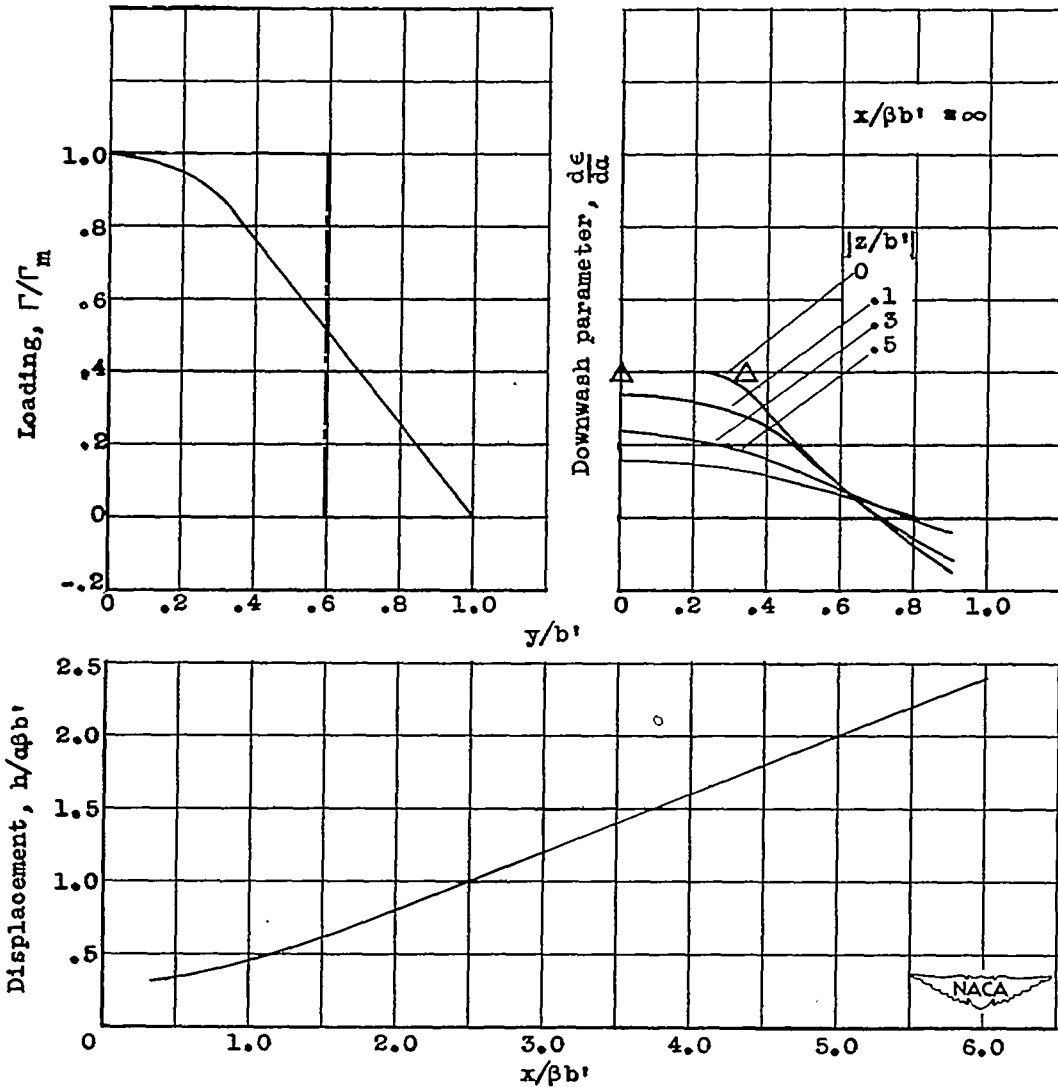
(a) Plan form, load distribution, downwash in Trefftz plane, and vortex-sheet displacement.
