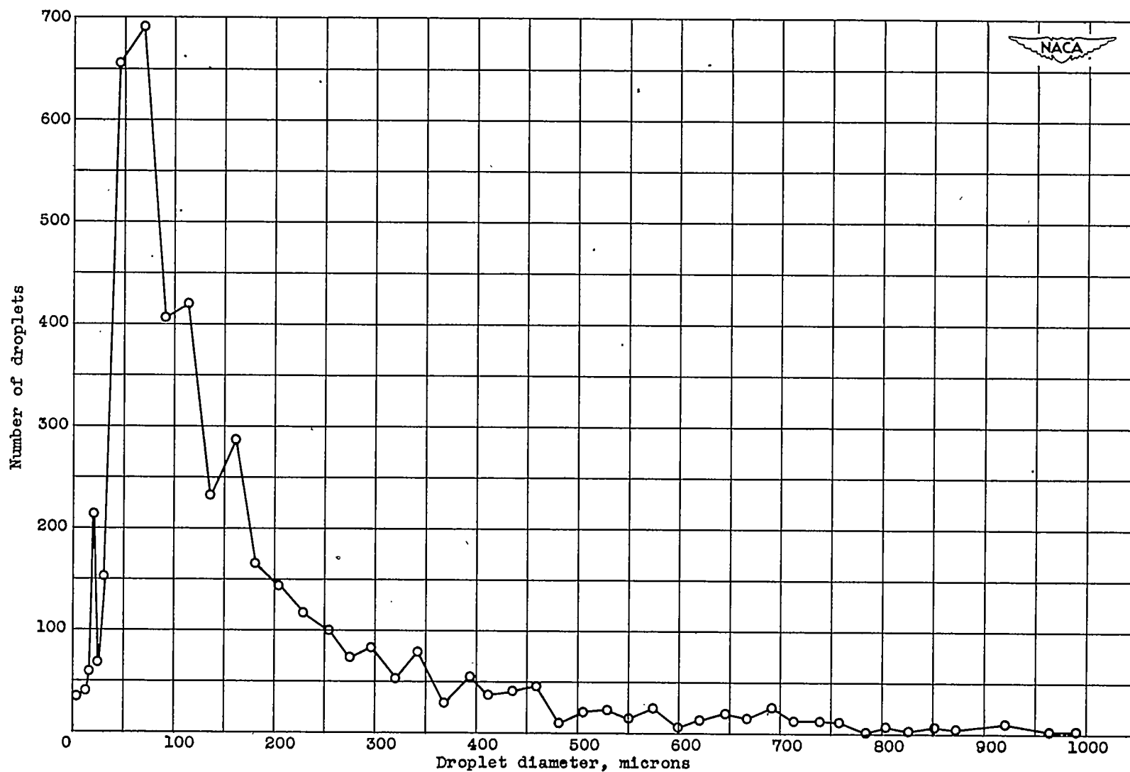
Figure 6. - Distribution of droplet sizes obtained in range of 8.75 to 1000 microns.
