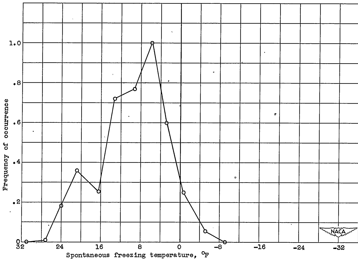
Figure 9. - Distribution of spontaneous freezing temperatures for 3- to 4-millilitre samples of water. (Data from reference 7.)
