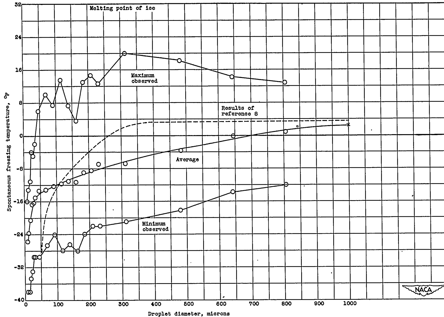
Figure 10. - Variation of spontaneous freezing temperature with droplet size for droplets supported by platinum surface.
