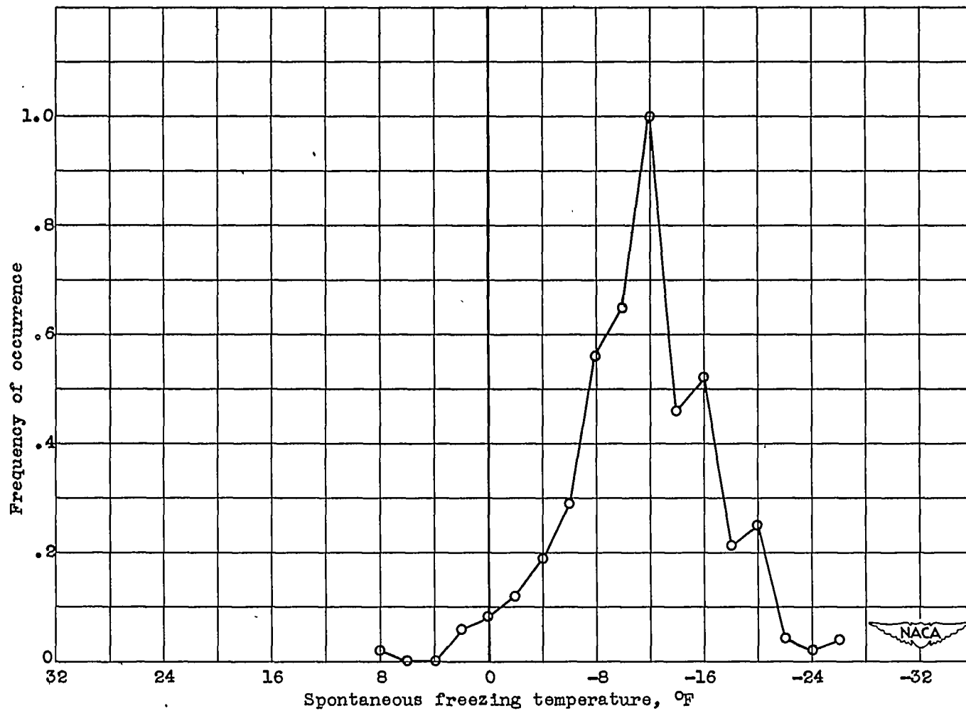
(j) Droplet diameter, 138.0 \pm 11.5 microns; droplets observed, 234; average spontaneous freezing temperature, -11.1^\circ\text{F} ; standard deviation, 5.22^\circ\text{F} .
