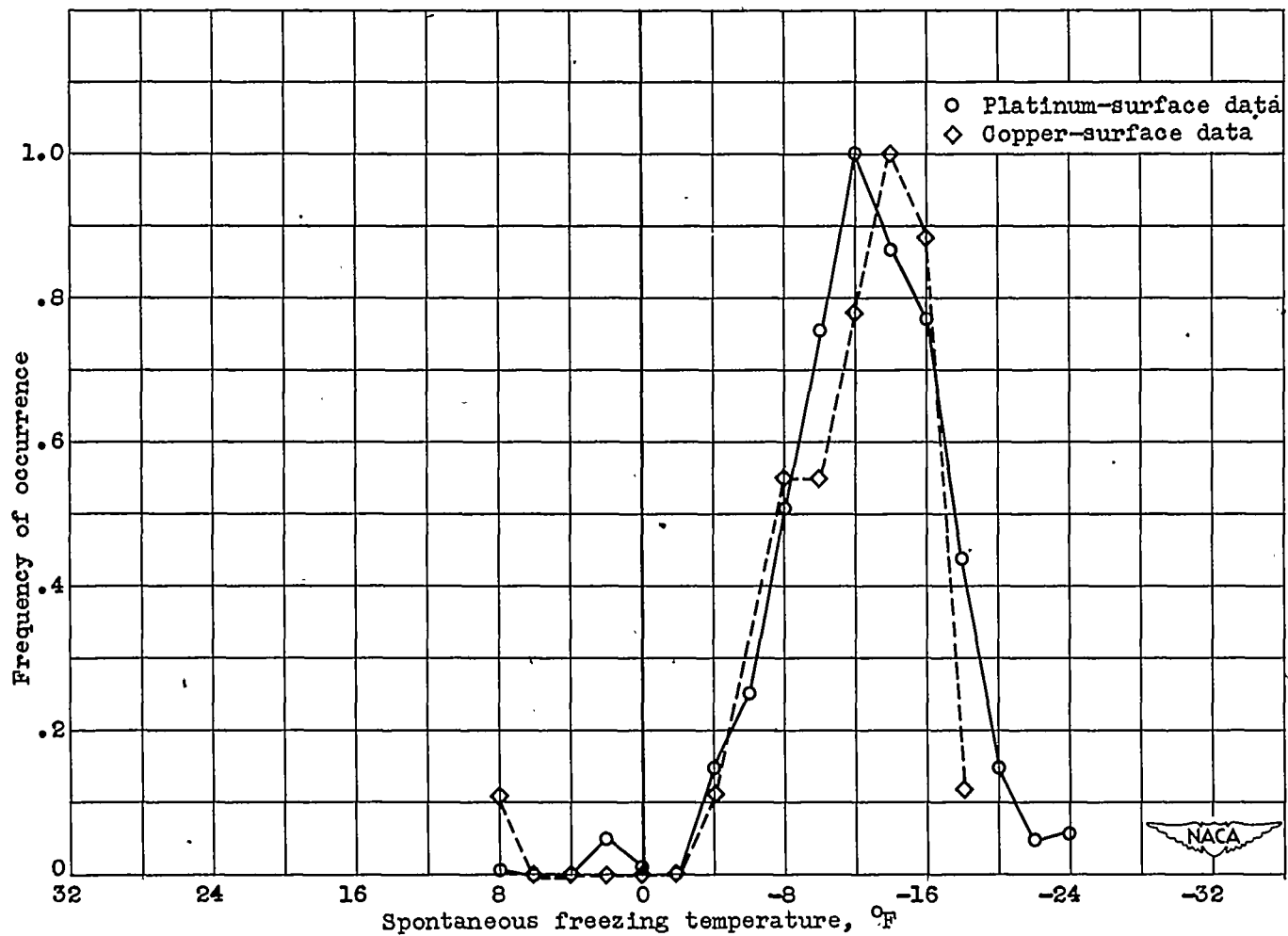
(h) Droplet diameter, 92.0 \pm 11.5 microns; droplets observed, on platinum 405, on copper 39; average spontaneous freezing temperature, platinum -12.1^\circ\text{F} , copper -11.6^\circ\text{F} ; standard deviation for platinum data, 4.48^\circ\text{F} .
