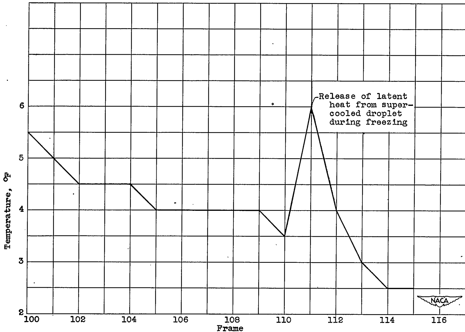
Figure 4. - Copy of chart from surface-thermocouple temperature recorder illustrating rise in temperature due to release of latent heat of fusion.
