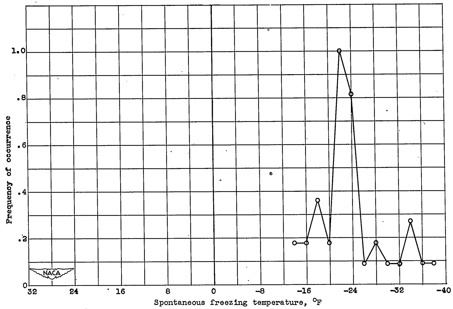
(b) Droplet diameter, 13.75 \pm 2.5 microns; droplets observed, 40; average spontaneous freezing temperature, -23.8^\circ\text{F} ; standard deviation, 5.75^\circ\text{F} .
