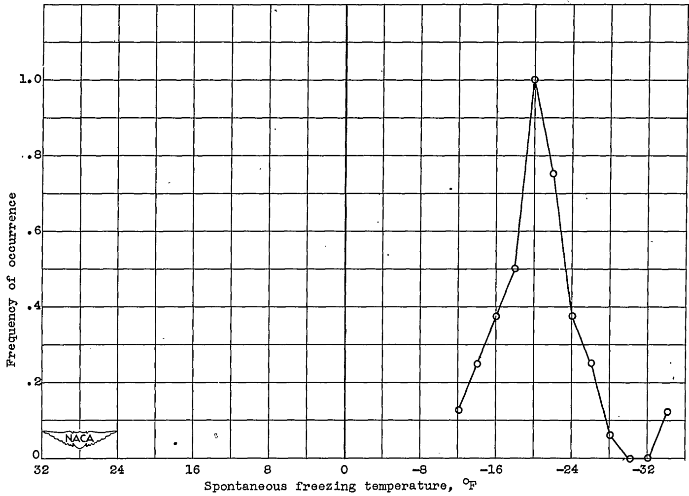
(c) Droplet diameter, 18.75 \pm 2.5 microns; droplets observed, 61; average spontaneous freezing temperature, -20.5^{\circ} F; standard deviation, 4.31^{\circ} F.
