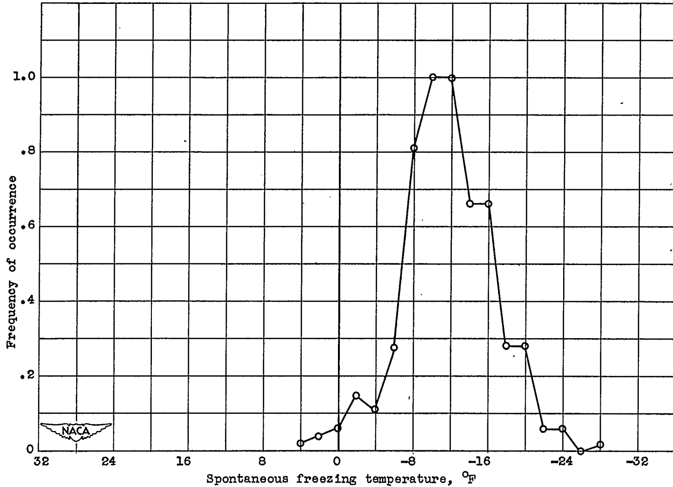
Figure 8. - Continued. Distribution of spontaneous freezing temperatures.
