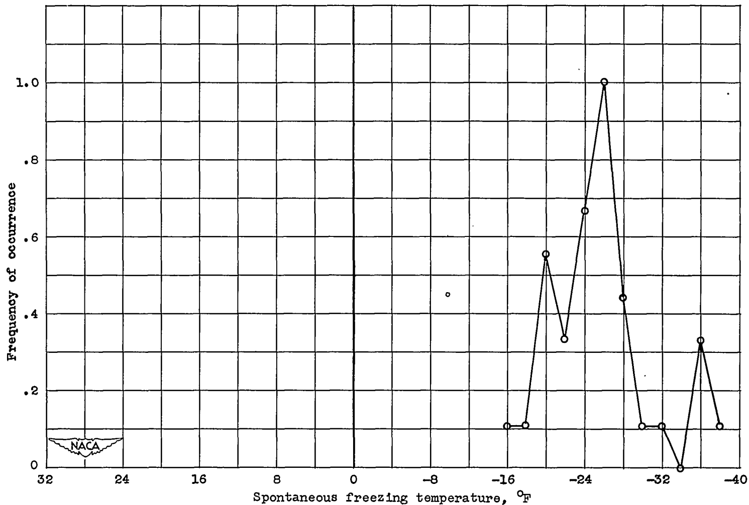
(a) Droplet diameter, 8.75 \pm 2.5 microns; droplets observed, 35; average spontaneous freezing temperature, -25.7^\circ\text{F} ; standard deviation, 5.13^\circ\text{F} .
