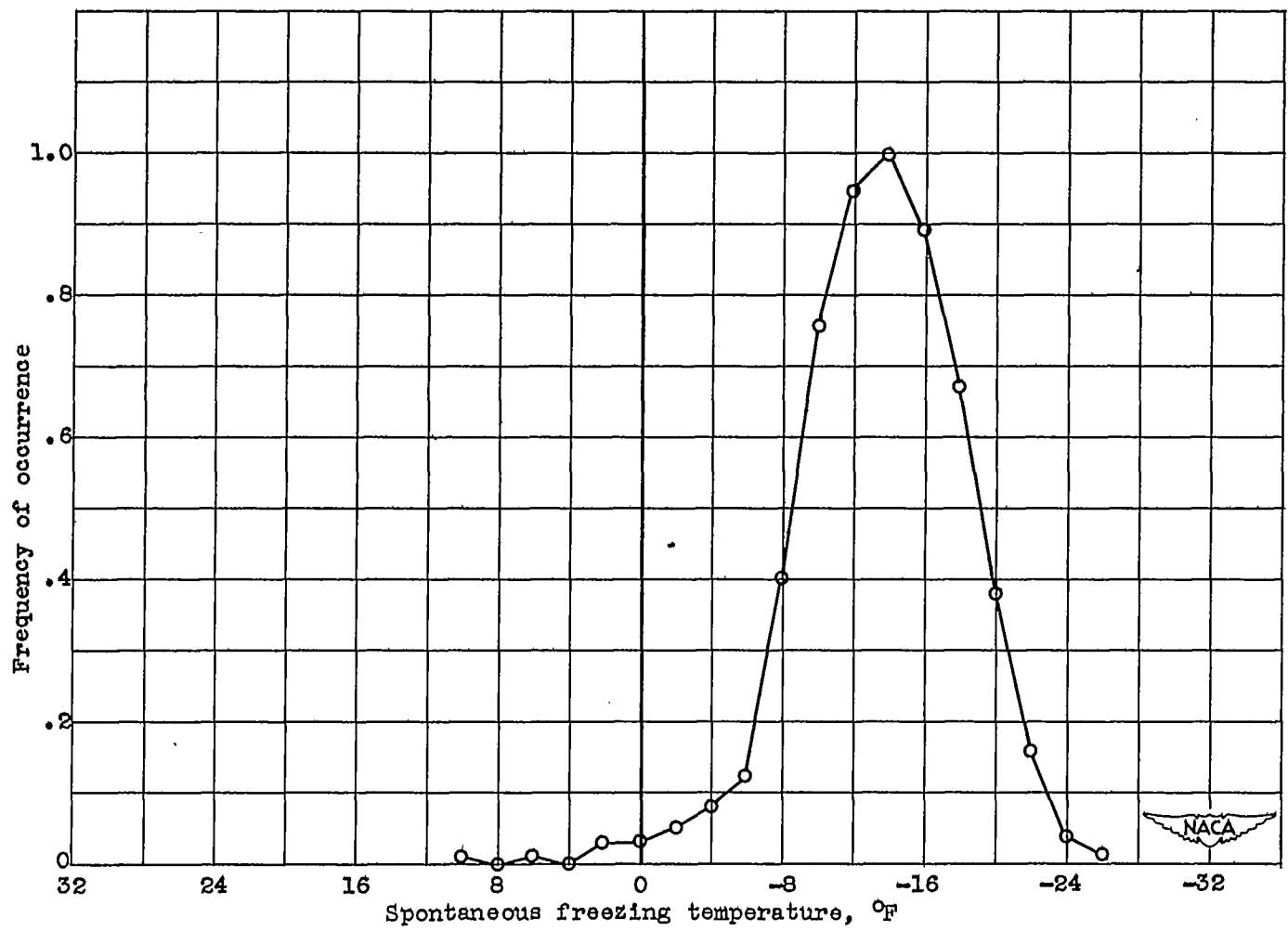
(g) Droplet diameter, 69.0 \pm 11.5 microns; droplets observed, 692; average spontaneous freezing temperature, -13.3^{\circ} F; standard deviation, 4.66^{\circ} F.
