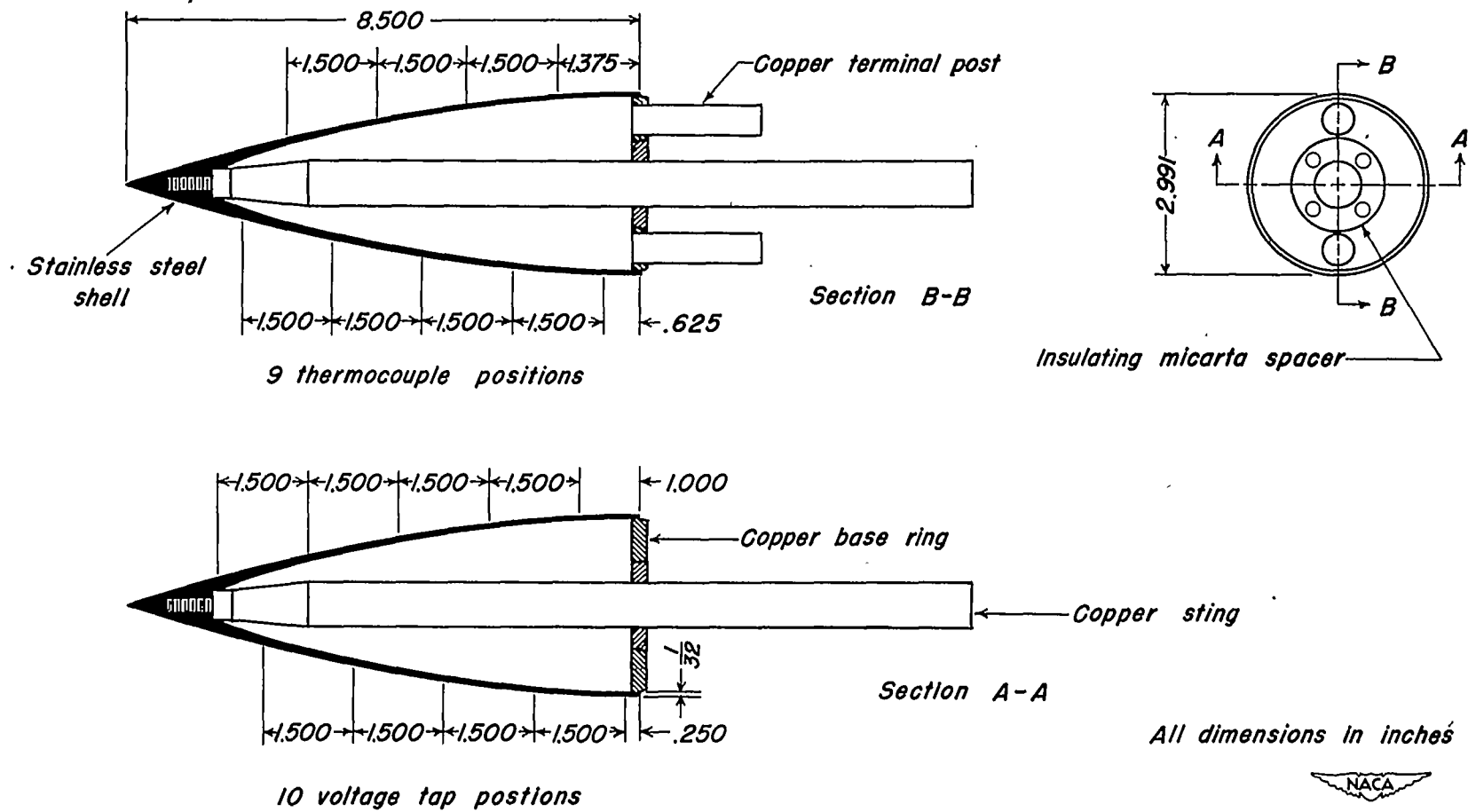
Figure 2.- Details of the test body.
