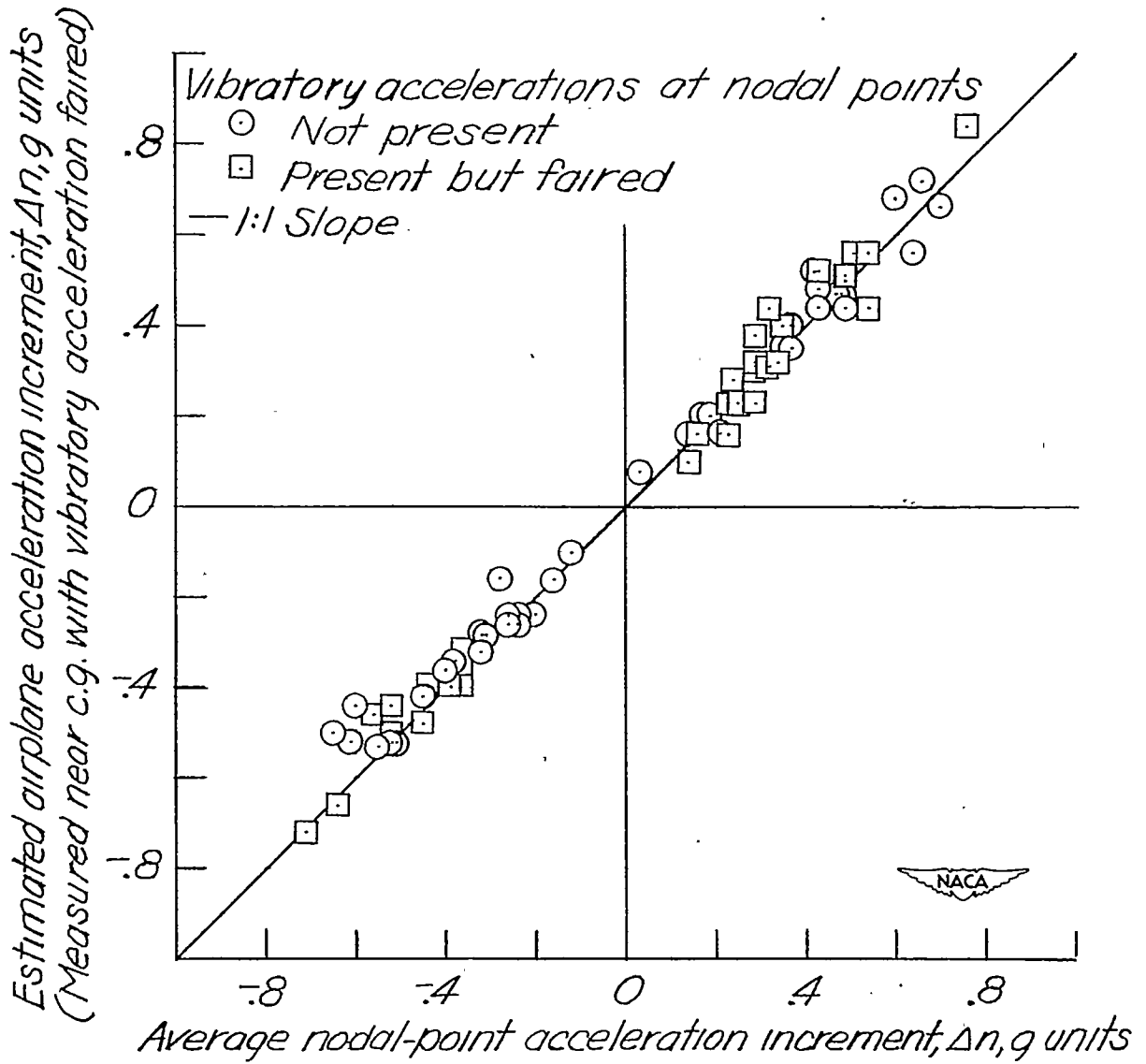
Figure 7.- Estimated airplane acceleration as a function of average nodal-point acceleration.
