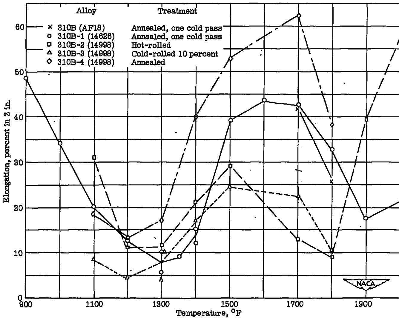
Figure 2.- Effect of treatment and temperature on tensile test elongation of 310B alloys.
