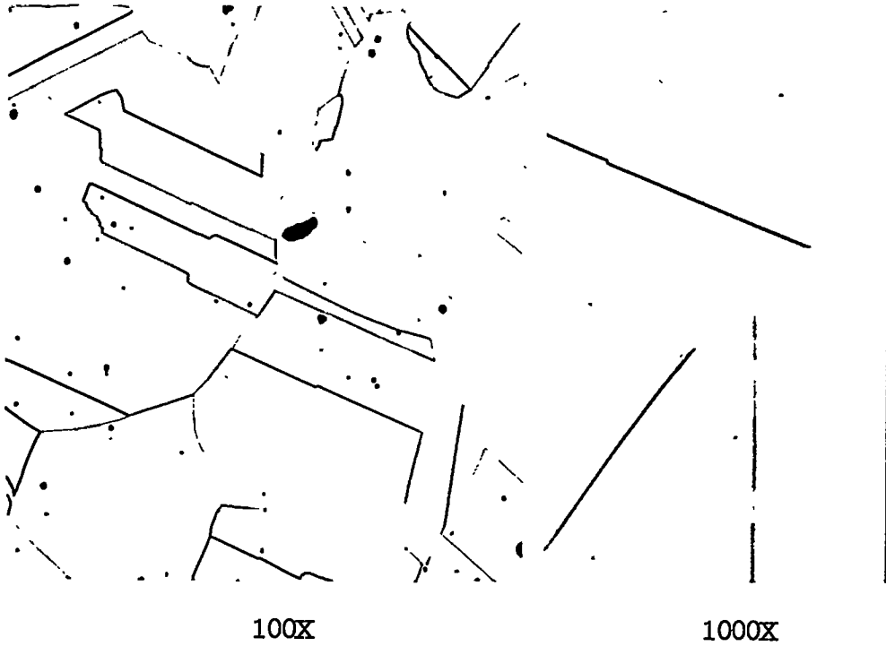
(b) Heat 14626; 310B-1 alloy sheet; annealed, one cold pass. No titanium.
