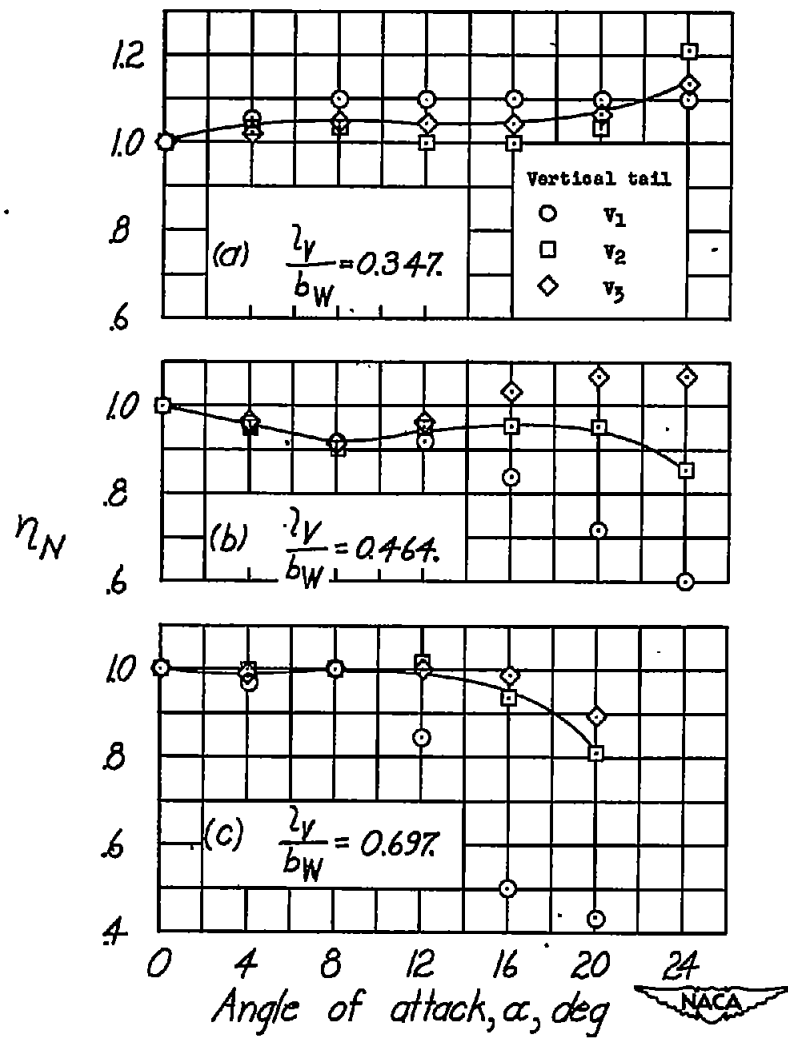
Figure 23.- Effect of tail area and length on the angle-of-attack correction to the vertical-tail contribution to C_{n_\alpha} . Circular-arc fuselages.
