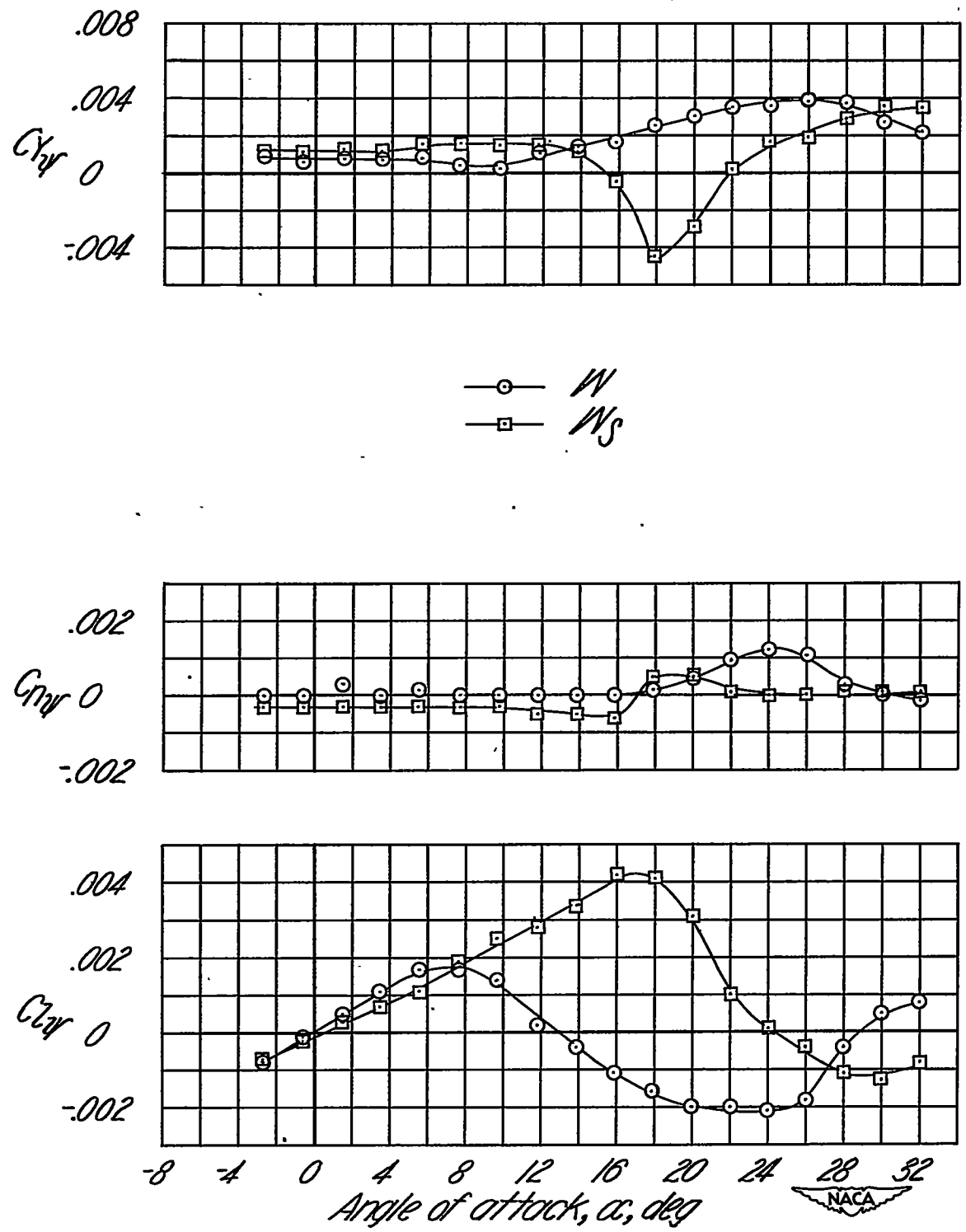
Figure 7.- Static lateral stability characteristics of the wing.
