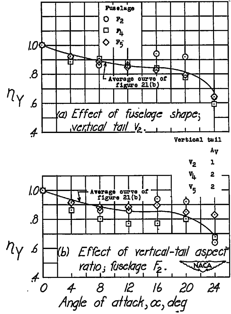
Figure 22.- Effect of fuselage shape and vertical-tail aspect ratio on the angle-of-attack correction to the vertical-tail contribution to C_{Y_p} .
