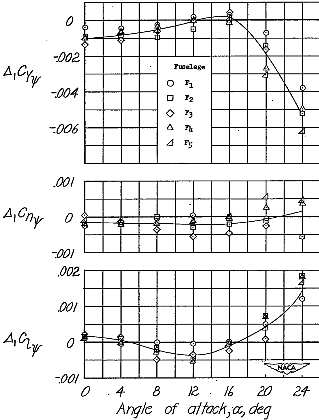
Figure 25.- Variation of increments of C_{Y\psi} , C_{N\psi} , and C_{Z\psi} caused by wing-fuselage interference with angle of attack.
