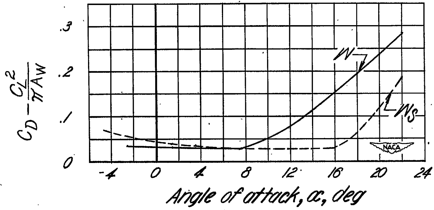
Figure 15.- Effect of wing leading-edge slat on the variation of C_D - \frac{C_L^2}{\pi A_w} of the wing with angle of attack.
