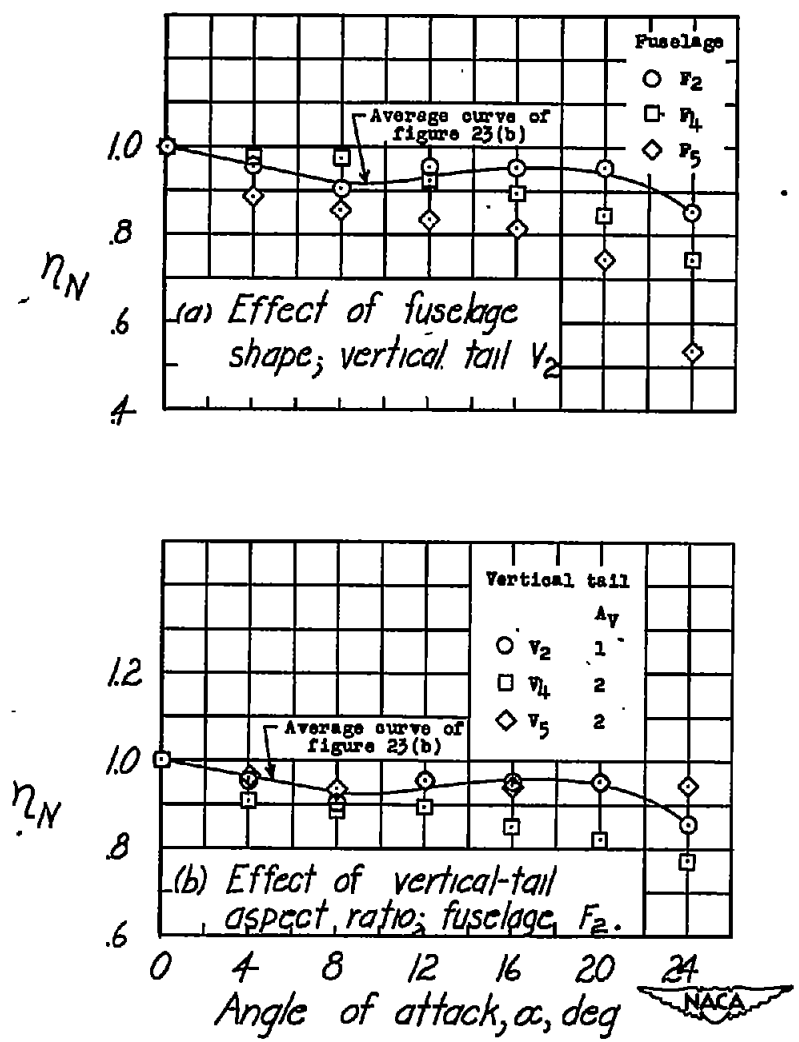
Figure 24.- Effect of fuselage shape and vertical-tail aspect ratio on the angle-of-attack correction to the vertical-tail contribution to C_{n_\alpha} .
