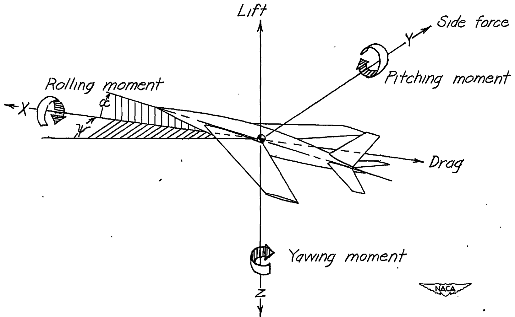
Figure 1.- System of axes used. Arrows indicate positive direction of angles, forces, and moments.
