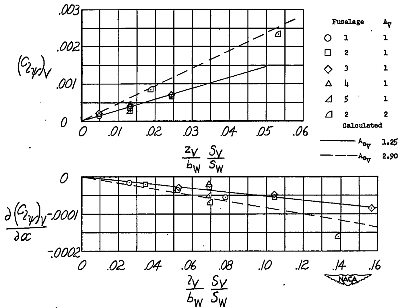
Figure 20.- Effect of tail area and length on the vertical-tail contribution to C_{2\psi} . \alpha = 0^\circ .
