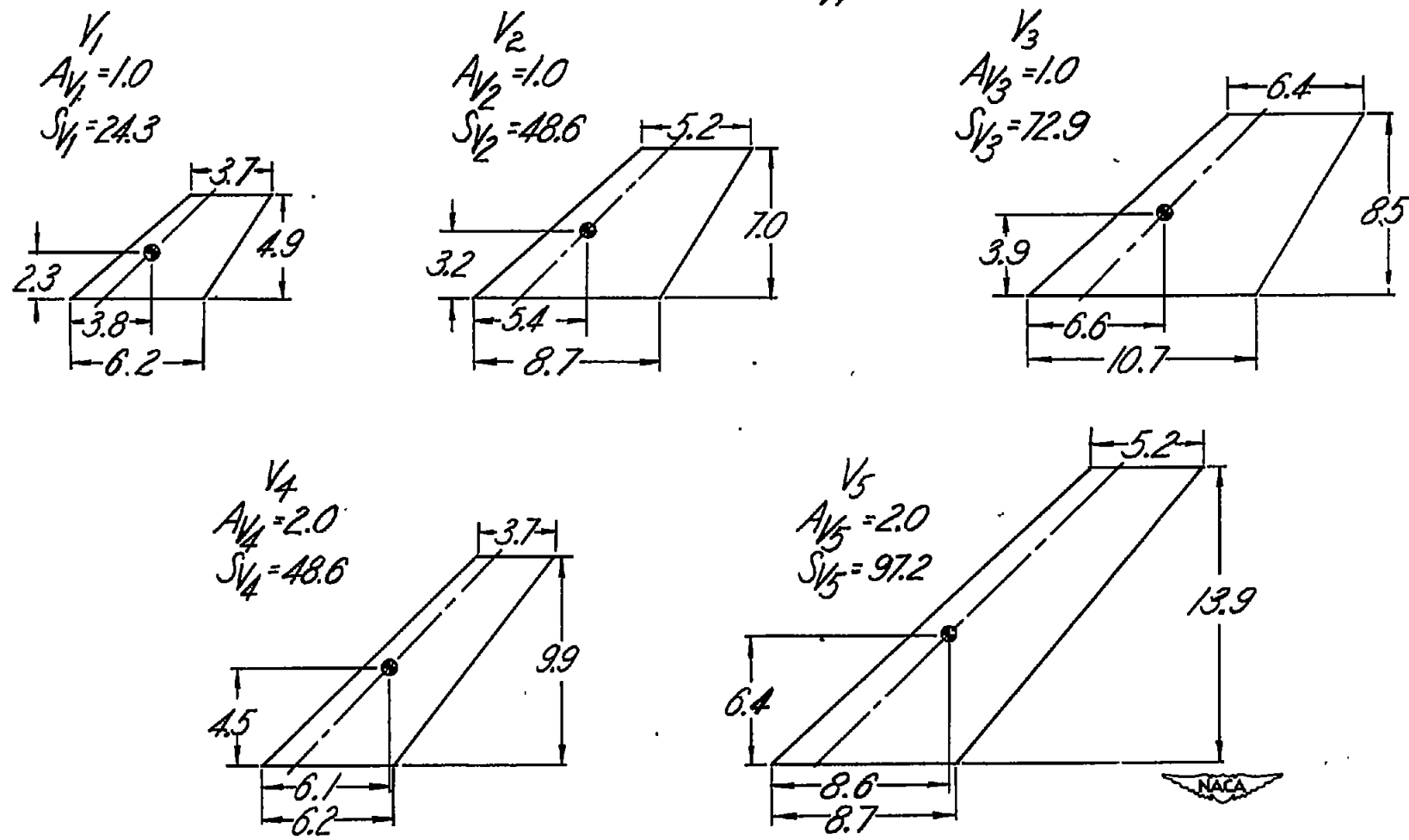
Figure 2.- Dimensions of vertical tails tested. \lambda = 0.6 ; \Lambda = 45^\circ ; profile, NACA 65A008. All dimensions are in inches.
