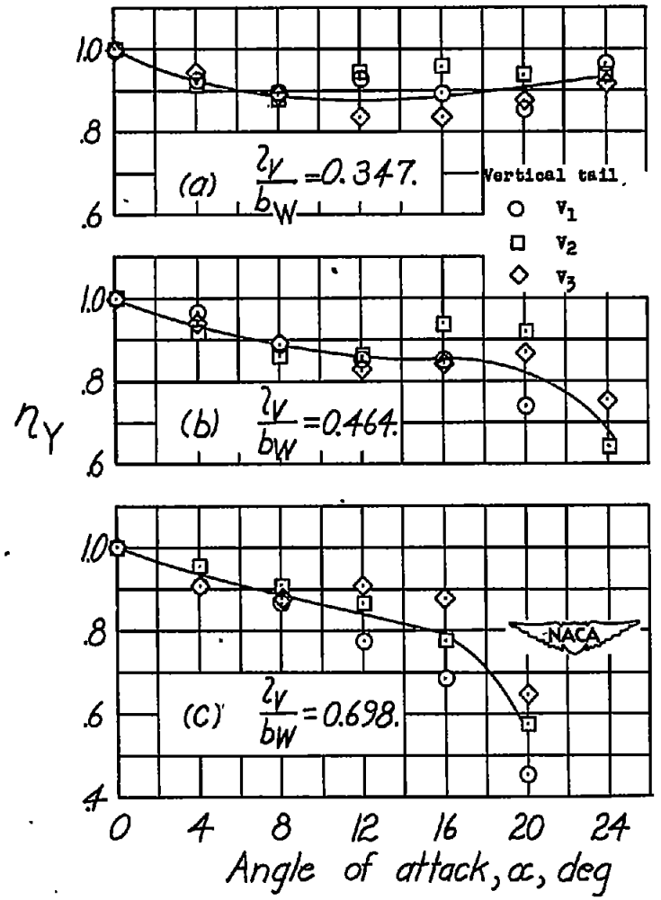
Figure 21.- Effect of tail area and length on the angle-of-attack correction to the vertical-tail contribution to C_{Y_p} . Circular-arc fuselages.
