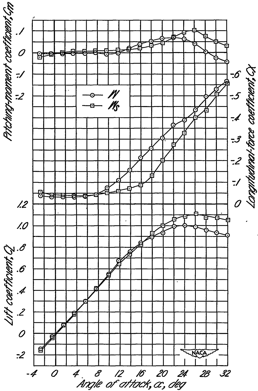
Figure 6.- Aerodynamic characteristics of the wing.
