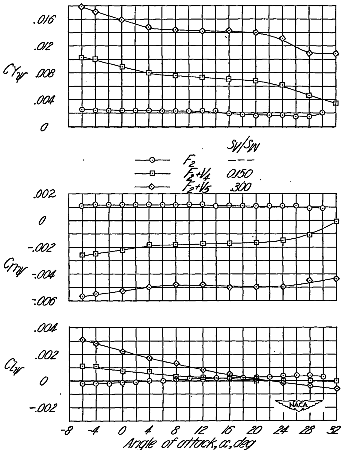
Figure 12.- Effect of vertical tail on the static lateral stability characteristics. Wing off; fuselage 2; A_y = 2.0 .
