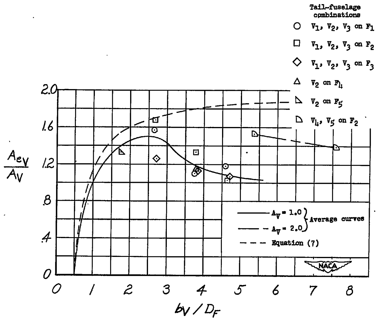
Figure 18.- Effective aspect ratio of vertical tails as influenced by the fuselage. \alpha = 0^\circ .
