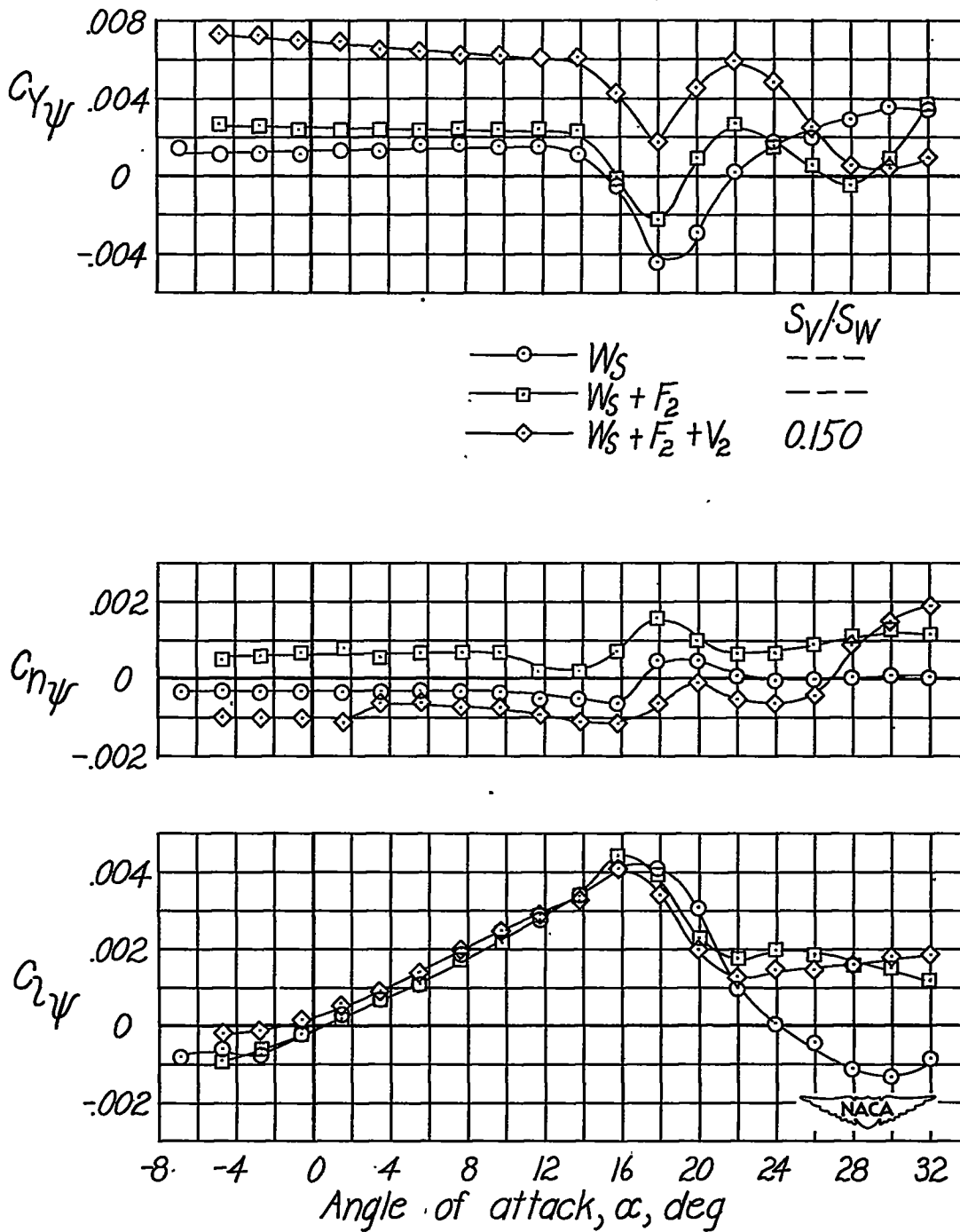
Figure 14.- Static lateral stability characteristics of configurations having wing leading-edge slat. A_{\psi} = 1.0 .
