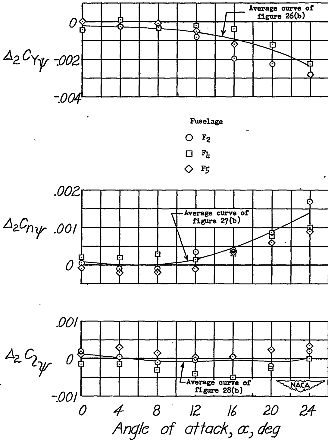
Figure 29.- Effect of fuselage shape on the increments of C_{Y\psi} , C_{n\psi} , and C_{z\psi} caused by the wing-fuselage interference on the vertical-tail effectiveness. Vertical tail V_2 .
