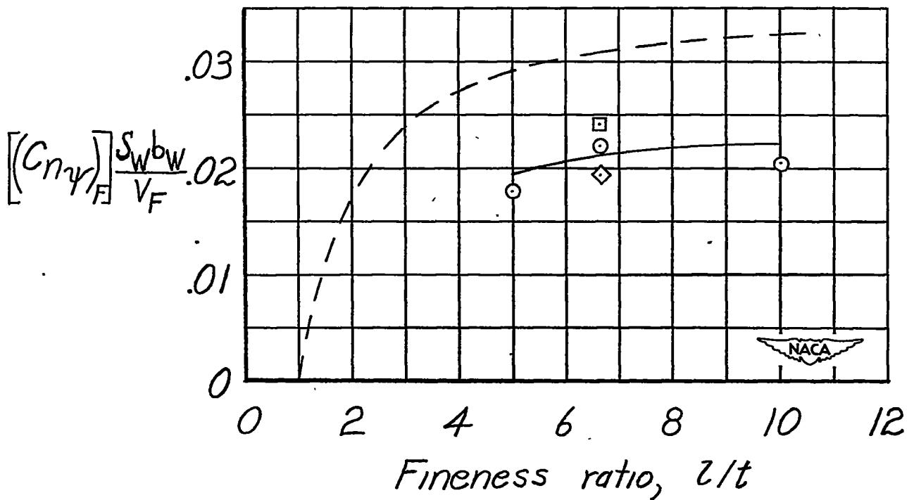
Figure 16.- Summary of fuselage contributions to C_{Y_p} and C_{n_p} . \alpha = 0^\circ .
