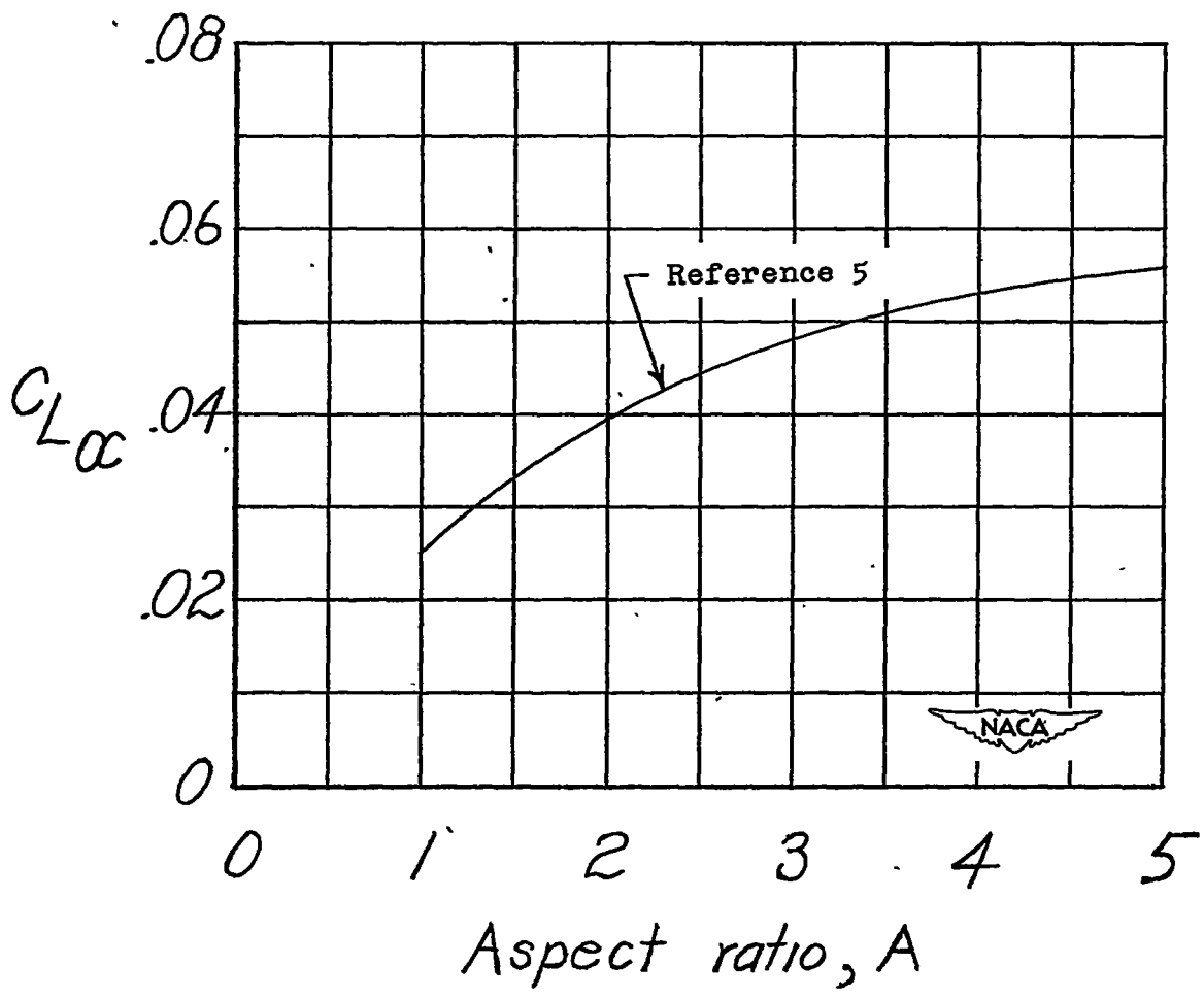
Figure 17.- Variation of lift-curve slope with aspect ratio for 45° sweptback wings with taper ratio 0.6.
