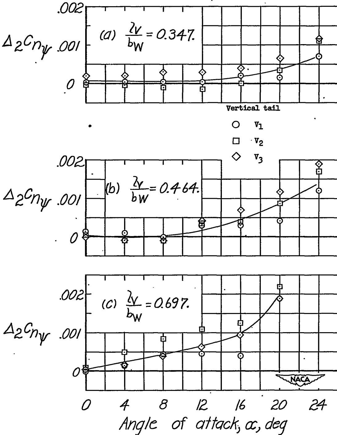
Figure 27.- Effect of tail area and length on the increment of C_{n\psi} caused by the wing-fuselage interference on the vertical-tail effectiveness. Circular-arc fuselages.
