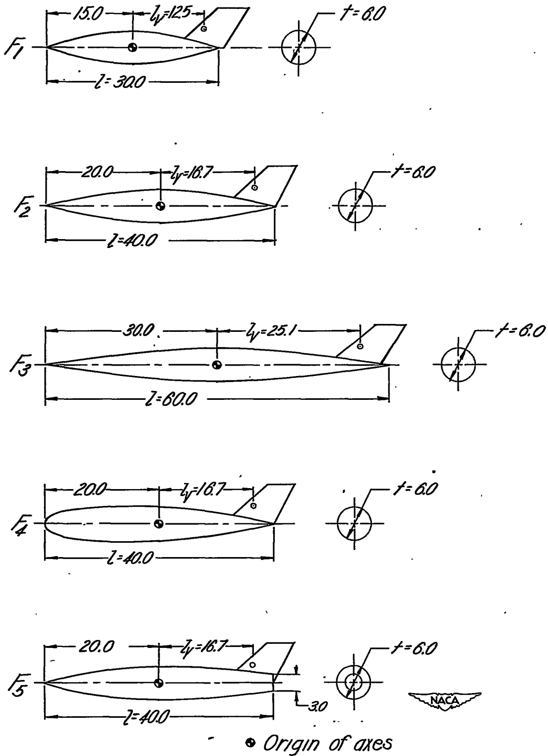
Figure 3.- Dimensions of fuselages; profile ordinates in table II. All dimensions are in inches.
