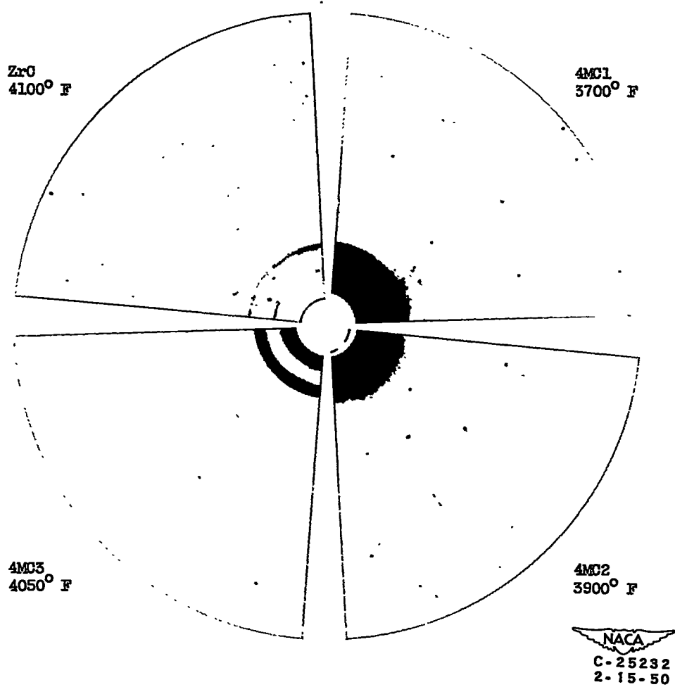
Figure 2. - Back-reflection X-ray diffraction patterns of zirconium carbide - columbium ceramals showing effect of various sintering temperatures on lattice parameters as compared with zirconium carbide. Sintering time, 5 minutes.
