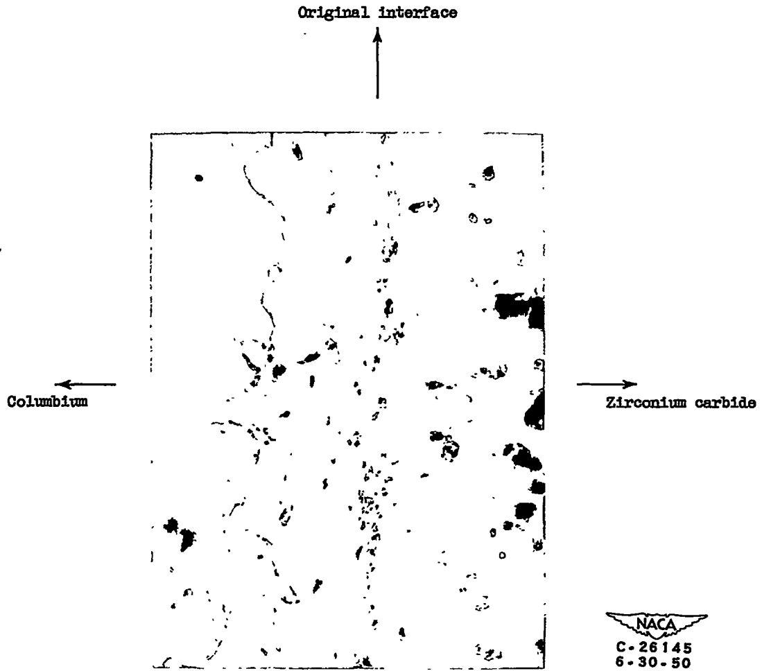
Figure 1. - Microstructure of unetched columbium - zirconium carbide bonding specimen after 15 minutes at 4250° F. X250.
