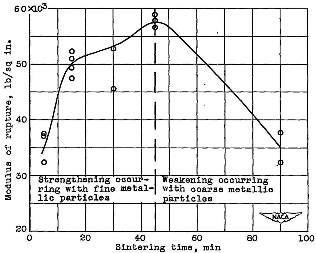
Figure 6. - Variation of room-temperature modulus of rupture with sintering time at 3900^{\circ} F for zirconium carbide - columbium ceramal.
