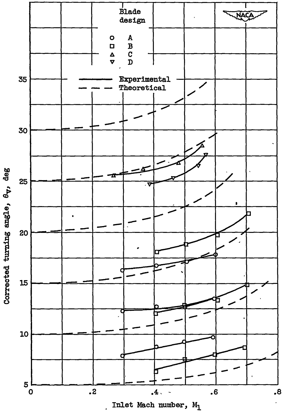
Figure 8. - Comparison of compressibility variation of corrected turning angles obtained from two-dimensional flow with experimental corrected turning angles obtained from inlet guide vanes in annular cascade. All angles corrected to constant axial velocity based on inlet axial velocity and assumption of constant circulation.
