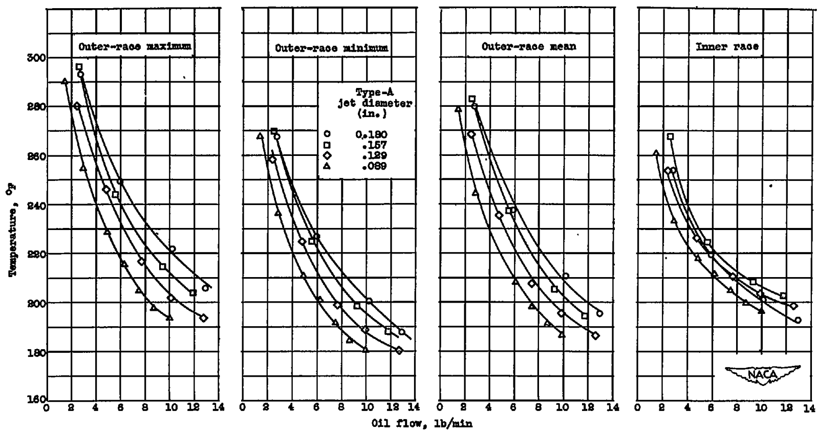
Figure 8. - Effect of oil flow on temperatures of bearing 9 for type-A jets. Load, 115 pounds; DN, 1.43 \times 10^6 ; oil inlet temperature, 100^\circ \text{F} .
