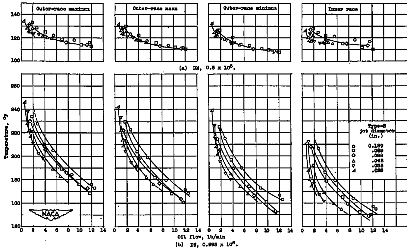
Figure 7. - Variation of temperature of bearing 6 with oil flow for type-B jets. Load, 368 pounds; oil inlet temperature, 100° F.
