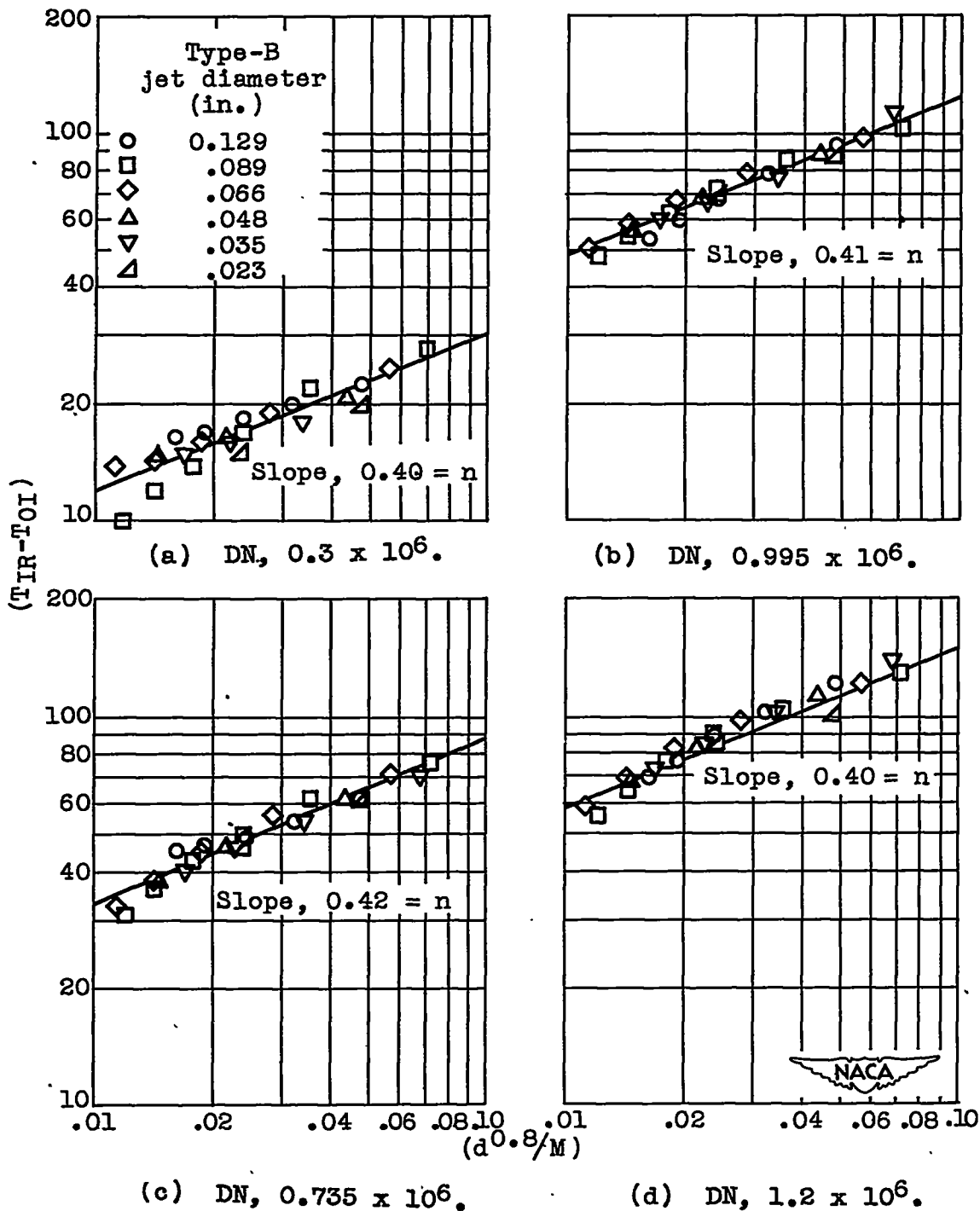
Figure 12. - Determination of exponent n for cooling correlation equation [(T_{IR} - T_{OI}) = E^n (d^{0.8}/M)^n] for inner-race temperature of bearing 6. Load, 368 pounds; oil inlet temperature, 100^\circ F; oil flows, 0.6 to 12.9 pounds per minute; oil-jet diameters, 0.023 to 0.129 inch.
