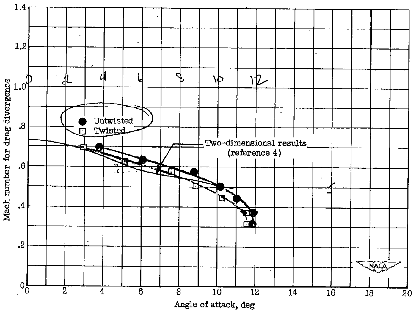
Figure 7.- Comparison of rotor experimental results with two-dimensional drag-divergence Mach number against angle of attack for NACA 23015 airfoil section.
