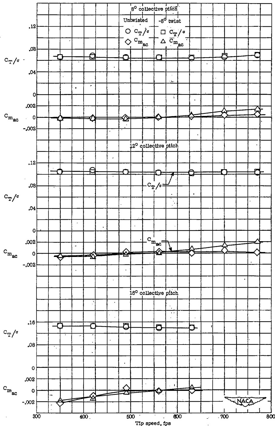
Figure 6.- Comparison of C_T/\sigma and C_{m_{ac}} for both untwisted and twisted blades over a tip-speed range from 350 to 770 feet per second for three representative collective pitch settings of 8°, 12°, and 16°.
