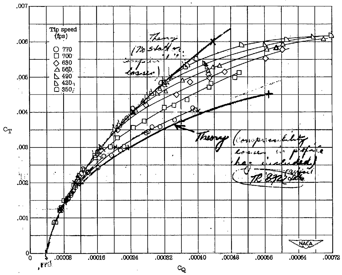
Figure 2.- Hovering performance of the untwisted rotor blades over a range of tip speeds from 350 to 770 feet per second. \sigma = 0.038 .
