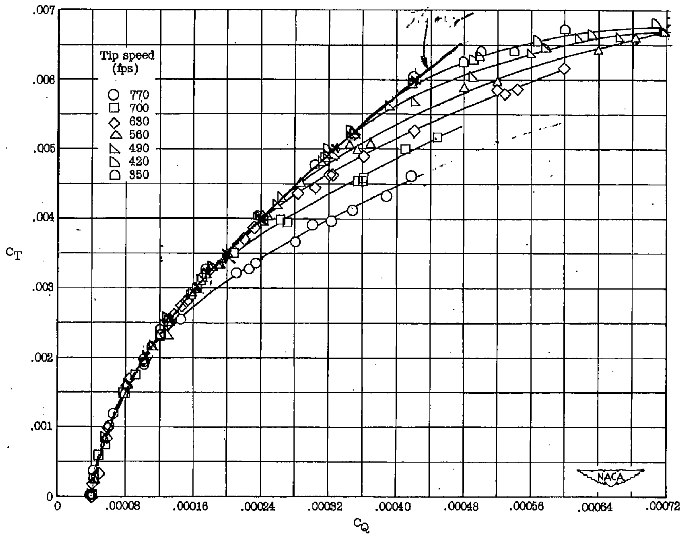
Figure 3.- Hovering performance of the rotor blades having -8^\circ of linear twist over a range of tip speeds from 350 to 770 feet per second. \sigma = 0.038 .
