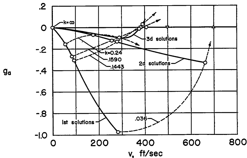
(a) Variation of artificial damping with airspeed.
