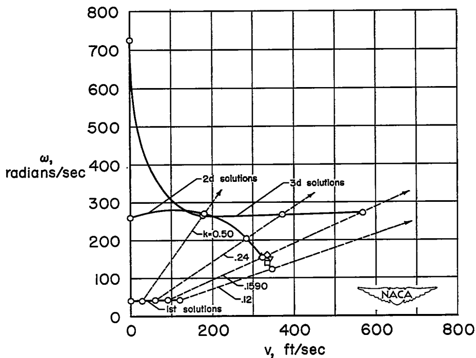
(b) Variation of frequency with airspeed.
