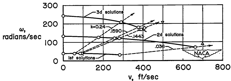
(b) Variation of frequency with airspeed.
