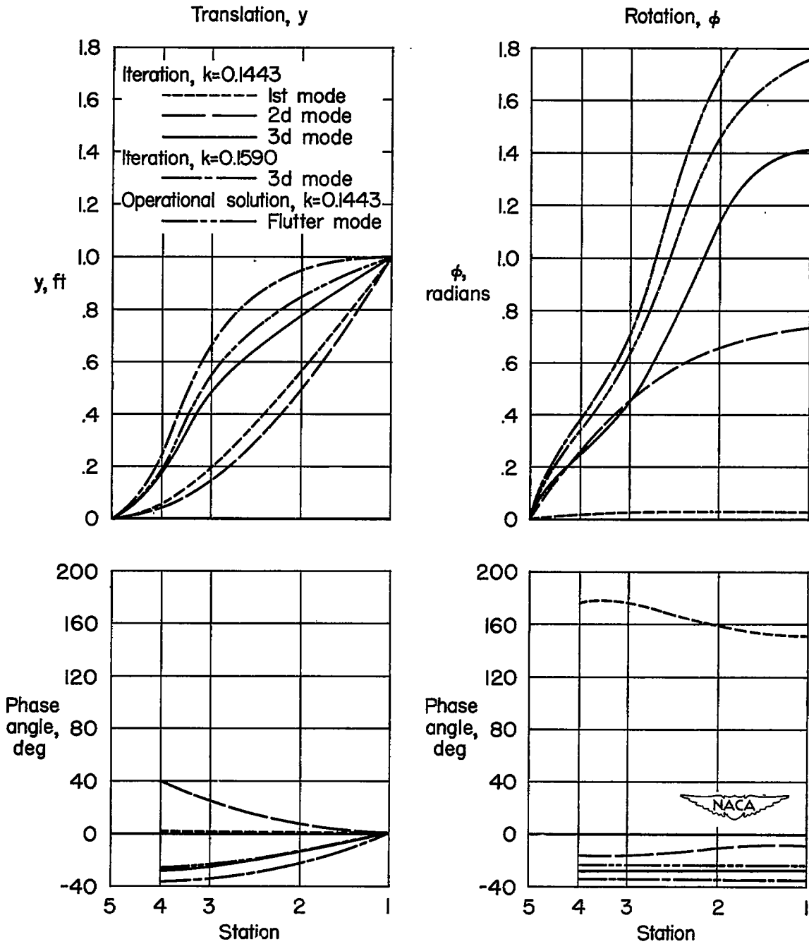
Figure 5.- Amplitudes and phases of modes. Wing with concentrated mass.
