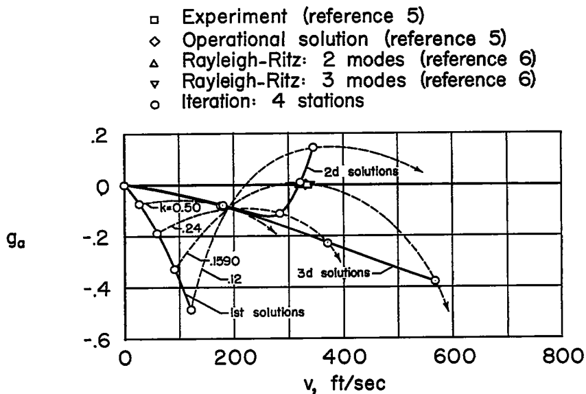
(a) Variation of artificial damping with airspeed.
