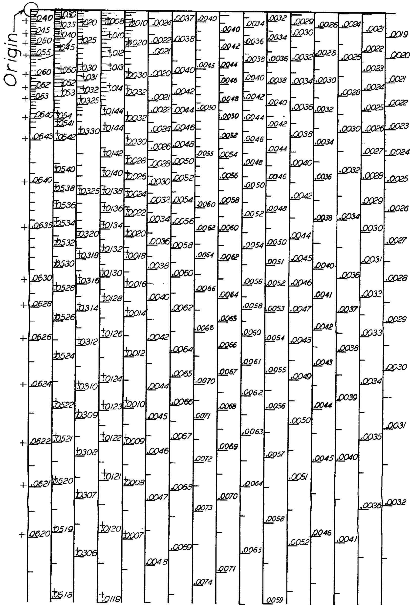
Figure 4.- Downwash chart for points 0.4 semispan above plane of wake. (All values are negative except those specifically marked with a plus sign.)
