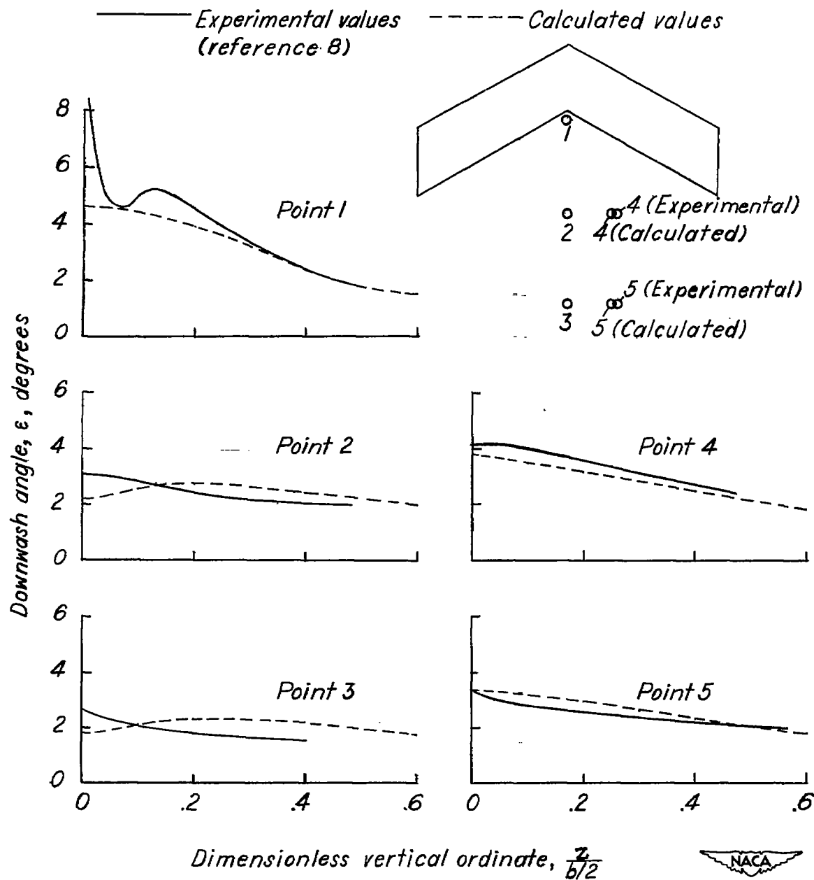
Figure 8.- Downwash angles behind 30^\circ sweptback wing. A = 4.5 ; \lambda = 1 ; \alpha = 8.18^\circ .
