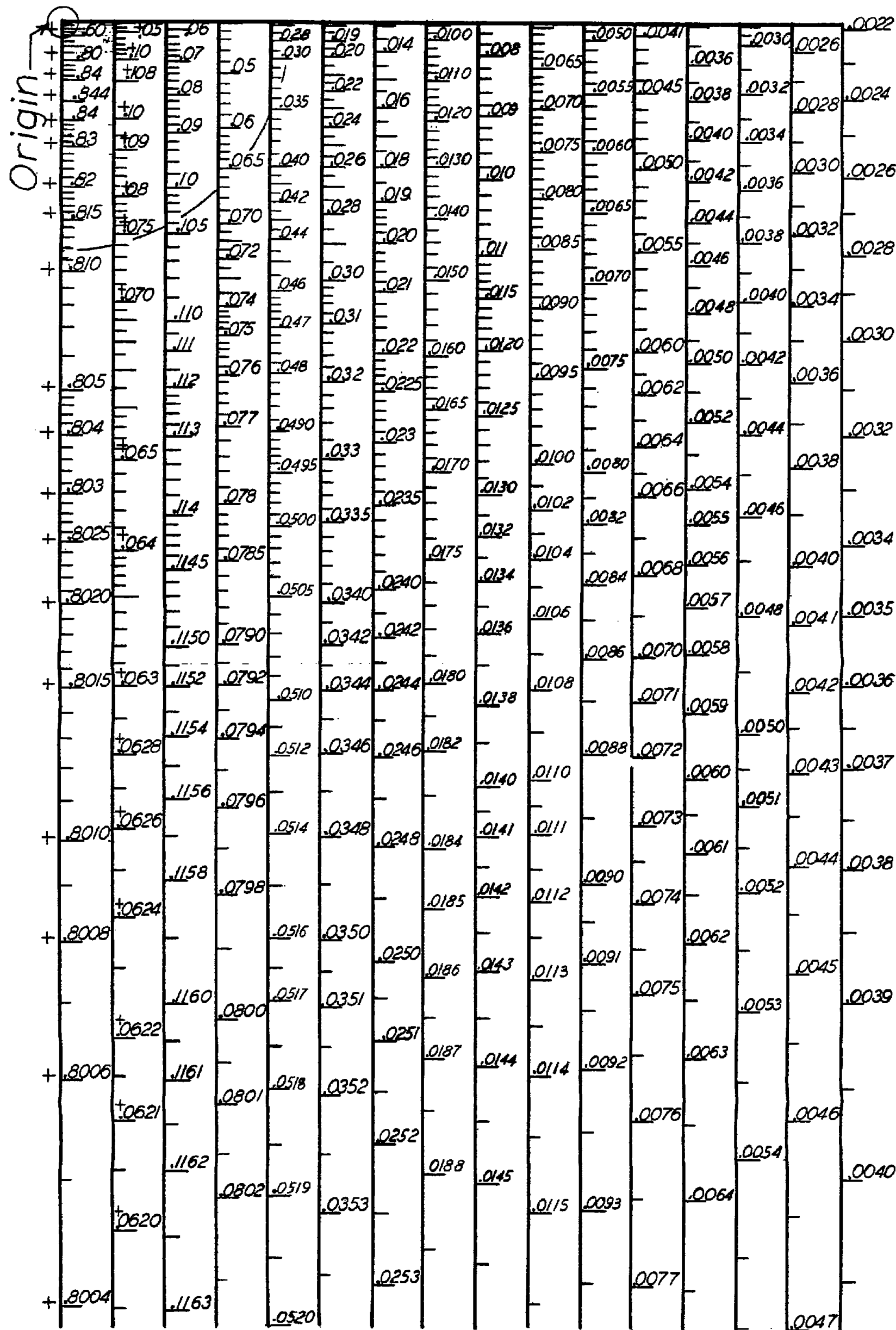
Figure 2.- Downwash chart for points 0.1 semispan above plane of wake. (All values are negative except those specifically marked with a plus sign.)
