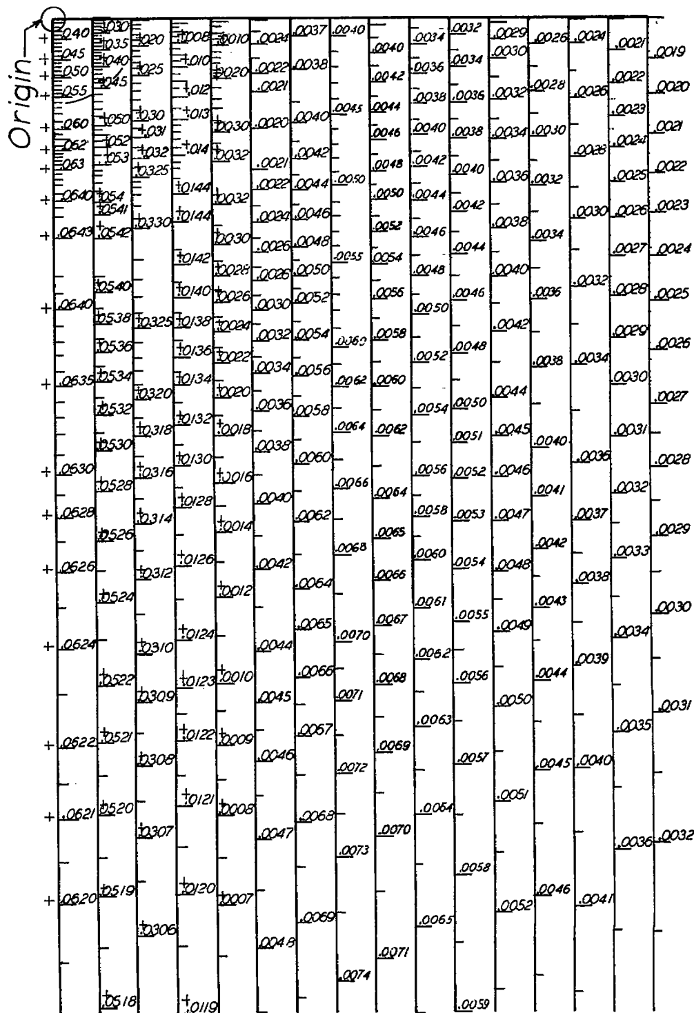
Figure 4.- Downwash chart for points 0.4 semispan above plane of wake. (All values are negative except those specifically marked with a plus sign.) (Full-size figure will be found in the flap at the back of this paper.)
