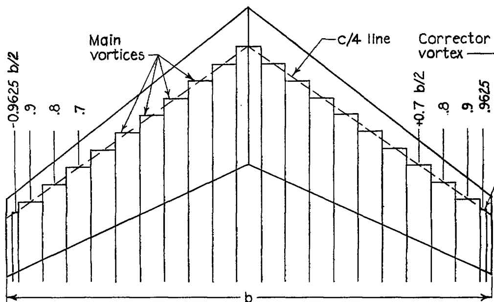
(a) Location of horseshoe vortices.
