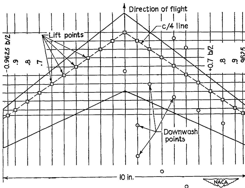
(a) Location of horseshoe vortices.
