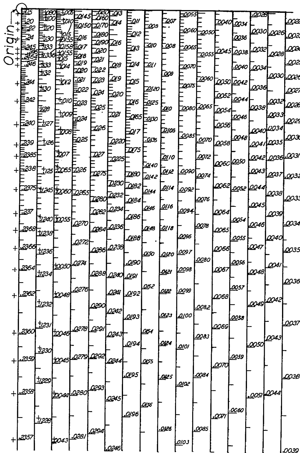
Figure 3.- Downwash chart for points 0.2 semispan above plane of wake. (All values are negative except those specifically marked with a plus sign.) (Full-size figure will be found in the flap at the back of this paper.)
