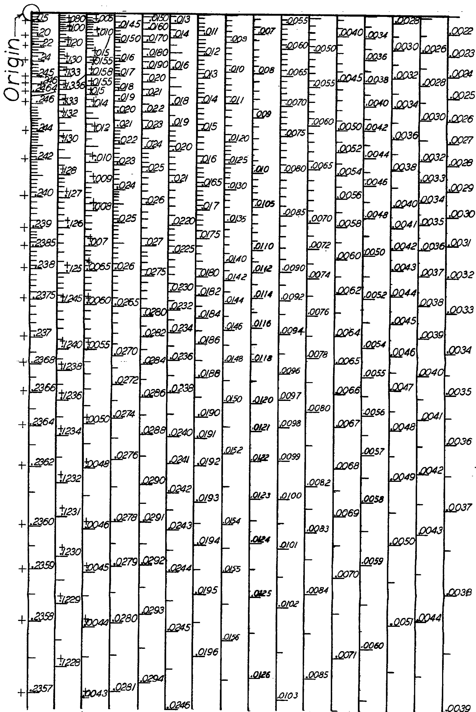
Figure 3.- Downwash chart for points 0.2 semispan above plane of wake. (All values are negative except those specifically marked with a plus sign.)
