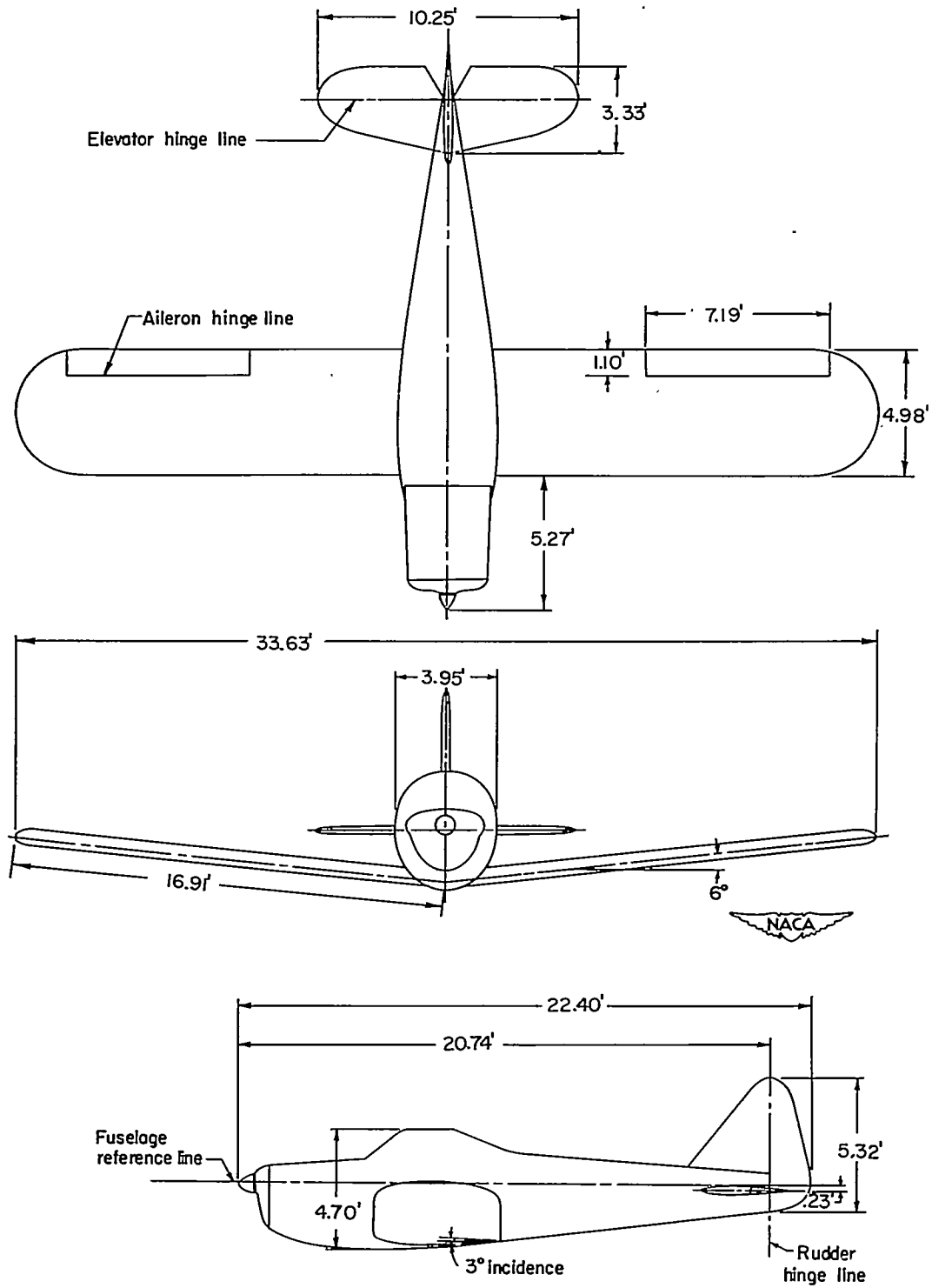
Figure 2.- Three-view drawing of the typical personal-owner airplane simulated by the \frac{1}{6} -scale model.
