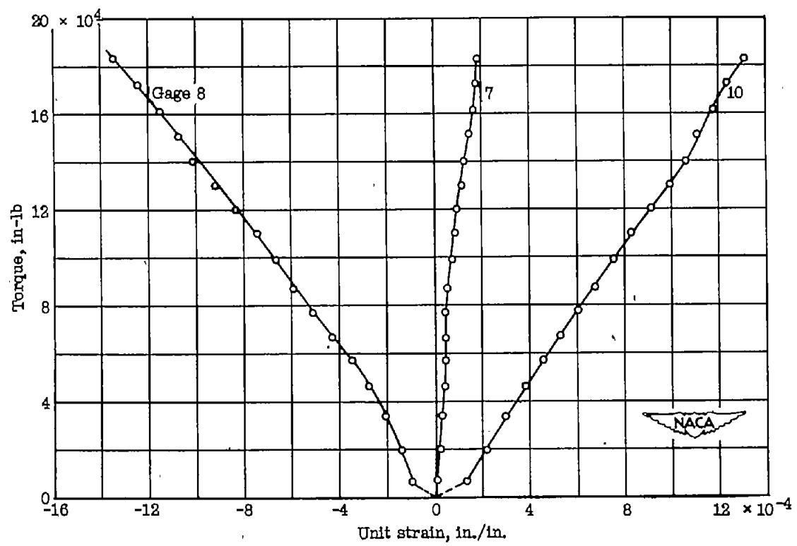
Figure 16.- Web strain distribution of specimen 21, a stiffened D-tube with NACA 0012 section and closing web at 30-percent station. Strain measured on rosette strain gages; specimen made of alclad 24S-T3 aluminum alloy; E = 10.2 \times 10^6 psi, \mu = 0.33 , thickness of web is 0.081 inch.
