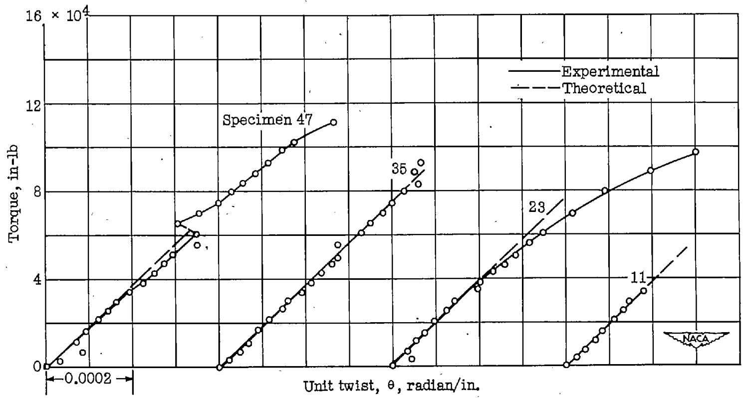
Figure 14.- Effect of addition of stringers on torsional stiffness of D-tubes with NACA 0012 section and closing web at 30-percent station. Specimens made of alclad 24S-T3 aluminum alloy; E = 10.2 \times 10^6 psi, \mu = 0.33 , t = 0.049 inch, a = 18 inches, L = 8 inches.
