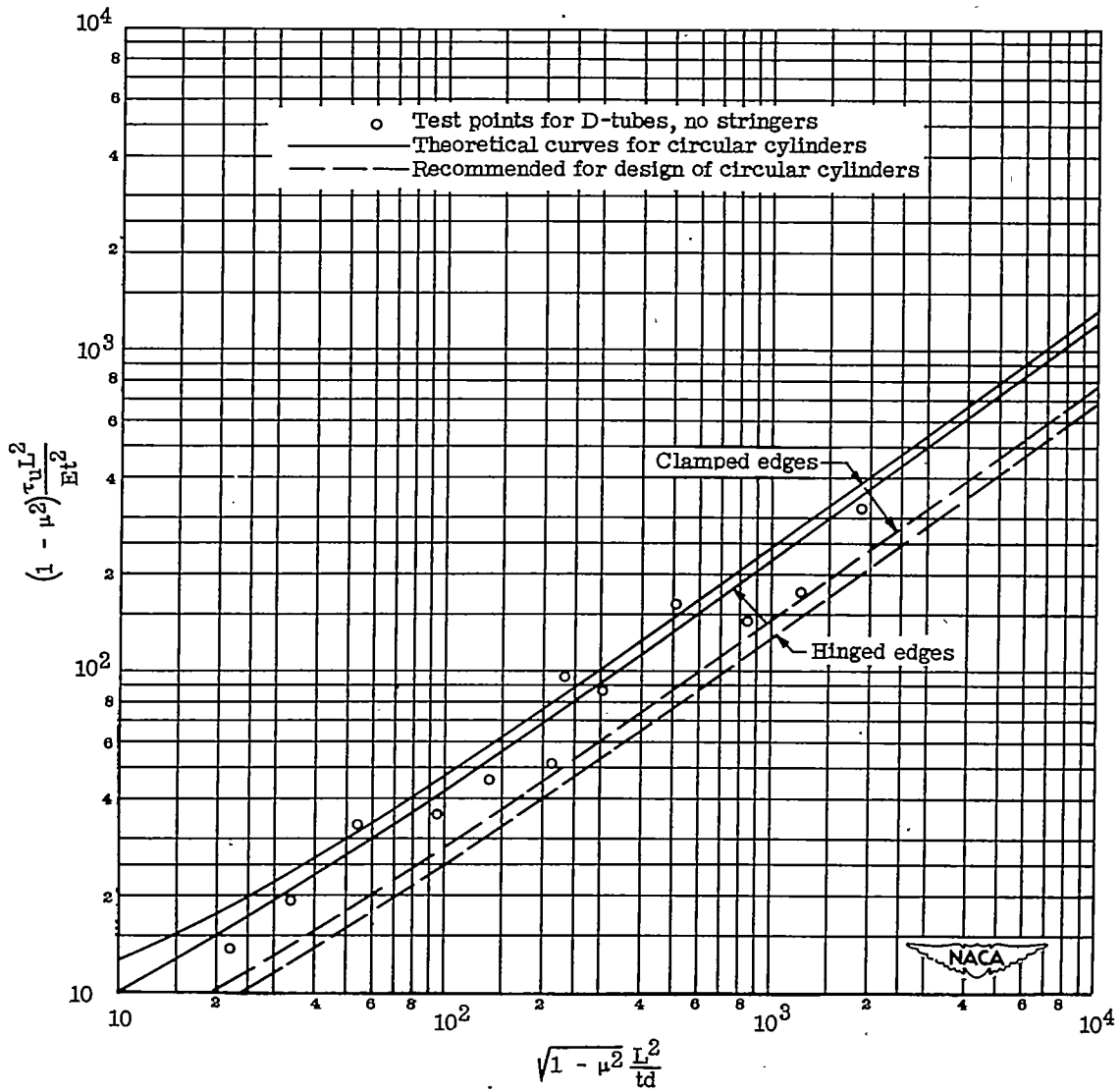
Figure 10.- Comparison of critical torsional stress for circular cylinders and D-tubes. Short and medium-length tubes tested; diameter d of circular cylinders taken as 2a for D-tubes.
