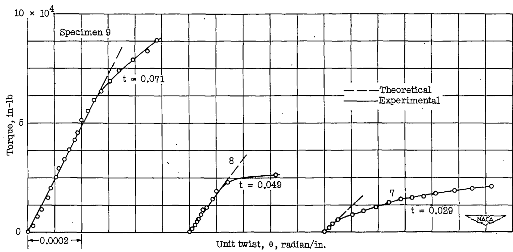
Figure 12.- Effect of increasing skin thickness on section rigidity of D-tubes with NACA 0012 section and closing web at 30-percent station. Specimens made of alclad 24S-T3 aluminum alloy; E = 10.2 \times 10^6 psi, \mu = 0.33 , gage length 16 inches, no stringers.
