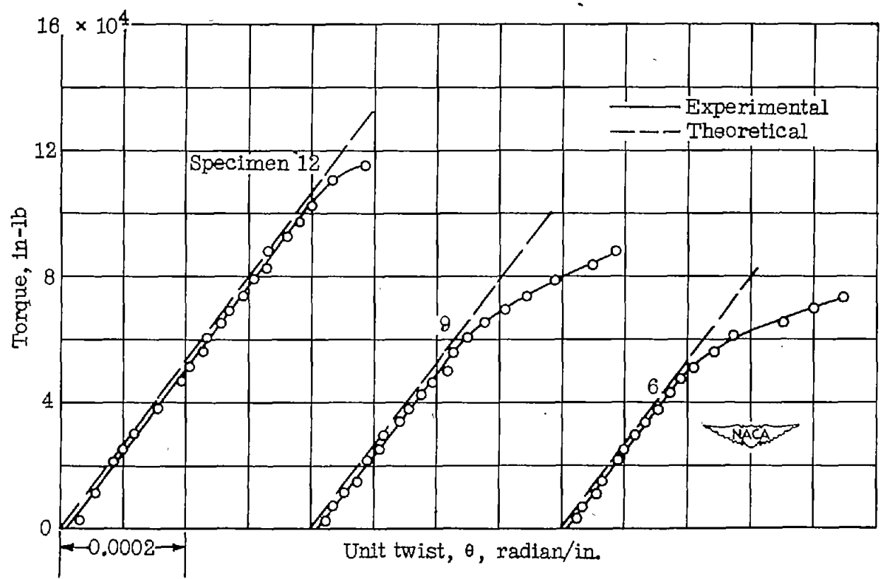
Figure 13.- Experimental and theoretical values of torsional stiffness of D-tubes revealing experimental error encountered during testing. Specimens made of alclad 24S-T3 aluminum alloy with NACA 0012 airfoil section and closing web at 30-percent station; E = 10.2 \times 10^6 psi, \mu = 0.33 , t = 0.071 inch, a = 18 inches, no stringers.
