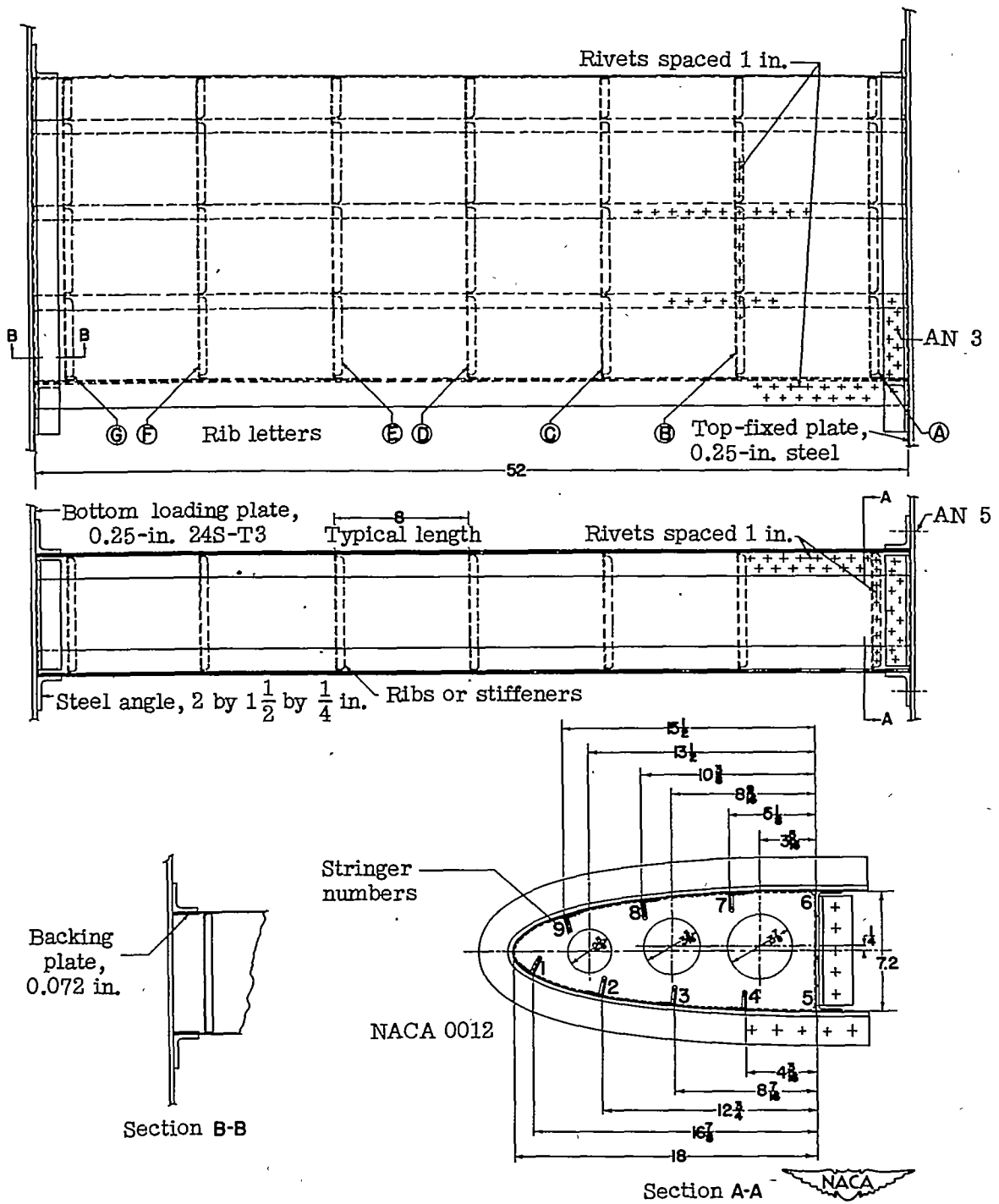
Figure 1.- Details of specimen 48; dimensions given in inches. Other specimens similar except for number of ribs and stringers. Dimensions vary with specimen; see table I.
