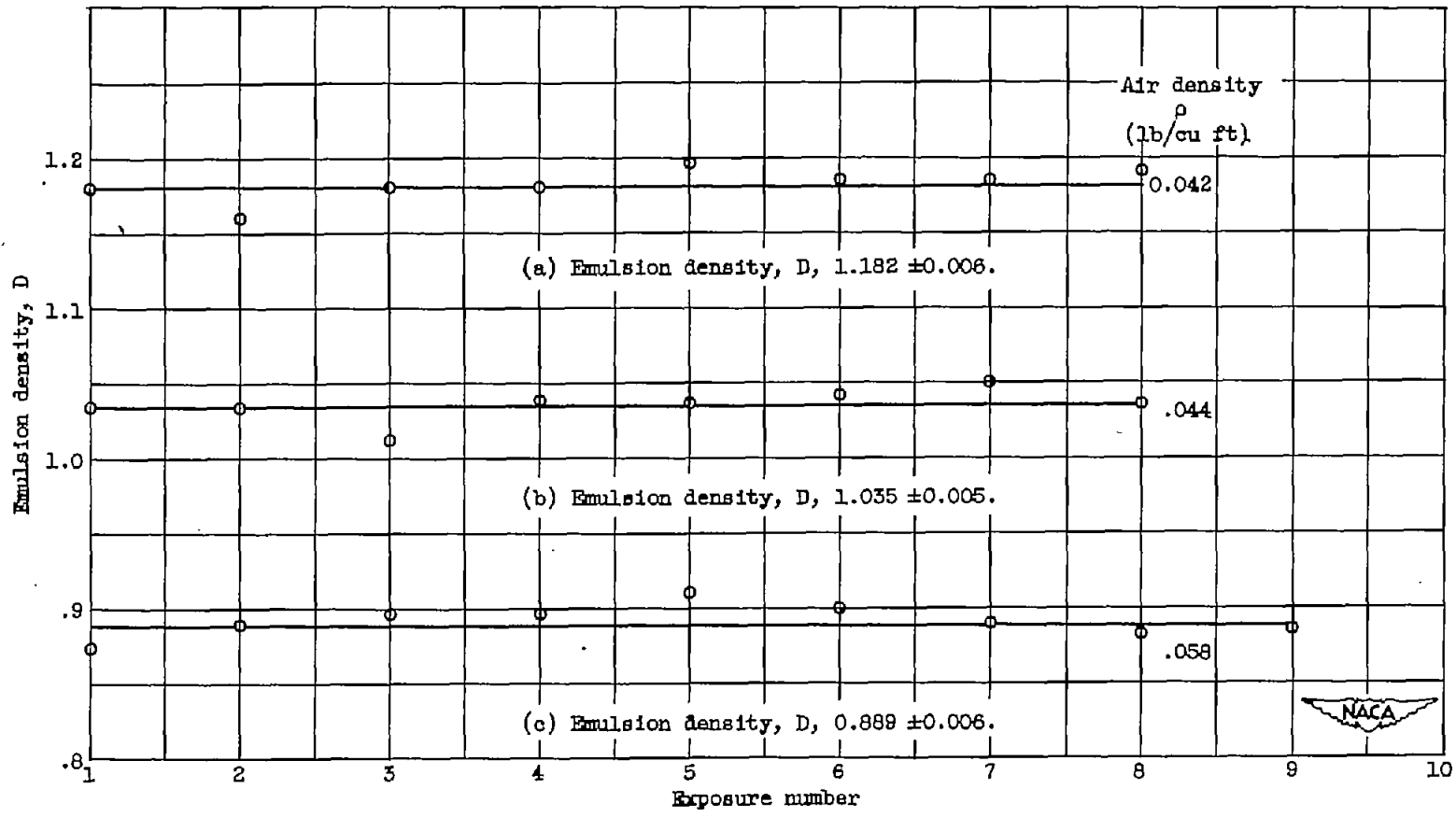
Figure 8. - Emulsion-density reproducibility at 4.0 kilovolts, 17.5-milliampere plate current, and 45-second exposure. Average \Delta D , \pm 0.0055 .
