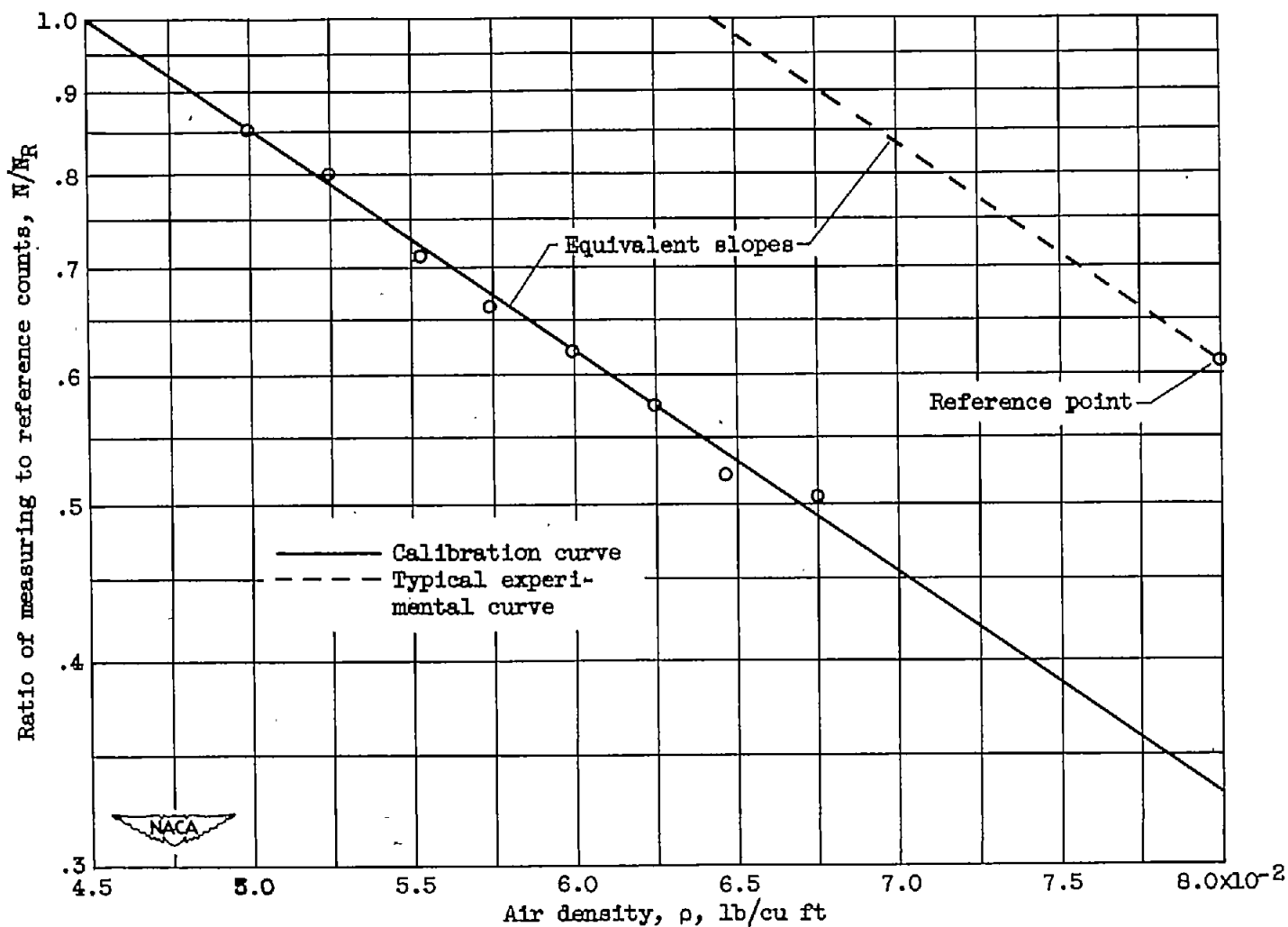
Figure 11. - Calibration curves at X-ray voltage of 3.2 kilovolts and tunnel width of 4 inches.
