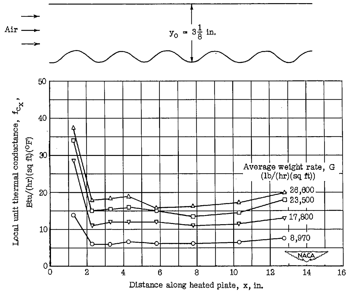
(c) Large wave plate at y_0 = 3\frac{1}{8} inches.
