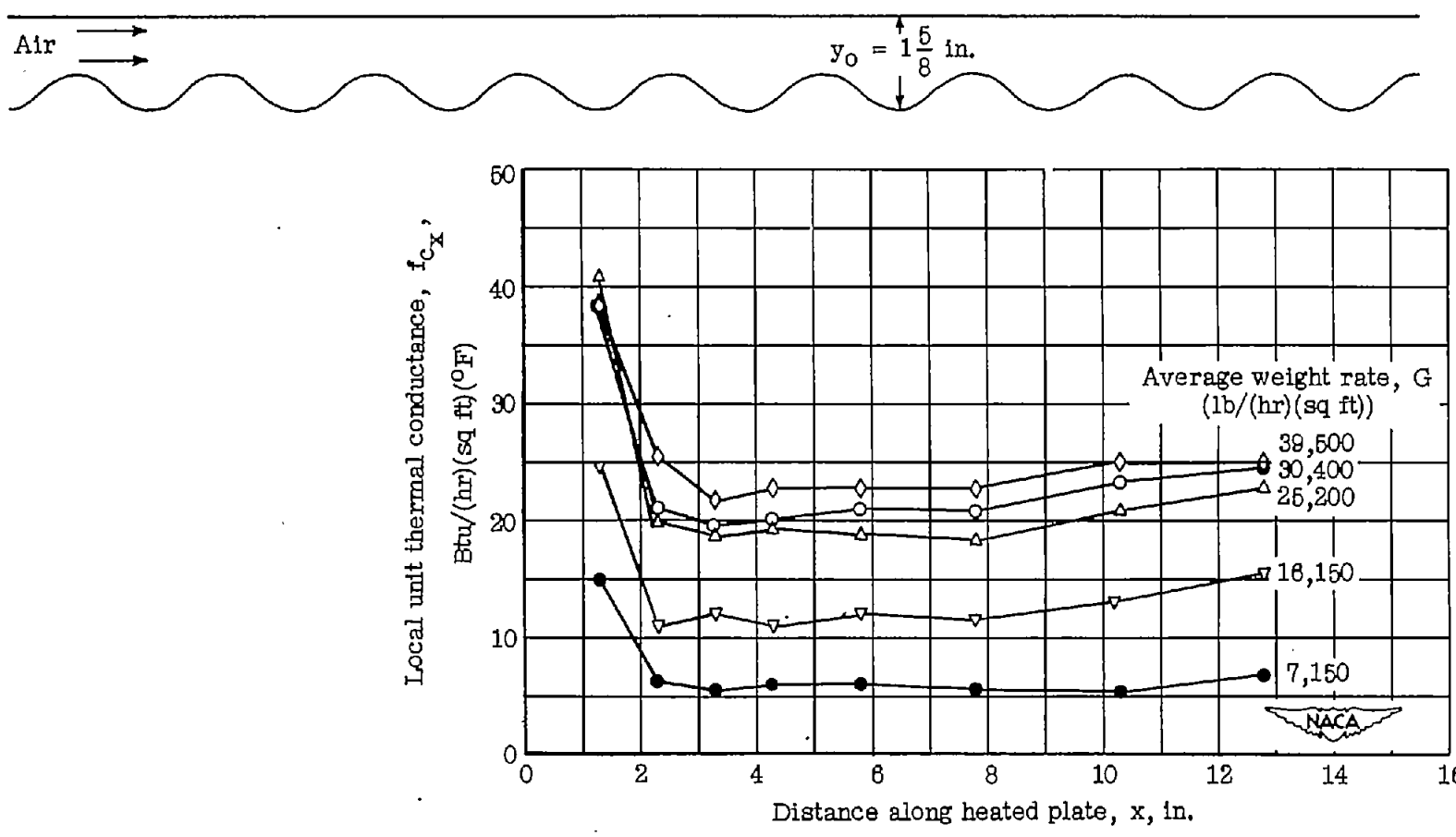
(b) Large wave plate (leading edge upstream) at y_0 = 1\frac{5}{8} inches.
