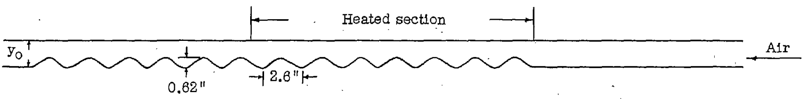
(b) System (2), large wave plate.
